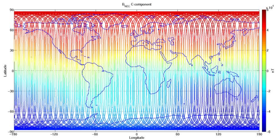
Figure 3-12: S/C C, world map plots of the geomagnetic field and components measured during monitoring period 22/10-28/10. From top to bottom: B_{NEC} components (North, East, and Centre) of magnetic field from VFM measurement.
