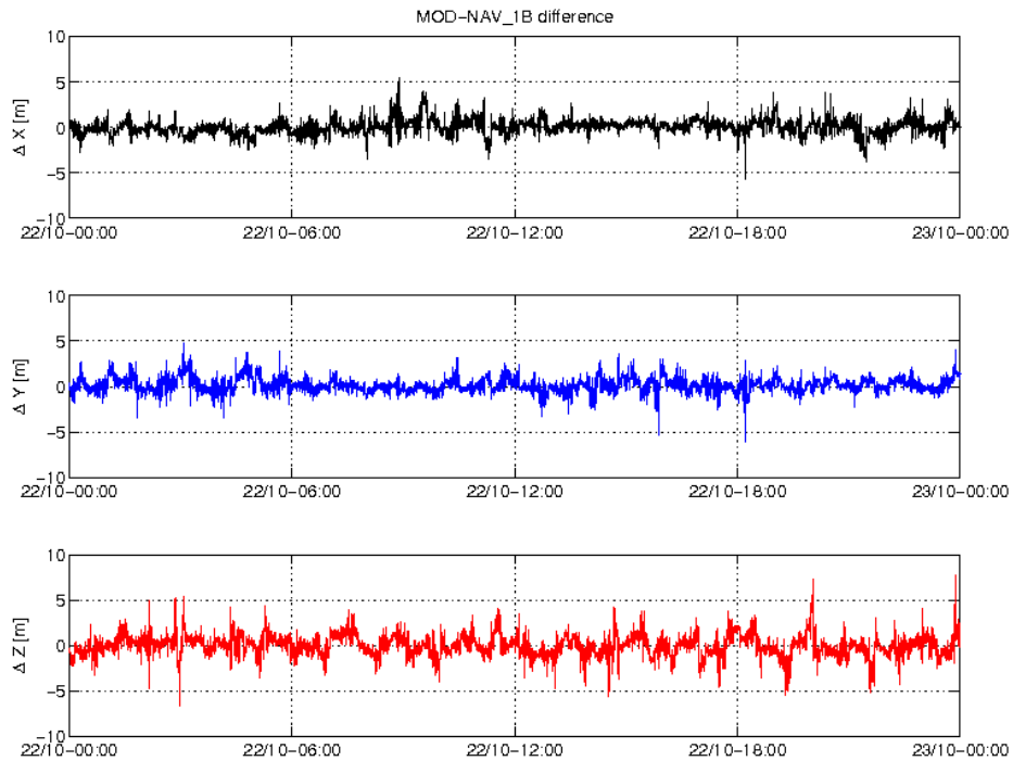
Figure 3-3: Difference MOD-GPSNAV, S/C A, 22.10. From top to bottom: X, Y and Z-axis
