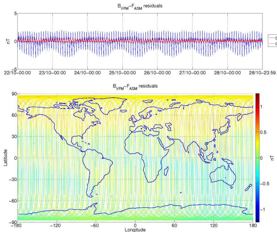
Figure 3-8: ASM-VFM residuals for S/C A, during monitoring period 22/10-28/10. In top figure are plotted: difference between |B_{VFM}| and F_{ASM} (without dB_{Sun} correction) (blue colour), and the residuals with dB_{Sun} corrections (red colour). In bottom figure residuals are presented on the world map.
