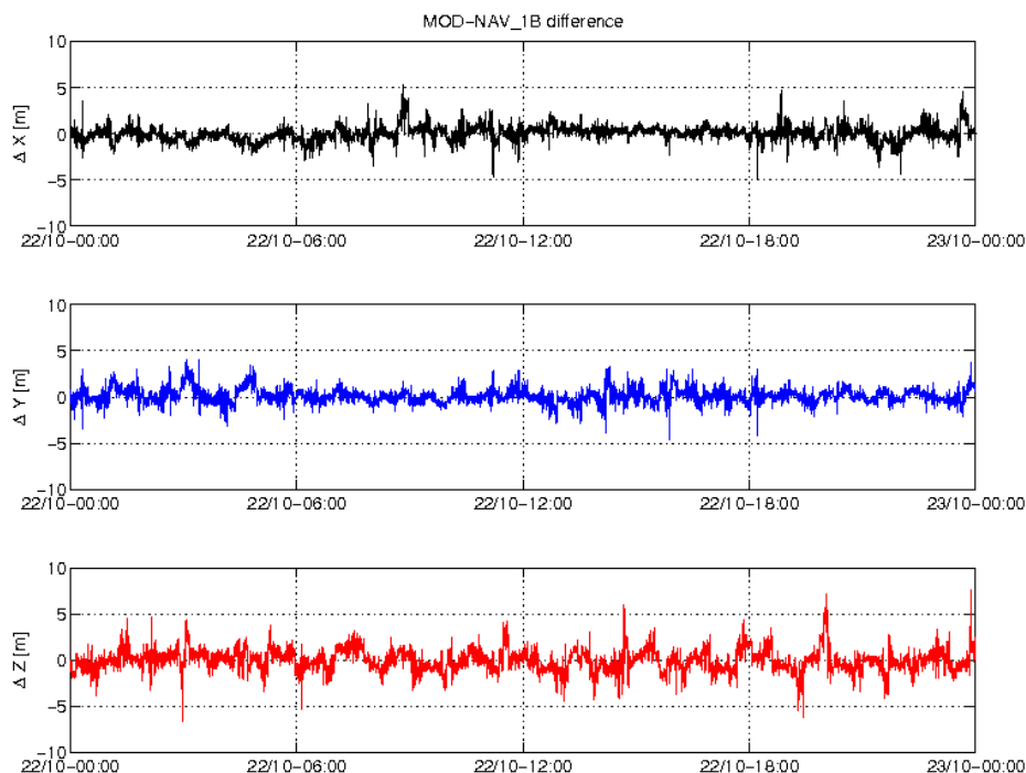
Figure 3-5: Difference MOD-GPSNAV, S/C C, 22.10. From top to bottom: X, Y and Z-axis
