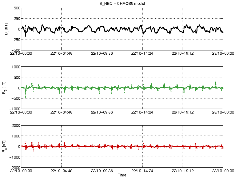
Figure 3-22: S/C C day 22.10 time series of B_{NEC} - B_{Chaos} residuals.
