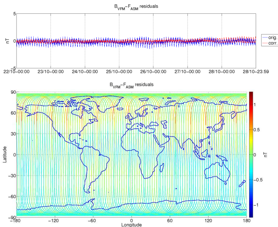
Figure 3-9: ASM-VFM residuals for S/C B, during monitoring period 22/10-28/10. In top figure are plotted: difference between |B\_VFM| and F\_ASM (without dB\_Sun correction) (blue colour), and the residuals with dB\_Sun corrections (red colour). In bottom figure residuals are presented on the world map.
