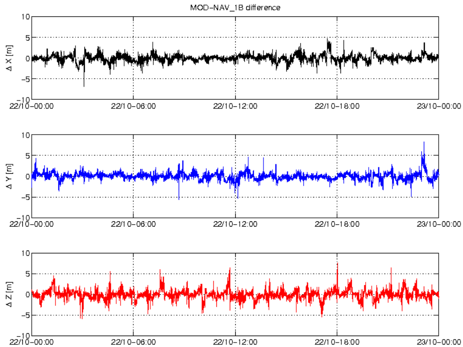
Figure 3-4: Difference MOD-GPSNAV, S/C B, 22.10. From top to bottom: X, Y and Z-axis
