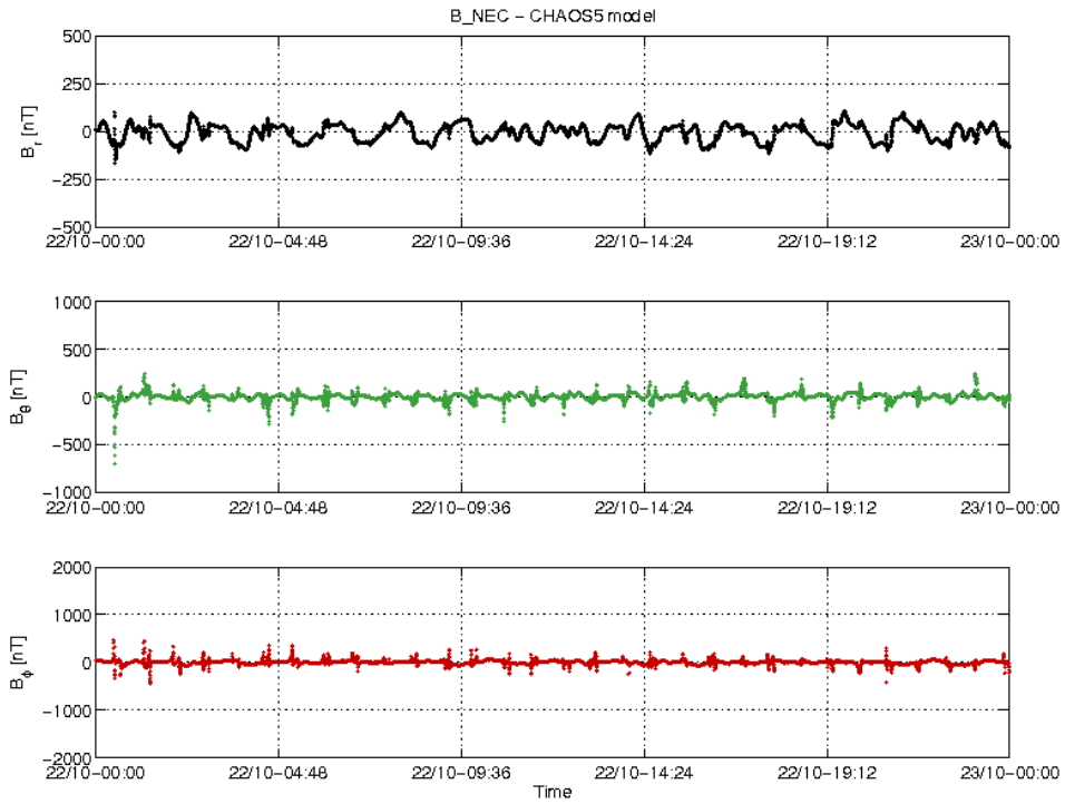
Figure 3-18: S/C A day 22.10: time series of B_{NEC} - B_{Chaos} residuals.
