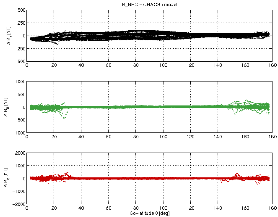
Figure 3-21: S/C C day 22.10 B_{NEC} - B_{Chaos} difference vs colatitude.
