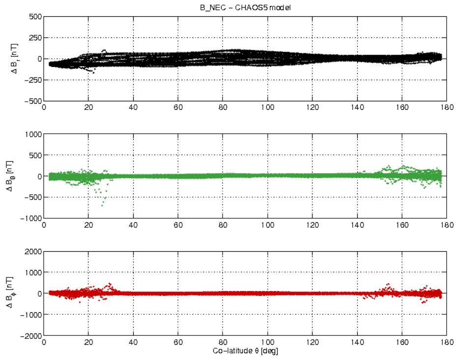
Figure 3-17: S/C A day 22.10 B_{NEC} - B_{Chaos} vs colatitude.
