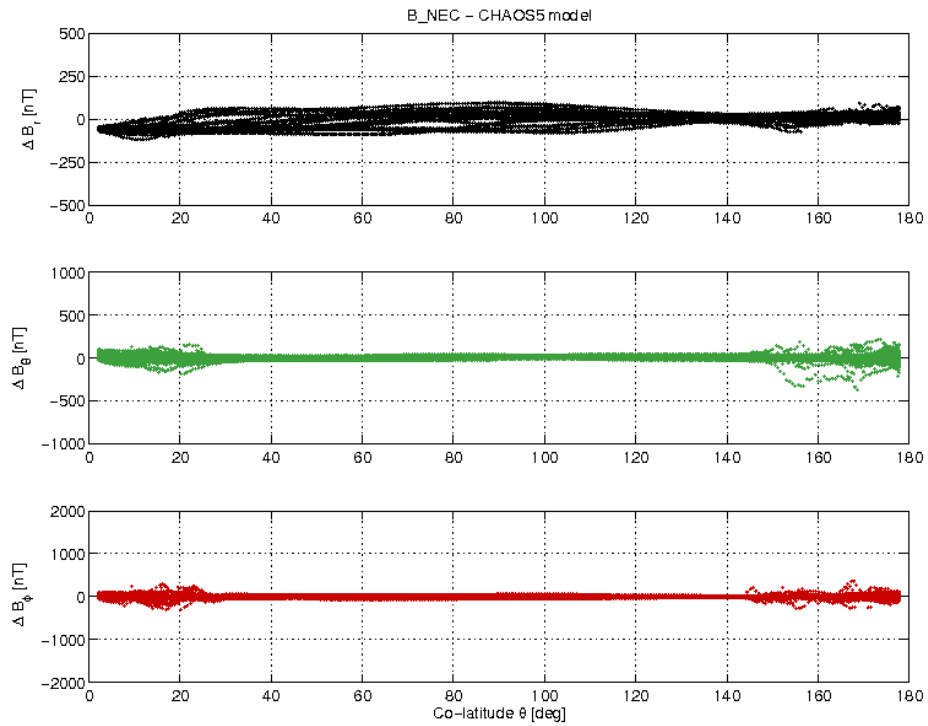
Figure 3-19: S/C B day 22.10 B_{NEC} - B_{Chaos} difference vs colatitude.
