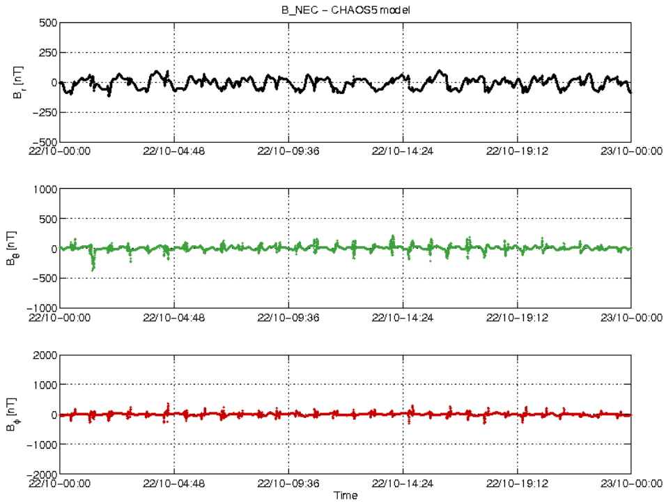
Figure 3-20: S/C B day 22.10 time series of B_{NEC} - B_{Chaos} residuals.
