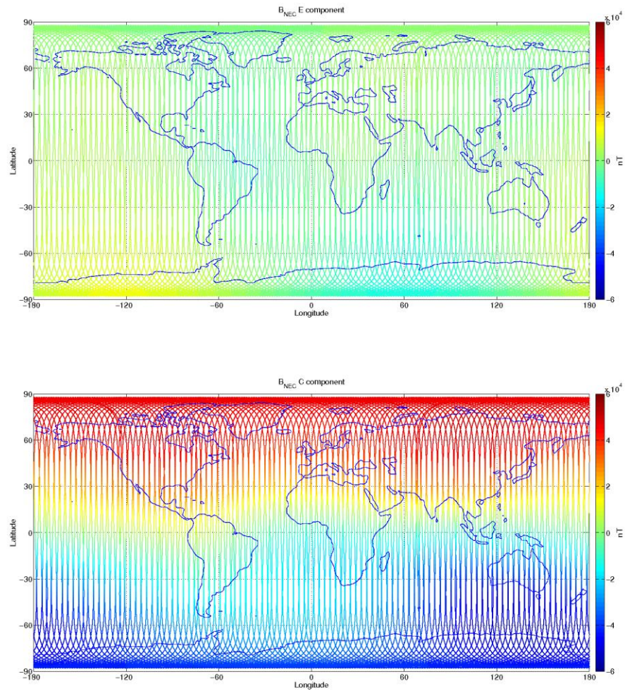
Figure 3-11: S/C B, world map plots of the geomagnetic field and components measured during monitoring period 22/10-28/10. From top to bottom: F-magnetic field from ASM measurement, B_{NEC} components (North, East, and Centre) of magnetic field from VFM measurement.
