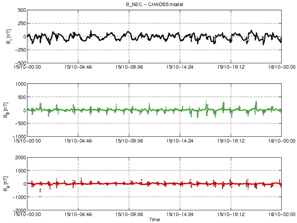
Figure 3-18: S/C A day 15.10: time series of B_{NEC} - B_{Chaos} residuals.
