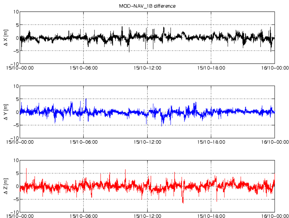
Figure 3-5: Difference MOD-GPSNAV, S/C C, 15.10. From top to bottom: X, Y and Z-axis
