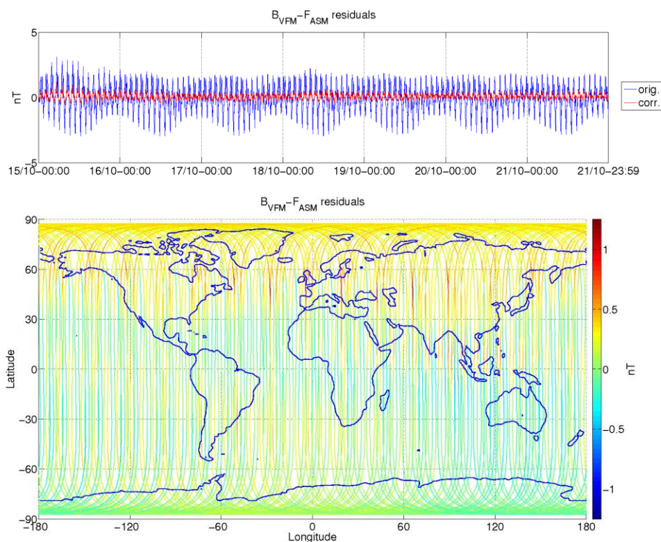
Figure 3-8: ASM-VFM residuals for S/C A, during monitoring period 15/10-21/10. In top figure are plotted: difference between |B_{VFM}| and F_{ASM} (without dB_{Sun} correction) (blue colour), and the residuals with dB_{Sun} corrections (red colour). In bottom figure residuals are presented on the world map.
