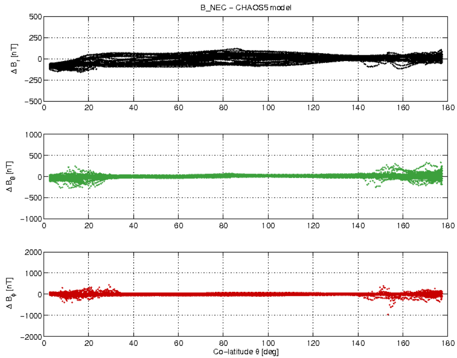
Figure 3-17: S/C A day 15.10 B_{NEC} - B_{Chaos} vs colatitude.
