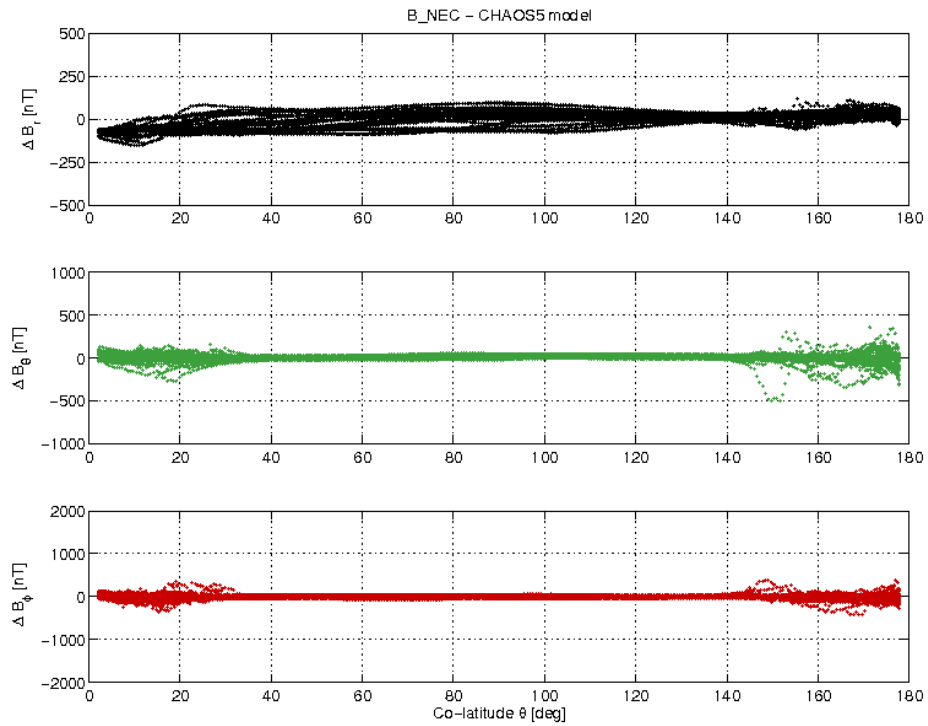
Figure 3-19: S/C B day 15.10 B_{NEC} - B_{Chaos} difference vs colatitude.
