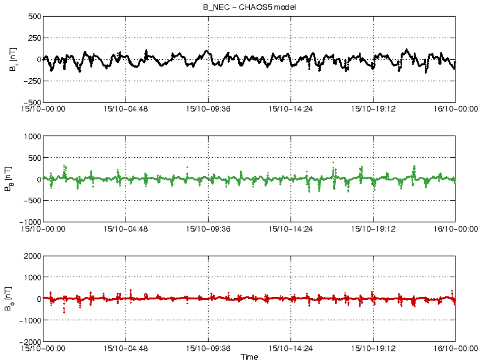
Figure 3-22: S/C C day 15.10 time series of B_{NEC} - B_{Chaos} residuals.
