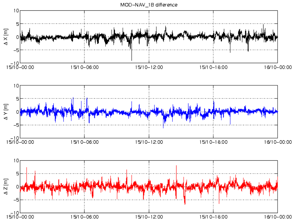
Figure 3-3: Difference MOD-GPSNAV, S/C A, 15.10. From top to bottom: X, Y and Z-axis
