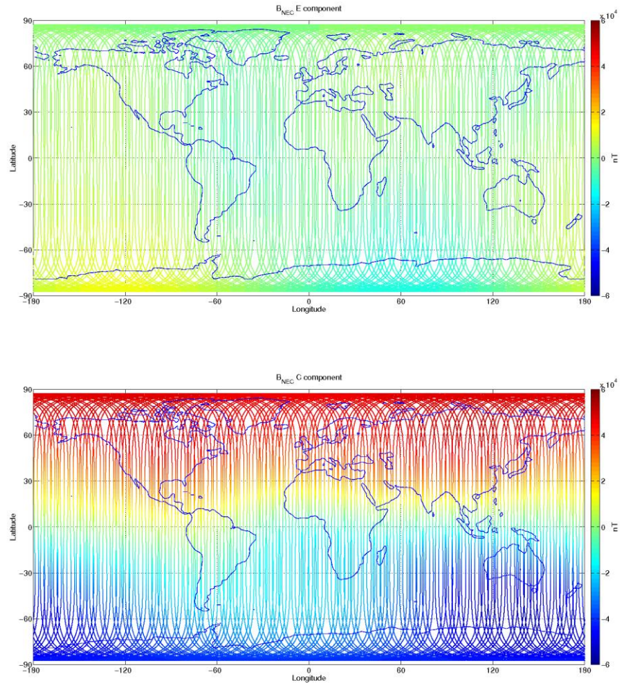
Figure 3-10: S/C A, world map plots of the geomagnetic field and components measured during monitoring period 15/10-21/10. From top to bottom: F-magnetic field from ASM measurement, B NEC components (North, East, and Centre) of magnetic field from VFM measurement.
