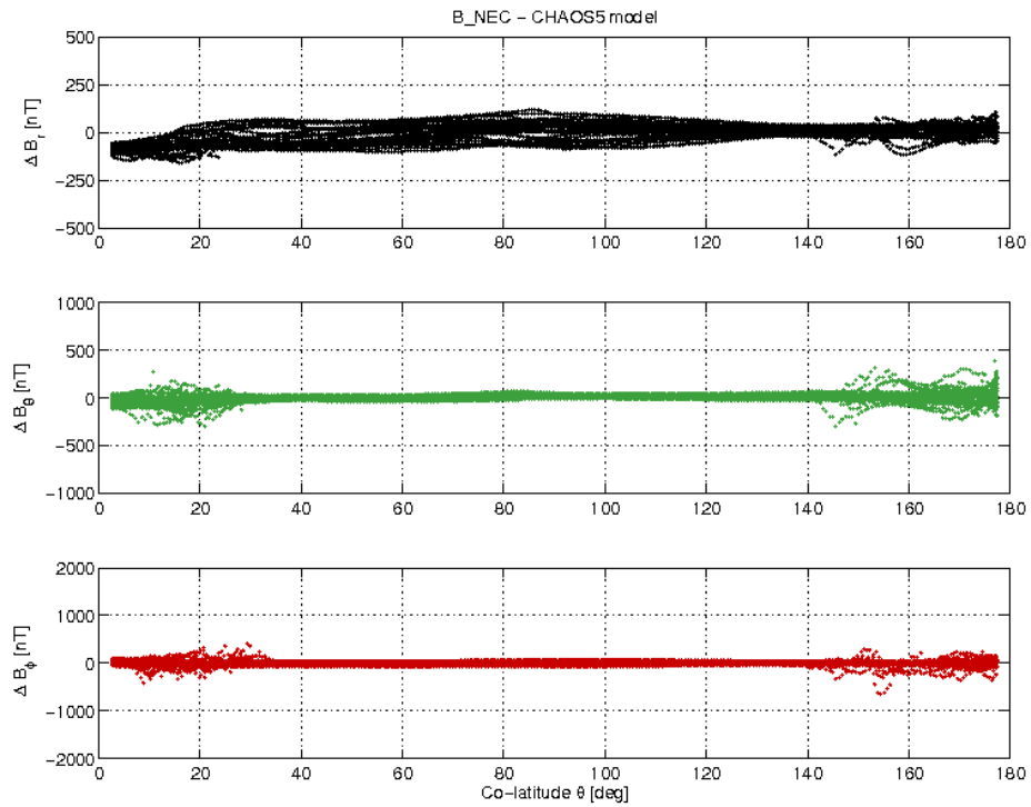
Figure 3-21: S/C C day 15.10 B_{NEC} - B_{Chaos} difference vs colatitude.
