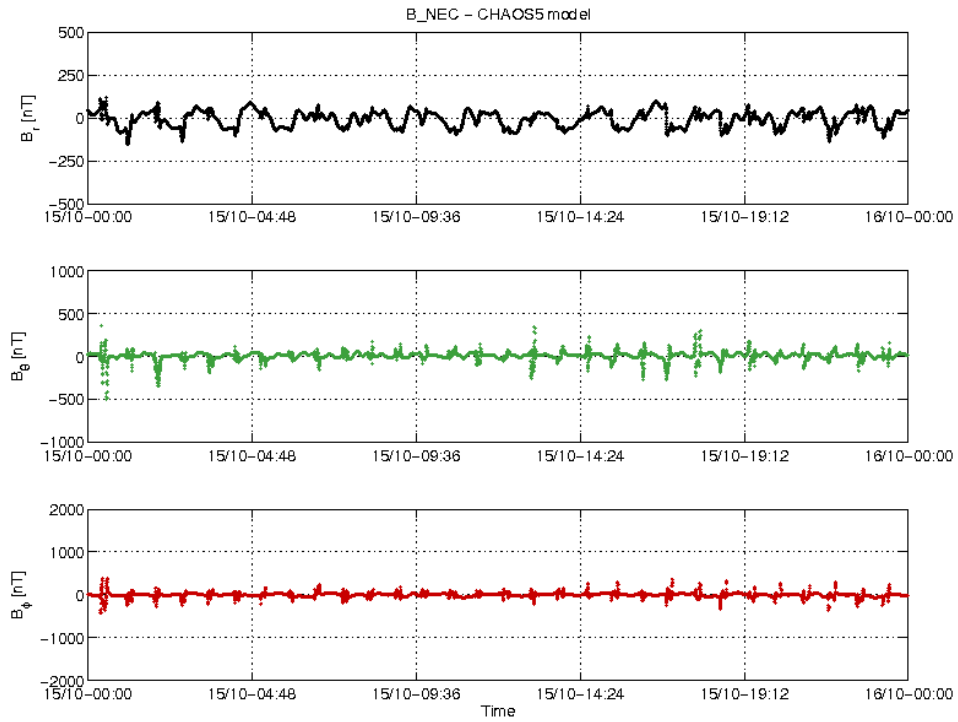
Figure 3-20: S/C B day 15.10 time series of B_{NEC} - B_{Chaos} residuals.
