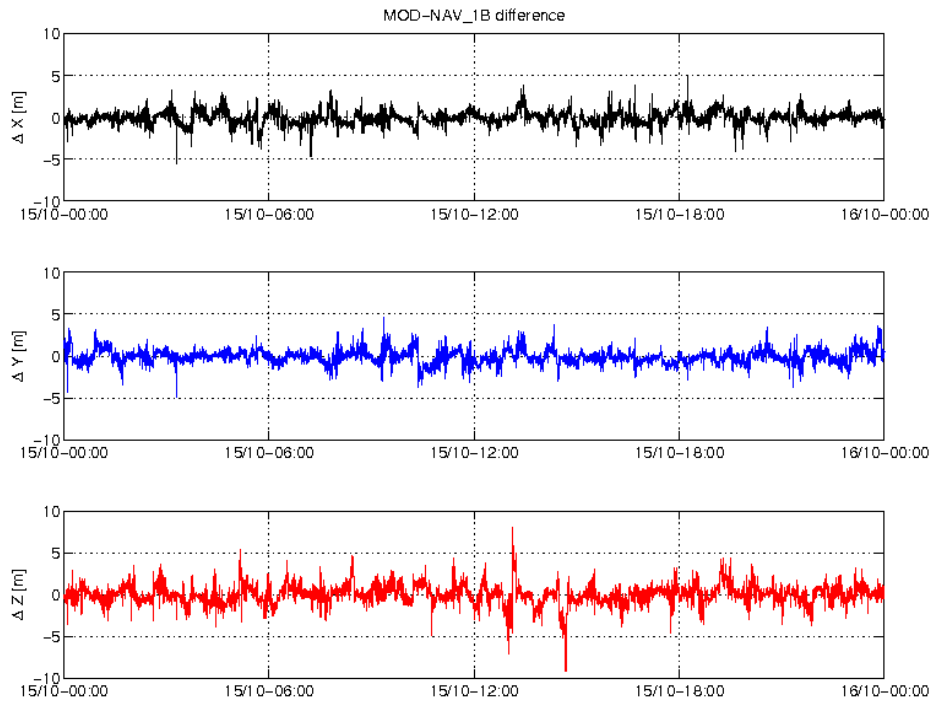
Figure 3-4: Difference MOD-GPSNAV, S/C B, 15.10. From top to bottom: X, Y and Z-axis
