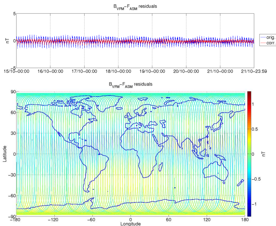
Figure 3-9: ASM-VFM residuals for S/C B, during monitoring period 15/10-21/10. In top figure are plotted: difference between |B\_VFM| and F\_ASM (without dB\_Sun correction) (blue colour), and the residuals with dB\_Sun corrections (red colour). In bottom figure residuals are presented on the world map.
