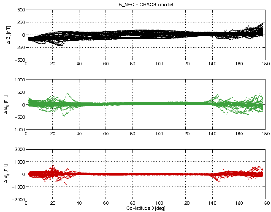
Figure 3-19: S/C B day 08.10 B_{NEC} - B_{Chaos} difference vs colatitude.
