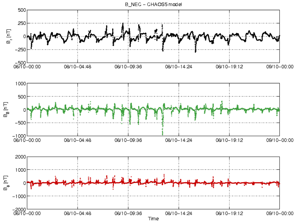
Figure 3-18: S/C A day 08.10: time series of B_{NEC} - B_{Chaos} residuals.
