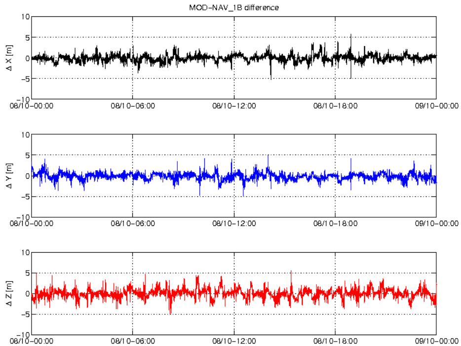
Figure 3-4: Difference MOD-GPSNAV, S/C B, 08.10. From top to bottom: X, Y and Z-axis
