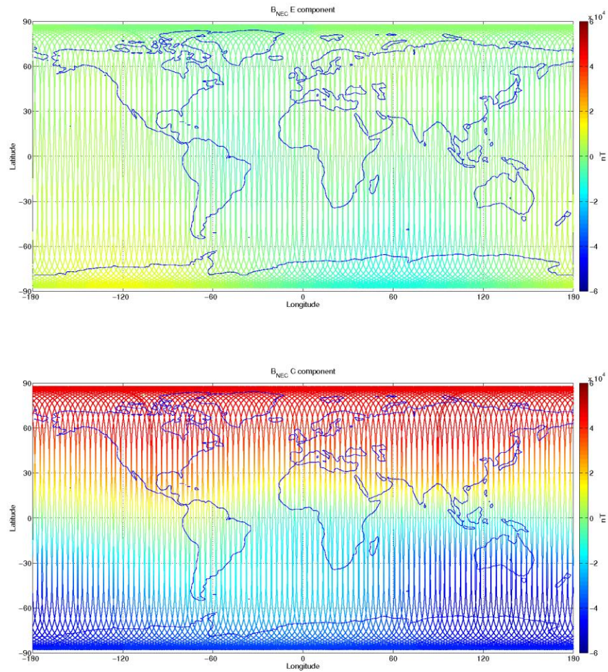
Figure 3-11: S/C B, world map plots of the geomagnetic field and components measured during monitoring period 08/10-14/10. From top to bottom: F-magnetic field from ASM measurement, B_{NEC} components (North, East, and Centre) of magnetic field from VFM measurement.
