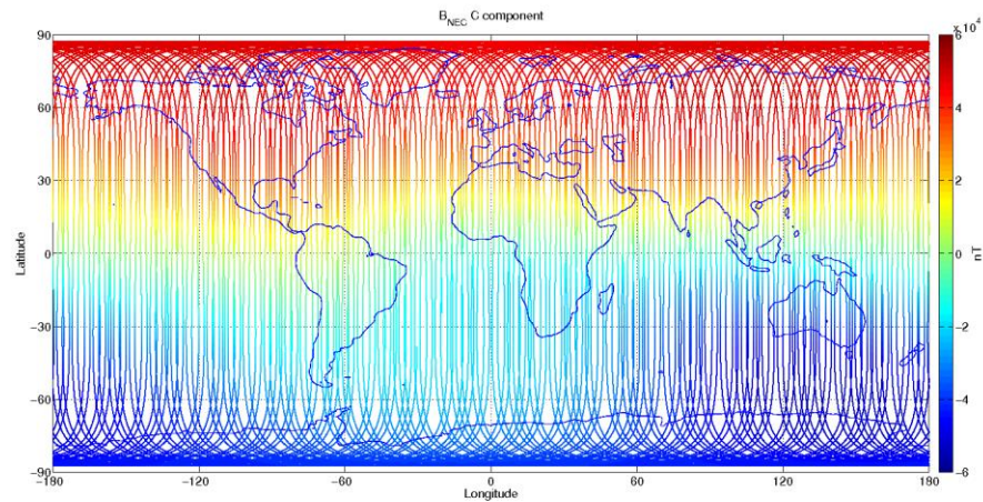
Figure 3-12: S/C C, world map plots of the geomagnetic field and components measured during monitoring period 08/10-14/10. From top to bottom: B_{NEC} components (North, East, and Centre) of magnetic field from VFM measurement.
