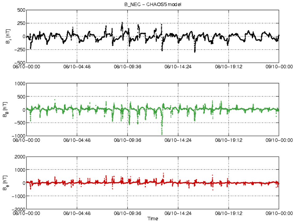
Figure 3-22: S/C C day 08.10 time series of B_{NEC} - B_{Chaos} residuals.
