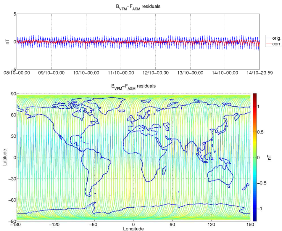
Figure 3-9: ASM-VFM residuals for S/C B, during monitoring period 08/10-14/10. In top figure are plotted: difference between |B_{VFM}| and F_{ASM} (without dB_{Sun} correction) (blue colour), and the residuals with dB_{Sun} corrections (red colour). In bottom figure residuals are presented on the world map.
