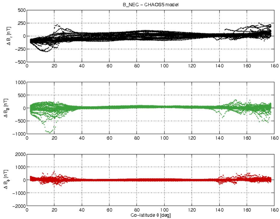
Figure 3-17: S/C A day 08.10 B_{NEC} - B_{Chaos} vs colatitude.
