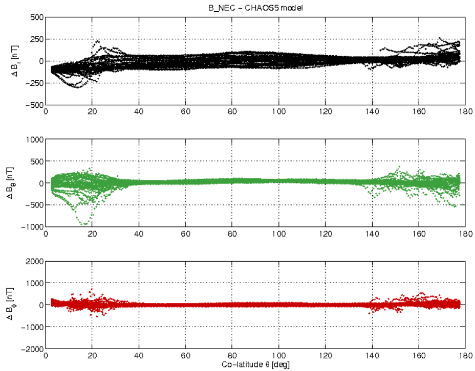
Figure 3-21: S/C C day 08.10 B_{NEC} - B_{Chaos} difference vs colatitude.
