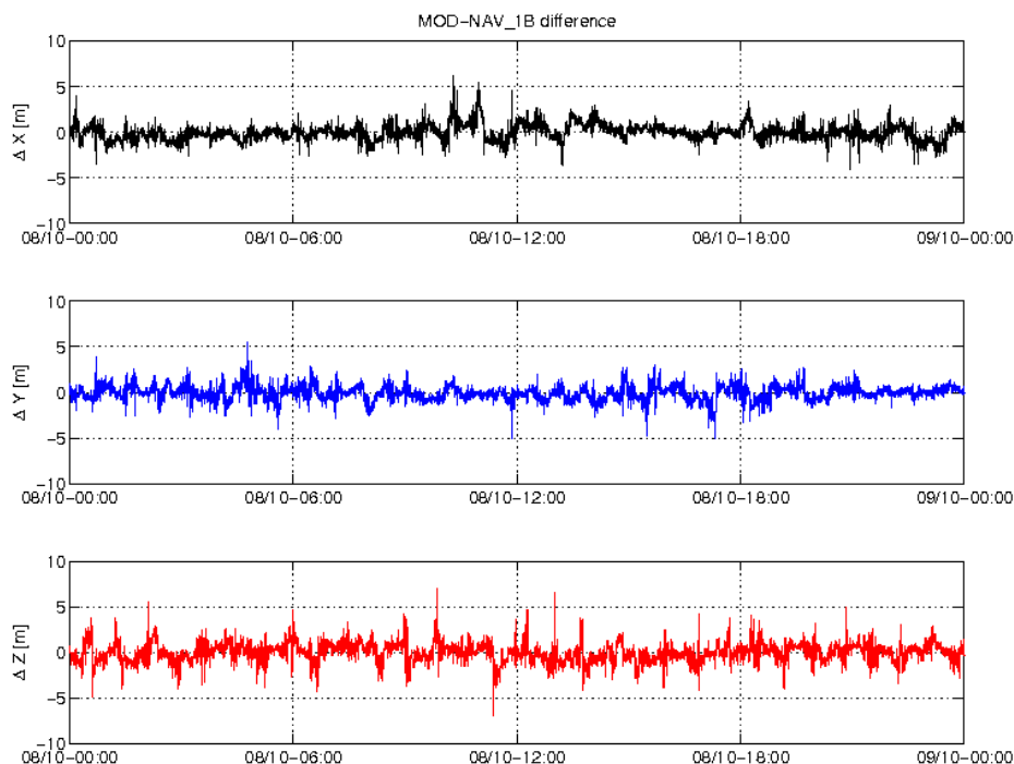
Figure 3-5: Difference MOD-GPSNAV, S/C C, 08.10. From top to bottom: X, Y and Z-axis
