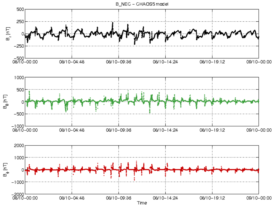
Figure 3-20: S/C B day 08.10 time series of B_{NEC} - B_{Chaos} residuals.
