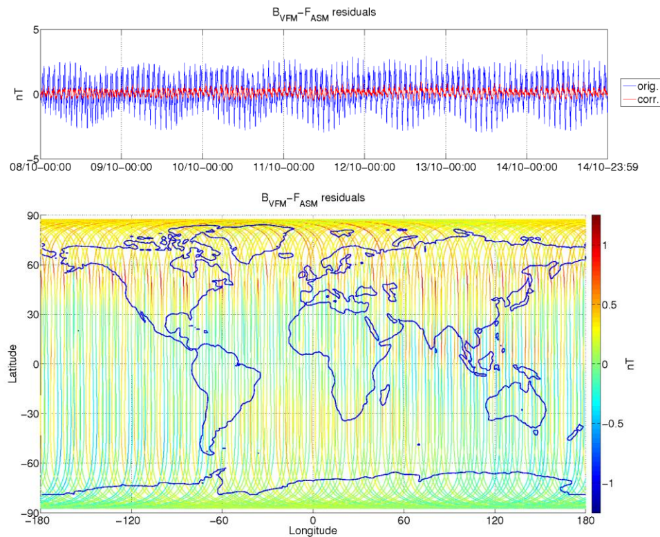
Figure 3-8: ASM-VFM residuals for S/C A, during monitoring period 08/10-14/10. In top figure are plotted: difference between |B VFM | and F ASM (without dB Sun correction) (blue colour), and the residuals with dB Sun corrections (red colour). In bottom figure residuals are presented on the world map.
