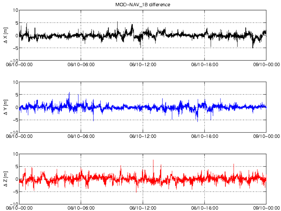
Figure 3-3: Difference MOD-GPSNAV, S/C A, 08.10. From top to bottom: X, Y and Z-axis
