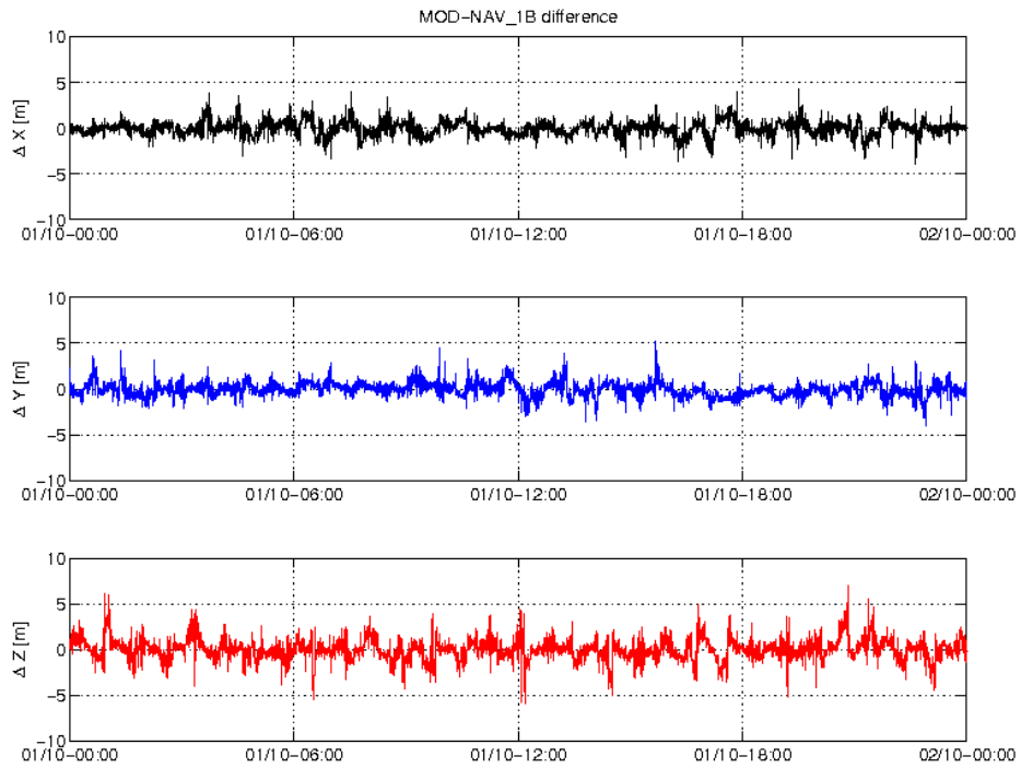
Figure 3-4: Difference MOD-GPSNAV, S/C B, 01.10. From top to bottom: X, Y and Z-axis
