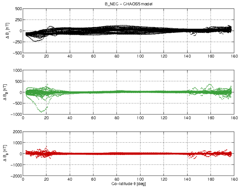
Figure 3-21: S/C C day 01.10 B_{NEC} - B_{Chaos} difference vs colatitude.
