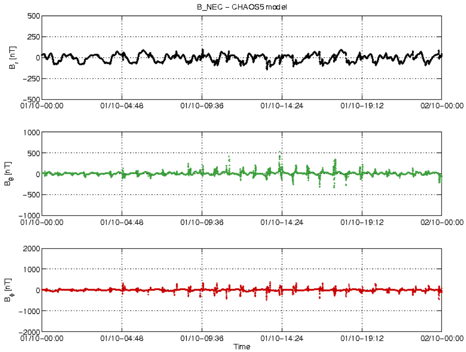
Figure 3-20: S/C B day 01.10 time series of B_{NEC} - B_{Chaos} residuals.
