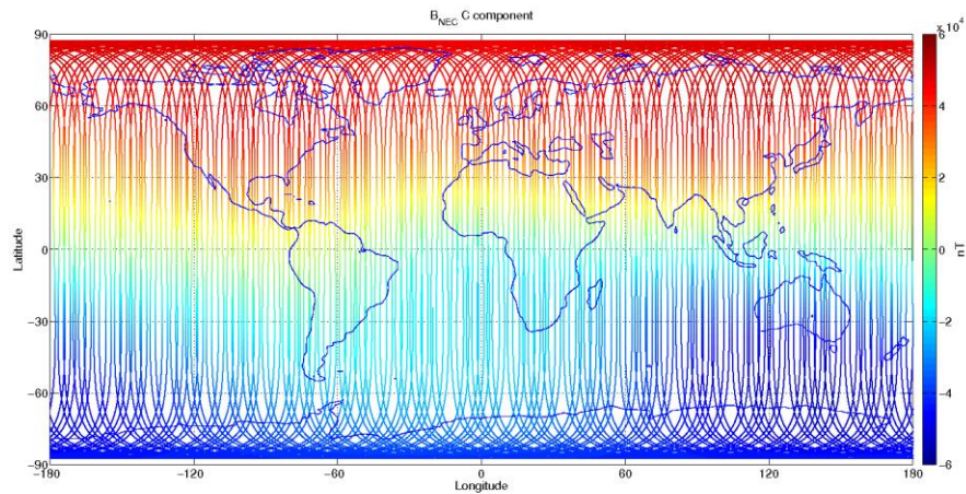
Figure 3-12: S/C C, world map plots of the geomagnetic field and components measured during monitoring period 01/10-07/10. From top to bottom: B_{NEC} components (North, East, and Centre) of magnetic field from VFM measurement.
