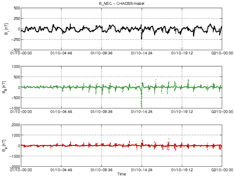
Figure 3-22: S/C C day 01.10 time series of B_{NEC} - B_{Chaos} residuals.
