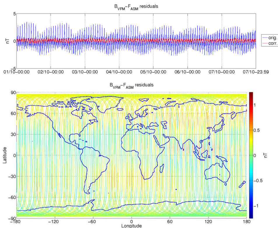
Figure 3-8: ASM-VFM residuals for S/C A, during monitoring period 01/10-07/10. In top figure are plotted: difference between |B_{VFM}| and F_{ASM} (without dB_{Sun} correction) (blue colour), and the residuals with dB_{Sun} corrections (red colour). In bottom figure residuals are presented on the world map.
