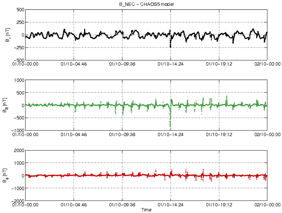
Figure 3-18: S/C A day 01.10: time series of B_{NEC} - B_{Chaos} residuals.
