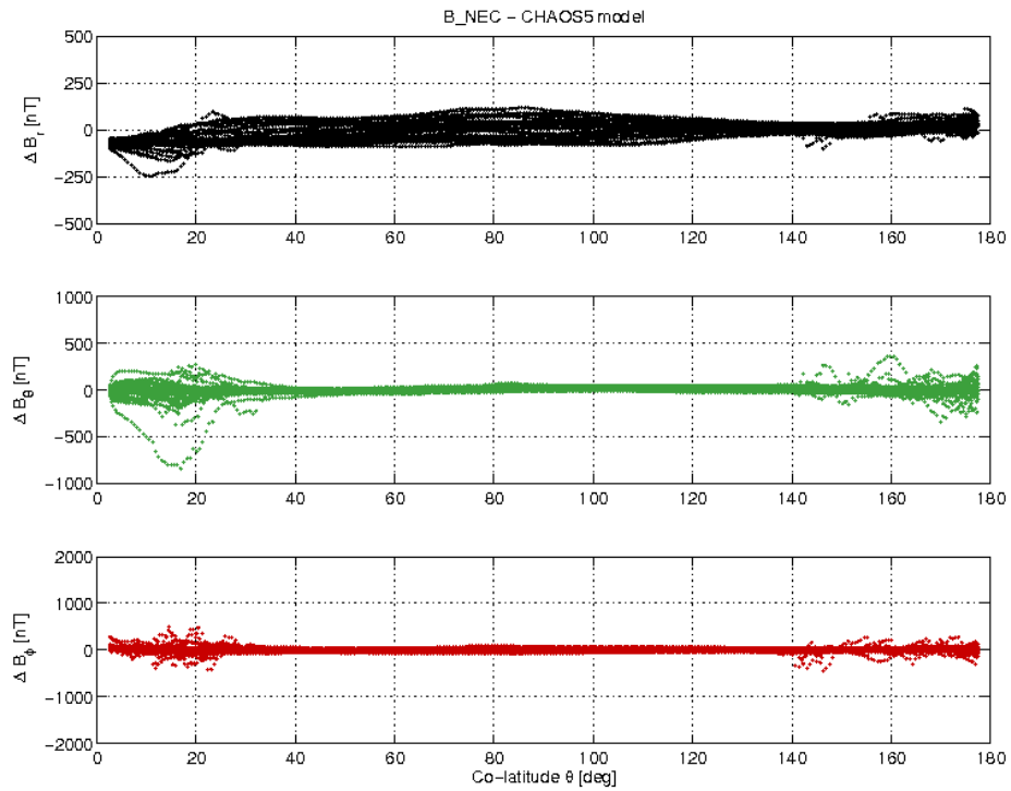
Figure 3-17: S/C A day 01.10 B_{NEC} - B_{Chaos} vs colatitude.
