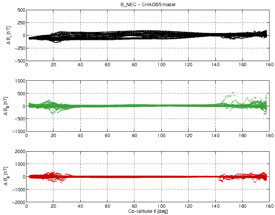
Figure 3-19: S/C B day 01.10 B_{NEC} - B_{Chaos} difference vs colatitude.
