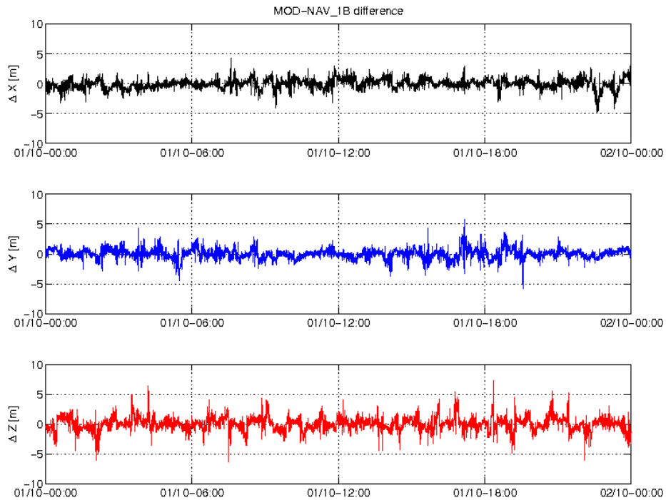
Figure 3-3: Difference MOD-GPSNAV, S/C A, 01.10. From top to bottom: X, Y and Z-axis
