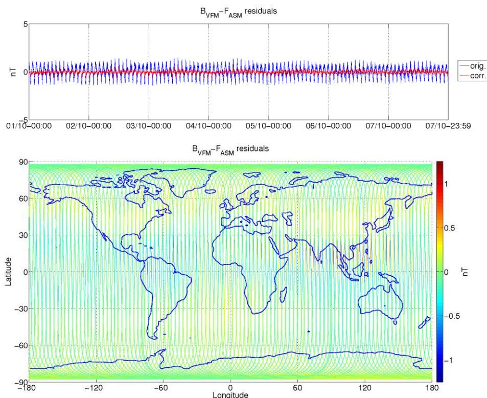
Figure 3-9: ASM-VFM residuals for S/C B, during monitoring period 01/10-07/10. In top figure are plotted: difference between |B_{VFM}| and F_{ASM} (without dB_{Sun} correction) (blue colour), and the residuals with dB_{Sun} corrections (red colour). In bottom figure residuals are presented on the world map.
