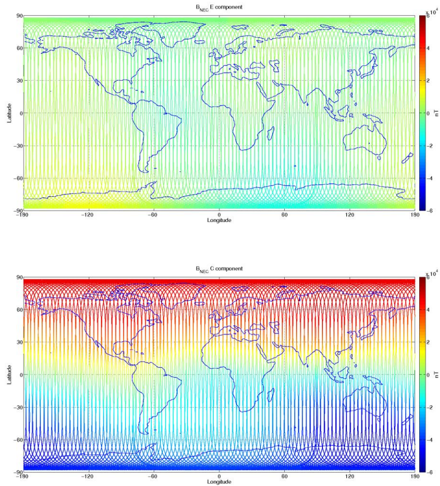
Figure 3-11: S/C B, world map plots of the geomagnetic field and components measured during monitoring period 01/10-07/10. From top to bottom: F-magnetic field from ASM measurement, B_{NEC} components (North, East, and Centre) of magnetic field from VFM measurement.
