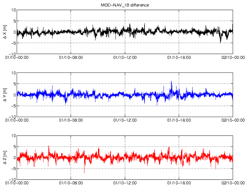
Figure 3-5: Difference MOD-GPSNAV, S/C C, 01.10. From top to bottom: X, Y and Z-axis
