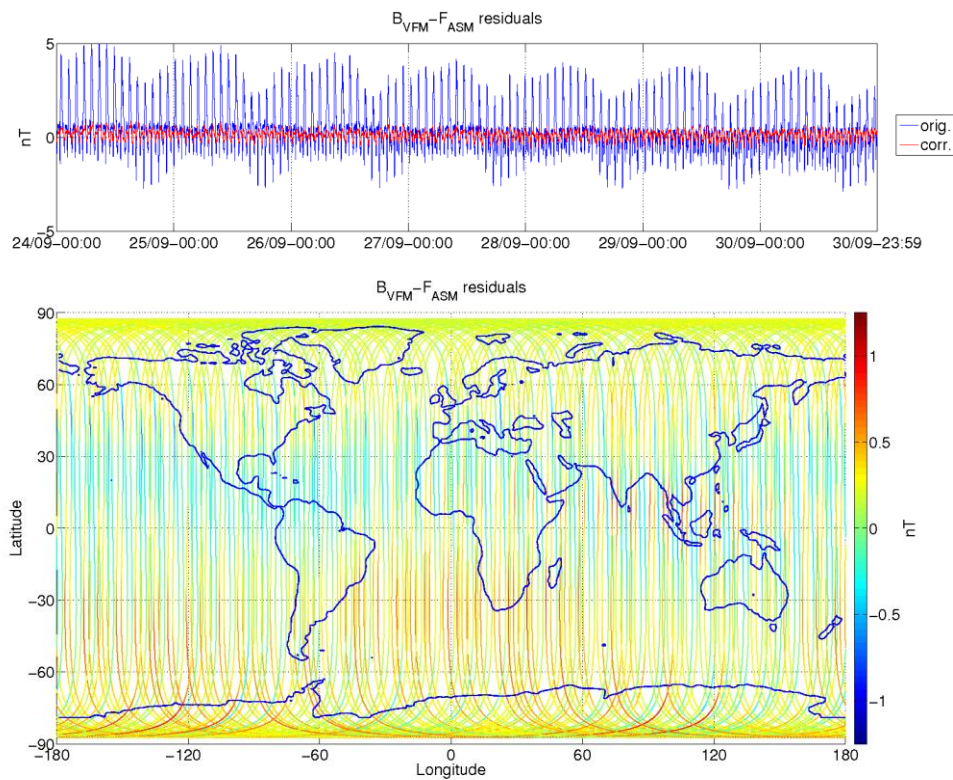
Figure 3-8: ASM-VFM residuals for S/C A, during monitoring period 24/09-30/09. In top figure are plotted: difference between |B_{VFM}| and F_{ASM} (without dB_{Sun} correction) (blue colour), and the residuals with dB_{Sun} corrections (red colour). In bottom figure residuals are presented on the world map.
