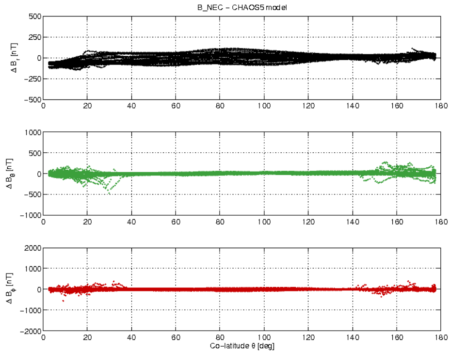
Figure 3-21: S/C C day 24.09 B_{NEC} - B_{Chaos} difference vs colatitude.
