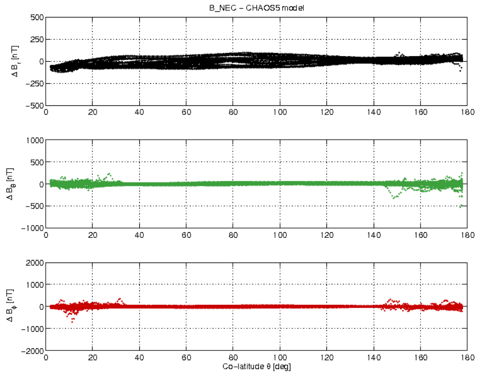
Figure 3-19: S/C B day 24.09 B_{NEC} - B_{Chaos} difference vs colatitude.
