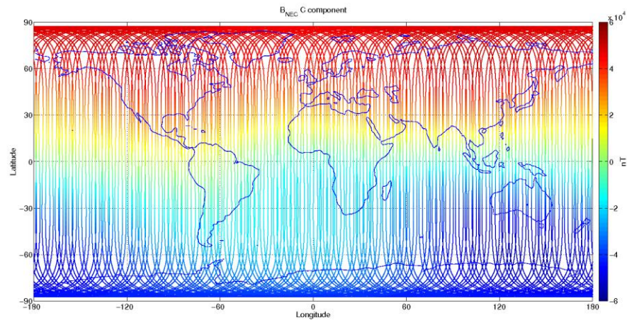
Figure 3-12: S/C C, world map plots of the geomagnetic field and components measured during monitoring period 24/09-30/09. From top to bottom: B_{NEC} components (North, East, and Centre) of magnetic field from VFM measurement.
