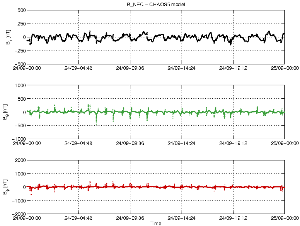
Figure 3-22: S/C C day 24.09 time series of B_{NEC} - B_{Chaos} residuals.
