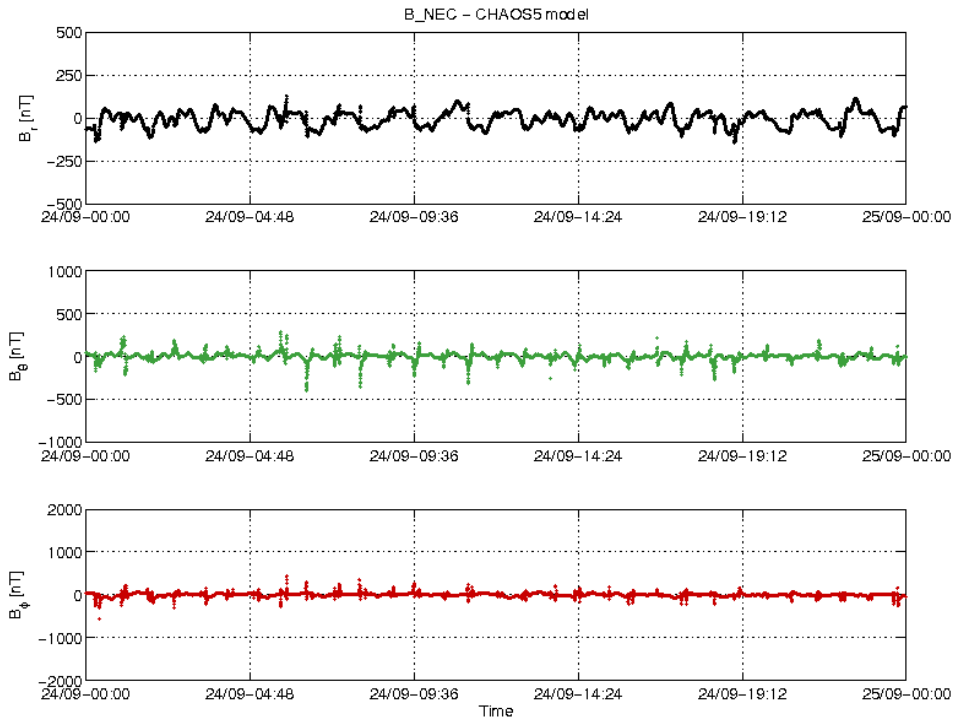
Figure 3-18: S/C A day 24.09: time series of B_{NEC} - B_{Chaos} residuals.
