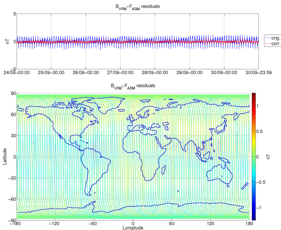
Figure 3-9: ASM-VFM residuals for S/C B, during monitoring period 24/09-30/09. In top figure are plotted: difference between |B_{VFM}| and F_{ASM} (without dB_Sun correction) (blue colour), and the residuals with dB_Sun corrections (red colour). In bottom figure residuals are presented on the world map.
