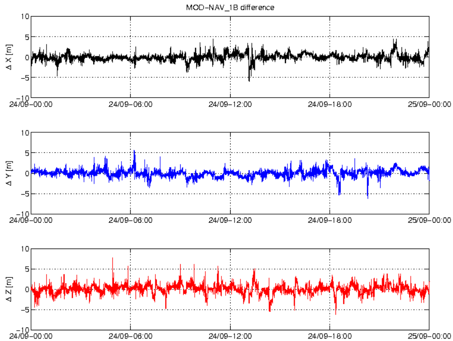
Figure 3-3: Difference MOD-GPSNAV, S/C A, 24.09. From top to bottom: X, Y and Z-axis
