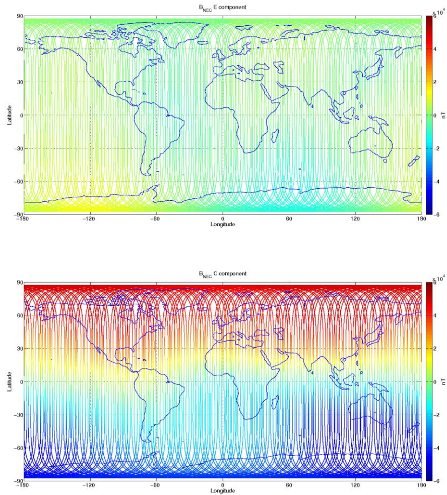
Figure 3-10: S/C A, world map plots of the geomagnetic field and components measured during monitoring period 24/09-30/09. From top to bottom: F-magnetic field from ASM measurement, B_{NEC} components (North, East, and Centre) of magnetic field from VFM measurement.
