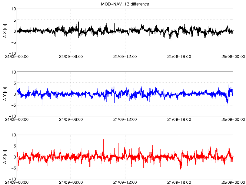
Figure 3-4: Difference MOD-GPSNAV, S/C B, 24.09. From top to bottom: X, Y and Z-axis
