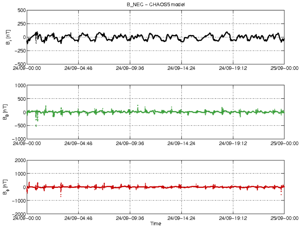
Figure 3-20: S/C B day 24.09 time series of B_{NEC} - B_{Chaos} residuals.
