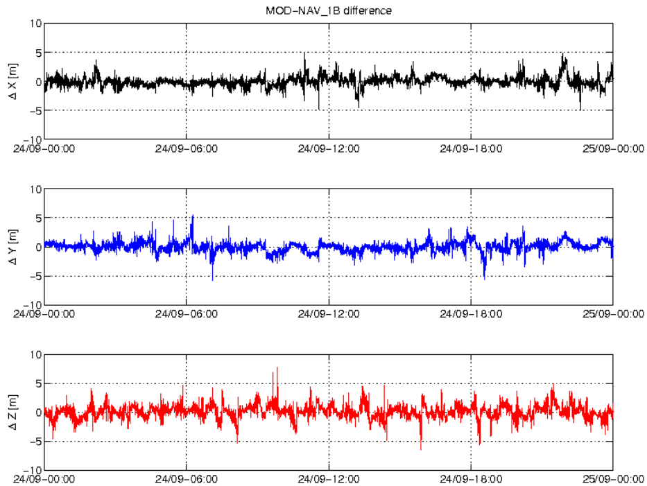
Figure 3-5: Difference MOD-GPSNAV, S/C C, 24.09. From top to bottom: X, Y and Z-axis
