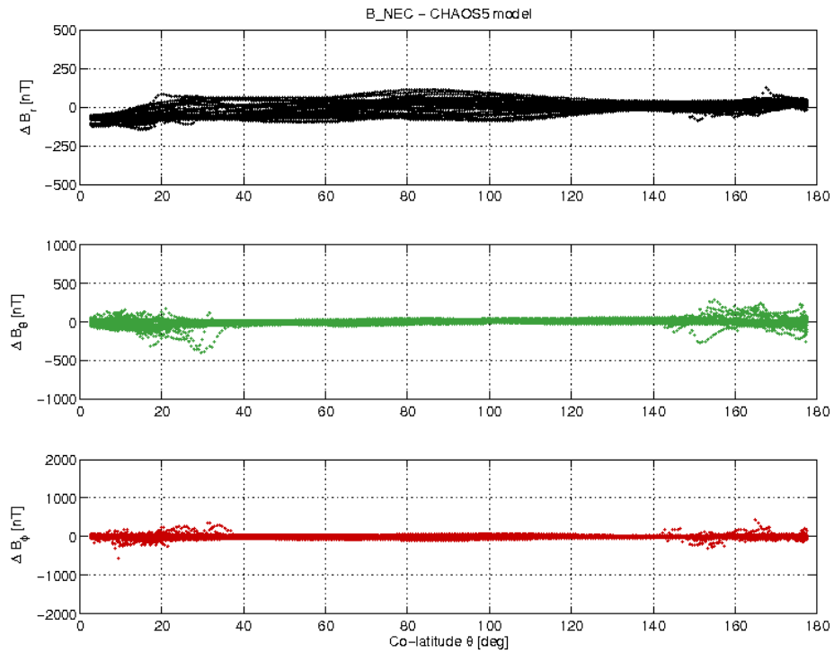
Figure 3-17: S/C A day 24.09 B_{NEC} - B_{Chaos} vs colatitude.
