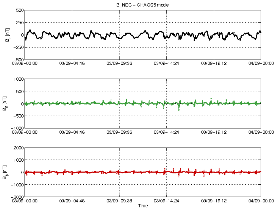
Figure 3-22: S/C C day 03.09 time series of B_{NEC} - B_{Chaos} residuals.
