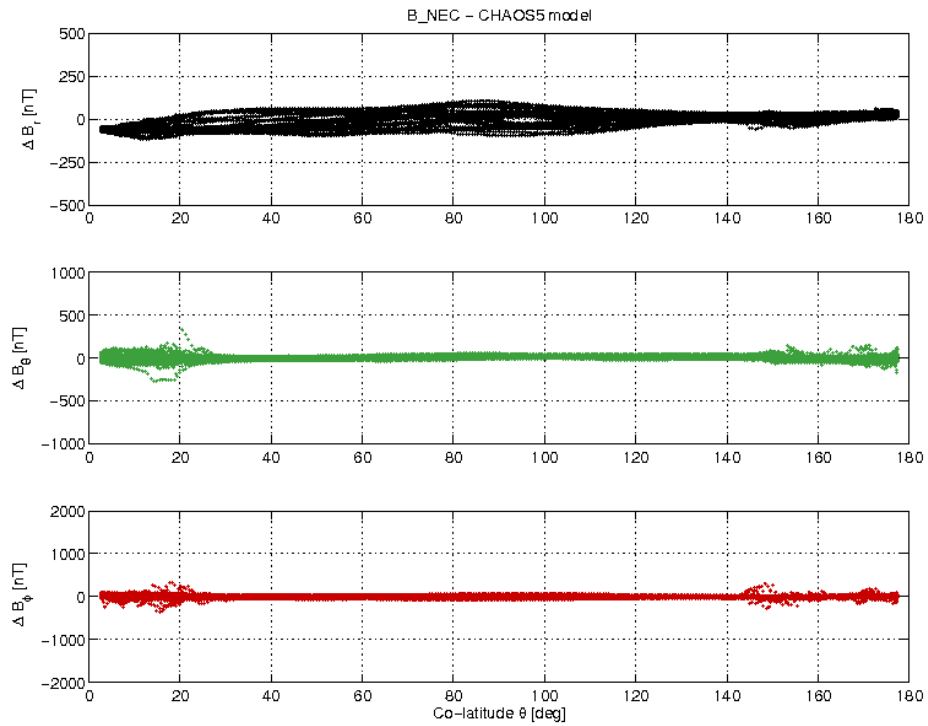
Figure 3-17: S/C A day 03.09 B_{NEC} - B_{Chaos} vs colatitude.
