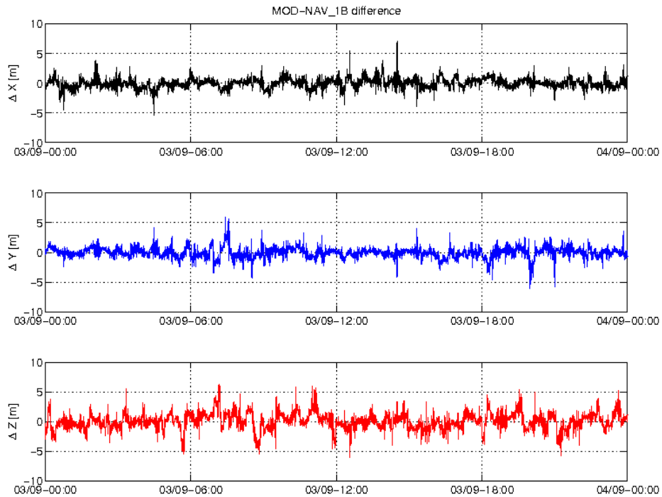
Figure 3-5: Difference MOD-GPSNAV, S/C C, 03.09. From top to bottom: X, Y and Z-axis
