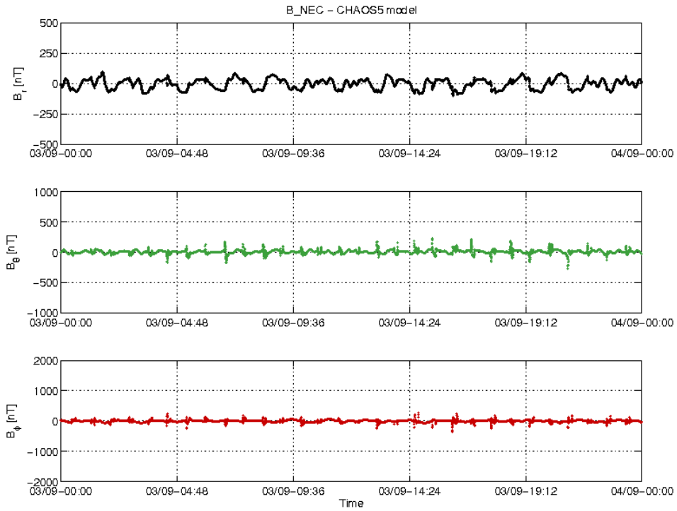
Figure 3-20: S/C B day 03.09 time series of B_{NEC} - B_{Chaos} residuals.
