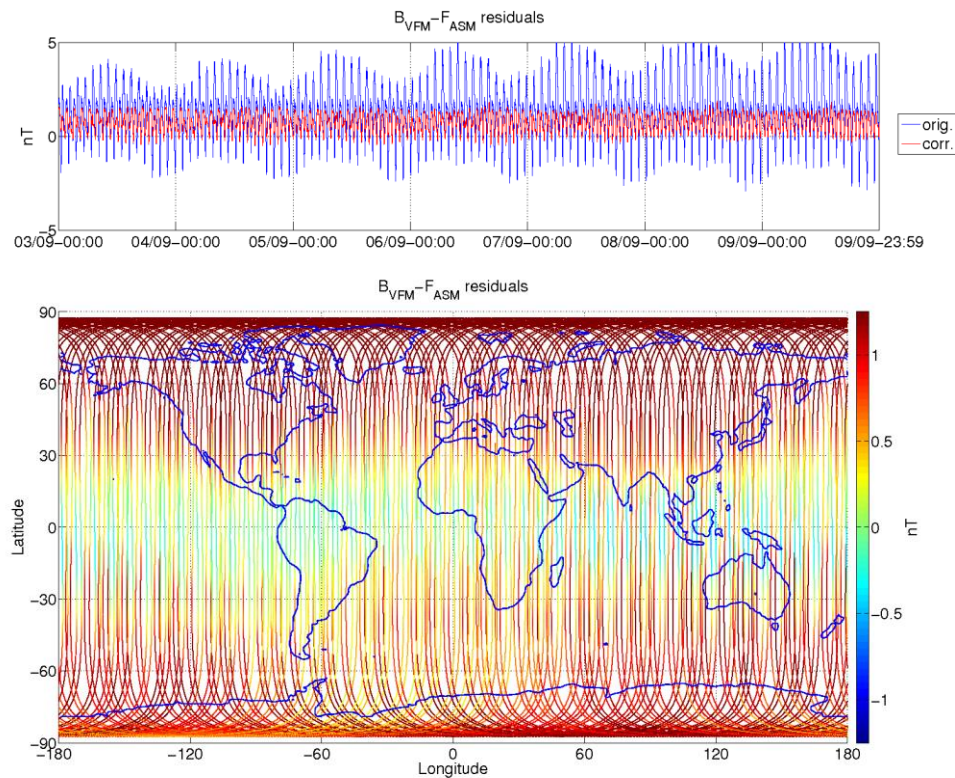
Figure 3-8: ASM-VFM residuals for S/C A, during monitoring period 03/09-09/09. In top figure are plotted: difference between |B VFM | and F ASM (without dB Sun correction) (blue colour), and the residuals with dB Sun corrections (red colour). In bottom figure residuals are presented on the world map.
