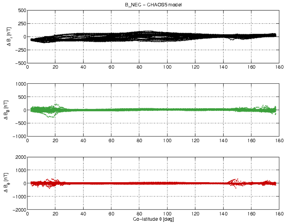
Figure 3-21: S/C C day 03.09 B_{NEC} - B_{Chaos} difference vs colatitude.
