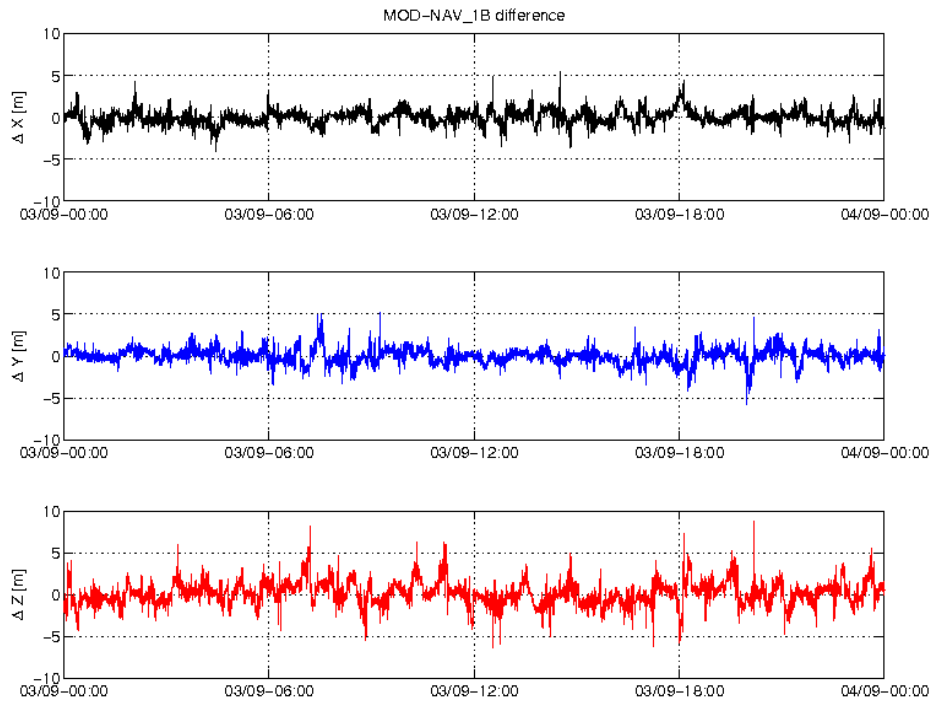
Figure 3-3: Difference MOD-GPSNAV, S/C A, 03.09. From top to bottom: X, Y and Z-axis
