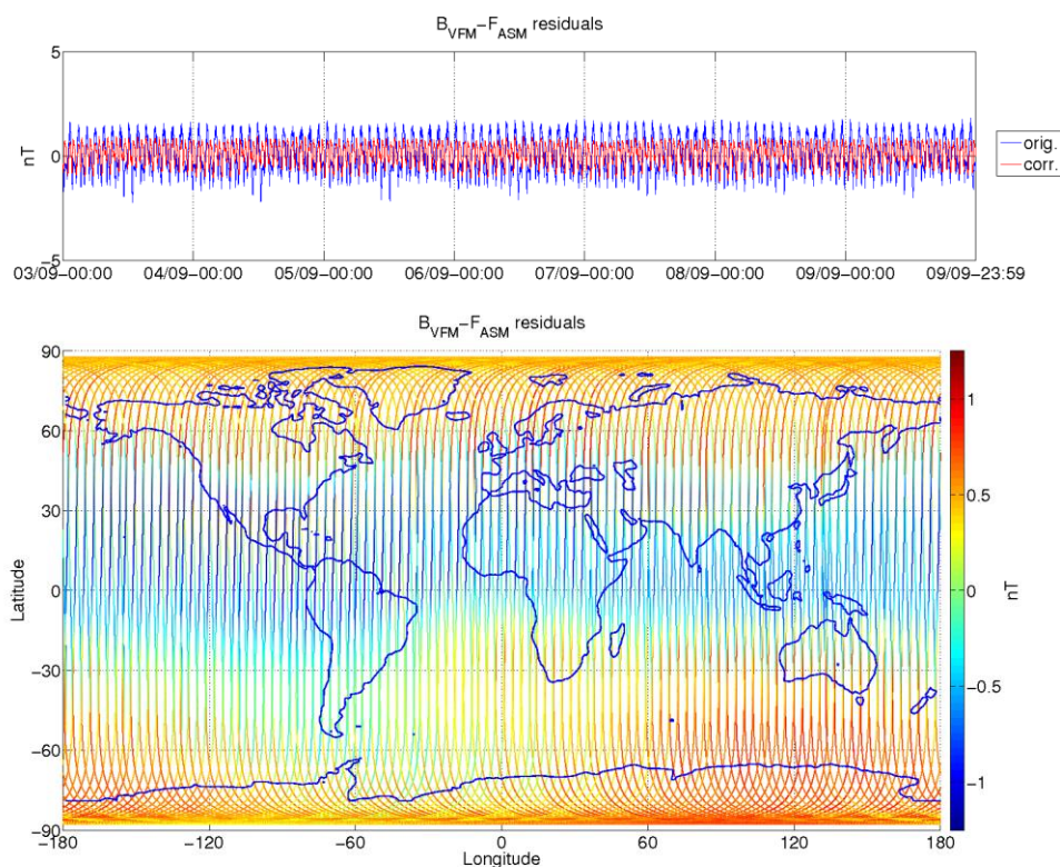
Figure 3-9: ASM-VFM residuals for S/C B, during monitoring period 03/09-09/09. In top figure are plotted: difference between |B_{VFM}| and F_{ASM} (without dB Sun correction) (blue colour), and the residuals with dB Sun corrections (red colour). In bottom figure residuals are presented on the world map.
