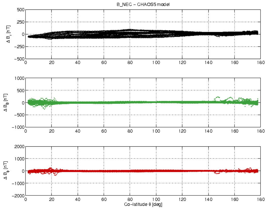
Figure 3-19: S/C B day 03.09 B_{NEC} - B_{Chaos} difference vs colatitude.
