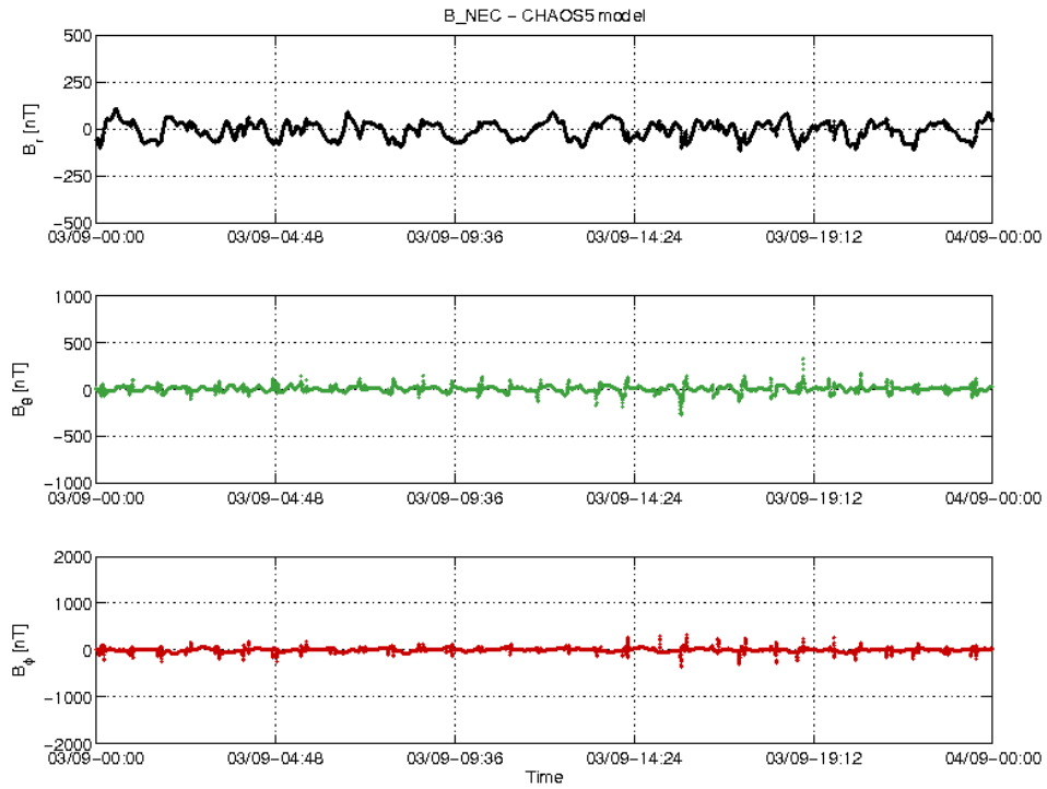
Figure 3-18: S/C A day 03.09: time series of B_{NEC} - B_{Chaos} residuals.
