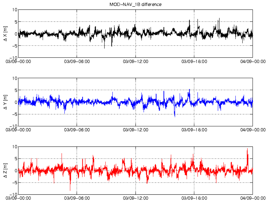
Figure 3-4: Difference MOD-GPSNAV, S/C B, 03.09. From top to bottom: X, Y and Z-axis
