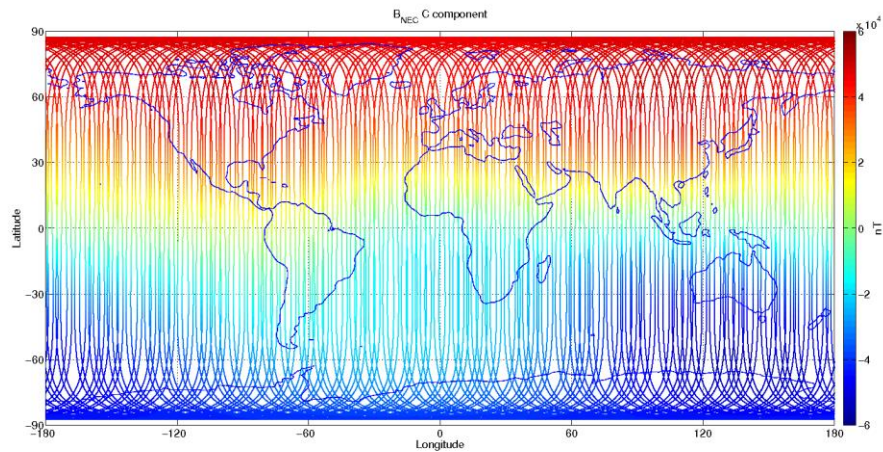
Figure 3-12: S/C C, world map plots of the geomagnetic field and components measured during monitoring period 03/09-09/09. From top to bottom: B_{NEC} components (North, East, and Centre) of magnetic field from VFM measurement.
