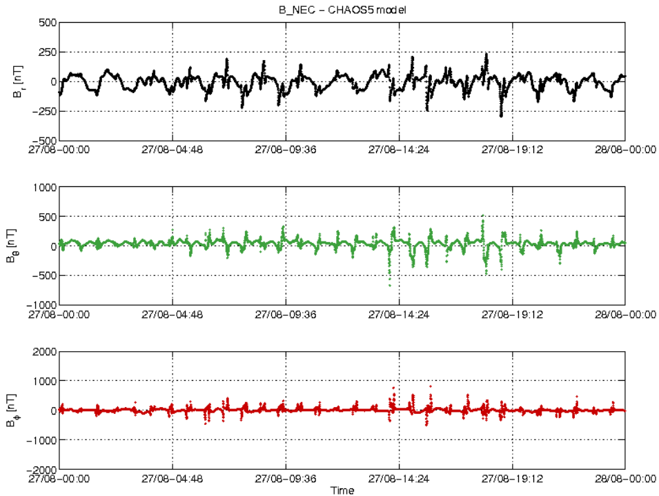
Figure 3-20: S/C C day 27.08 time series of B_{NEC} - B_{Chaos} residuals.
