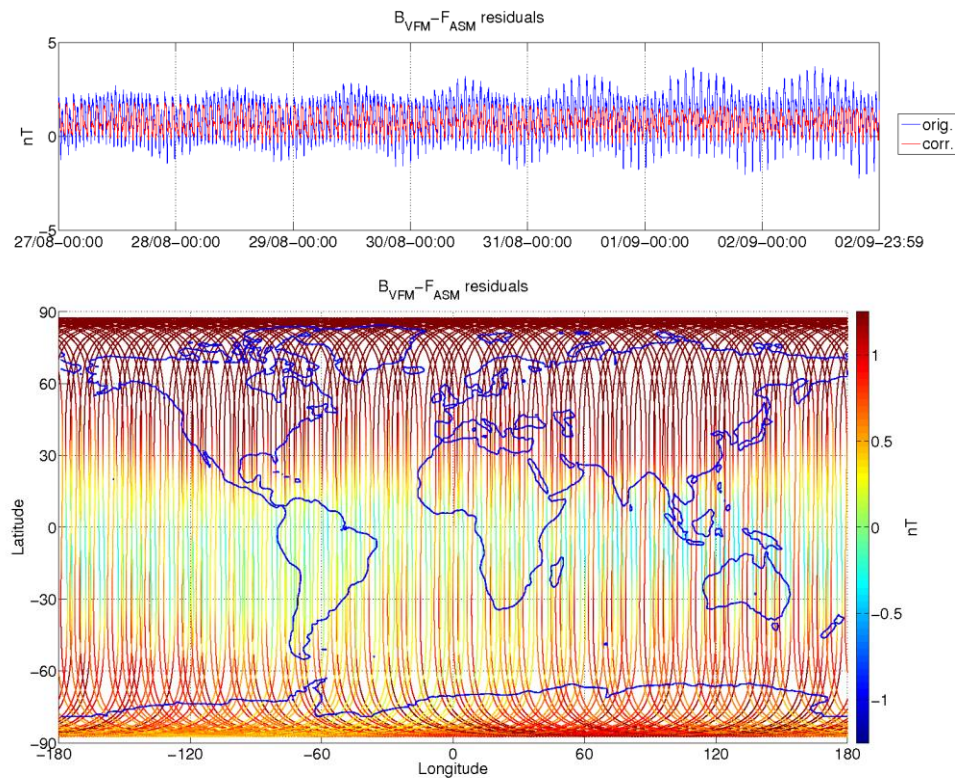
Figure 3-8: ASM-VFM residuals for S/C A, during monitoring period 27/08-02/09. In top figure are plotted: difference between |B VFM | and F ASM (without dB Sun correction) (blue colour), and the residuals with dB Sun corrections (red colour). In bottom figure residuals are presented on the world map.
