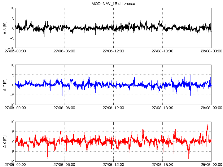
Figure 3-3: Difference MOD-GPSNAV, S/C A, 27.08. From top to bottom: X, Y and Z-axis
