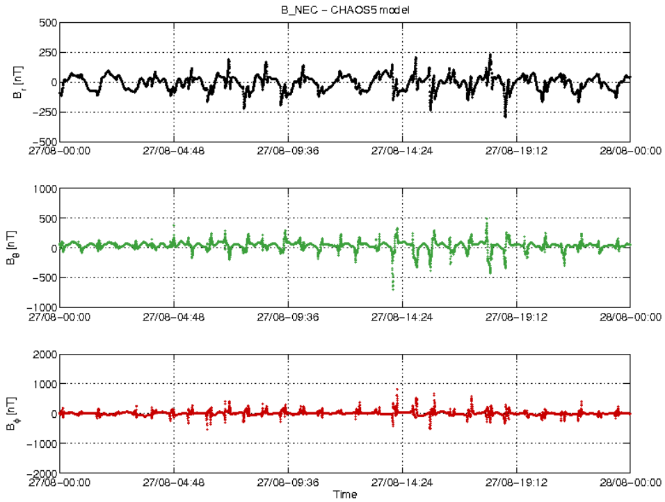
Figure 3-18: S/C A day 27.08: time series of B_{NEC} - B_{Chaos} residuals.
