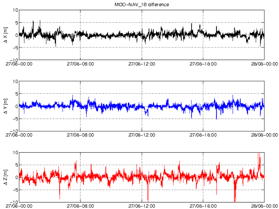
Figure 3-5: Difference MOD-GPSNAV, S/C C, 27.08. From top to bottom: X, Y and Z-axis
