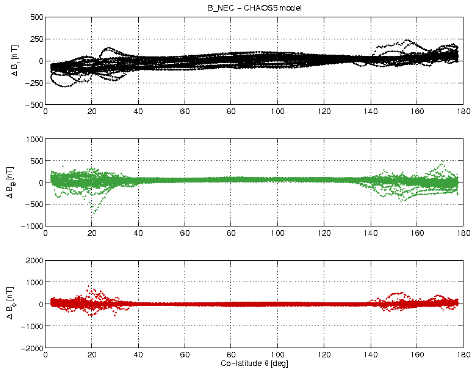
Figure 3-17: S/C A day 27.08 B_{NEC} - B_{Chaos} vs colatitude.
