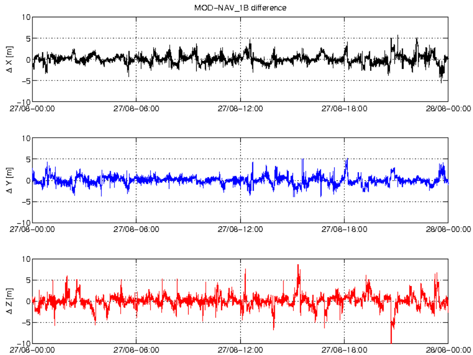
Figure 3-4: Difference MOD-GPSNAV, S/C B, 27.08. From top to bottom: X, Y and Z-axis
