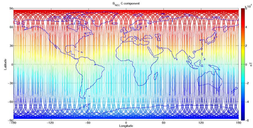
Figure 3-12: S/C C, world map plots of the geomagnetic field and components measured during monitoring period 27/08-02/09. From top to bottom: B_{NEC} components (North, East, and Centre) of magnetic field from VFM measurement.
