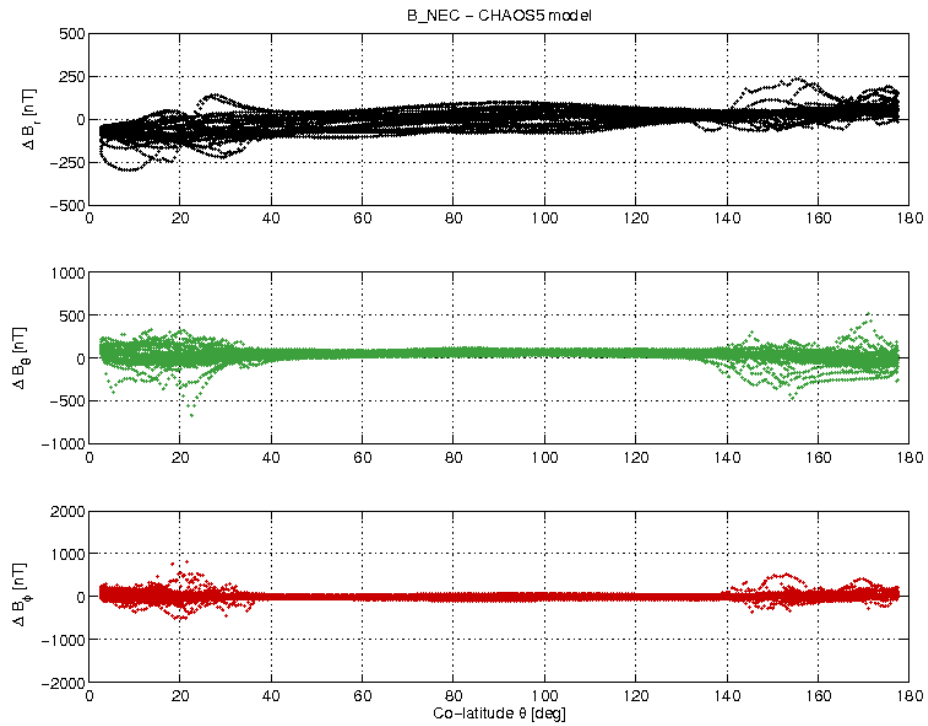
Figure 3-19: S/C C day 27.08 B_{NEC} - B_{Chaos} difference vs colatitude.
