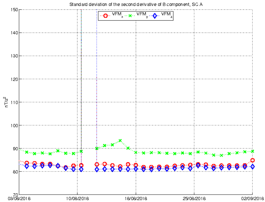
Figure 3-21: Standard deviation of the second derivative of B component
