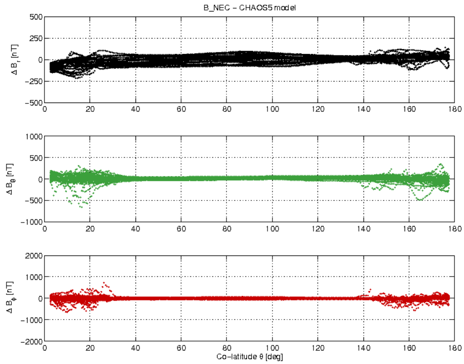
Figure 3-17: S/C C day 20.08 B_{NEC} - B_{Chaos} difference vs colatitude.
