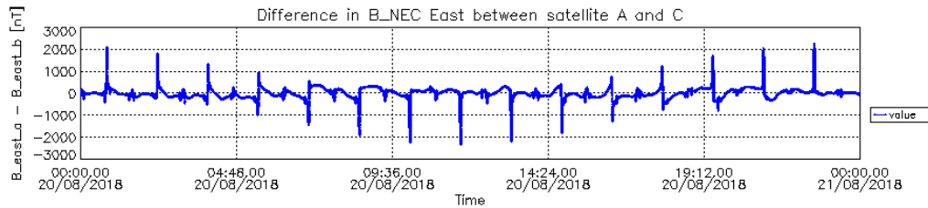
Figure 3-13: Difference in B_{NEC} East component between S/C A and S/C C.
