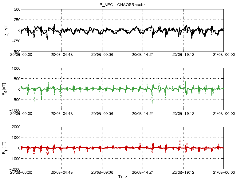
Figure 3-18: S/C C day 20.08 time series of B_{NEC} - B_{Chaos} residuals.
