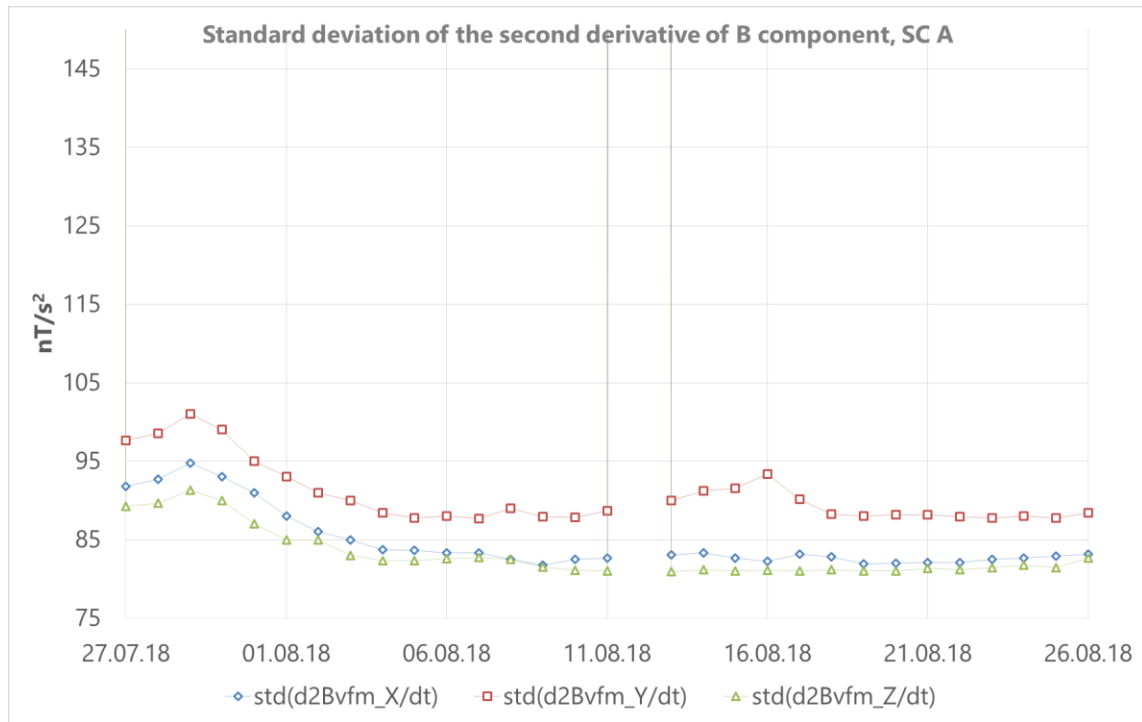
Figure 3-19: Standard deviation of the second derivative of B component
