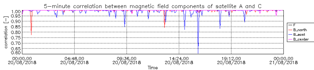
Figure 3-11: Correlation in magnetic data between satellite A and C for B_{north} , B_{east} , and B_{center} components of B_{NEC} are the components of the magnetic field vector in NEC frame
