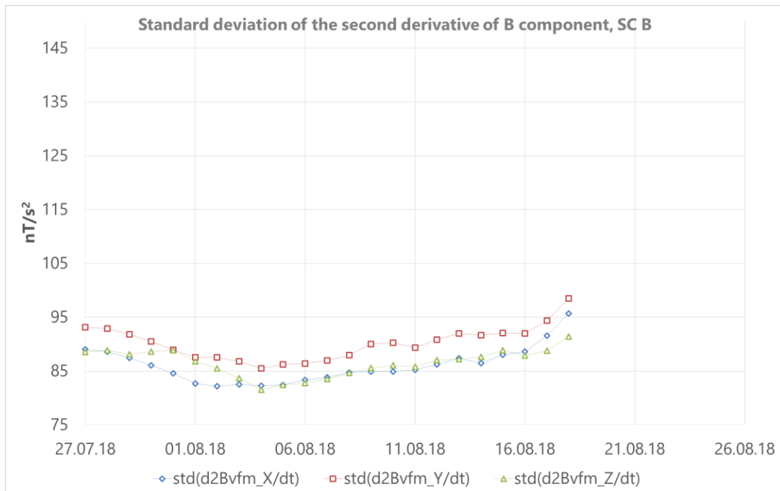
Figure 3-20: Standard deviation of the second derivative of B component
