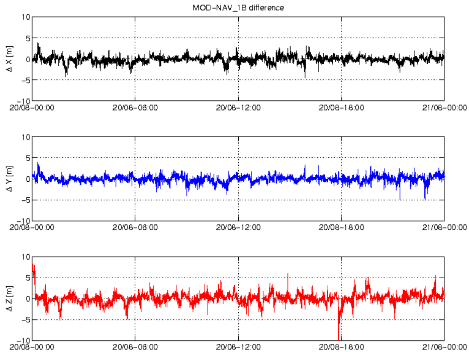
Figure 3-5: Difference MOD-GPSNAV, S/C C, 20.08. From top to bottom: X, Y and Z-axis
