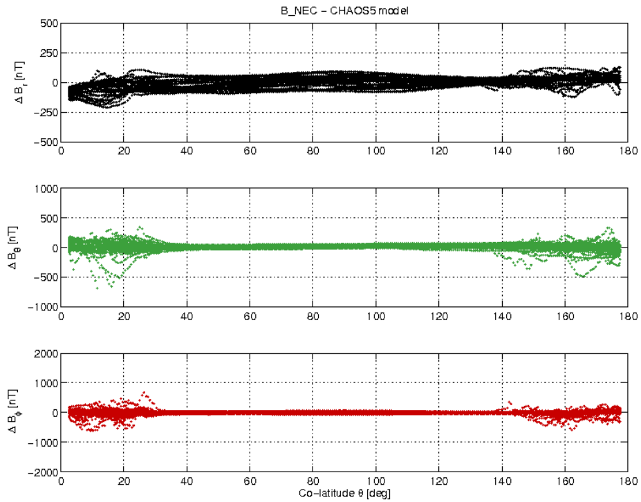
Figure 3-15: S/C A day 20.08 B_{NEC} - B_{Chaos} vs colatitude.
