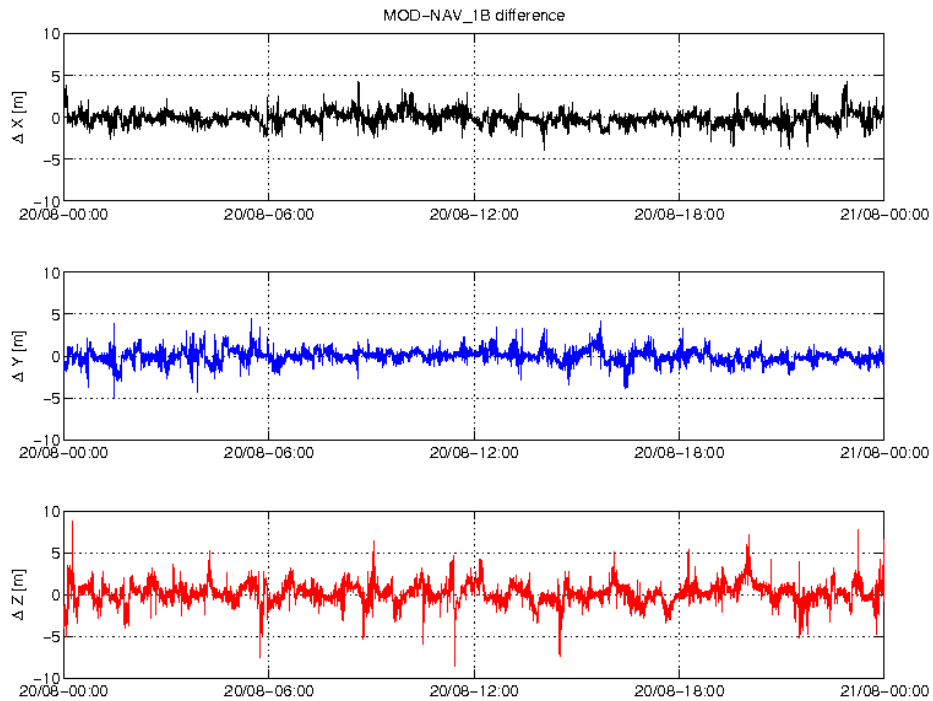
Figure 3-4: Difference MOD-GPSNAV, S/C B, 20.08. From top to bottom: X, Y and Z-axis
