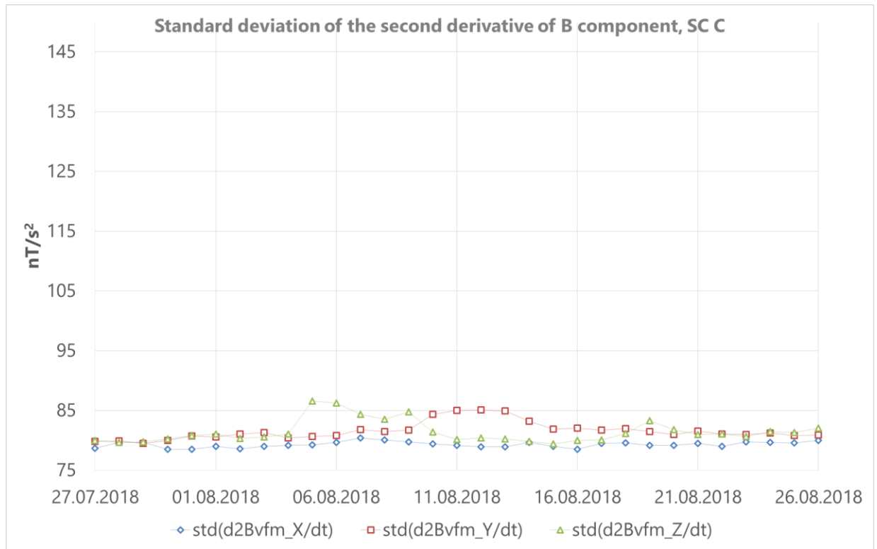
Figure 3-21: Standard deviation of the second derivative of B component
