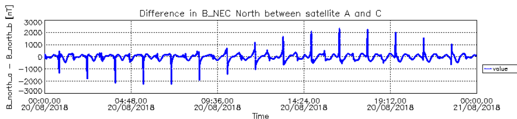
Figure 3-12: Difference in B_{NEC} North component between S/C A and S/C C.
