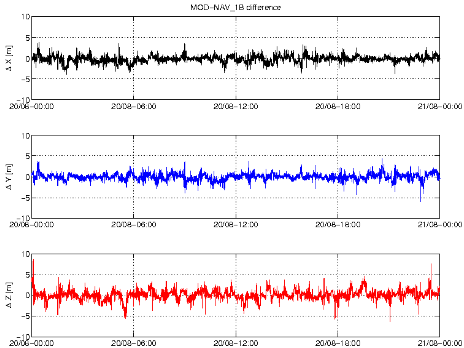
Figure 3-3: Difference MOD-GPSNAV, S/C A, 20.08. From top to bottom: X, Y and Z-axis
