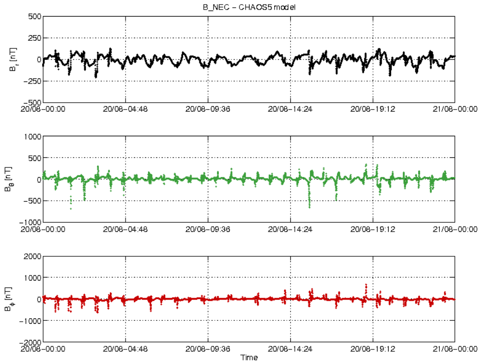
Figure 3-16: S/C A day 20.08: time series of B_{NEC} - B_{Chaos} residuals.
