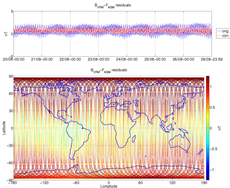
Figure 3-8: ASM-VFM residuals for S/C A, during monitoring period 20/08-26/08. In top figure are plotted: difference between |B_{VFM}| and F_{ASM} (without dB_Sun correction) (blue colour), and the residuals with dB_Sun corrections (red colour). In bottom figure residuals are presented on the world map.
