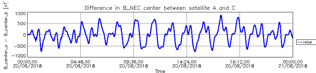
Figure 3-14: Difference in B_{NEC} Center component between S/C A and S/C C.
