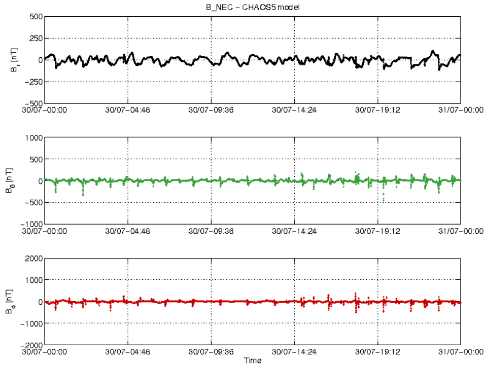
Figure 3-20: S/C B day 30.07 time series of B_{NEC} - B_{Chaos} residuals.
