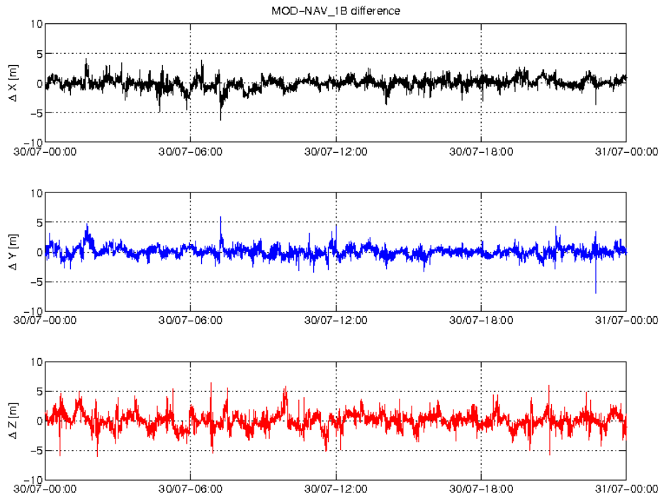
Figure 3-3: Difference MOD-GPSNAV, S/C A, 30.07. From top to bottom: X, Y and Z-axis
