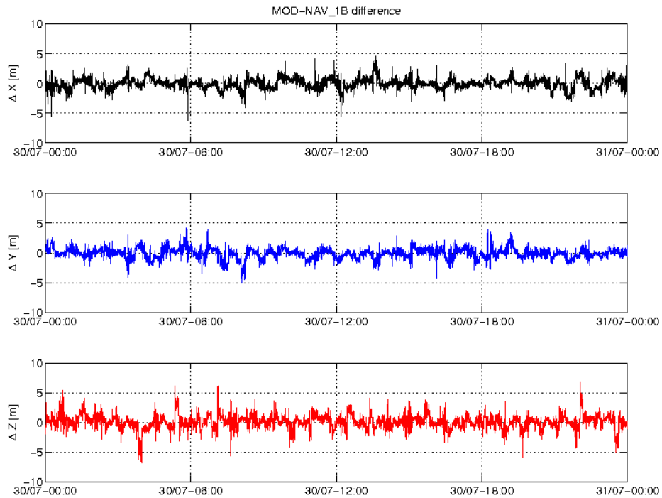
Figure 3-4: Difference MOD-GPSNAV, S/C B, 30.07. From top to bottom: X, Y and Z-axis
