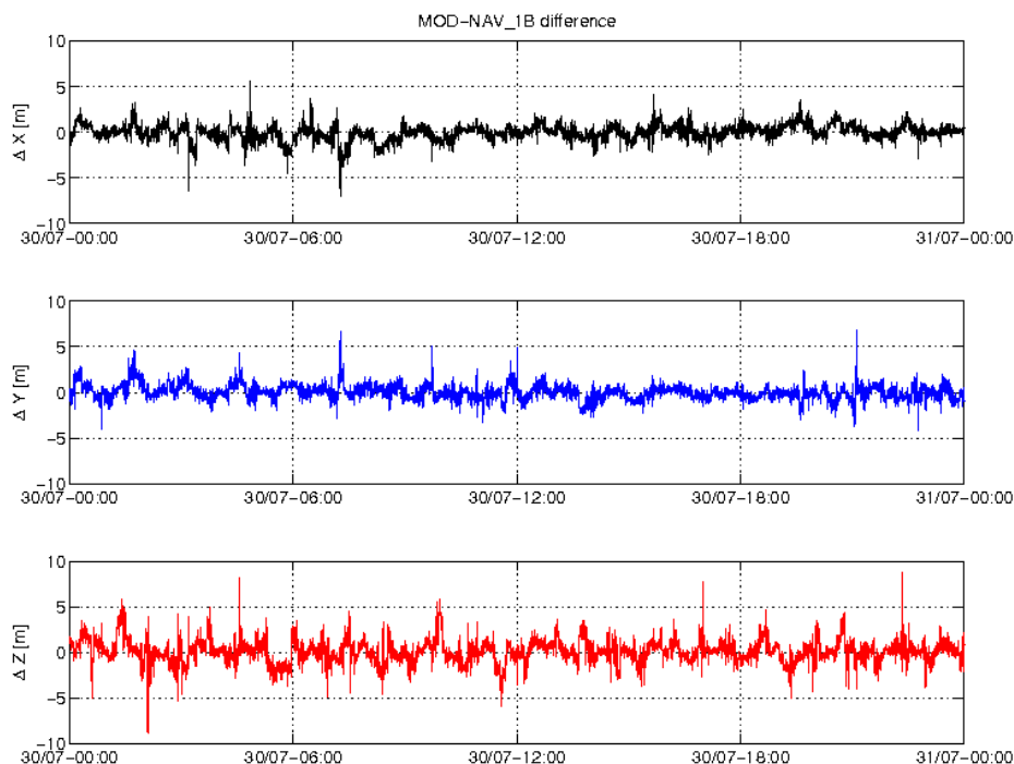
Figure 3-5: Difference MOD-GPSNAV, S/C C, 30.07. From top to bottom: X, Y and Z-axis
