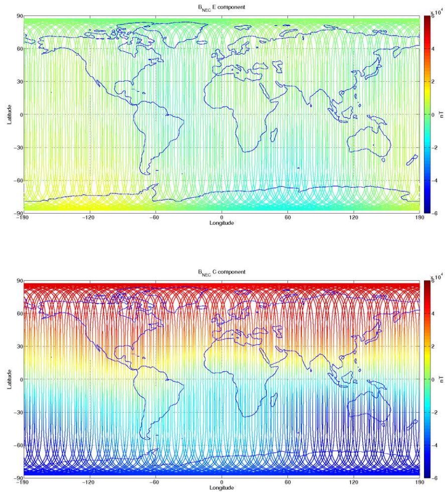
Figure 3-10: S/C A, world map plots of the geomagnetic field and components measured during monitoring period 30/07-05/08. From top to bottom: F-magnetic field from ASM measurement, B_{NEC} components (North, East, and Centre) of magnetic field from VFM measurement.
