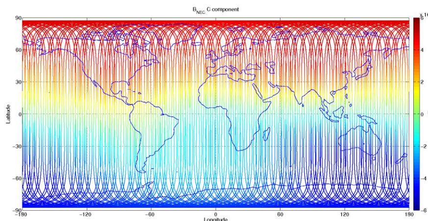
Figure 3-12: S/C C, world map plots of the geomagnetic field and components measured during monitoring period 30/07-05/08. From top to bottom: B_{NEC} components (North, East, and Centre) of magnetic field from VFM measurement.
