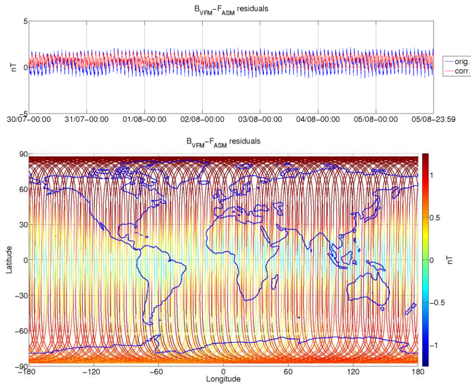
Figure 3-8: ASM-VFM residuals for S/C A, during monitoring period 30/07-05/08. In top figure are plotted: difference between |B VFM | and F ASM (without dB Sun correction) (blue colour), and the residuals with dB Sun corrections (red colour). In bottom figure residuals are presented on the world map.
