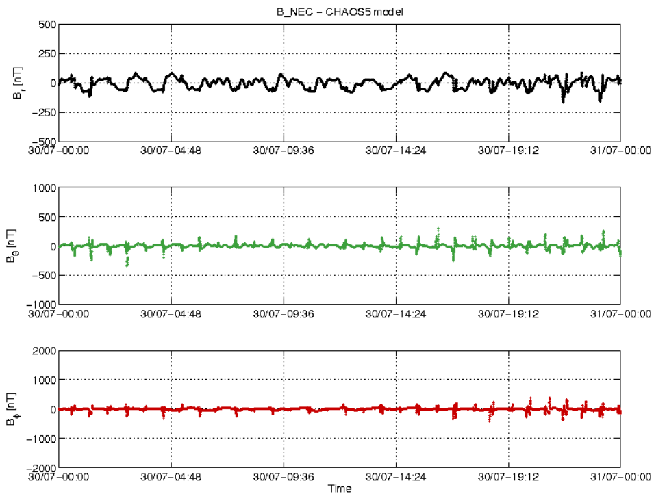
Figure 3-22: S/C C day 30.07 time series of B_{NEC} - B_{Chaos} residuals.
