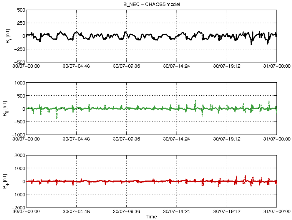
Figure 3-18: S/C A day 30.07: time series of B_{NEC} - B_{Chaos} residuals.
