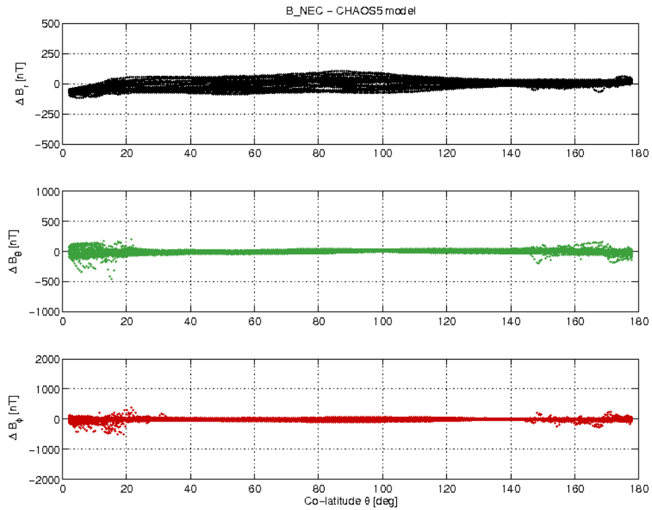
Figure 3-19: S/C B day 30.07 B_{NEC} - B_{Chaos} difference vs colatitude.
