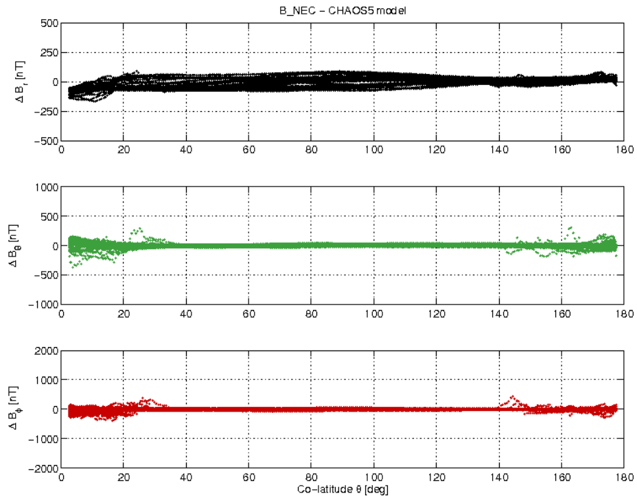
Figure 3-17: S/C A day 30.07 B_{NEC} - B_{Chaos} vs colatitude.
