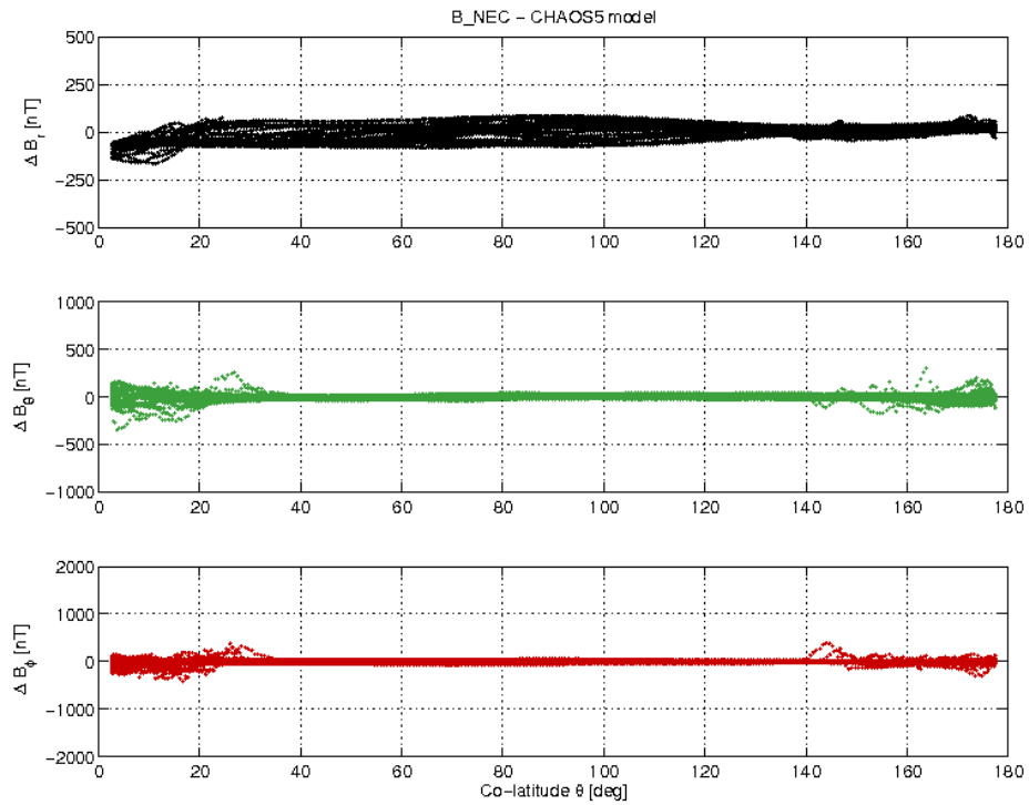
Figure 3-21: S/C C day 30.07 B_{NEC} - B_{Chaos} difference vs colatitude.
