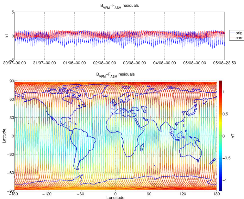
Figure 3-9: ASM-VFM residuals for S/C B, during monitoring period 30/07-05/08. In top figure are plotted: difference between |B_{VFM}| and F_{ASM} (without dB_{Sun} correction) (blue colour), and the residuals with dB_{Sun} corrections (red colour). In bottom figure residuals are presented on the world map.
