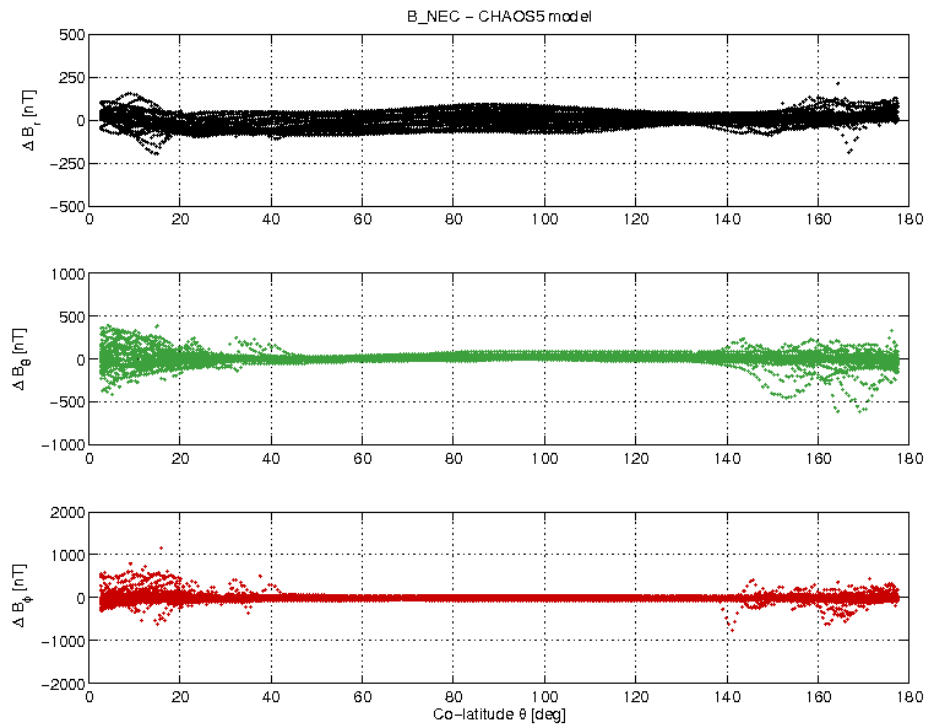
Figure 3-17: S/C A day 18.06 B_{NEC} - B_{Chaos} vs colatitude.
