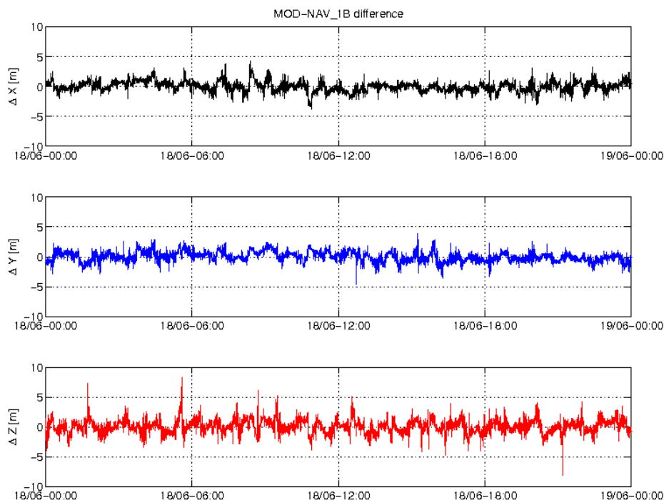
Figure 3-5: Difference MOD-GPSNAV, S/C C, 18.06. From top to bottom: X, Y and Z-axis
