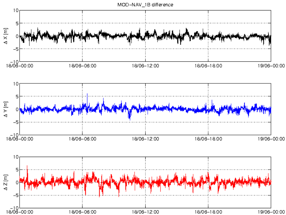
Figure 3-4: Difference MOD-GPSNAV, S/C B, 18.06. From top to bottom: X, Y and Z-axis
