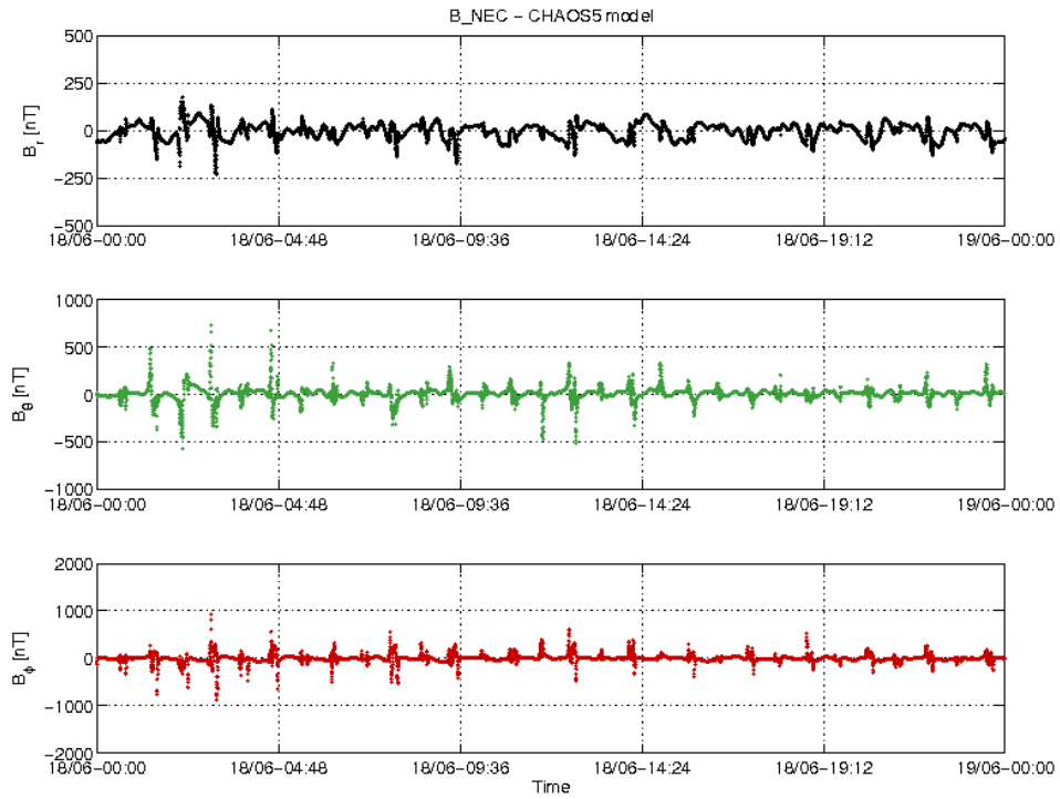
Figure 3-20: S/C B day 18.06 time series of B_{NEC} - B_{Chaos} residuals.
