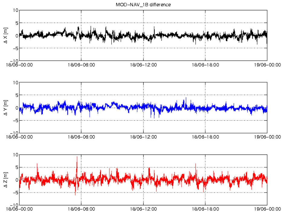
Figure 3-3: Difference MOD-GPSNAV, S/C A, 18.06. From top to bottom: X, Y and Z-axis
