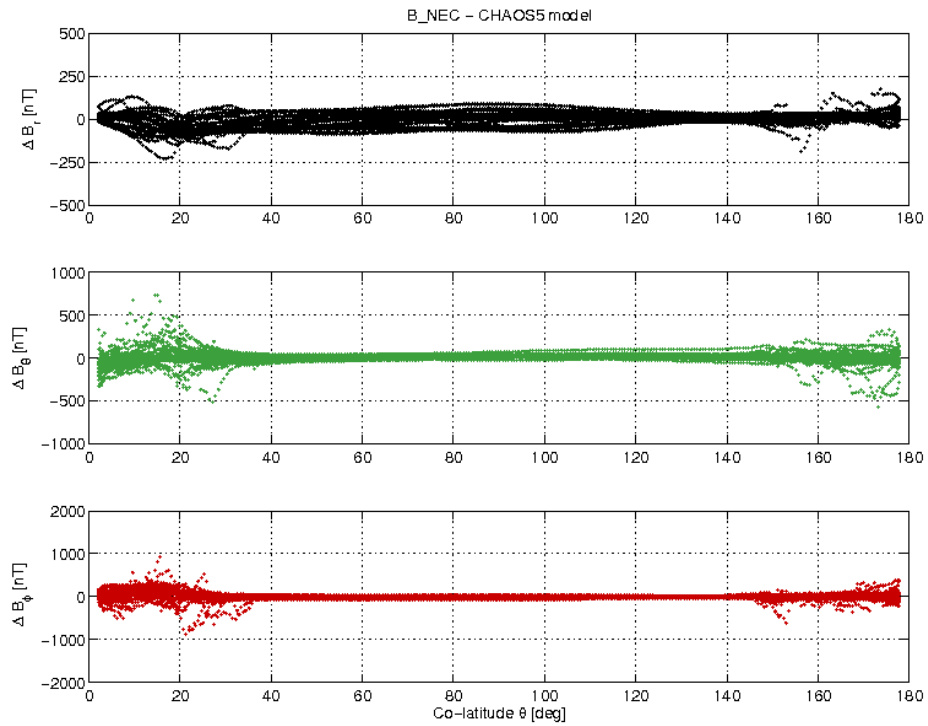
Figure 3-19: S/C B day 18.06 B_{NEC} - B_{Chaos} difference vs colatitude.
