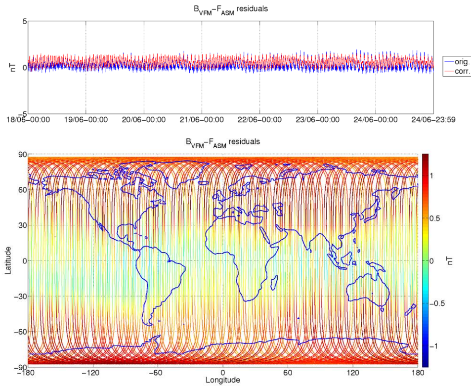
Figure 3-8: ASM-VFM residuals for S/C A, during monitoring period 18/06-24/06. In top figure are plotted: difference between |B VFM | and F ASM (without dB Sun correction) (blue colour), and the residuals with dB Sun corrections (red colour). In bottom figure residuals are presented on the world map.
