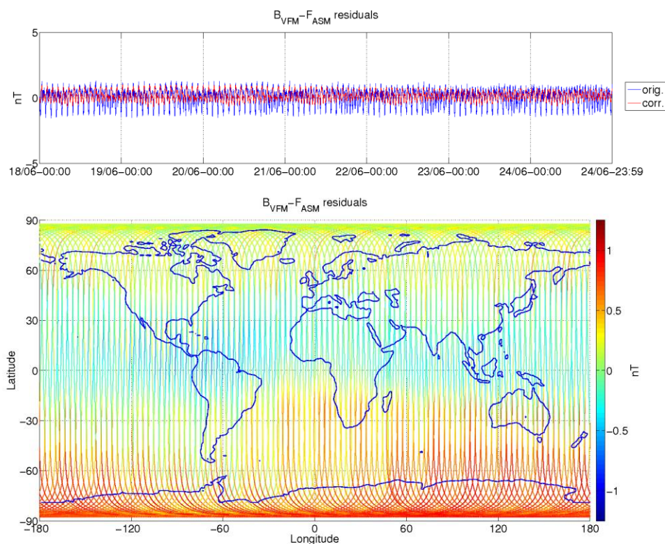
Figure 3-9: ASM-VFM residuals for S/C B, during monitoring period 18/06-24/06. In top figure are plotted: difference between |B_{VFM}| and F_{ASM} (without dB_{Sun} correction) (blue colour), and the residuals with dB_{Sun} corrections (red colour). In bottom figure residuals are presented on the world map.
