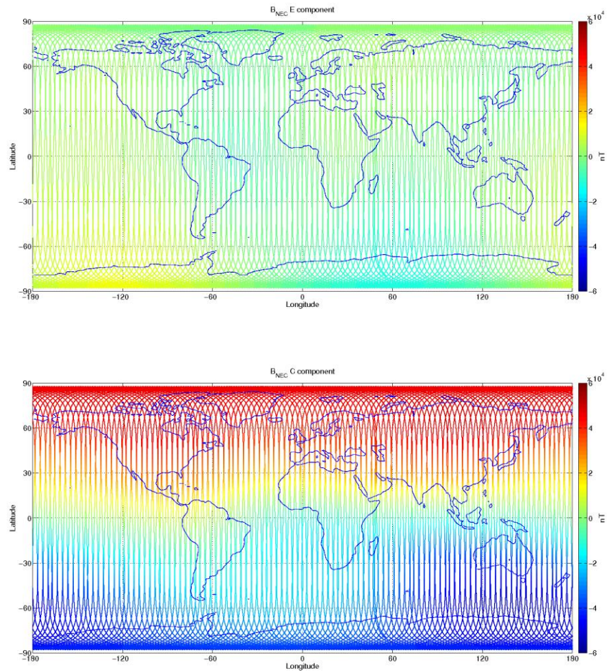
Figure 3-11: S/C B, world map plots of the geomagnetic field and components measured during monitoring period 18/06-24/06. From top to bottom: F-magnetic field from ASM measurement, B_{NEC} components (North, East, and Centre) of magnetic field from VFM measurement.
