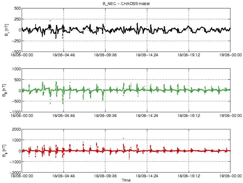
Figure 3-18: S/C A day 18.06: time series of B_{NEC} - B_{Chaos} residuals.
