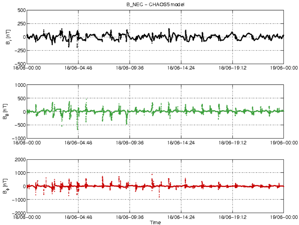
Figure 3-22: S/C C day 18.06 time series of B_{NEC} - B_{Chaos} residuals.
