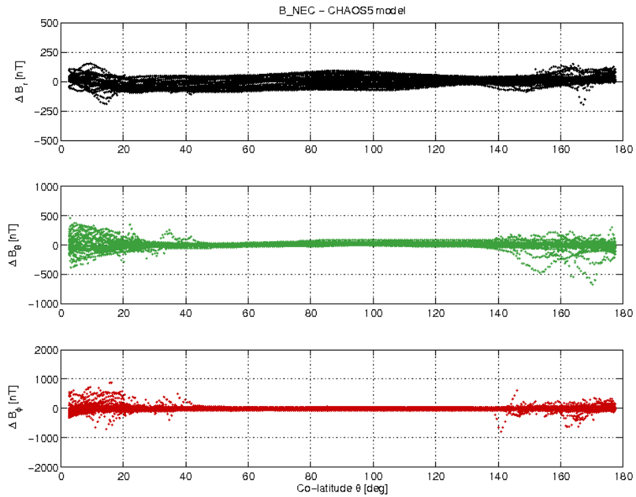
Figure 3-21: S/C C day 18.06 B_{NEC} - B_{Chaos} difference vs colatitude.
