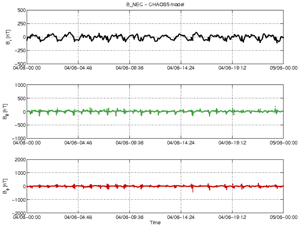
Figure 3-20: S/C B day 04.06 time series of B_{NEC} - B_{Chaos} residuals.
