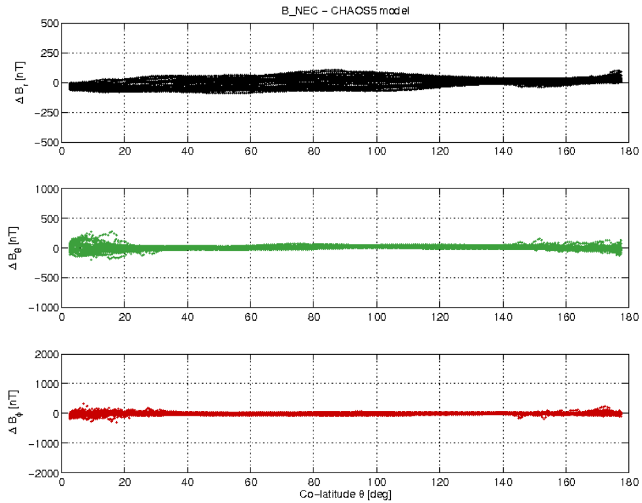
Figure 3-21: S/C C day 04.06 B_{NEC} - B_{Chaos} difference vs colatitude.
