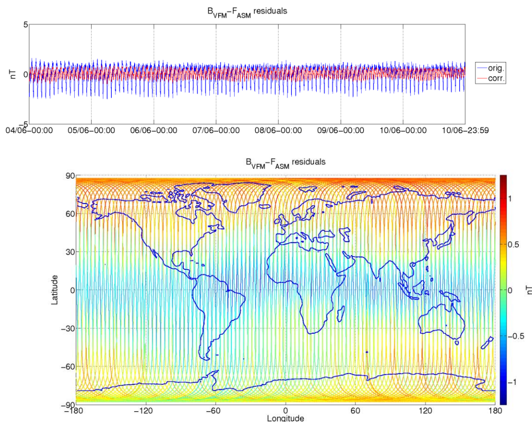
Figure 3-9: ASM-VFM residuals for S/C B, during monitoring period 04/06-10/06. In top figure are plotted: difference between |B VFM | and F ASM (without dB Sun correction) (blue colour), and the residuals with dB Sun corrections (red colour). In bottom figure residuals are presented on the world map.
