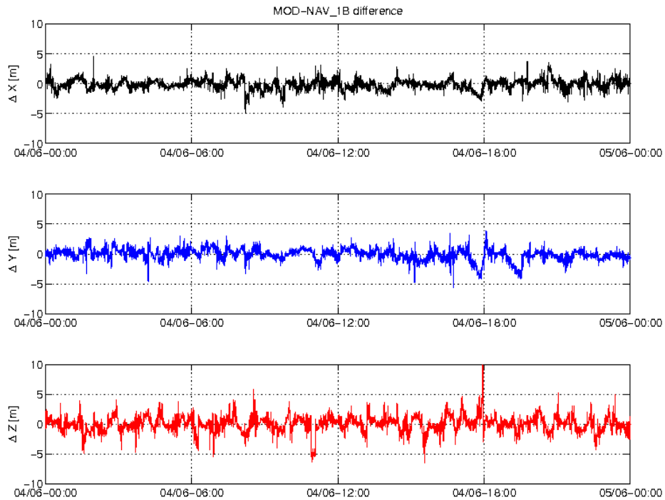
Figure 3-5: Difference MOD-GPSNAV, S/C C, 04.06. From top to bottom: X, Y and Z-axis
