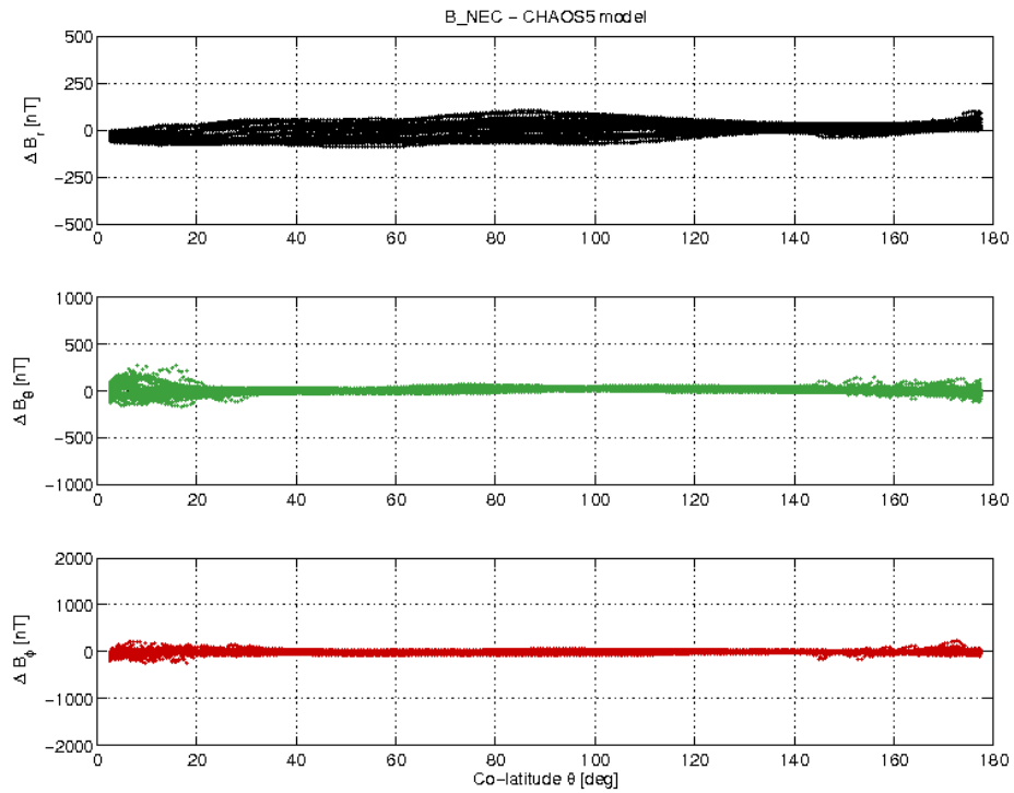
Figure 3-17: S/C A day 04.06 B_{NEC} - B_{Chaos} vs colatitude.
