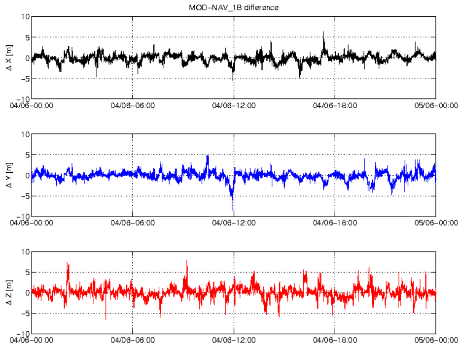
Figure 3-4: Difference MOD-GPSNAV, S/C B, 04.06. From top to bottom: X, Y and Z-axis
