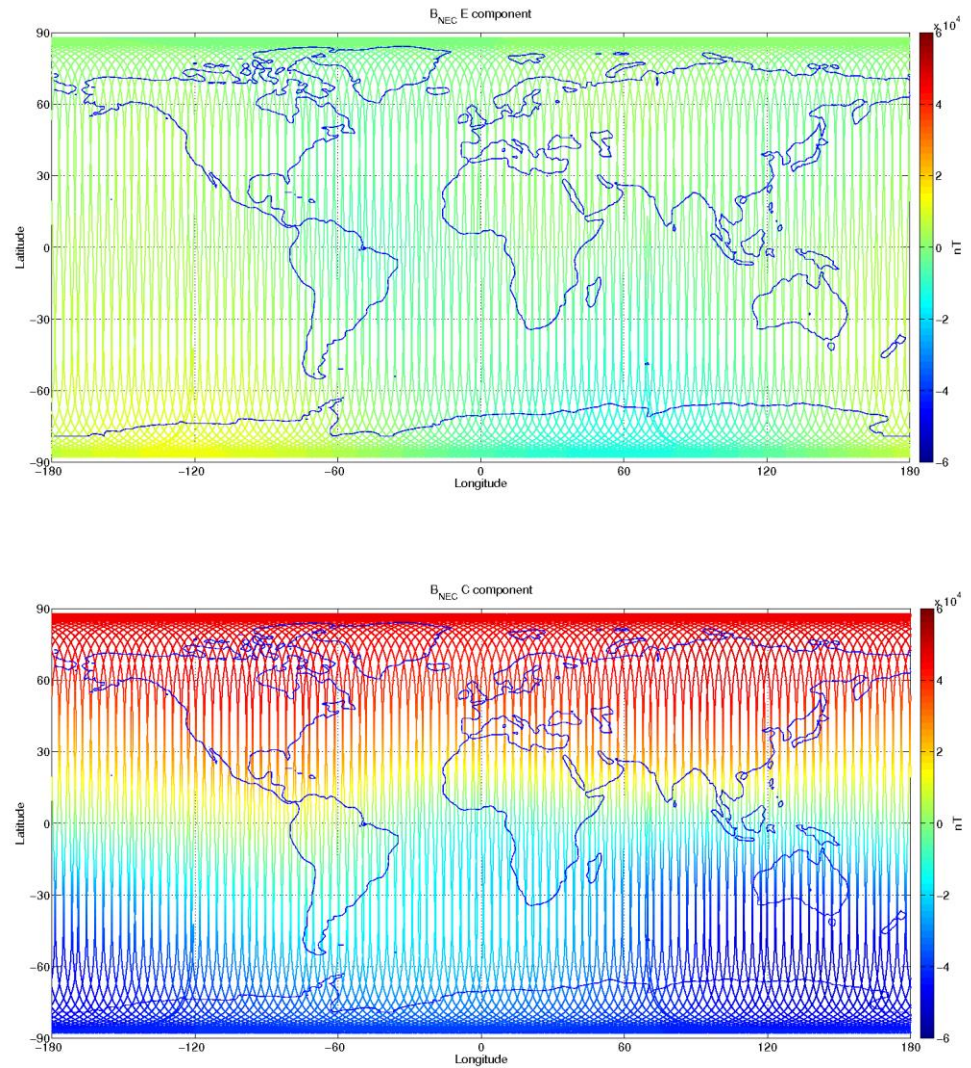
Figure 3-11: S/C B, world map plots of the geomagnetic field and components measured during monitoring period 04/06-10/06. From top to bottom: F-magnetic field from ASM measurement, B_{NEC} components (North, East, and Centre) of magnetic field from VFM measurement.
