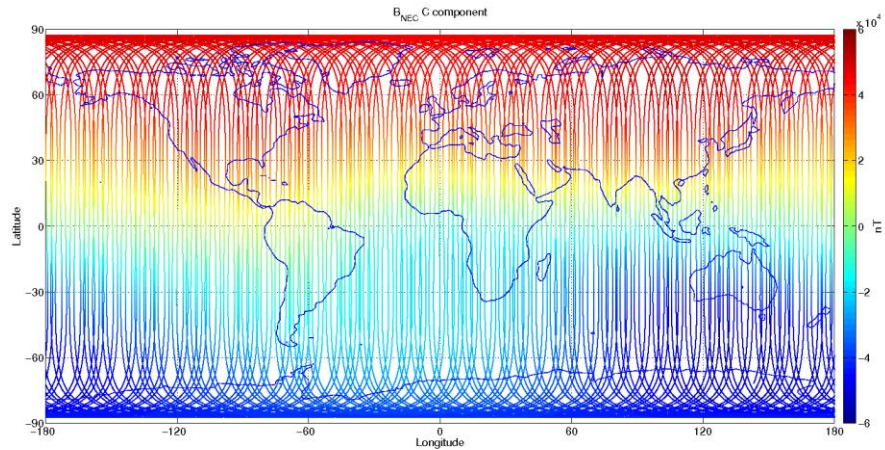
Figure 3-12: S/C C, world map plots of the geomagnetic field and components measured during monitoring period 04/06-10/06. From top to bottom: B_{NEC} components (North, East, and Centre) of magnetic field from VFM measurement.
