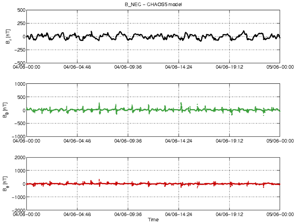
Figure 3-22: S/C C day 04.06 time series of B_{NEC} - B_{Chaos} residuals.
