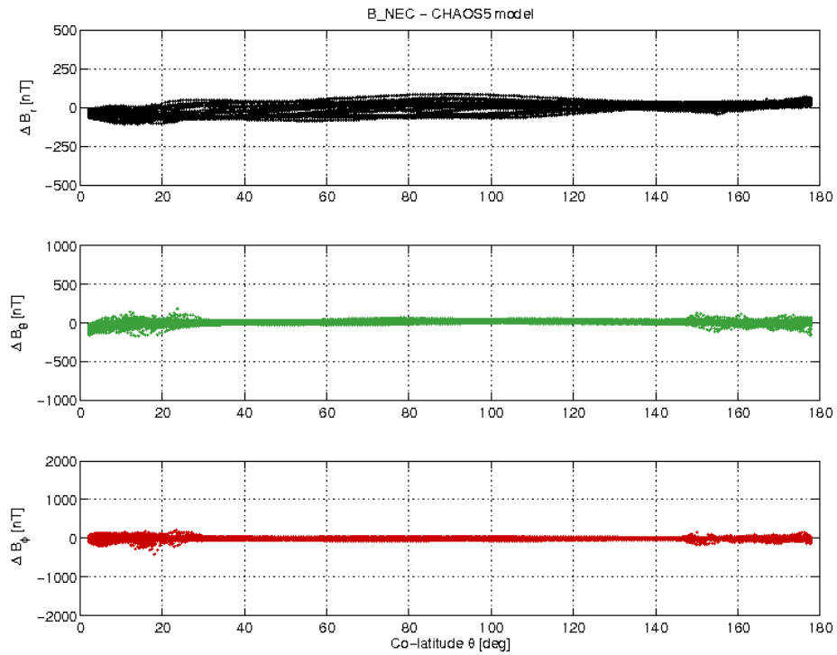
Figure 3-19: S/C B day 04.06 B_{NEC} - B_{Chaos} difference vs colatitude.
