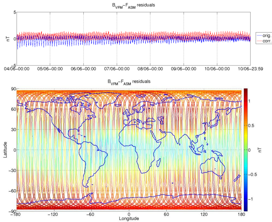
Figure 3-8: ASM-VFM residuals for S/C A, during monitoring period 04/06-10/06. In top figure are plotted: difference between |B VFM | and F ASM (without dB Sun correction) (blue colour), and the residuals with dB Sun corrections (red colour). In bottom figure residuals are presented on the world map.
