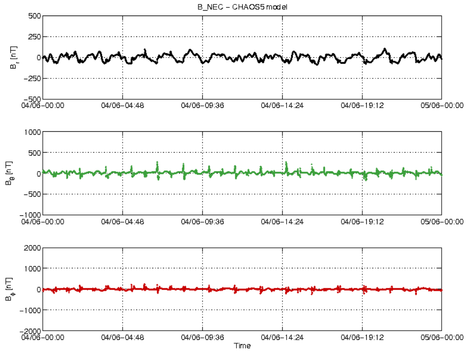
Figure 3-18: S/C A day 04.06: time series of B_{NEC} - B_{Chaos} residuals.
