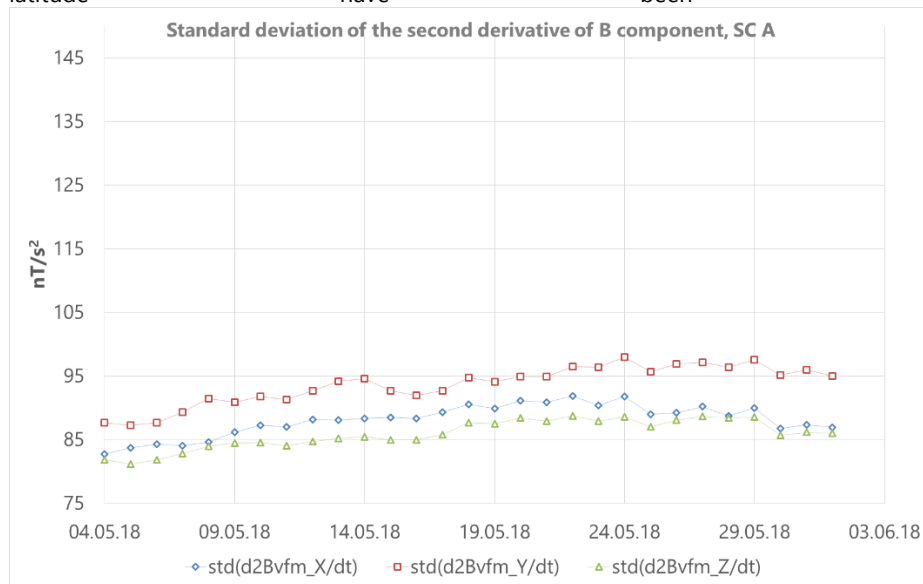
Figure 3-23, Figure 3-24 and Figure 3-25 show the daily standard deviation of the second derivative of BVFM of the last month for S/C A, B, and C respectively. Second derivative of B_{NEC} is not shown due to artificial spikes introduced during quaternions interpolation from 1Hz to 50Hz.
