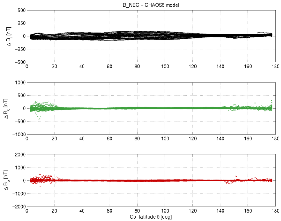
Figure 3-21: S/C C day 28.05 B_{NEC} - B_{Chaos} difference vs colatitude.
