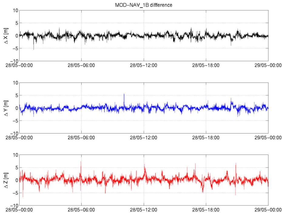
Figure 3-4: Difference MOD-GPSNAV, S/C B, 28.05. From top to bottom: X, Y and Z-axis
