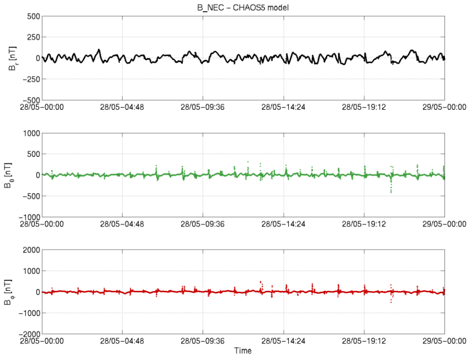
Figure 3-18: S/C A day 28.05: time series of B_{NEC} - B_{Chaos} residuals.
