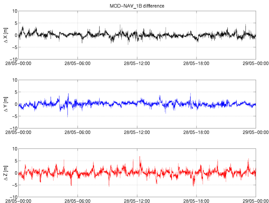
Figure 3-5: Difference MOD-GPSNAV, S/C C, 28.05. From top to bottom: X, Y and Z-axis
