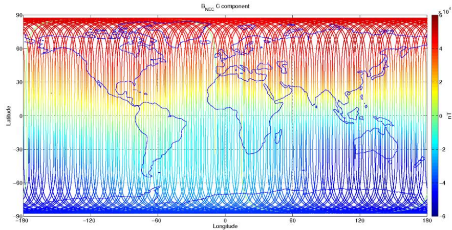
Figure 3-12: S/C C, world map plots of the geomagnetic field and components measured during monitoring period 28/05-03/06. From top to bottom: B_{NEC} components (North, East, and Centre) of magnetic field from VFM measurement.
