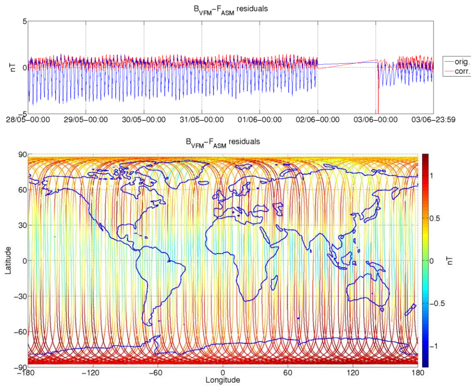
Figure 3-8: ASM-VFM residuals for S/C A, during monitoring period 28/05-03/06. In top figure are plotted: difference between |B VFM | and F ASM (without dB Sun correction) (blue colour), and the residuals with dB Sun corrections (red colour). In bottom figure residuals are presented on the world map.
