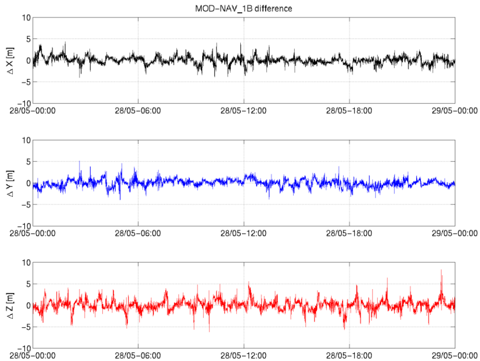
Figure 3-3: Difference MOD-GPSNAV, S/C A, 28.05. From top to bottom: X, Y and Z-axis
