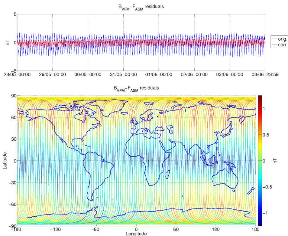
Figure 3-9: ASM-VFM residuals for S/C B, during monitoring period 28/05-03/06. In top figure are plotted: difference between |B_{VFM}| and F_{ASM} (without dB_Sun correction) (blue colour), and the residuals with dB_Sun corrections (red colour). In bottom figure residuals are presented on the world map.
