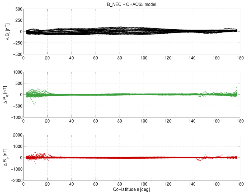
Figure 3-17: S/C A day 28.05 B_{NEC} - B_{Chaos} vs colatitude.
