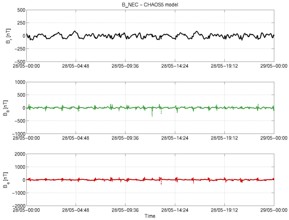
Figure 3-20: S/C B day 28.05 time series of B_{NEC} - B_{Chaos} residuals.
