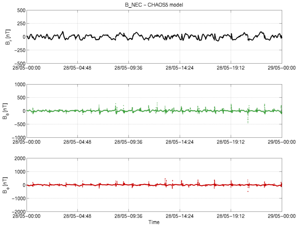
Figure 3-22: S/C C day 28.05 time series of B_{NEC} - B_{Chaos} residuals.
