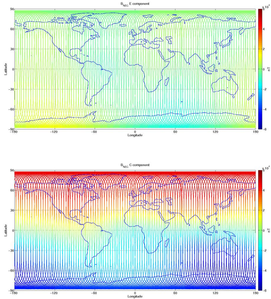
Figure 3-11: S/C B, world map plots of the geomagnetic field and components measured during monitoring period 28/05-03/06. From top to bottom: F-magnetic field from ASM measurement, B_{NEC} components (North, East, and Centre) of magnetic field from VFM measurement.
