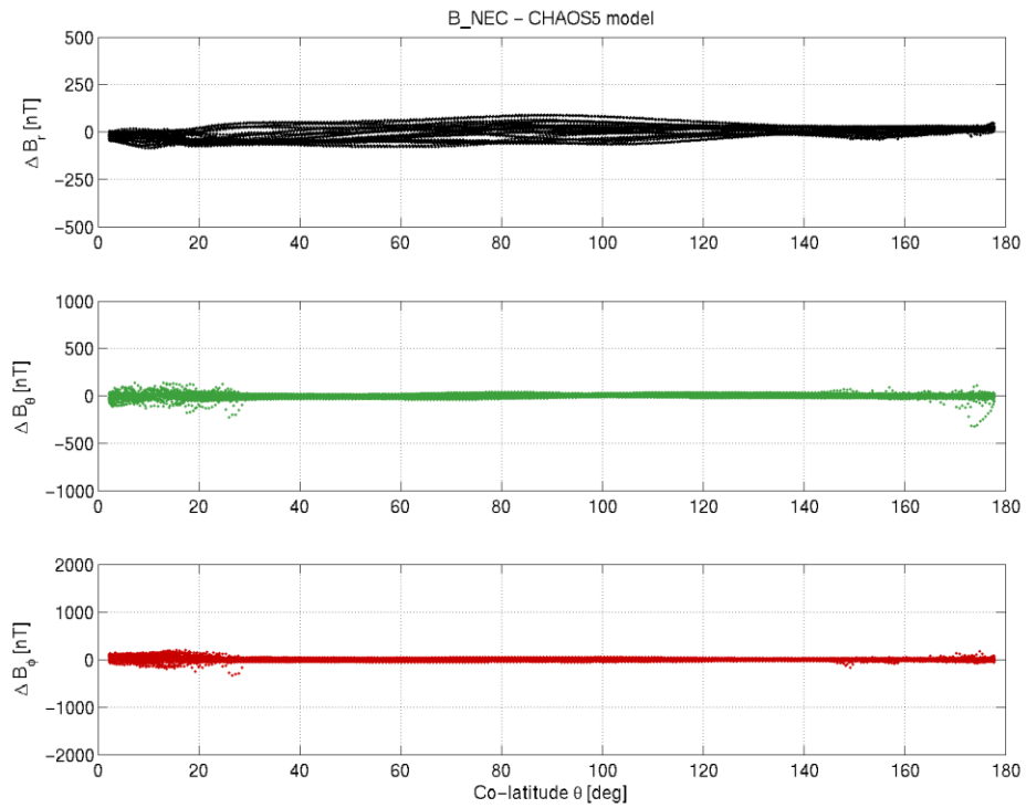
Figure 3-19: S/C B day 28.05 B_{NEC} - B_{Chaos} difference vs colatitude.
