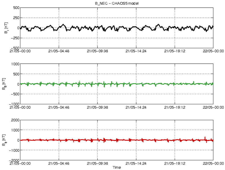
Figure 3-20: S/C B day 21.05 time series of B_{NEC} - B_{Chaos} residuals.
