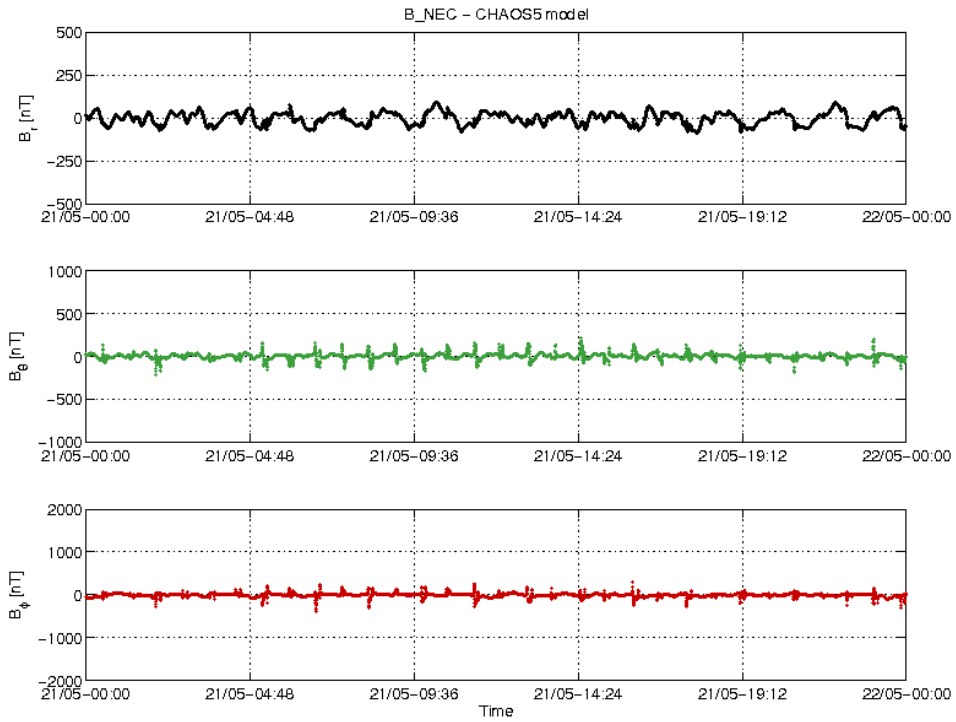
Figure 3-18: S/C A day 21.05: time series of B_{NEC} - B_{Chaos} residuals.
