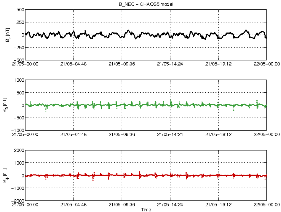
Figure 3-22: S/C C day 21.05 time series of B_{NEC} - B_{Chaos} residuals.
