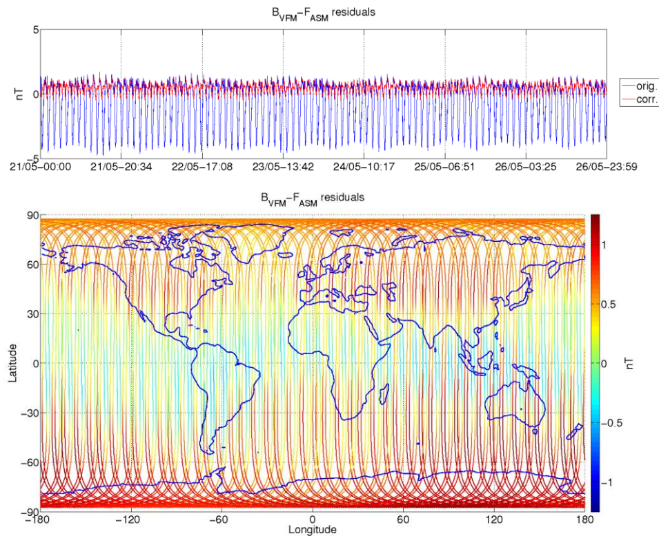
Figure 3-8: ASM-VFM residuals for S/C A, during monitoring period 21/05-27/05. In top figure are plotted: difference between |B VFM | and F ASM (without dB Sun correction) (blue colour), and the residuals with dB Sun corrections (red colour). In bottom figure residuals are presented on the world map.
