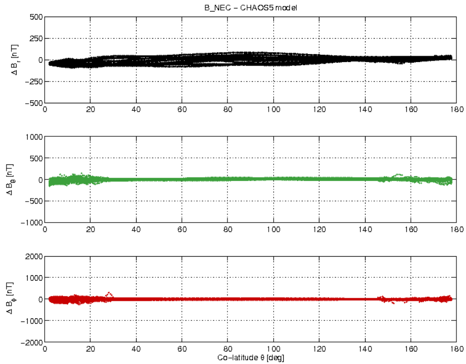
Figure 3-19: S/C B day 21.05 B_{NEC} - B_{Chaos} difference vs colatitude.
