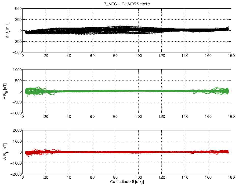
Figure 3-21: S/C C day 21.05 B_{NEC} - B_{Chaos} difference vs colatitude.
