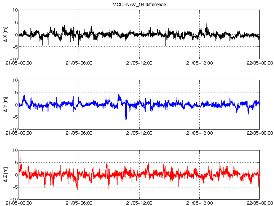
Figure 3-4: Difference MOD-GPSNAV, S/C B, 21.05. From top to bottom: X, Y and Z-axis
