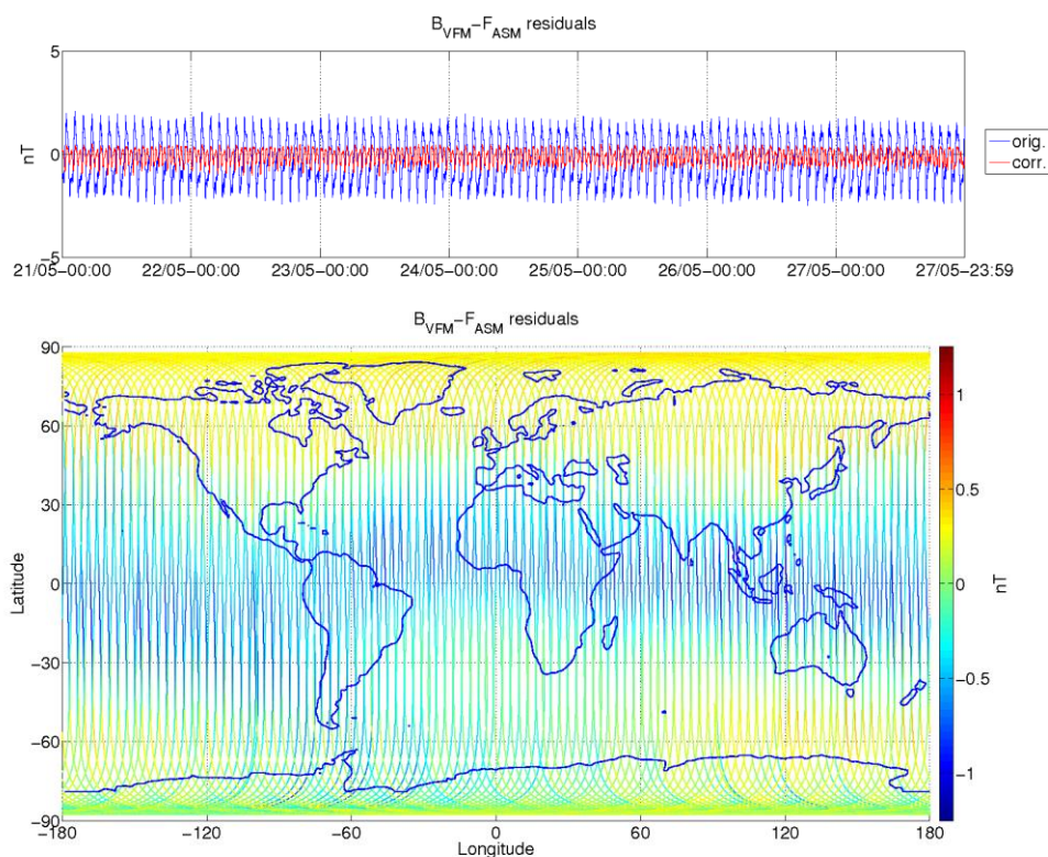
Figure 3-9: ASM-VFM residuals for S/C B, during monitoring period 21/05-27/05. In top figure are plotted: difference between |B_{VFM}| and F_{ASM} (without dB_{Sun} correction) (blue colour), and the residuals with dB_{Sun} corrections (red colour). In bottom figure residuals are presented on the world map.
