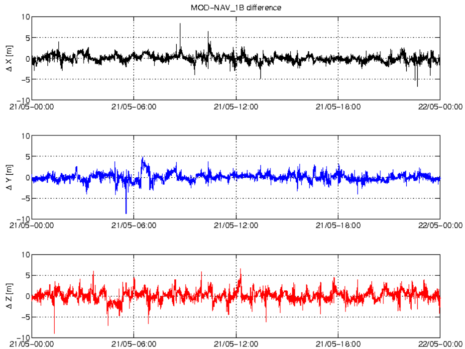
Figure 3-3: Difference MOD-GPSNAV, S/C A, 21.05. From top to bottom: X, Y and Z-axis
