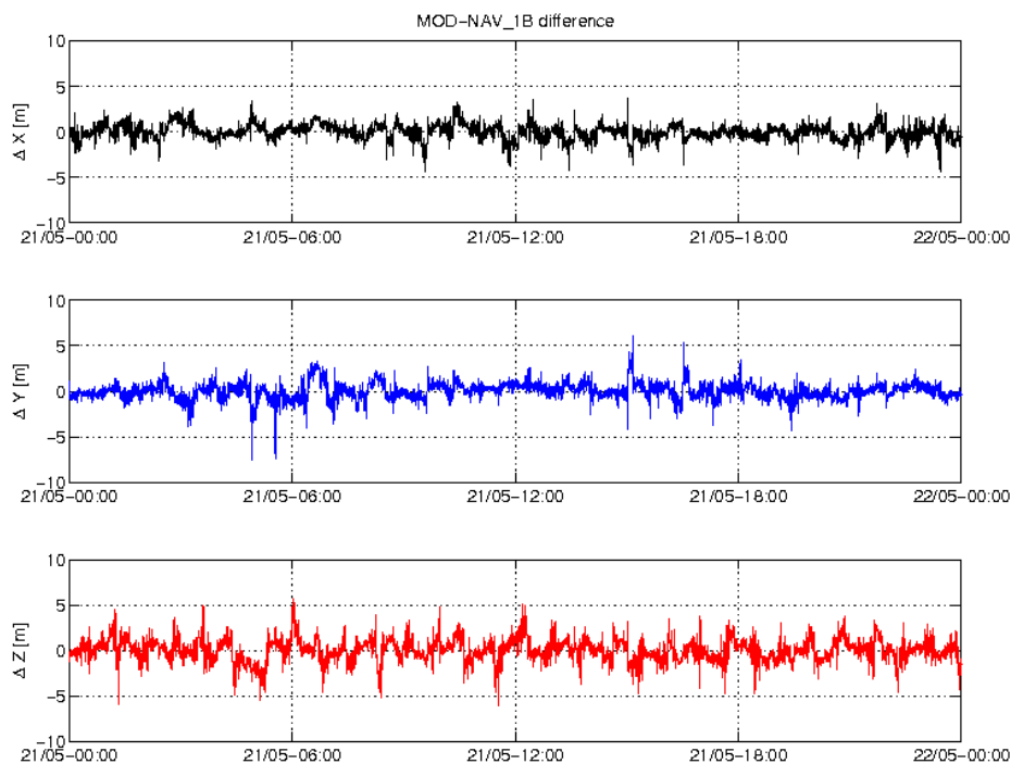
Figure 3-5: Difference MOD-GPSNAV, S/C C, 21.05. From top to bottom: X, Y and Z-axis
