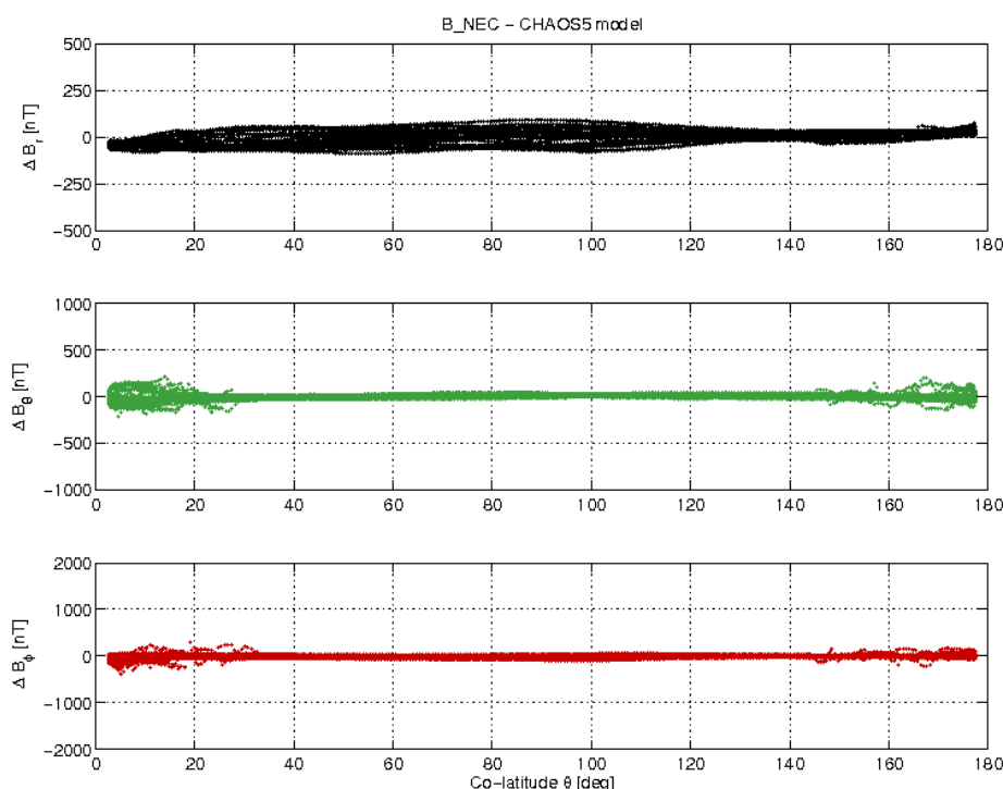
Figure 3-17: S/C A day 21.05 B_{NEC} - B_{Chaos} vs colatitude.
