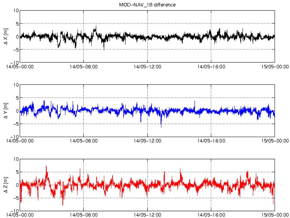
Figure 3-4: Difference MOD-GPSNAV, S/C B, 14.05. From top to bottom: X, Y and Z-axis
