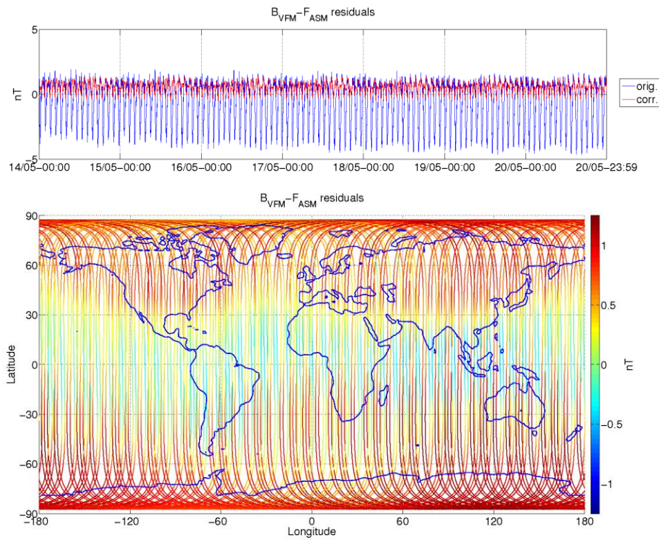
Figure 3-8: ASM-VFM residuals for S/C A, during monitoring period 14/05-20/05. In top figure are plotted: difference between |B VFM | and F ASM (without dB Sun correction) (blue colour), and the residuals with dB Sun corrections (red colour). In bottom figure residuals are presented on the world map.
