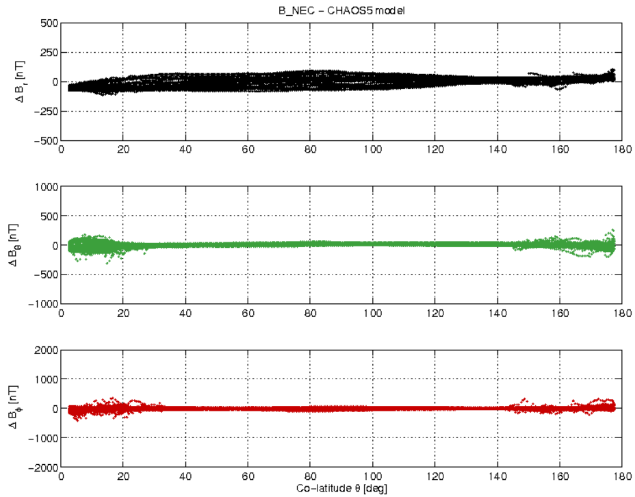
Figure 3-21: S/C C day 14.05 B_{NEC} - B_{Chaos} difference vs colatitude.
