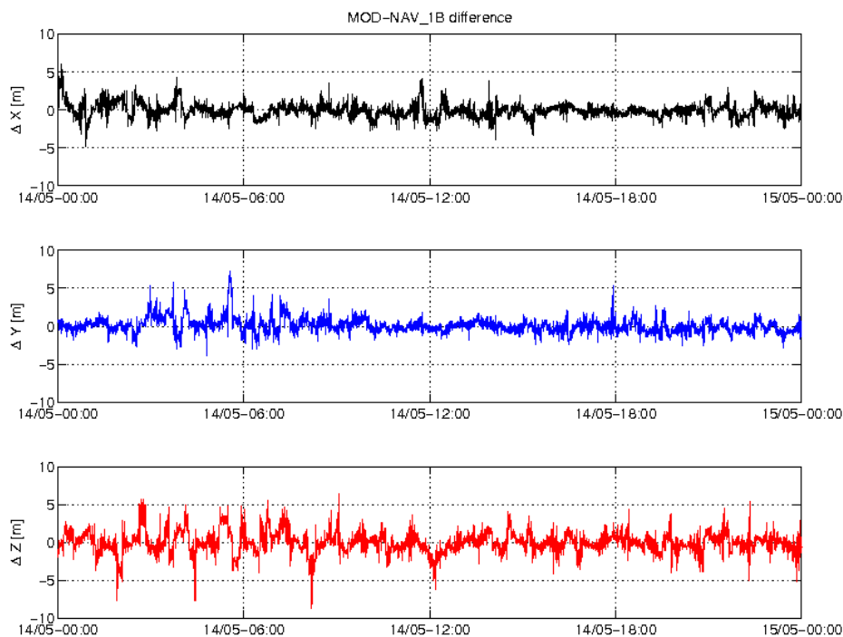
Figure 3-5: Difference MOD-GPSNAV, S/C C, 14.05. From top to bottom: X, Y and Z-axis
