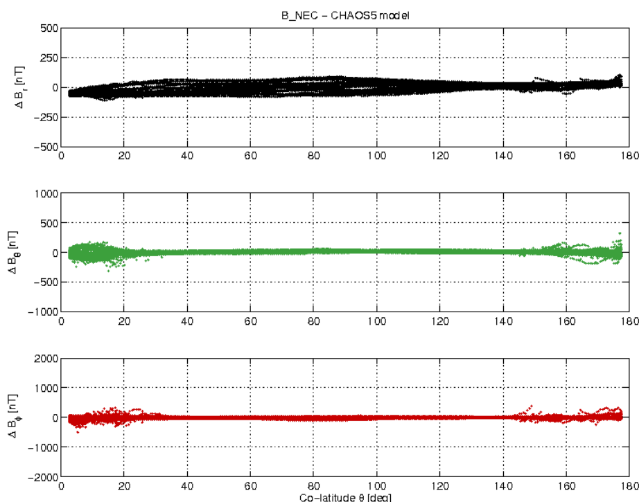
Figure 3-17: S/C A day 14.05 B_{NEC} - B_{Chaos} vs colatitude.
