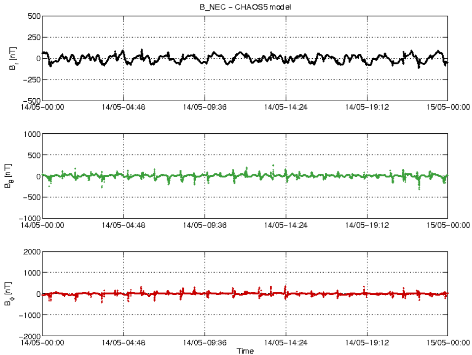
Figure 3-22: S/C C day 14.05 time series of B_{NEC} - B_{Chaos} residuals.
