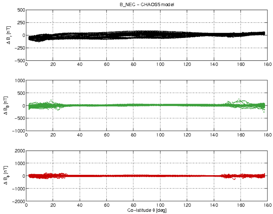
Figure 3-19: S/C B day 14.05 B_{NEC} - B_{Chaos} difference vs colatitude.
