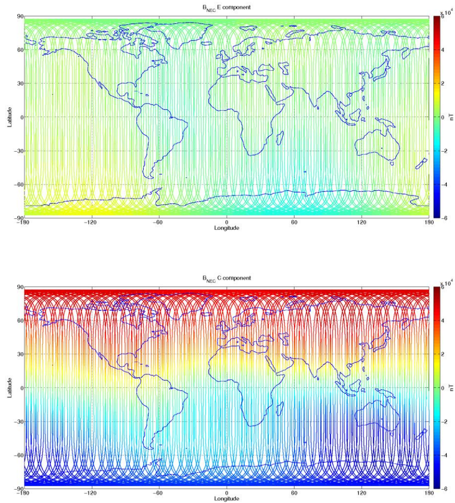
Figure 3-10: S/C A, world map plots of the geomagnetic field and components measured during monitoring period 14/05-20/05. From top to bottom: F-magnetic field from ASM measurement, B_{NEC} components (North, East, and Centre) of magnetic field from VFM measurement.
