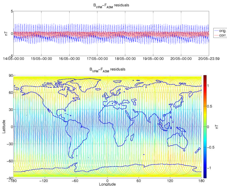
Figure 3-9: ASM-VFM residuals for S/C B, during monitoring period 14/05-20/05. In top figure are plotted: difference between |B_{VFM}| and F_{ASM} (without dB_{Sun} correction) (blue colour), and the residuals with dB_{Sun} corrections (red colour). In bottom figure residuals are presented on the world map.
