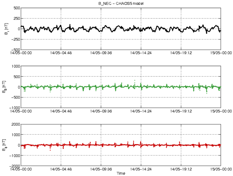
Figure 3-18: S/C A day 14.05: time series of B_{NEC} - B_{Chaos} residuals.
