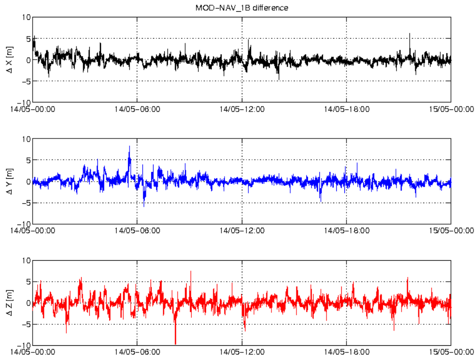
Figure 3-3: Difference MOD-GPSNAV, S/C A, 14.05. From top to bottom: X, Y and Z-axis
