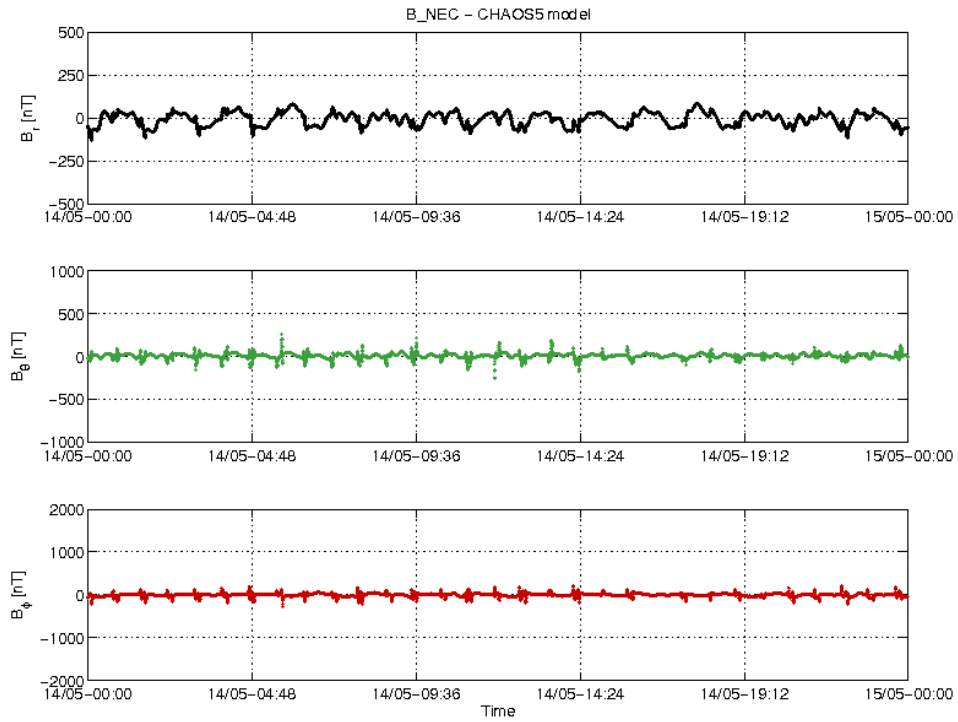
Figure 3-20: S/C B day 14.05 time series of B_{NEC} - B_{Chaos} residuals.
