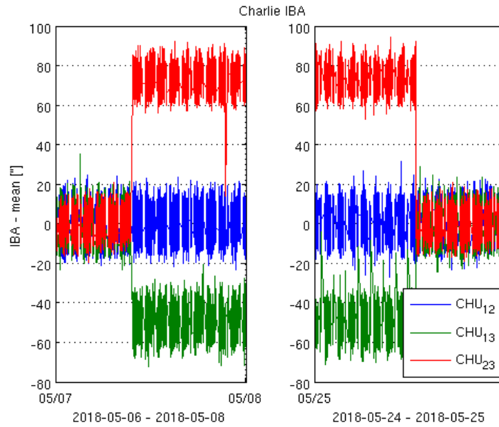
Figure 27 : Trend of the IBA's on the days 07/05 (when the anomaly was registered) and on 25/05 (when the anomaly was fixed).
