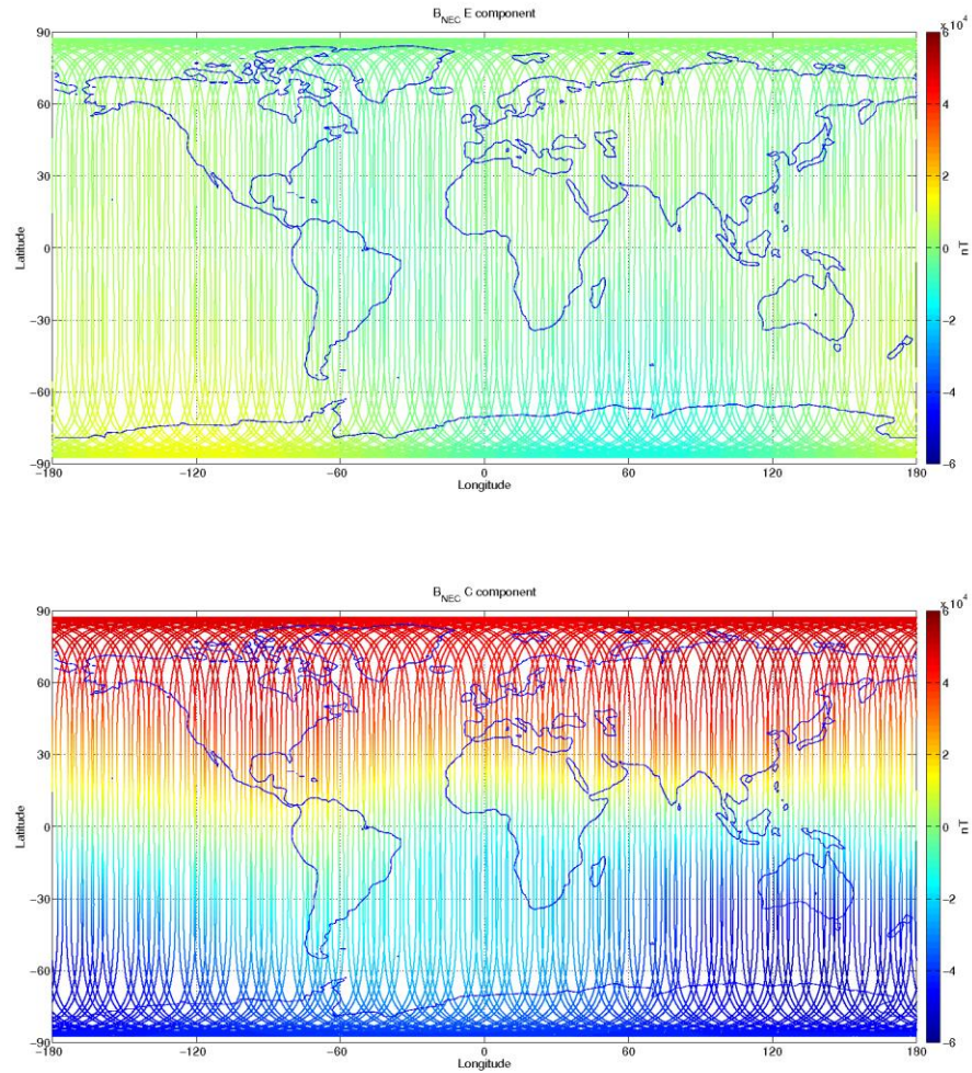
Figure 3-10: S/C A, world map plots of the geomagnetic field and components measured during monitoring period 07/05-13/05. From top to bottom: F-magnetic field from ASM measurement, B_{NEC} components (North, East, and Centre) of magnetic field from VFM measurement.
