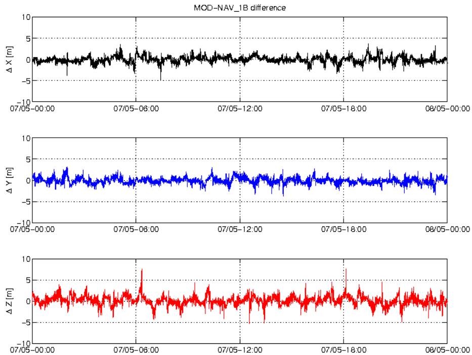
Figure 3-4: Difference MOD-GPSNAV, S/C B, 07.05. From top to bottom: X, Y and Z-axis
