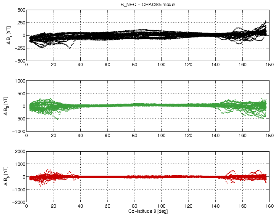
Figure 3-21: S/C C day 07.05 B_{NEC} - B_{Chaos} difference vs colatitude.
