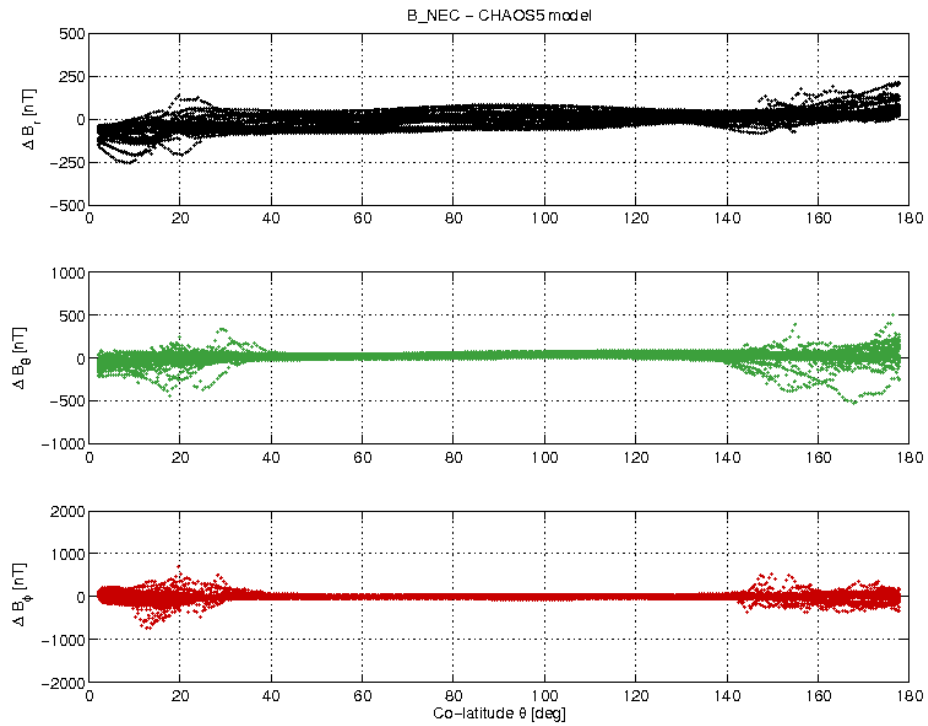
Figure 3-19: S/C B day 07.05 B_{NEC} - B_{Chaos} difference vs colatitude.
