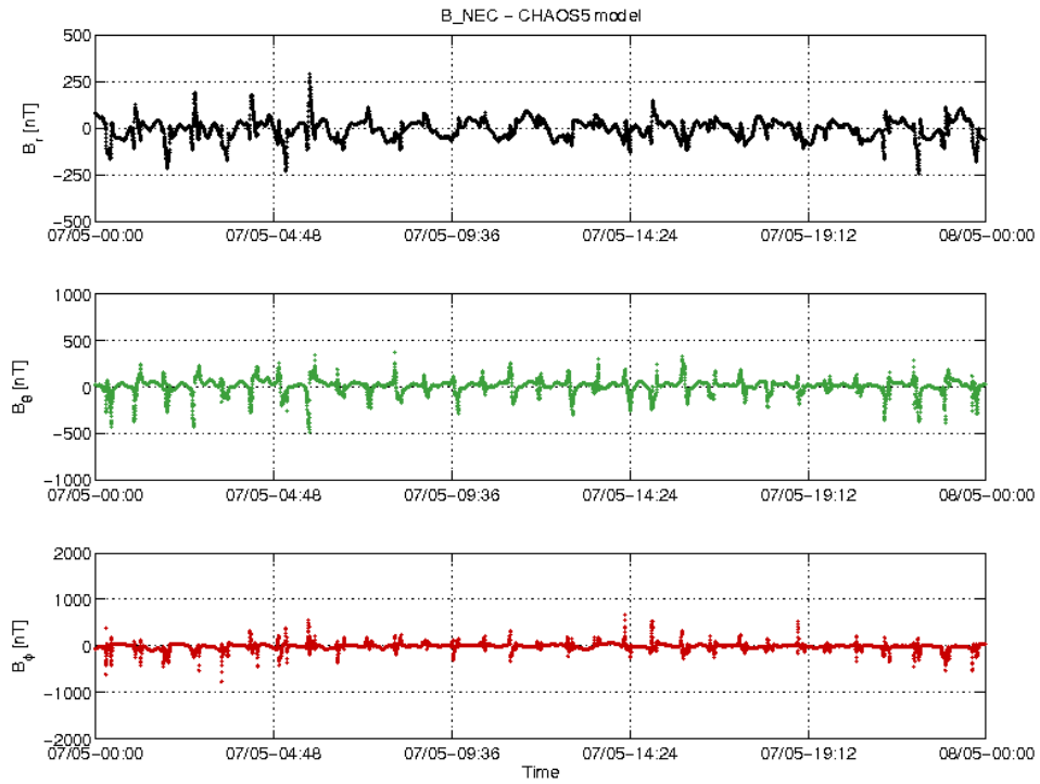
Figure 3-18: S/C A day 07.05: time series of B_{NEC} - B_{Chaos} residuals.
