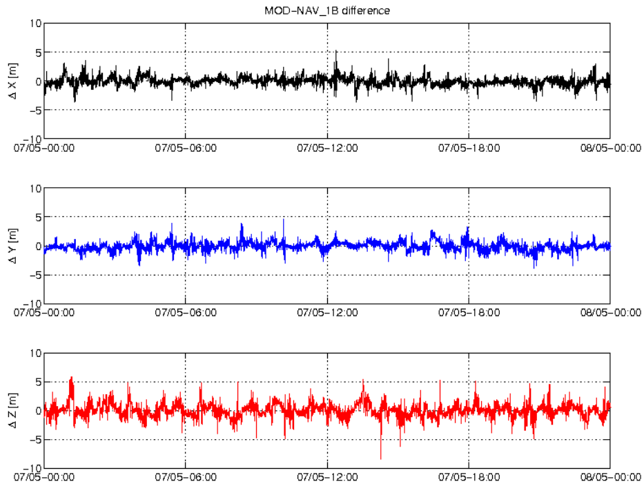
Figure 3-3: Difference MOD-GPSNAV, S/C A, 07.05. From top to bottom: X, Y and Z-axis
