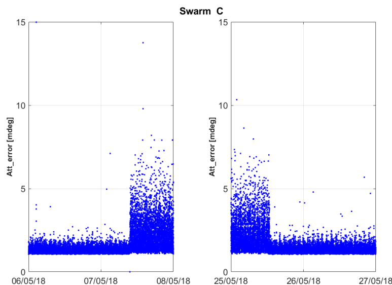
Figure 26 : Trend of Att_Error on the days 07/05 (when the anomaly was registered) and on 25/05 (when the anomaly was fixed).
