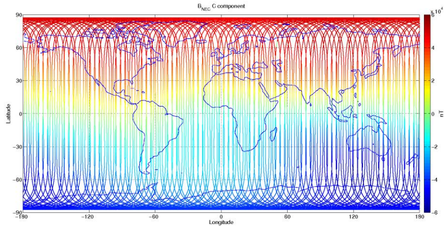
Figure 3-12: S/C C, world map plots of the geomagnetic field and components measured during monitoring period 07/05-13/05. From top to bottom: B_{NEC} components (North, East, and Centre) of magnetic field from VFM measurement.
