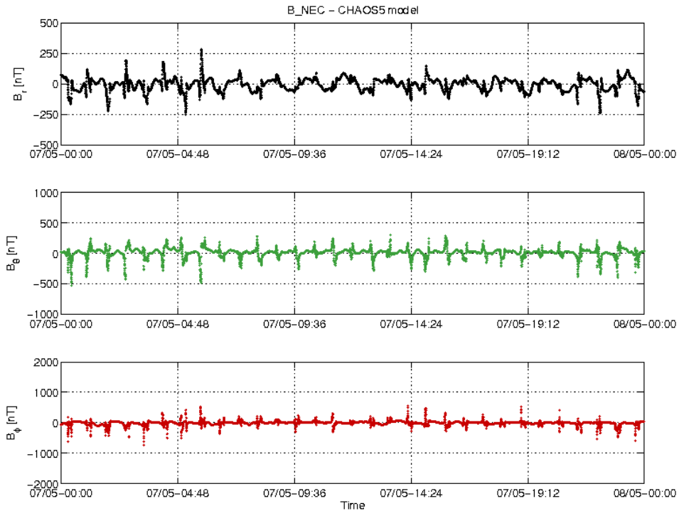
Figure 3-22: S/C C day 07.05 time series of B_{NEC} - B_{Chaos} residuals.
