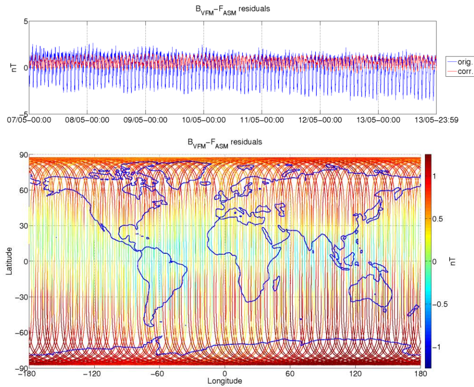
Figure 3-8: ASM-VFM residuals for S/C A, during monitoring period 07/05-13/05. In top figure are plotted: difference between |B VFM | and F ASM (without dB Sun correction) (blue colour), and the residuals with dB Sun corrections (red colour). In bottom figure residuals are presented on the world map.
