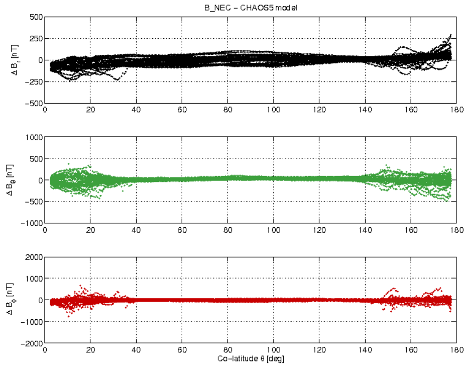
Figure 3-17: S/C A day 07.05 B_{NEC} - B_{Chaos} vs colatitude.
