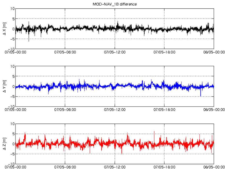
Figure 3-5: Difference MOD-GPSNAV, S/C C, 07.05. From top to bottom: X, Y and Z-axis
