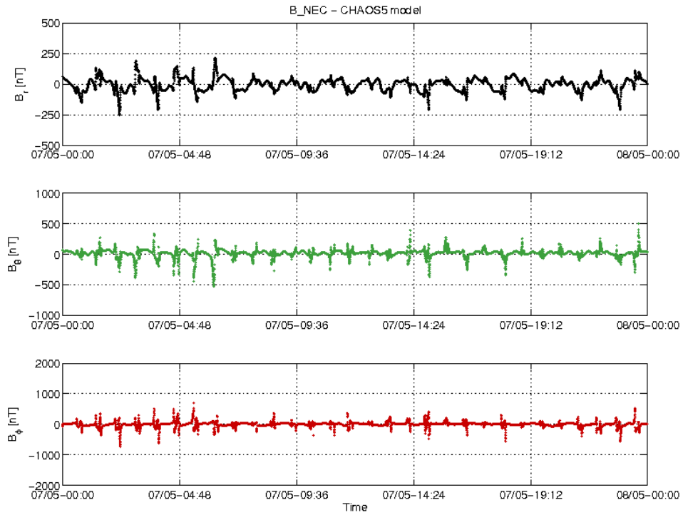
Figure 3-20: S/C B day 07.05 time series of B_{NEC} - B_{Chaos} residuals.
