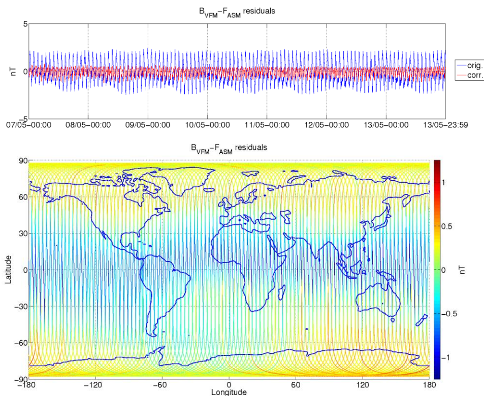
Figure 3-9: ASM-VFM residuals for S/C B, during monitoring period 07/05-13/05. In top figure are plotted: difference between |B_{VFM}| and F_{ASM} (without dB_{Sun} correction) (blue colour), and the residuals with dB_{Sun} corrections (red colour). In bottom figure residuals are presented on the world map.
