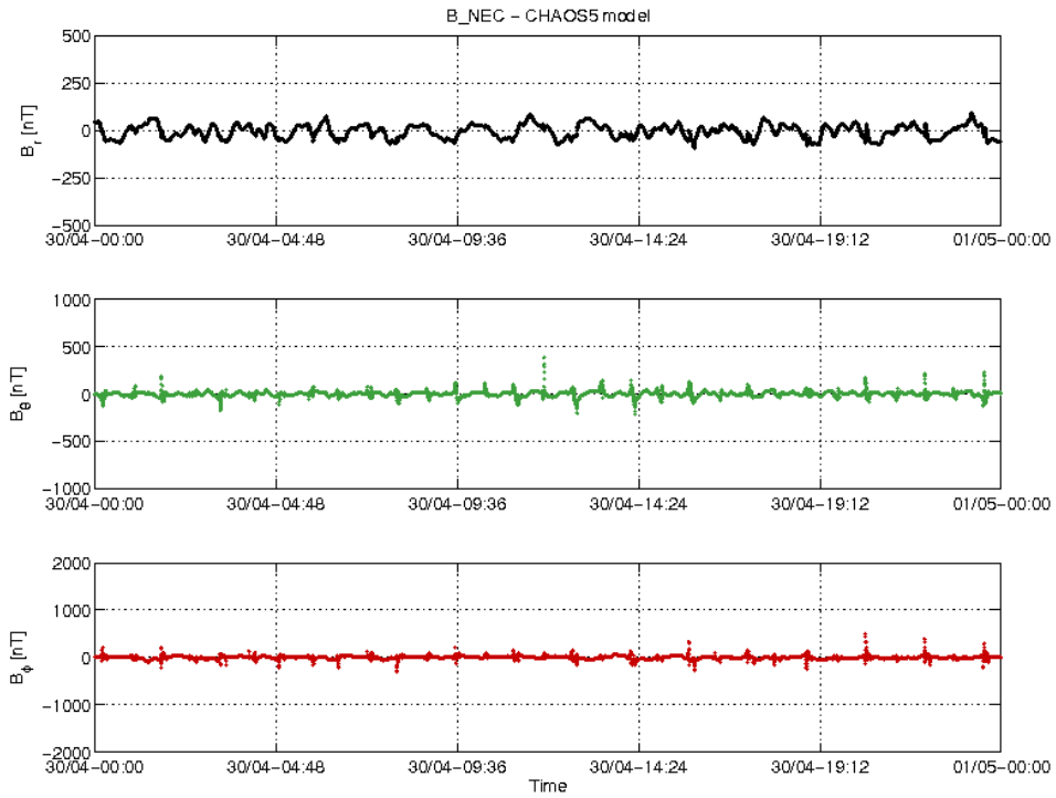
Figure 3-18: S/C A day 30.04: time series of B_{NEC} - B_{Chaos} residuals.
