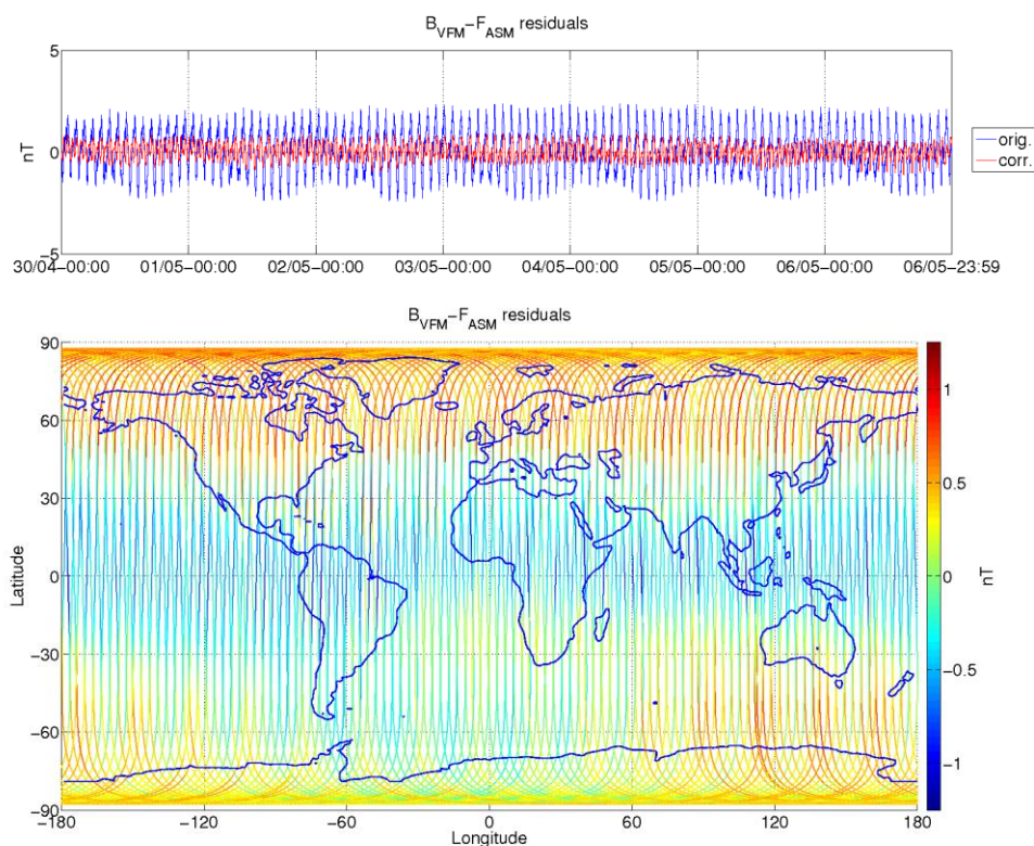
Figure 3-9: ASM-VFM residuals for S/C B, during monitoring period 30/04-06/05. In top figure are plotted: difference between |B_{VFM}| and F_{ASM} (without dB Sun correction) (blue colour), and the residuals with dB Sun corrections (red colour). In bottom figure residuals are presented on the world map.
