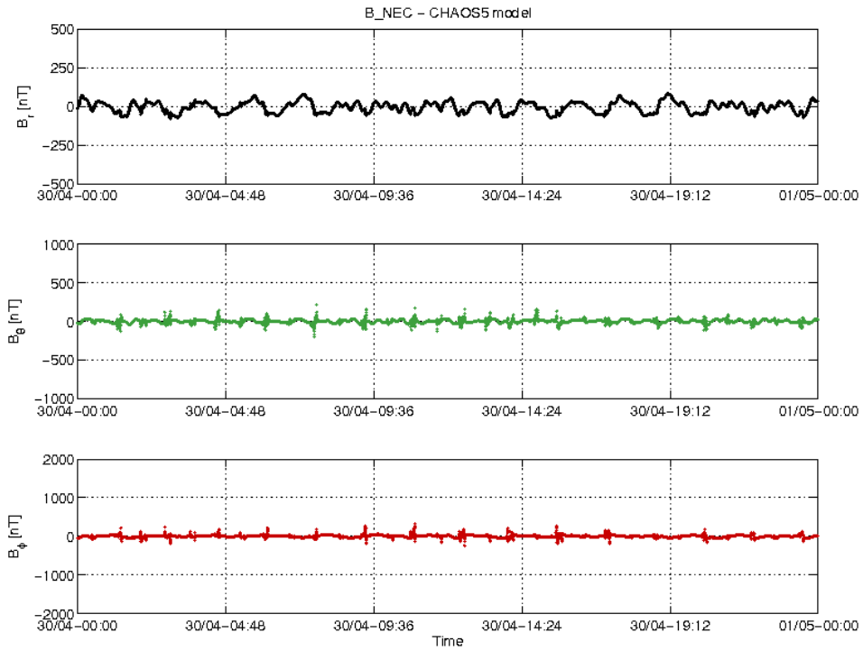
Figure 3-20: S/C B day 30.04 time series of B_{NEC} - B_{Chaos} residuals.
