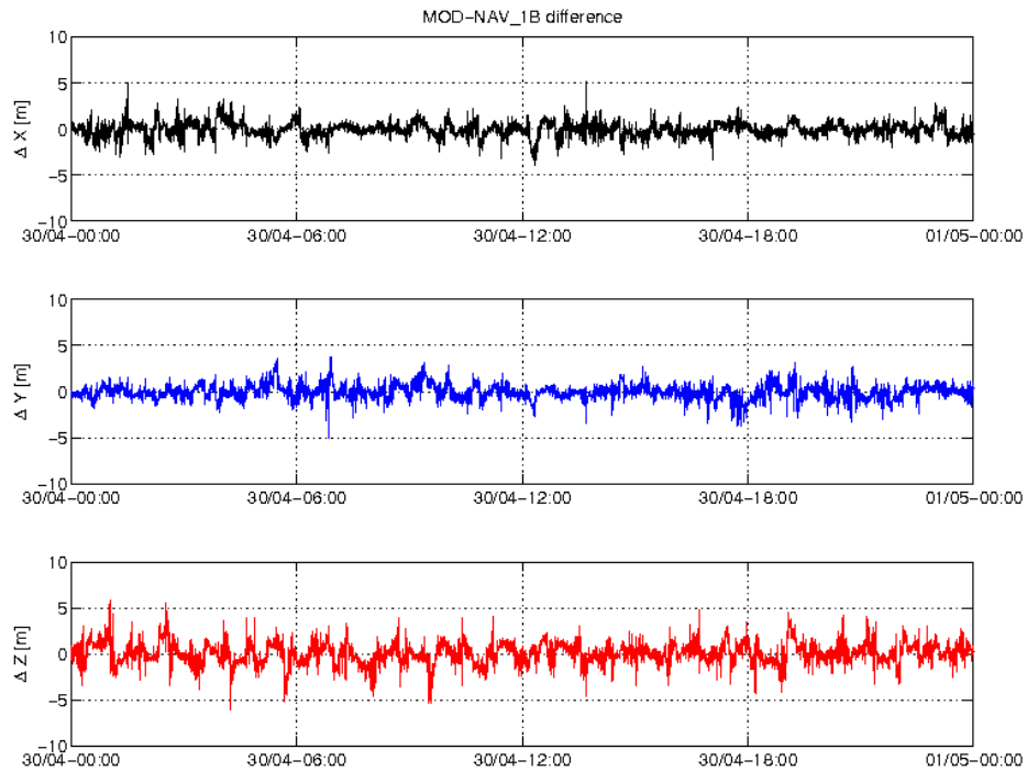
Figure 3-3: Difference MOD-GPSNAV, S/C A, 30.04. From top to bottom: X, Y and Z-axis
