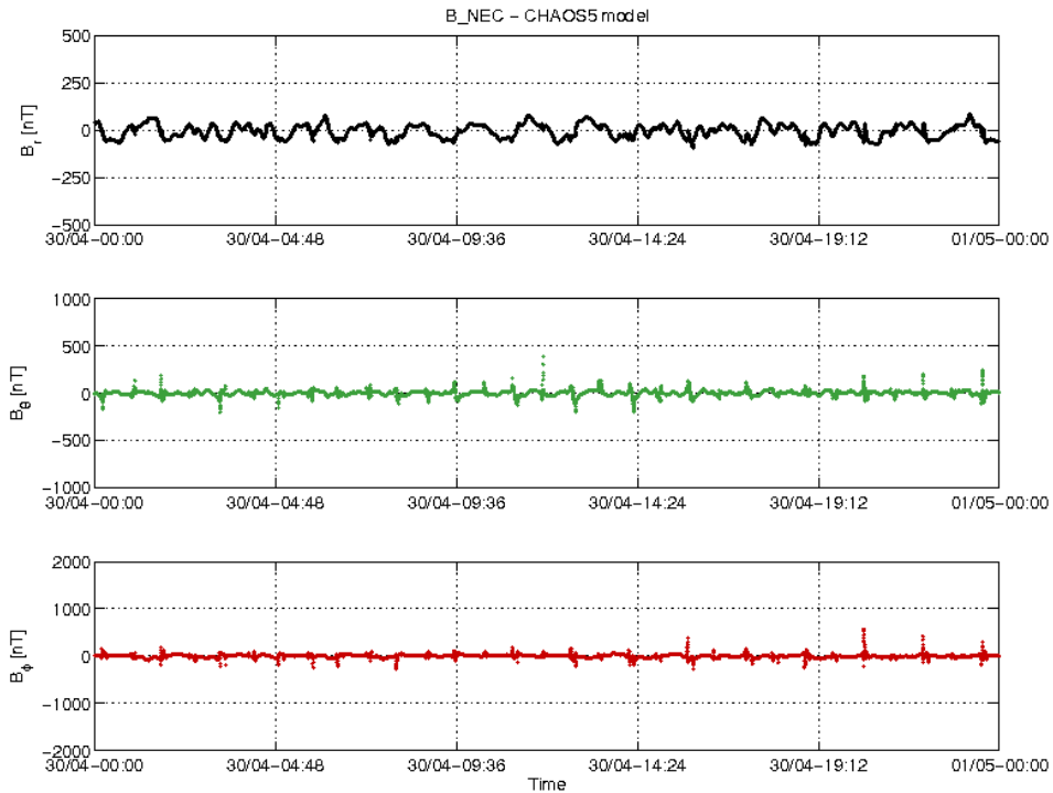
Figure 3-22: S/C C day 30.04 time series of B_{NEC} - B_{Chaos} residuals.
