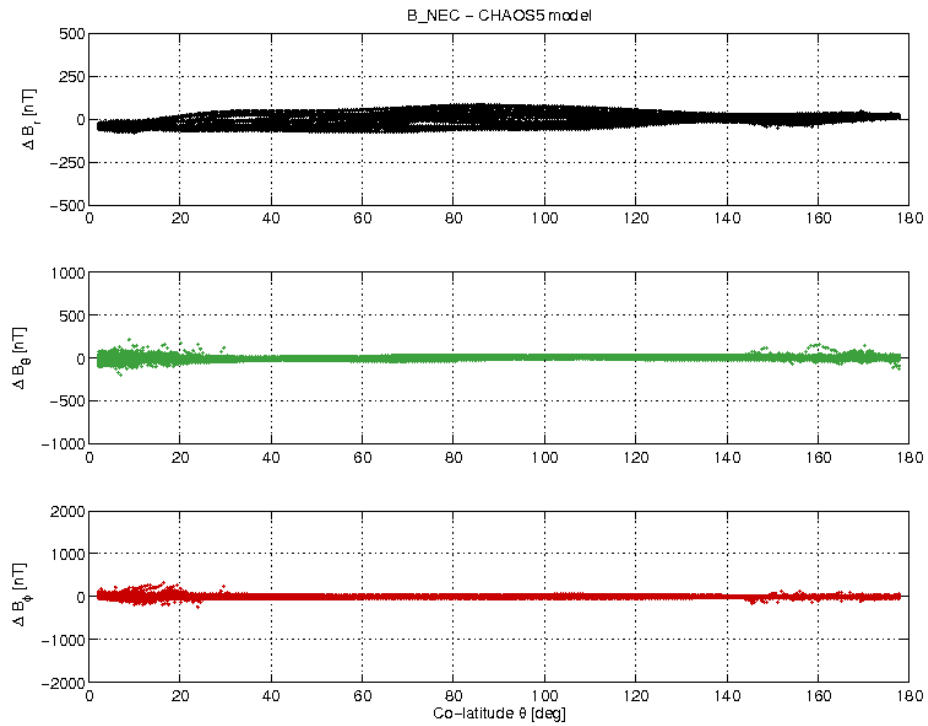
Figure 3-19: S/C B day 30.04 B_{NEC} - B_{Chaos} difference vs colatitude.
