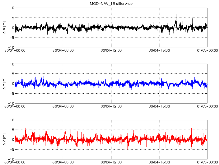
Figure 3-4: Difference MOD-GPSNAV, S/C B, 30.04. From top to bottom: X, Y and Z-axis
