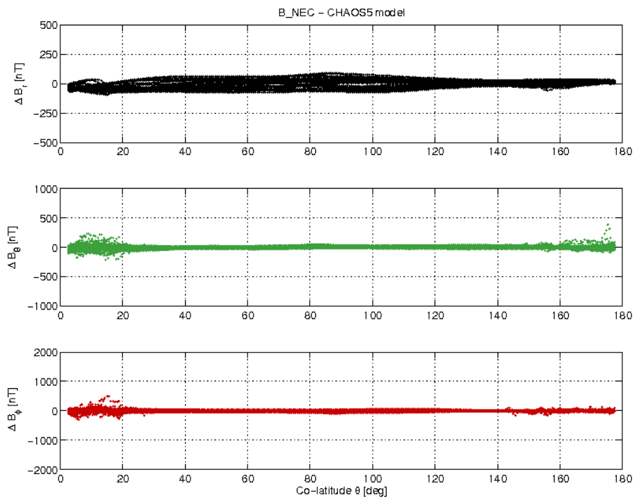
Figure 3-17: S/C A day 30.04 B_{NEC} - B_{Chaos} vs colatitude.
