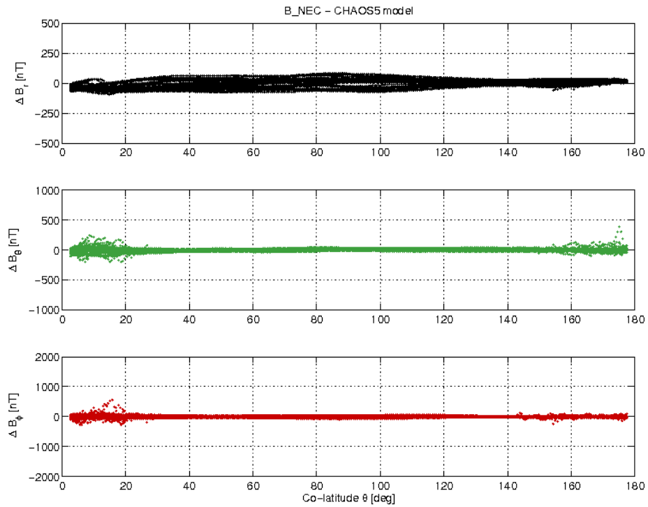
Figure 3-21: S/C C day 30.04 B_{NEC} - B_{Chaos} difference vs colatitude.
