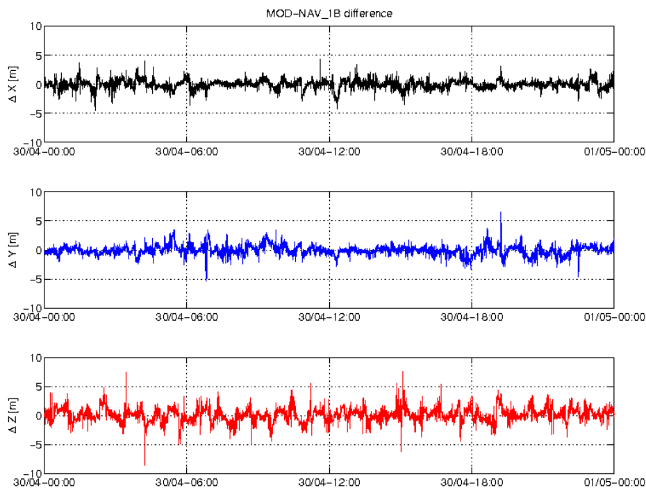
Figure 3-5: Difference MOD-GPSNAV, S/C C, 30.04. From top to bottom: X, Y and Z-axis
