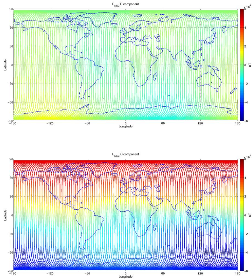
Figure 3-11: S/C B, world map plots of the geomagnetic field and components measured during monitoring period 30/04-06/05. From top to bottom: F-magnetic field from ASM measurement, B_{NEC} components (North, East, and Centre) of magnetic field from VFM measurement.
