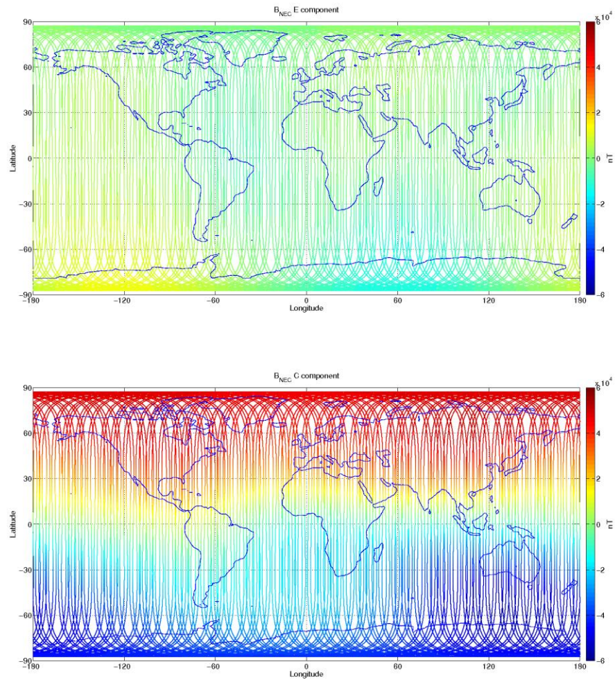
Figure 3-10: S/C A, world map plots of the geomagnetic field and components measured during monitoring period 30/04-06/05. From top to bottom: F-magnetic field from ASM measurement, B_{NEC} components (North, East, and Centre) of magnetic field from VFM measurement.
