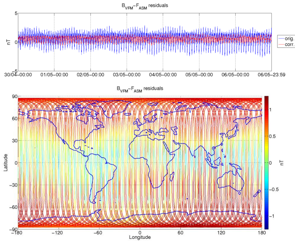
Figure 3-8: ASM-VFM residuals for S/C A, during monitoring period 30/04-06/05. In top figure are plotted: difference between |B VFM | and F ASM (without dB Sun correction) (blue colour), and the residuals with dB Sun corrections (red colour). In bottom figure residuals are presented on the world map.
