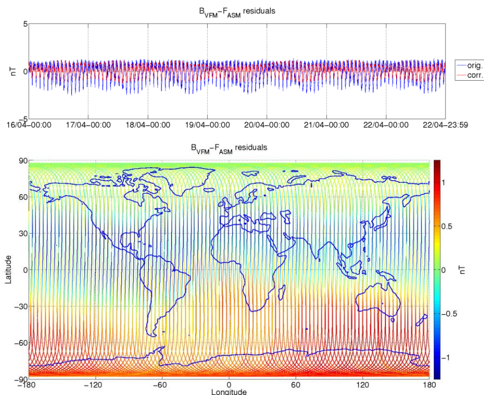
Figure 3-9: ASM-VFM residuals for S/C B, during monitoring period 16/04-22/04. In top figure are plotted: difference between |B_{VFM}| and F_{ASM} (without dB_Sun correction) (blue colour), and the residuals with dB_Sun corrections (red colour). In bottom figure residuals are presented on the world map.
