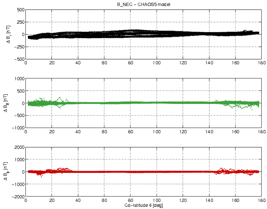
Figure 3-19: S/C B day 16.04 B_{NEC} - B_{Chaos} difference vs colatitude.
