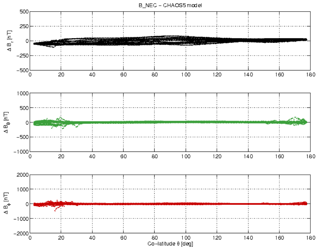
Figure 3-21: S/C C day 16.04 B_{NEC} - B_{Chaos} difference vs colatitude.
