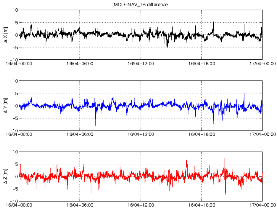
Figure 3-3: Difference MOD-GPSNAV, S/C A, 16.04. From top to bottom: X, Y and Z-axis
