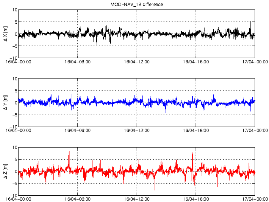
Figure 3-4: Difference MOD-GPSNAV, S/C B, 16.04. From top to bottom: X, Y and Z-axis
