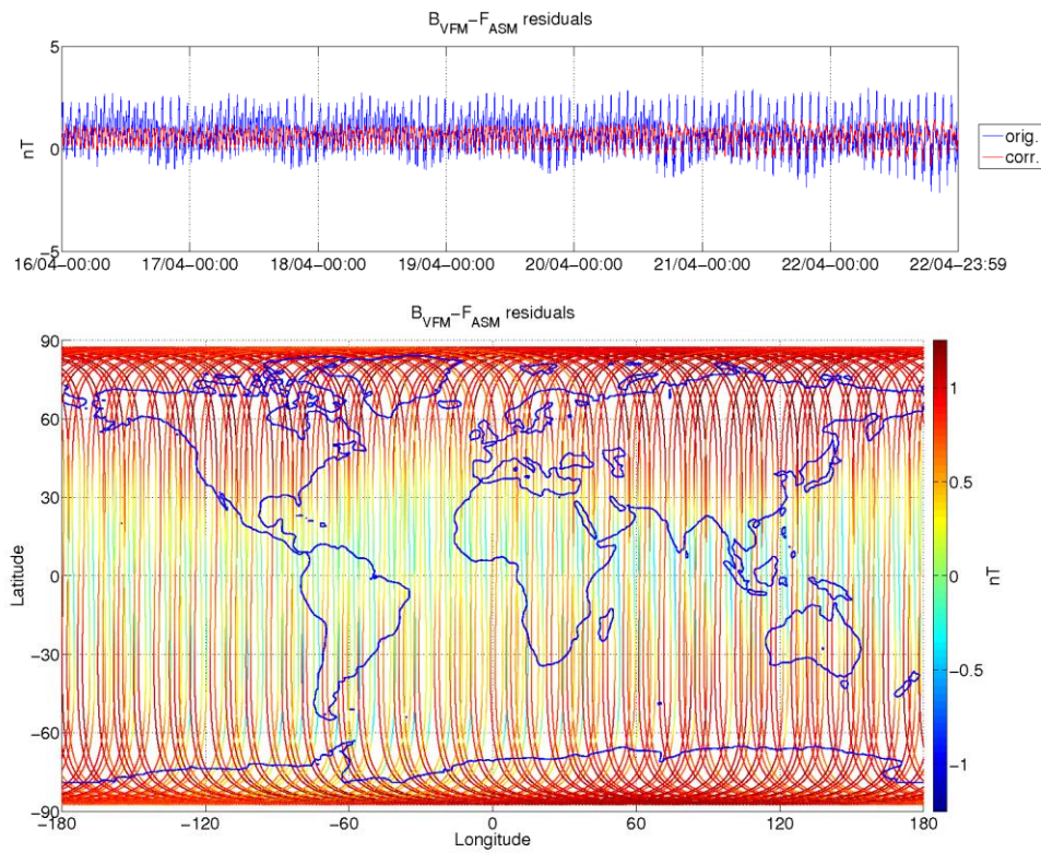
Figure 3-8: ASM-VFM residuals for S/C A, during monitoring period 16/04-22/04. In top figure are plotted: difference between |B VFM | and F ASM (without dB Sun correction) (blue colour), and the residuals with dB Sun corrections (red colour). In bottom figure residuals are presented on the world map.
