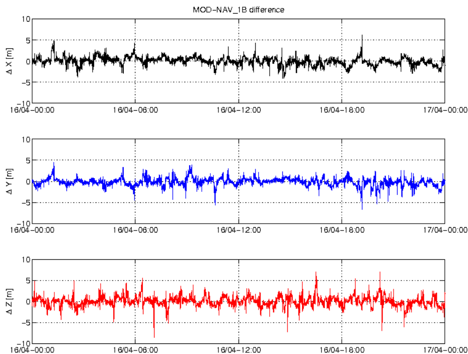
Figure 3-5: Difference MOD-GPSNAV, S/C C, 16.04. From top to bottom: X, Y and Z-axis
