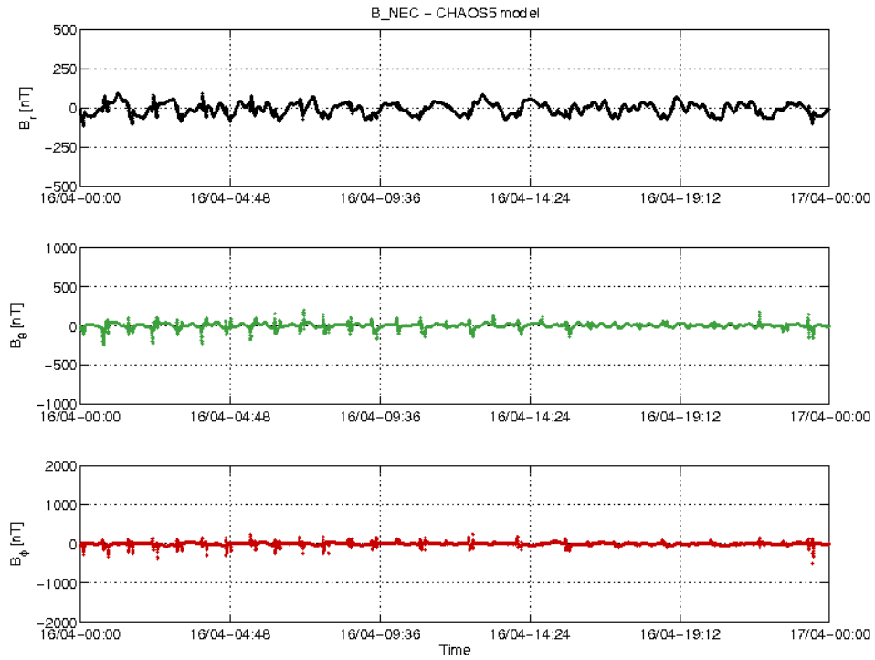
Figure 3-18: S/C A day 16.04: time series of B_{NEC} - B_{Chaos} residuals.
