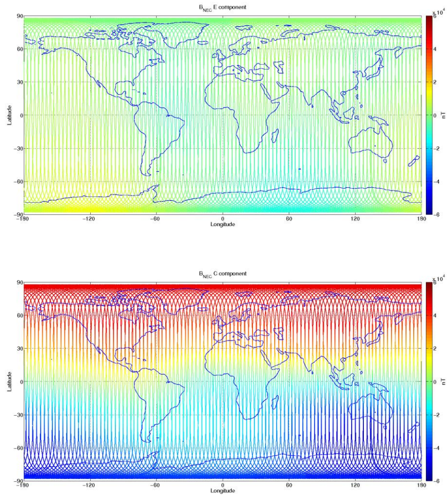
Figure 3-11: S/C B, world map plots of the geomagnetic field and components measured during monitoring period 16/04-22/04. From top to bottom: F-magnetic field from ASM measurement, B_{NEC} components (North, East, and Centre) of magnetic field from VFM measurement.
