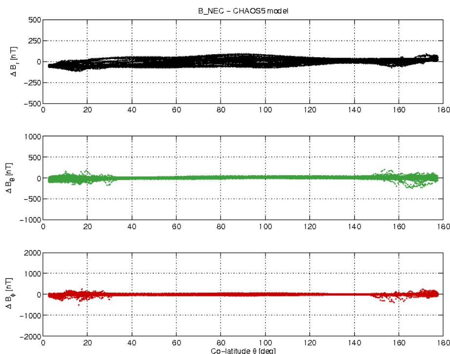
Figure 3-17: S/C A day 16.04 B_{NEC} - B_{Chaos} vs colatitude.
