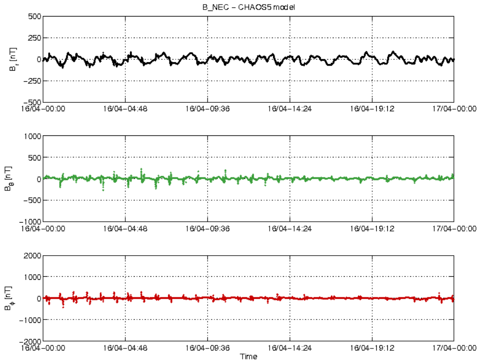
Figure 3-20: S/C B day 16.04 time series of B_{NEC} - B_{Chaos} residuals.
