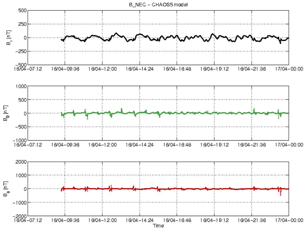
Figure 3-22: S/C C day 16.04 time series of B_{NEC} - B_{Chaos} residuals.
