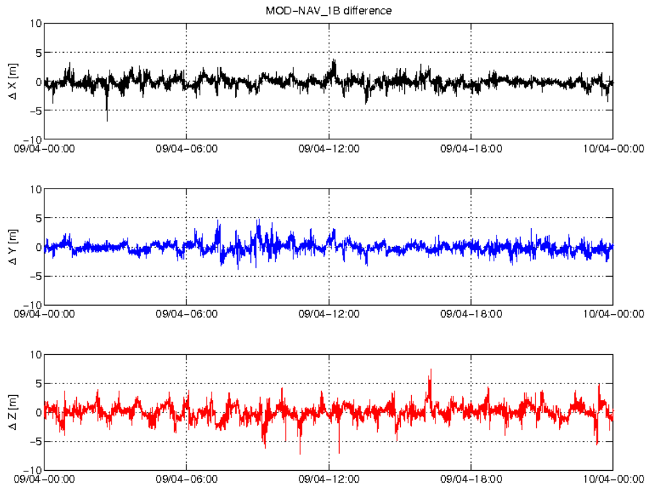
Figure 3-3: Difference MOD-GPSNAV, S/C A, 09.04. From top to bottom: X, Y and Z-axis
