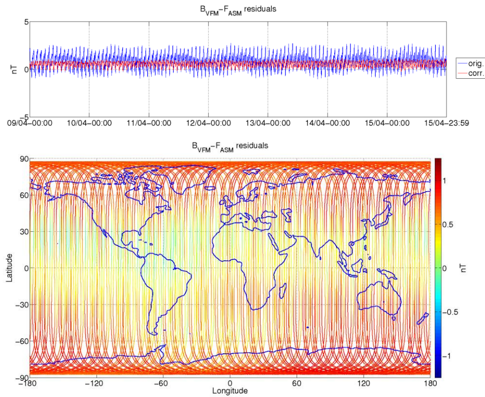
Figure 3-8: ASM-VFM residuals for S/C A, during monitoring period 09/04-15/04. In top figure are plotted: difference between |B VFM | and F ASM (without dB Sun correction) (blue colour), and the residuals with dB Sun corrections (red colour). In bottom figure residuals are presented on the world map.
