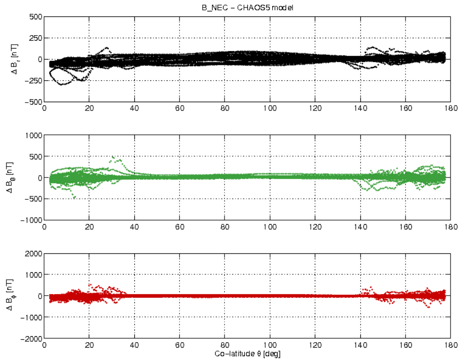
Figure 3-21: S/C C day 09.04 B_{NEC} - B_{Chaos} difference vs colatitude.
