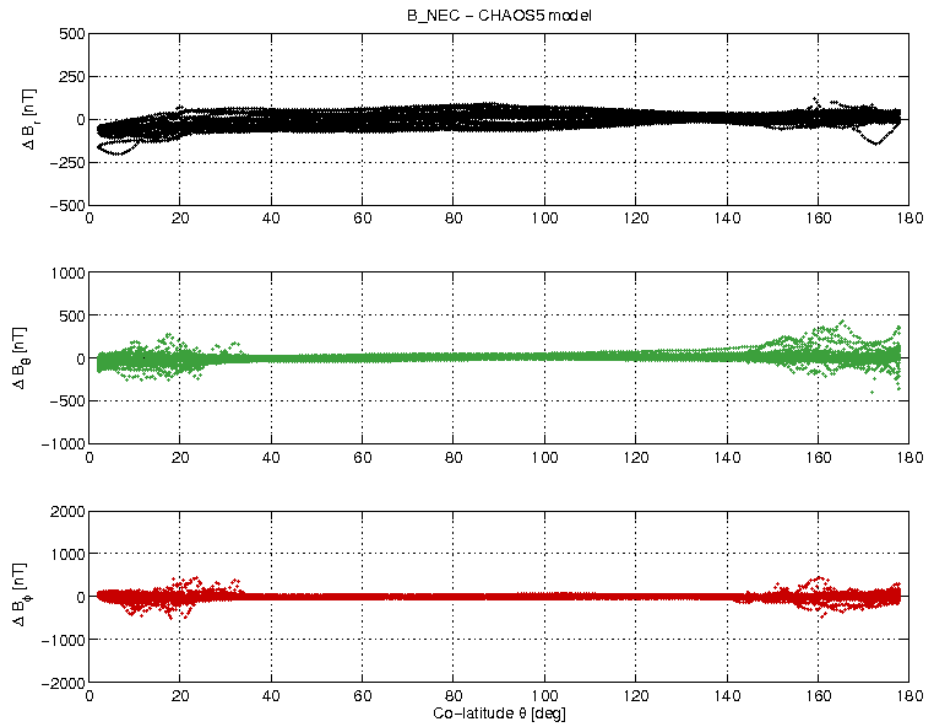
Figure 3-19: S/C B day 09.04 B_{NEC} - B_{Chaos} difference vs colatitude.
