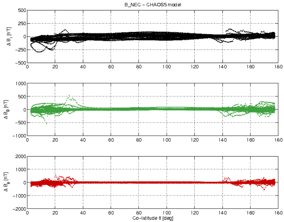
Figure 3-17: S/C A day 09.04 B_{NEC} - B_{Chaos} vs colatitude.
