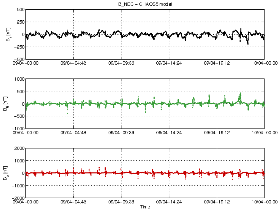
Figure 3-20: S/C B day 09.04 time series of B_{NEC} - B_{Chaos} residuals.
