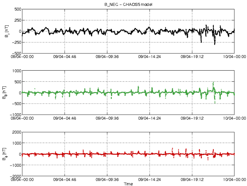
Figure 3-22: S/C C day 09.04 time series of B_{NEC} - B_{Chaos} residuals.
