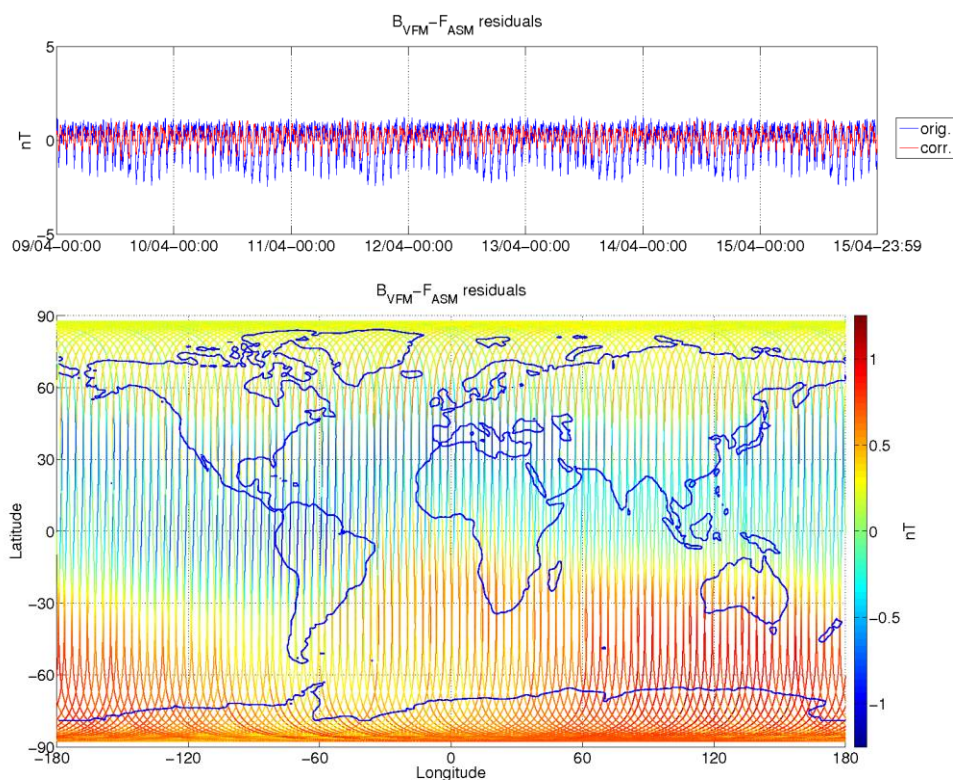
Figure 3-9: ASM-VFM residuals for S/C B, during monitoring period 09/04-15/04. In top figure are plotted: difference between |B_{VFM}| and F_{ASM} (without dB_{Sun} correction) (blue colour), and the residuals with dB_{Sun} corrections (red colour). In bottom figure residuals are presented on the world map.
