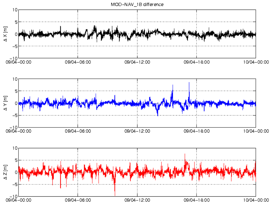
Figure 3-4: Difference MOD-GPSNAV, S/C B, 09.04. From top to bottom: X, Y and Z-axis
