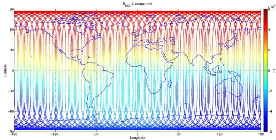
Figure 3-12: S/C C, world map plots of the geomagnetic field and components measured during monitoring period 09/04-15/04. From top to bottom: B_{NEC} components (North, East, and Centre) of magnetic field from VFM measurement.
