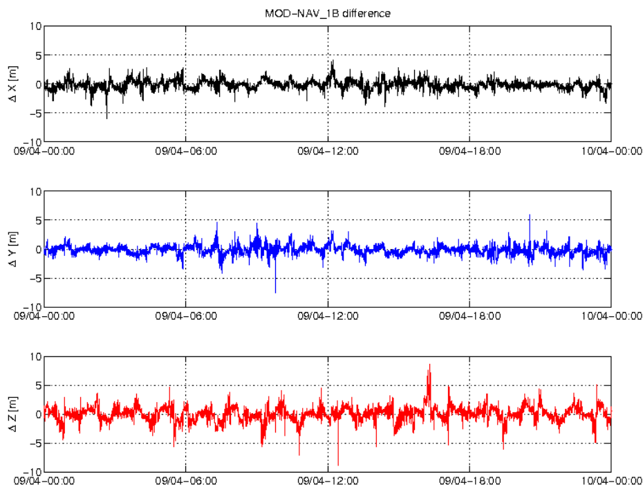
Figure 3-5: Difference MOD-GPSNAV, S/C C, 09.04. From top to bottom: X, Y and Z-axis
