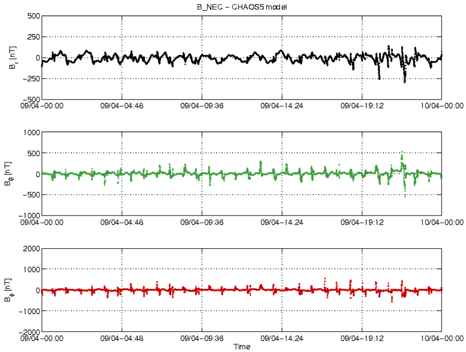
Figure 3-18: S/C A day 09.04: time series of B_{NEC} - B_{Chaos} residuals.
