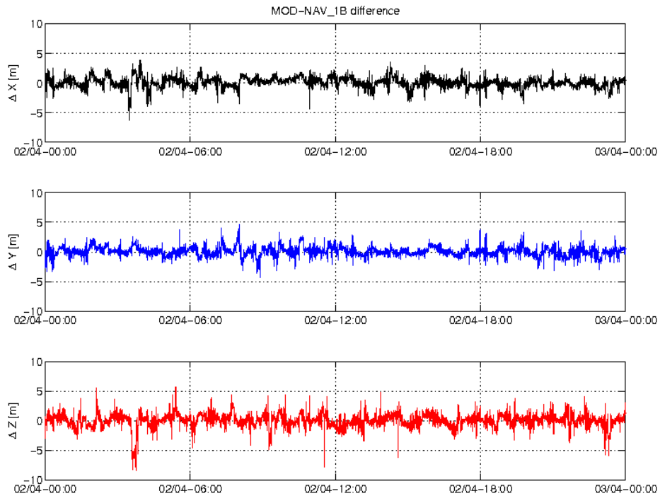
Figure 3-3: Difference MOD-GPSNAV, S/C A, 02.04. From top to bottom: X, Y and Z-axis
