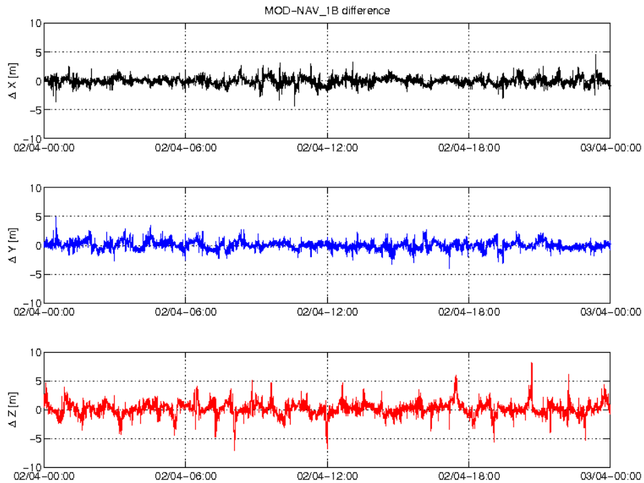
Figure 3-4: Difference MOD-GPSNAV, S/C B, 02.04. From top to bottom: X, Y and Z-axis
