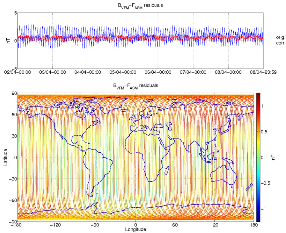
Figure 3-8: ASM-VFM residuals for S/C A, during monitoring period 02/04-08/04. In top figure are plotted: difference between |B VFM | and F ASM (without dB Sun correction) (blue colour), and the residuals with dB Sun corrections (red colour). In bottom figure residuals are presented on the world map.
