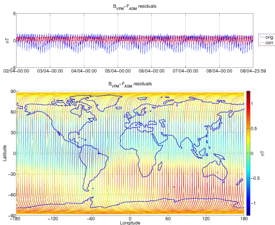
Figure 3-9: ASM-VFM residuals for S/C B, during monitoring period 02/04-08/04. In top figure are plotted: difference between |B\_VFM| and F\_ASM (without dB\_Sun correction) (blue colour), and the residuals with dB\_Sun corrections (red colour). In bottom figure residuals are presented on the world map.
