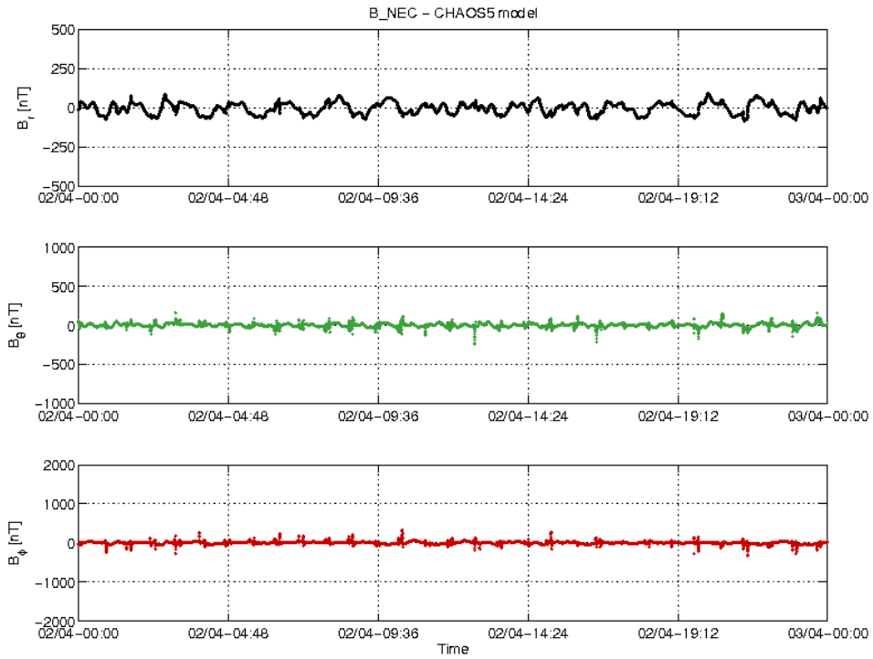
Figure 3-20: S/C B day 02.04 time series of B_{NEC} - B_{Chaos} residuals.
