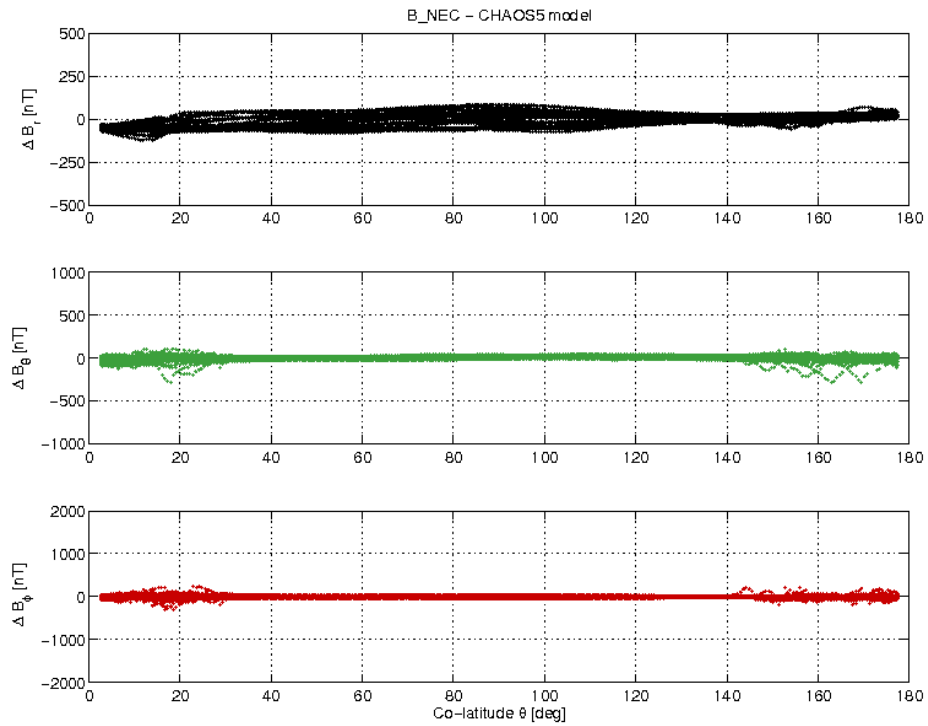
Figure 3-21: S/C C day 02.04 B_{NEC} - B_{Chaos} difference vs colatitude.
