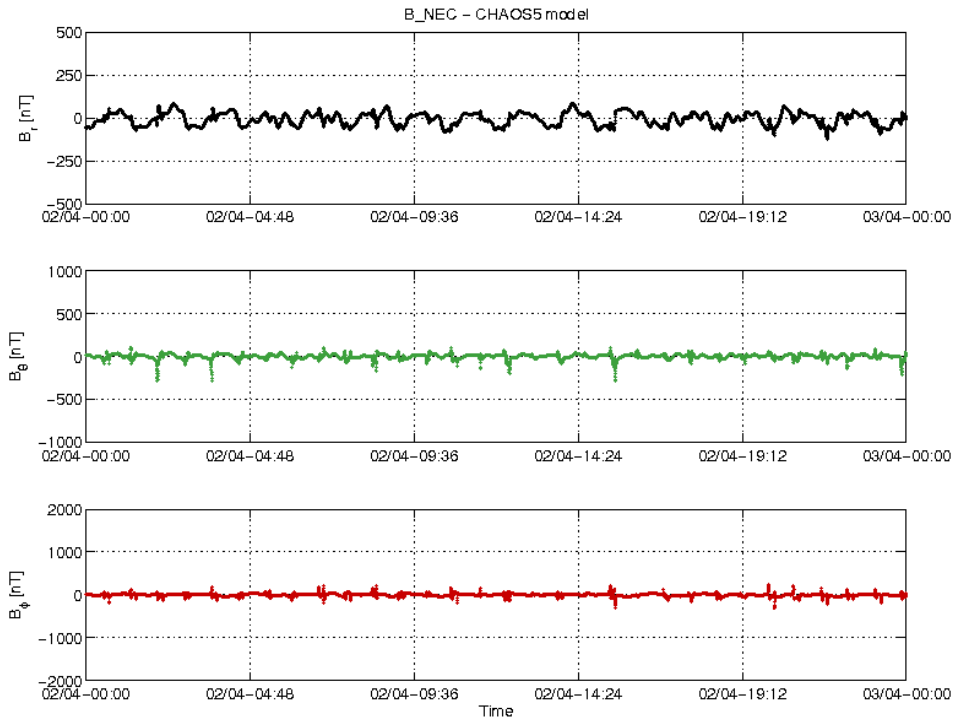
Figure 3-22: S/C C day 02.04 time series of B_{NEC} - B_{Chaos} residuals.
