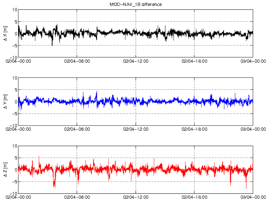
Figure 3-5: Difference MOD-GPSNAV, S/C C, 02.04. From top to bottom: X, Y and Z-axis
