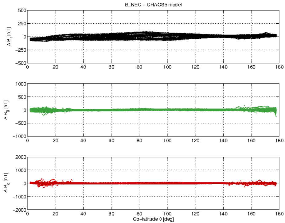
Figure 3-19: S/C B day 02.04 B_{NEC} - B_{Chaos} difference vs colatitude.
