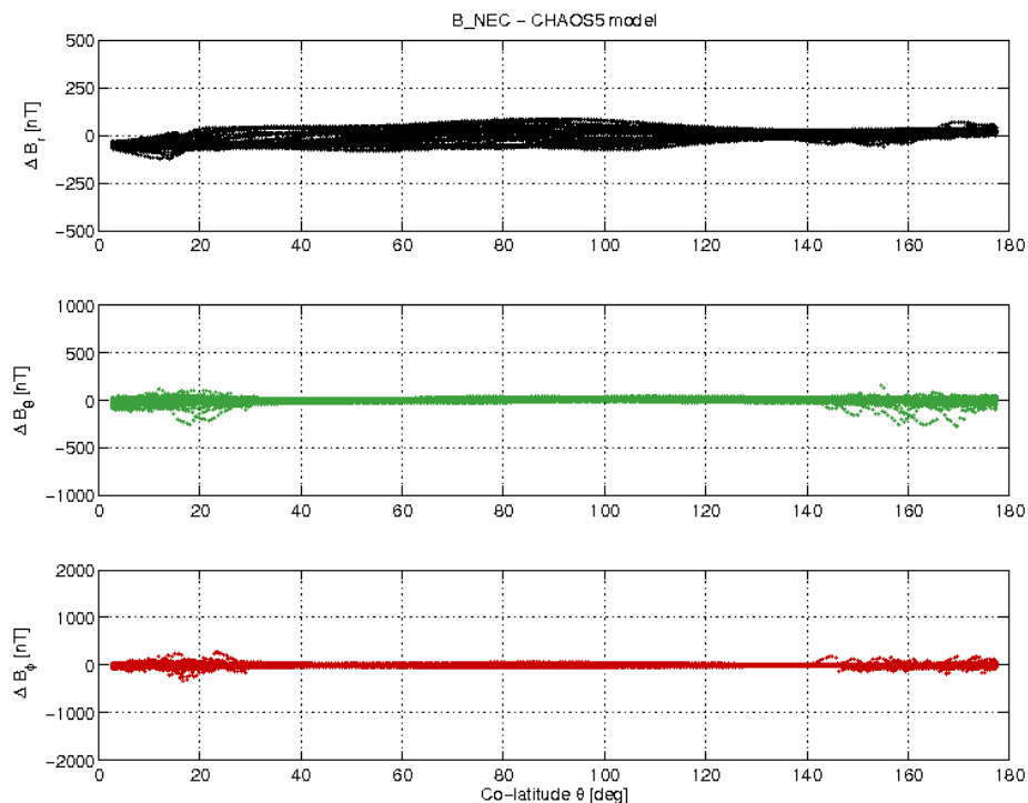
Figure 3-17: S/C A day 02.04 B_{NEC} - B_{Chaos} vs colatitude.
