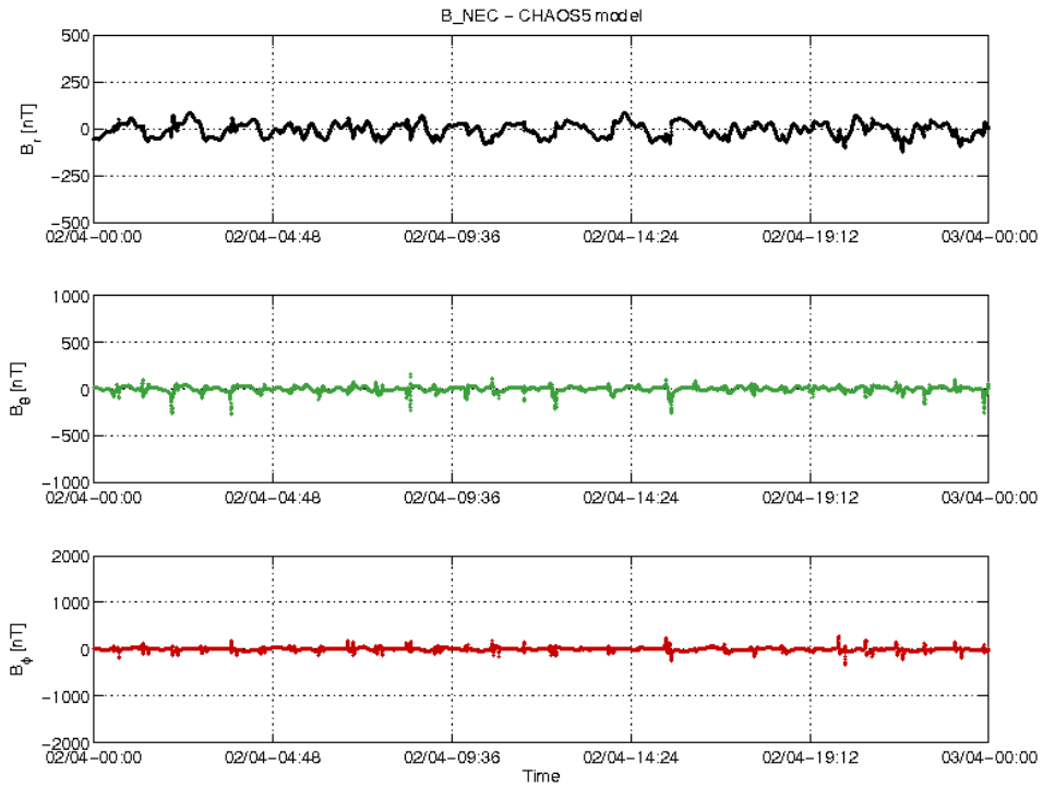
Figure 3-18: S/C A day 02.04: time series of B_{NEC} - B_{Chaos} residuals.
