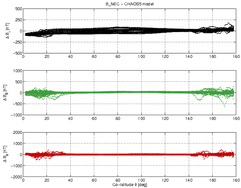
Figure 3-19: S/C B day 26.03 B_{NEC} - B_{Chaos} difference vs colatitude.
