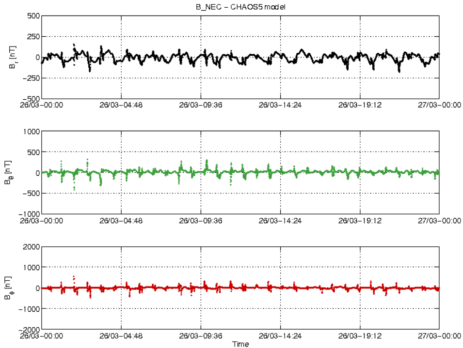
Figure 3-22: S/C C day 26.03 time series of B_{NEC} - B_{Chaos} residuals.
