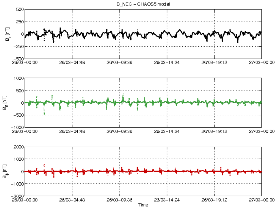
Figure 3-18: S/C A day 26.03: time series of B_{NEC} - B_{Chaos} residuals.
