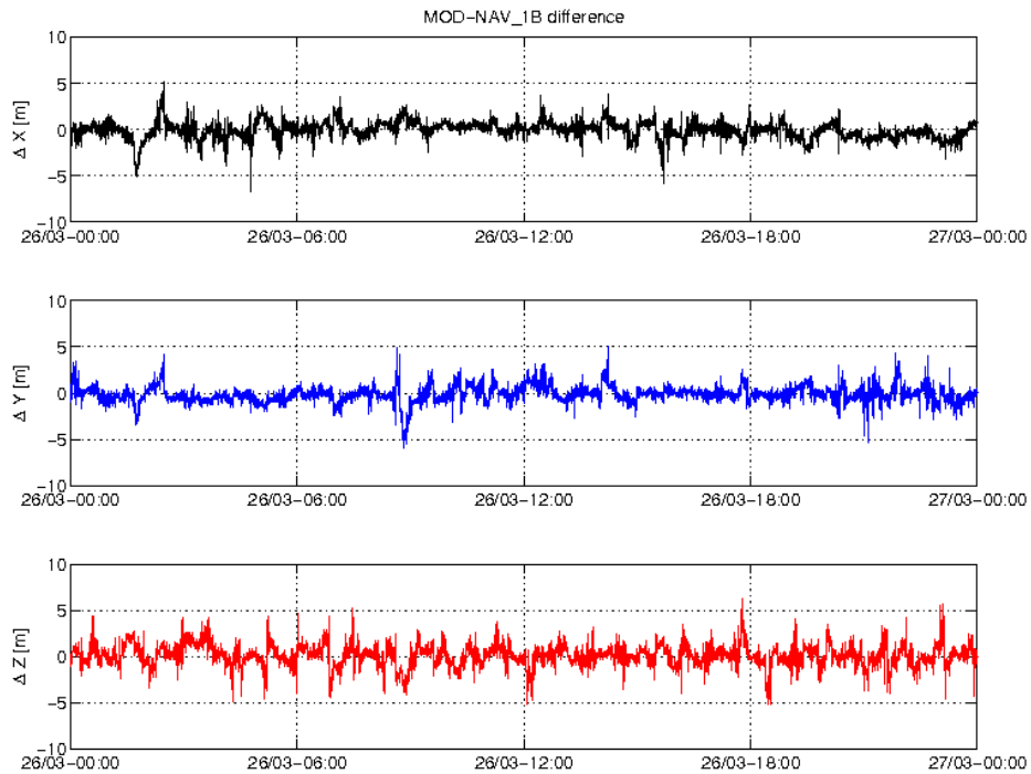
Figure 3-5: Difference MOD-GPSNAV, S/C C, 26.03. From top to bottom: X, Y and Z-axis
