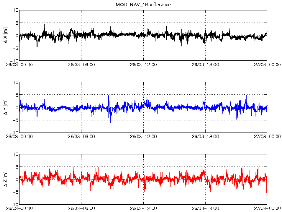
Figure 3-3: Difference MOD-GPSNAV, S/C A, 26.03. From top to bottom: X, Y and Z-axis
