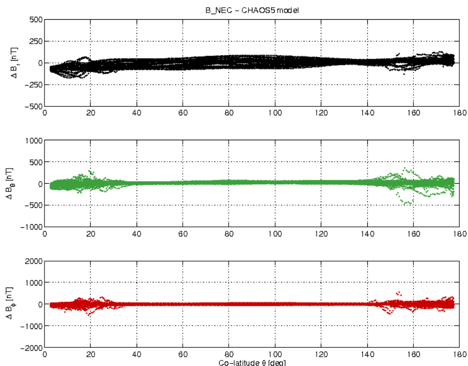
Figure 3-17: S/C A day 26.03 B_{NEC} - B_{Chaos} vs colatitude.
