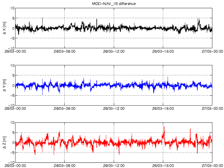
Figure 3-4: Difference MOD-GPSNAV, S/C B, 26.03. From top to bottom: X, Y and Z-axis
