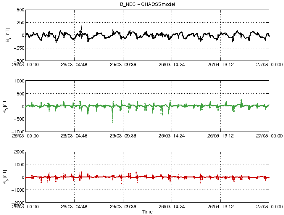
Figure 3-20: S/C B day 26.03 time series of B_{NEC} - B_{Chaos} residuals.
