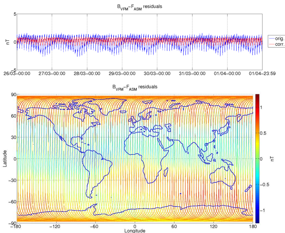
Figure 3-9: ASM-VFM residuals for S/C B, during monitoring period 26/03-01/04. In top figure are plotted: difference between |B_{VFM}| and F_{ASM} (without dB Sun correction) (blue colour), and the residuals with dB Sun corrections (red colour). In bottom figure residuals are presented on the world map.
