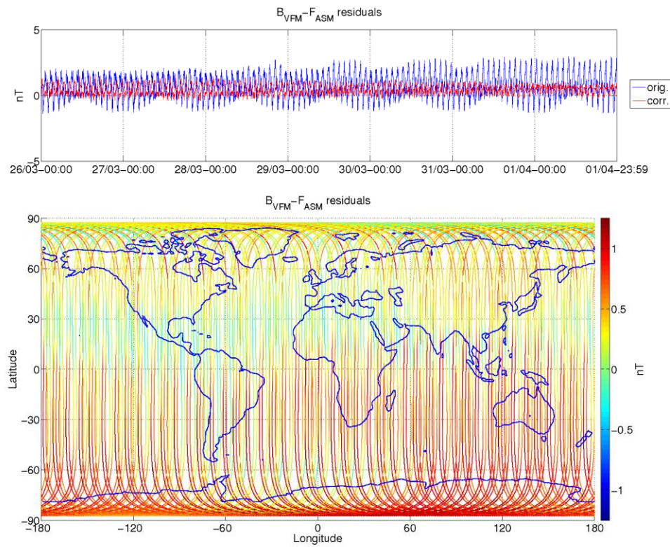
Figure 3-8: ASM-VFM residuals for S/C A, during monitoring period 26/03-01/04. In top figure are plotted: difference between |B VFM | and F ASM (without dB Sun correction) (blue colour), and the residuals with dB Sun corrections (red colour). In bottom figure residuals are presented on the world map.
