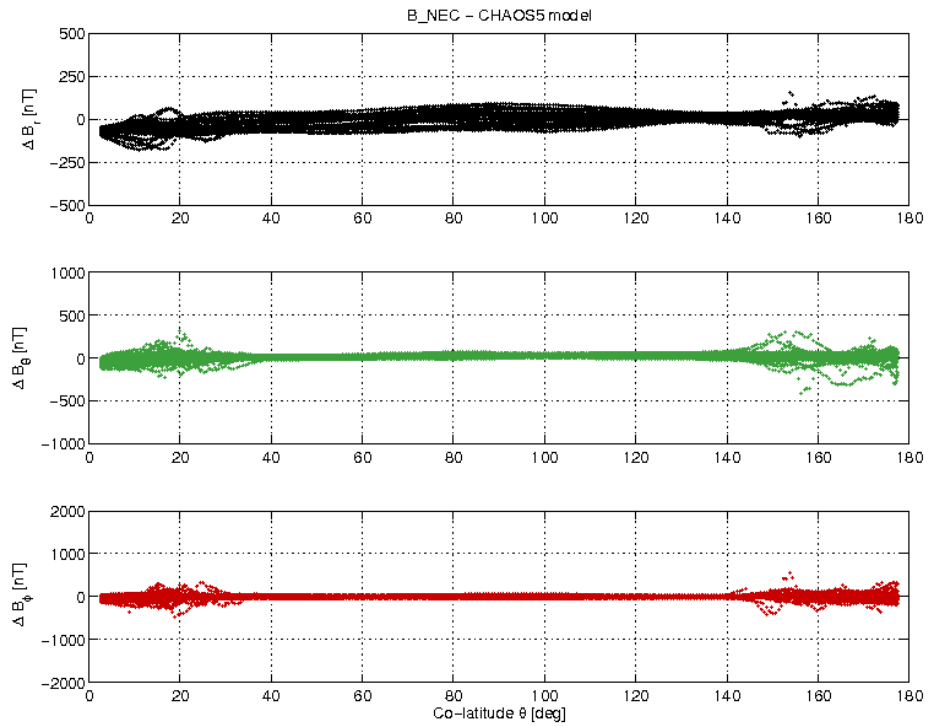
Figure 3-21: S/C C day 26.03 B NEC - B Chaos difference vs colatitude.
