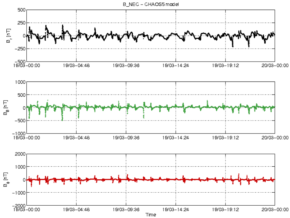
Figure 3-18: S/C A day 19.03: time series of B_{NEC} - B_{Chaos} residuals.
