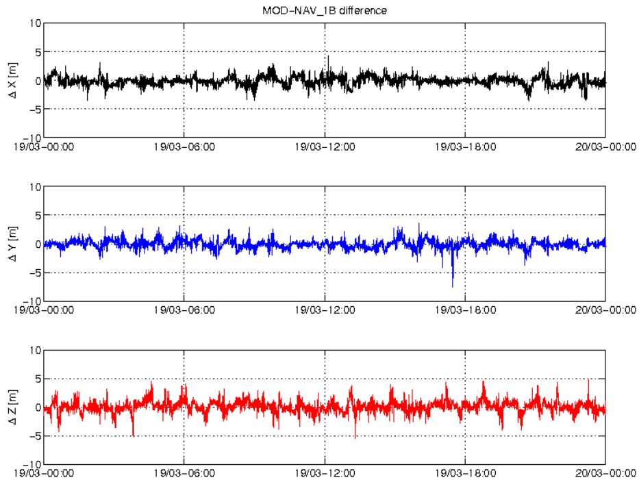
Figure 3-4: Difference MOD-GPSNAV, S/C B, 19.03. From top to bottom: X, Y and Z-axis
