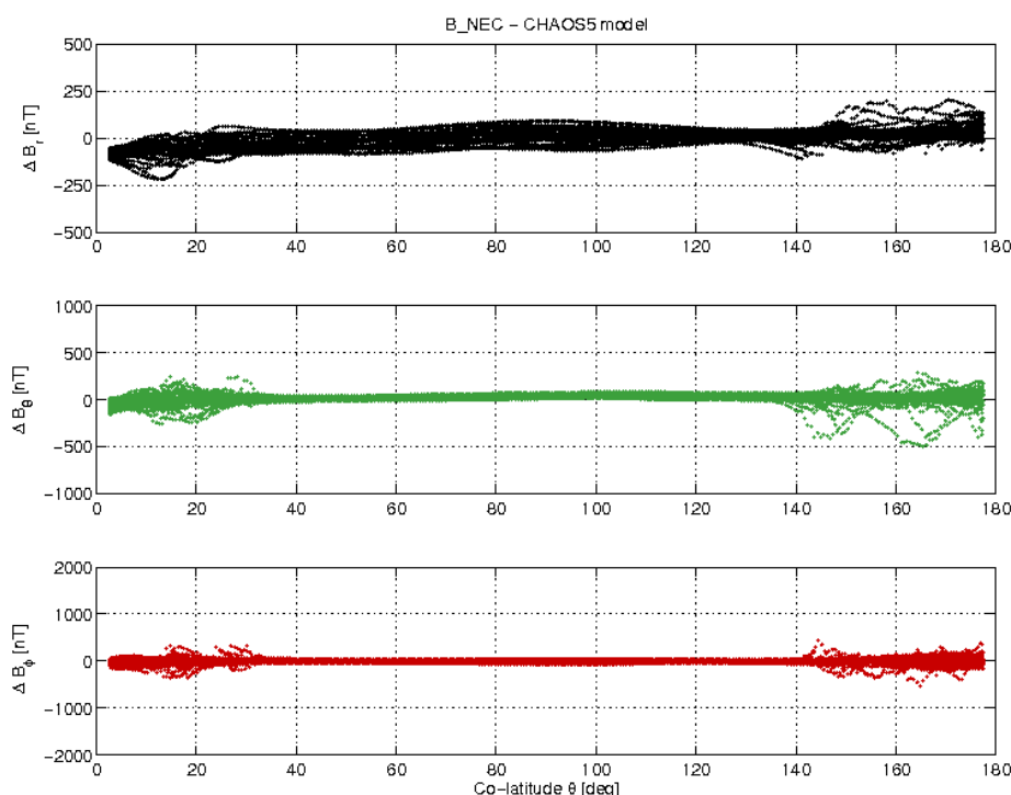
Figure 3-17: S/C A day 19.03 B_{NEC} - B_{Chaos} vs colatitude.
