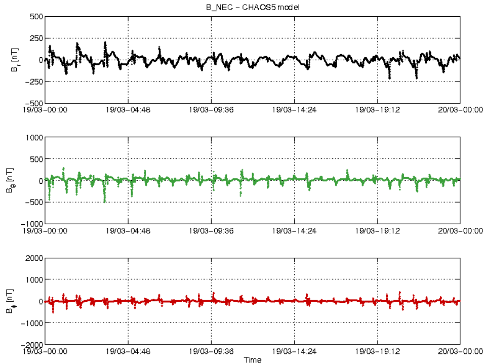
Figure 3-22: S/C C day 19.03 time series of B_{NEC} - B_{Chaos} residuals.
