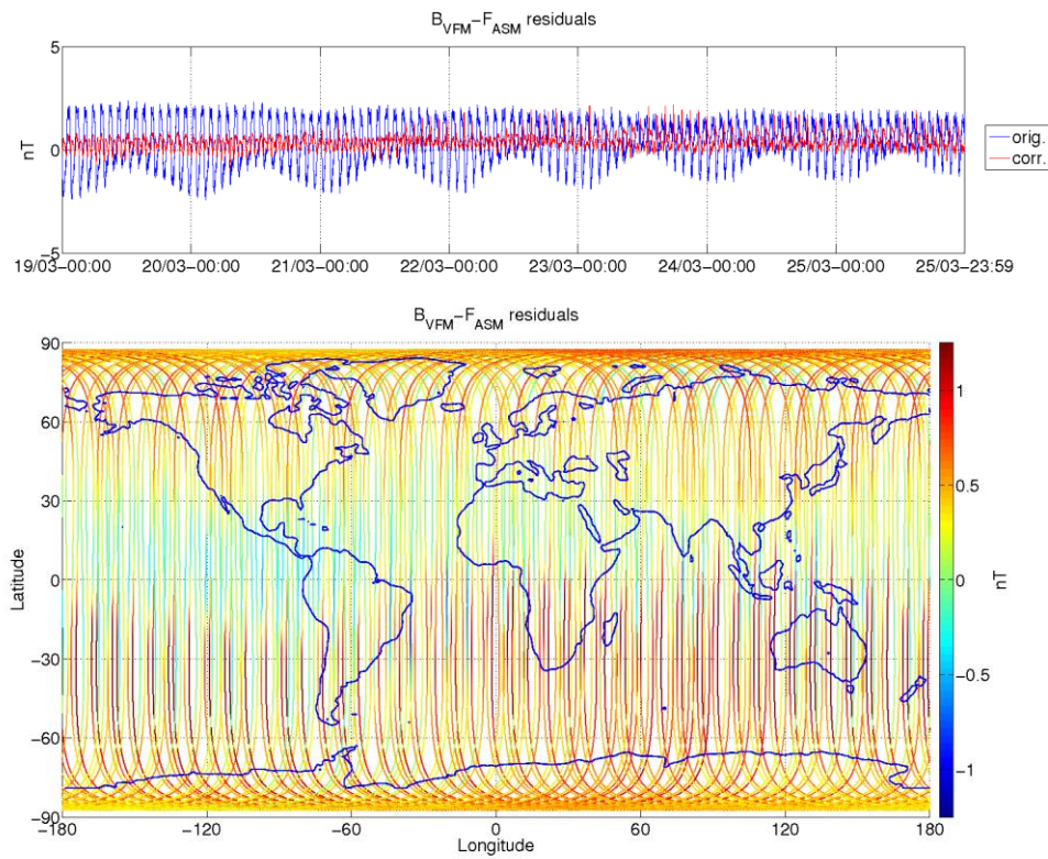
Figure 3-8: ASM-VFM residuals for S/C A, during monitoring period 19/03-25/03. In top figure are plotted: difference between |B VFM | and F ASM (without dB Sun correction) (blue colour), and the residuals with dB Sun corrections (red colour). In bottom figure residuals are presented on the world map.
