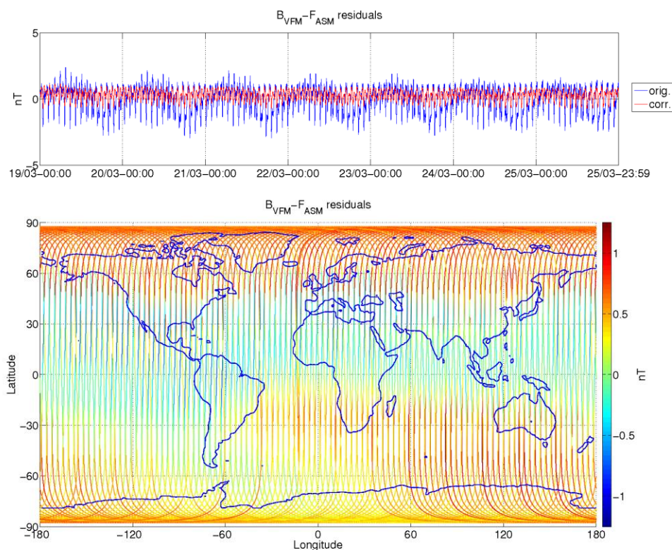
Figure 3-9: ASM-VFM residuals for S/C B, during monitoring period 19/03-25/03. In top figure are plotted: difference between |B_{VFM}| and F_{ASM} (without dB_Sun correction) (blue colour), and the residuals with dB_Sun corrections (red colour). In bottom figure residuals are presented on the world map.
