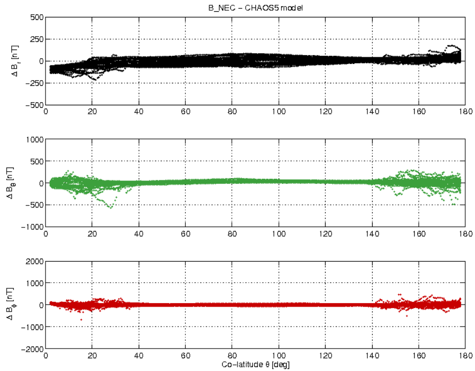
Figure 3-19: S/C B day 19.03 B_{NEC} - B_{Chaos} difference vs colatitude.
