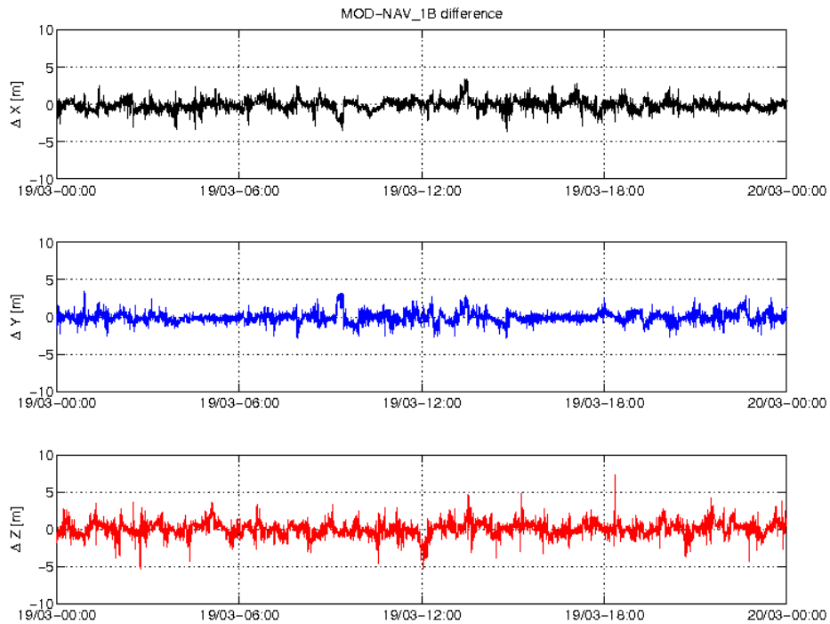
Figure 3-3: Difference MOD-GPSNAV, S/C A, 19.03. From top to bottom: X, Y and Z-axis
