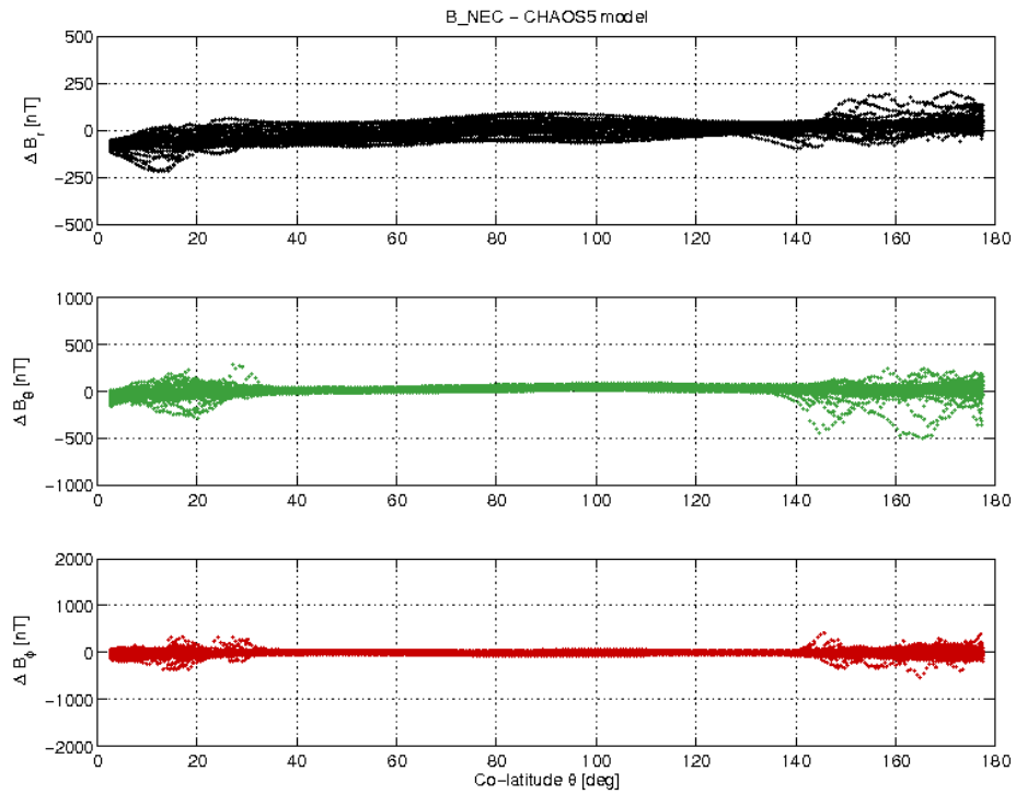
Figure 3-21: S/C C day 19.03 B_{NEC} - B_{Chaos} difference vs colatitude.
