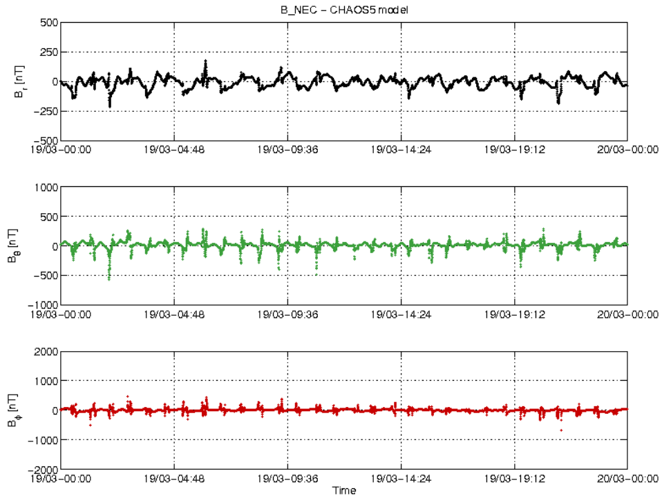
Figure 3-20: S/C B day 19.03 time series of B_{NEC} - B_{Chaos} residuals.
