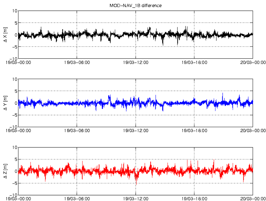
Figure 3-5: Difference MOD-GPSNAV, S/C C, 19.03. From top to bottom: X, Y and Z-axis
