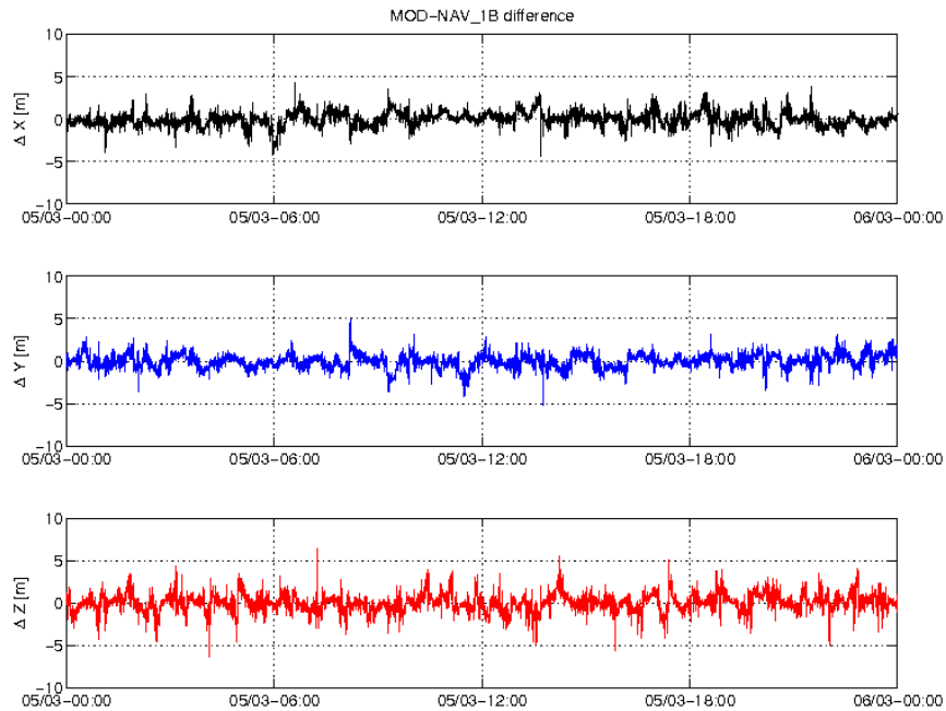
Figure 3-3: Difference MOD-GPSNAV, S/C A, 05/03. From top to bottom: X, Y and Z-axis
