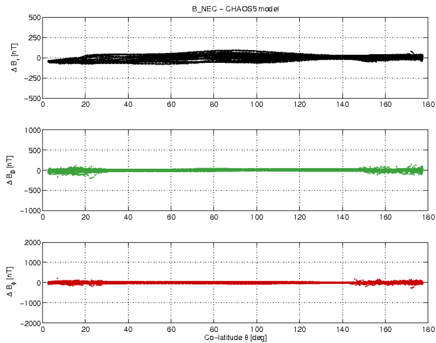
Figure 3-21: S/C C day 05/03 B_{NEC} - B_{Chaos} difference vs colatitude.
