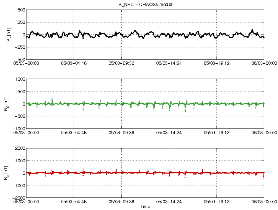
Figure 3-20: S/C B day 05/03 time series of B_{NEC} - B_{Chaos} residuals.
