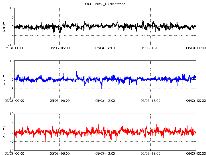
Figure 3-5: Difference MOD-GPSNAV, S/C C, 05/03. From top to bottom: X, Y and Z-axis
