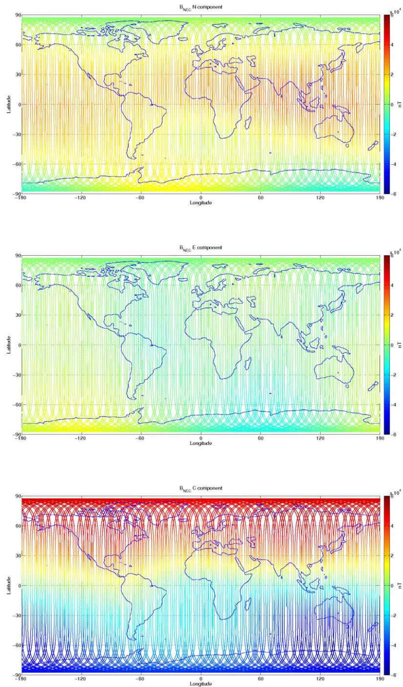
Figure 3-12: S/C C, world map plots of the geomagnetic field and components measured during monitoring period 05/03-11/03. From top to bottom: B NEC components (North, East, and Centre) of magnetic field from VFM measurement.
