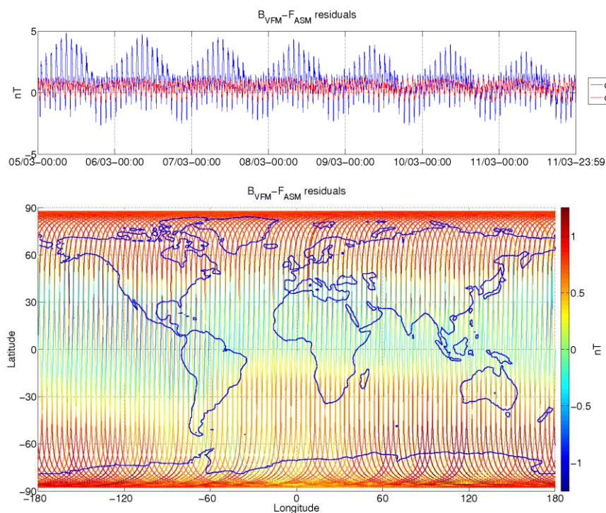
Figure 3-9: ASM-VFM residuals for S/C B, during monitoring period 05/03-11/03. In top figure are plotted: difference between |B_{VFM}| and F_{ASM} (without dB_{Sun} correction) (blue colour), and the residuals with dB_{Sun} corrections (red colour). In bottom figure residuals are presented on the world map.
