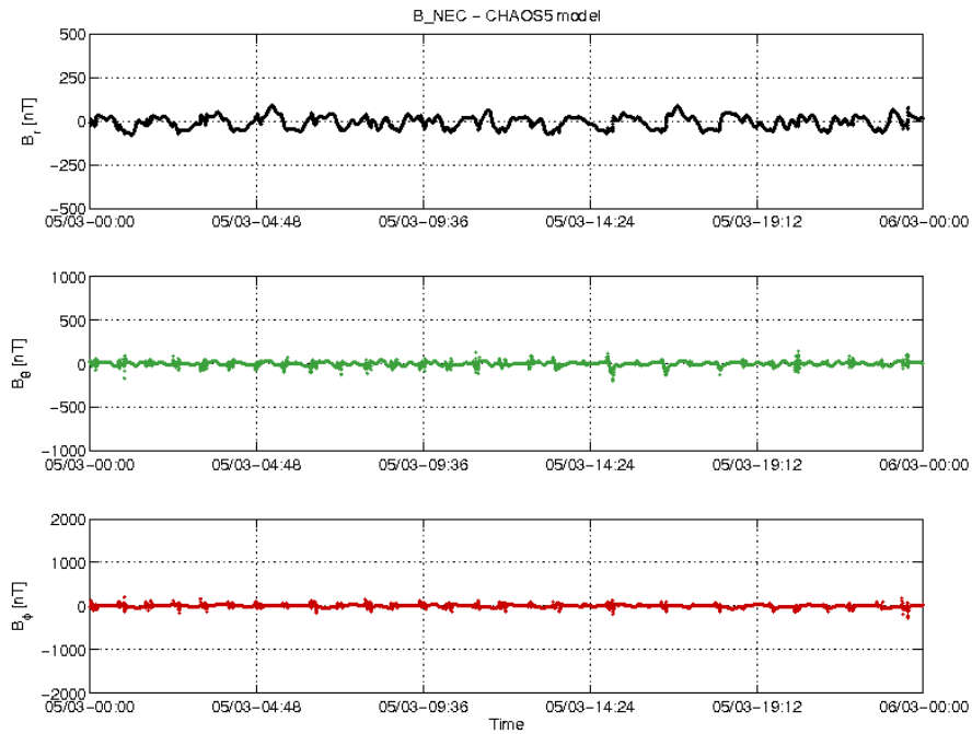
Figure 3-22: S/C C day 05/03 time series of B_{NEC} - B_{Chaos} residuals.
