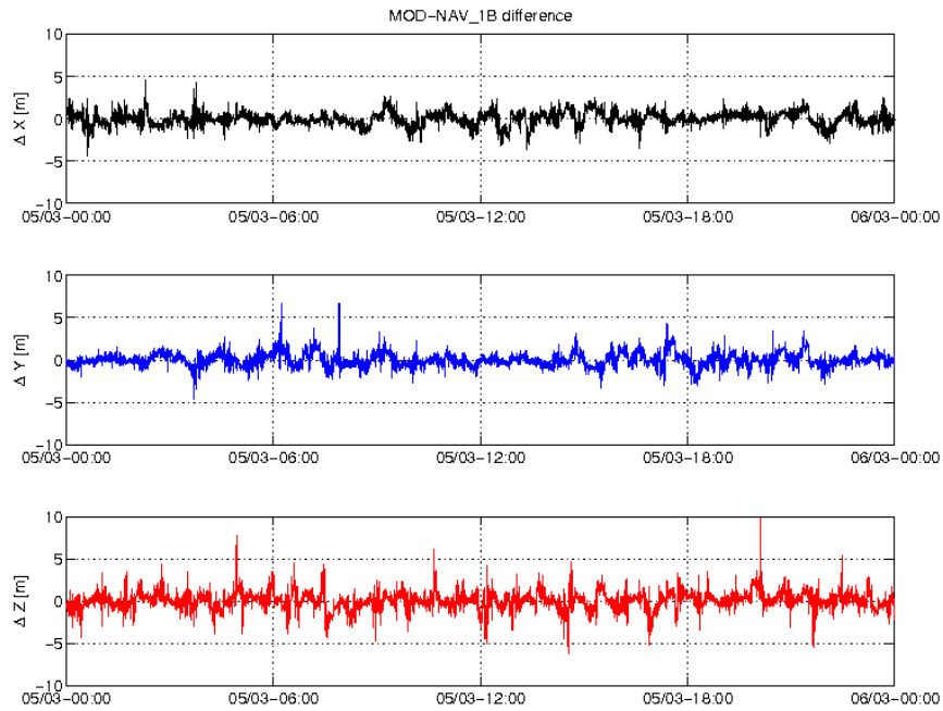
Figure 3-4: Difference MOD-GPSNAV, S/C B, 05/03. From top to bottom: X, Y and Z-axis
