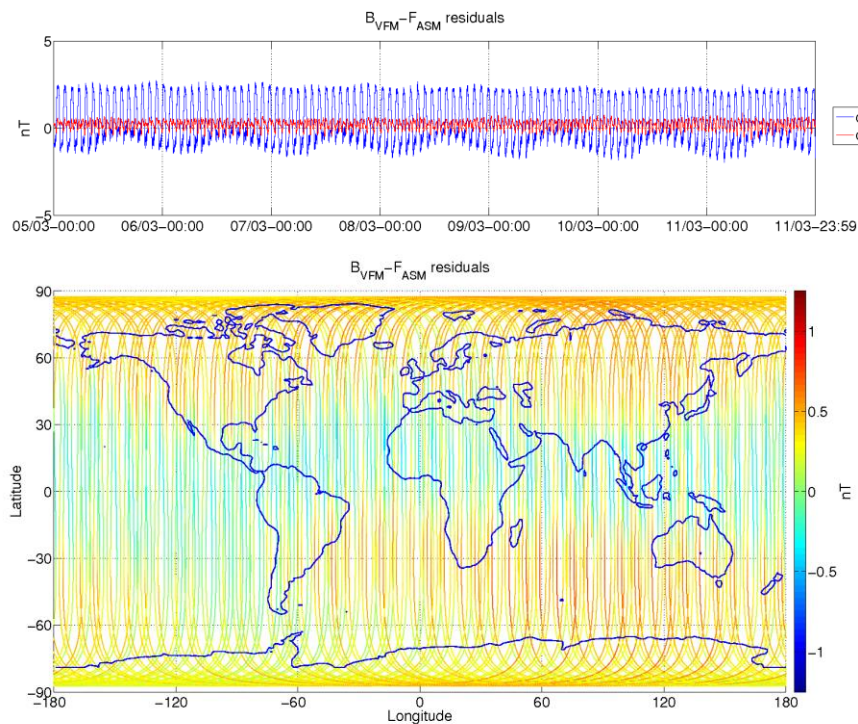
Figure 3-8: ASM-VFM residuals for S/C A, during monitoring period 05/03-11/03. In top figure are plotted: difference between |B_{VFM}| and F_{ASM} (without dB_{Sun} correction) (blue colour), and the residuals with dB_{Sun} corrections (red colour). In bottom figure residuals are presented on the world map.
