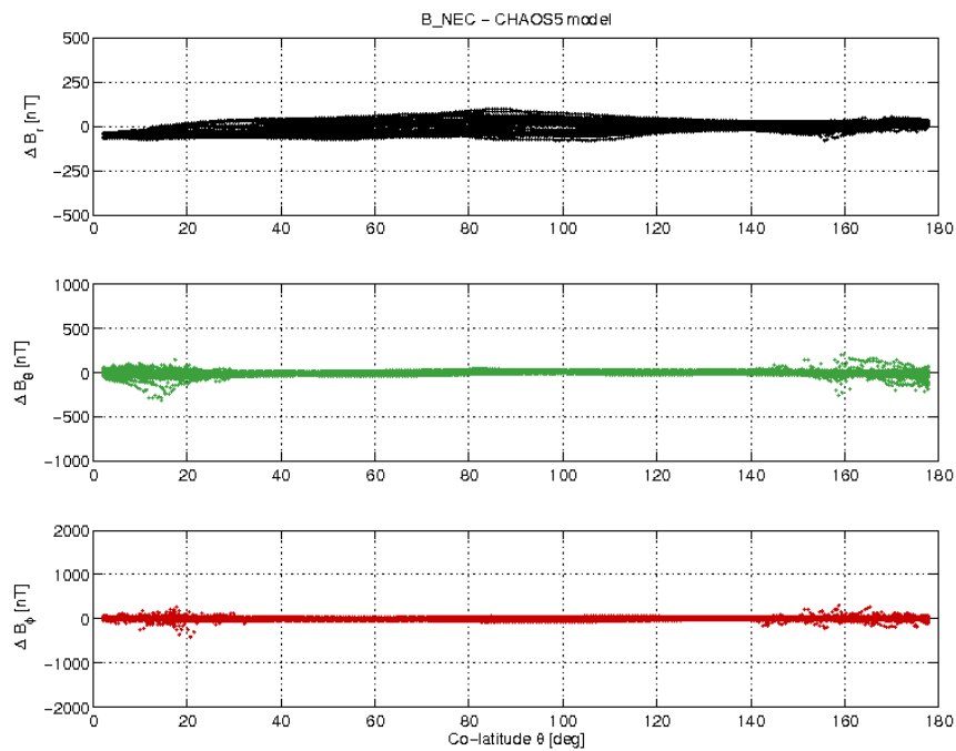
Figure 3-19: S/C B day 05/03 B_{NEC} - B_{Chaos} difference vs colatitude.
