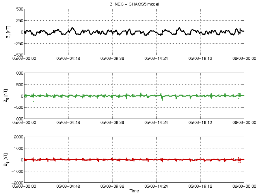
Figure 3-18: S/C A day 05/03: time series of B_{NEC} - B_{Chaos} residuals.
