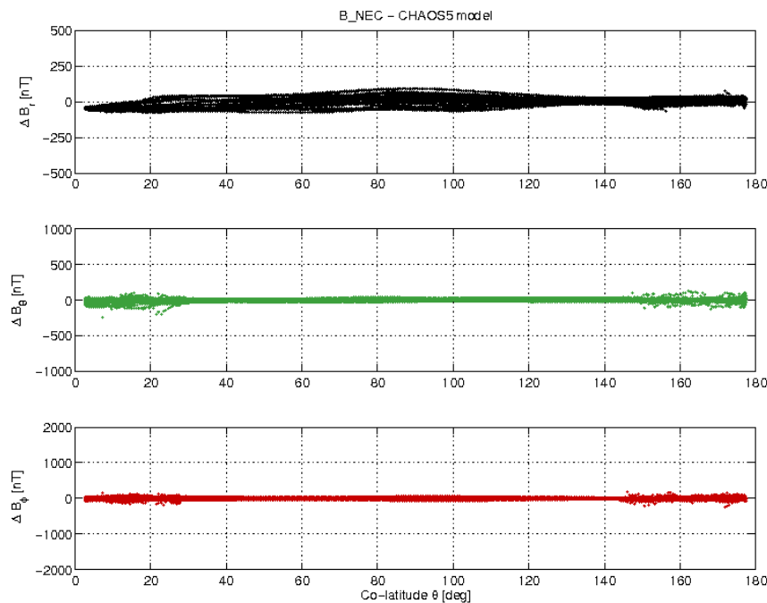
Figure 3-17: S/C A day 05/03 B_{NEC} - B_{Chaos} vs colatitude.
