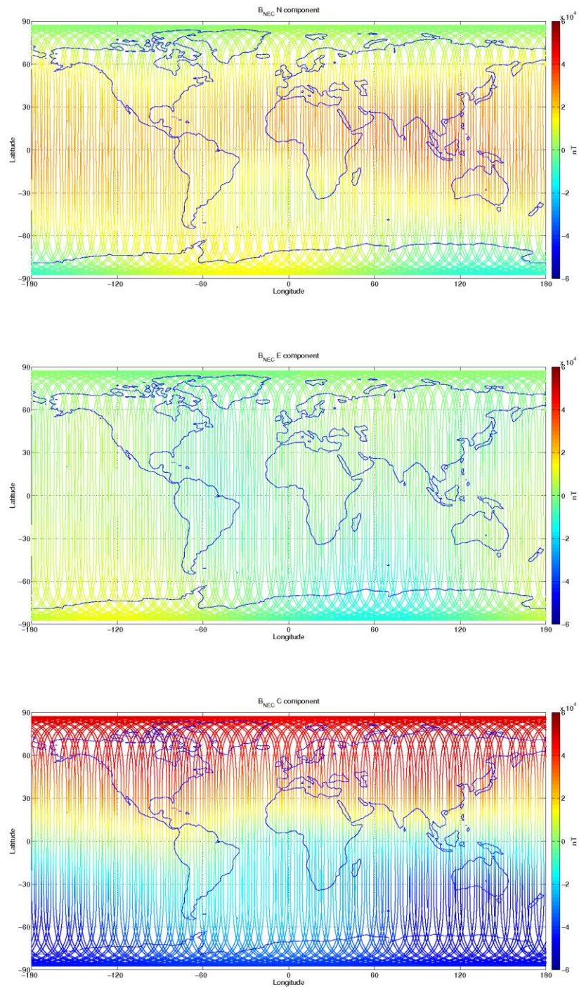
Figure 3-12: S/C C, world map plots of the geomagnetic field and components measured during monitoring period 26/02-04/03. From top to bottom: B NEC components (North, East, and Centre) of magnetic field from VFM measurement.
