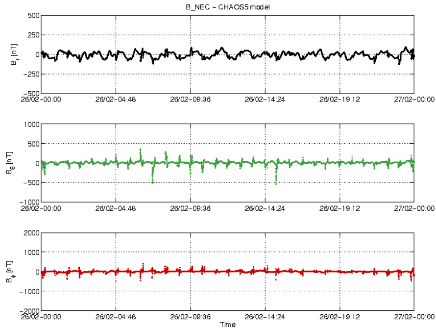
Figure 3-20: S/C B day 26/02 time series of B_{NEC} - B_{Chaos} residuals.
