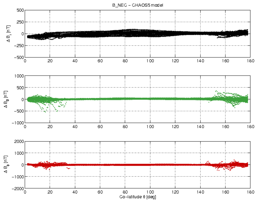
Figure 3-19: S/C B day 26/02 B_{NEC} - B_{Chaos} difference vs colatitude.
