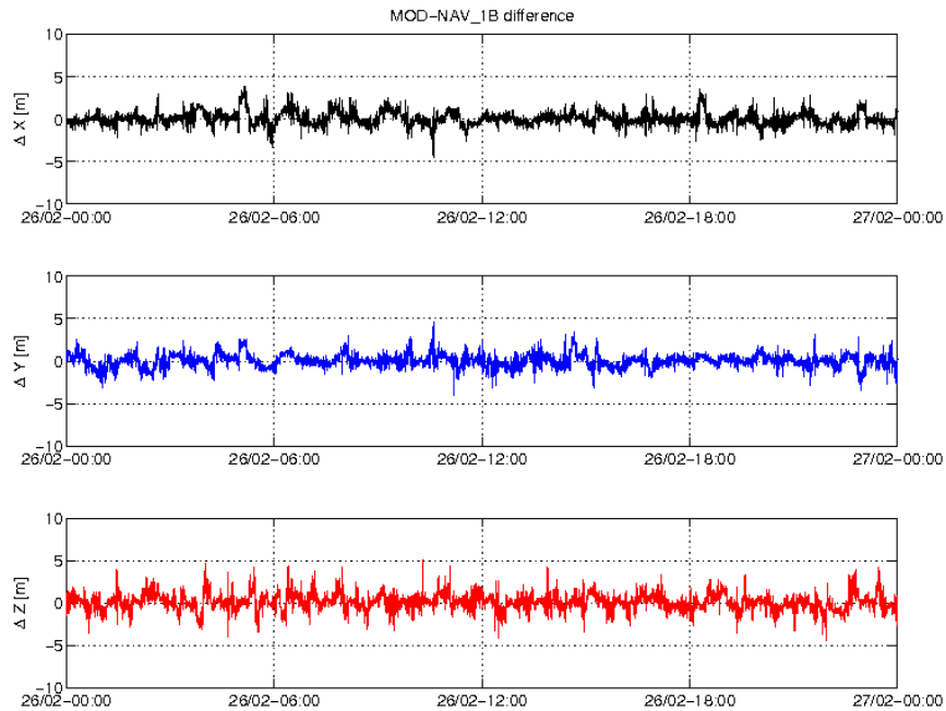
Figure 3-3: Difference MOD-GPSNAV, S/C A, 26/02. From top to bottom: X, Y and Z-axis
