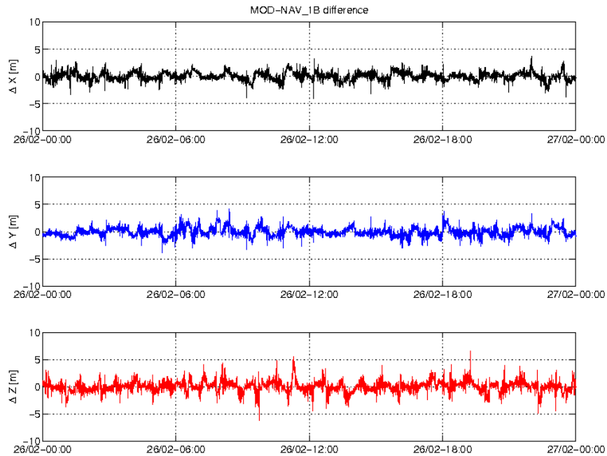
Figure 3-4: Difference MOD-GPSNAV, S/C B, 26/02. From top to bottom: X, Y and Z-axis
