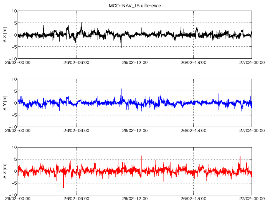
Figure 3-5: Difference MOD-GPSNAV, S/C C, 26/02. From top to bottom: X, Y and Z-axis
