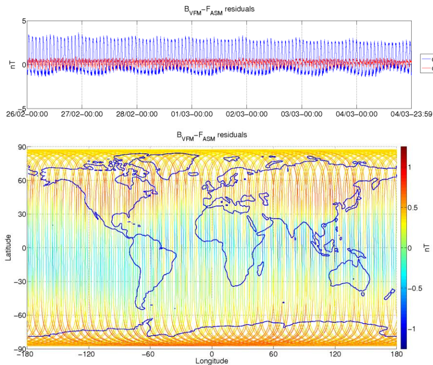
Figure 3-8: ASM-VFM residuals for S/C A, during monitoring period 26/02-04/03. In top figure are plotted: difference between |B_{VFM}| and F_{ASM} (without dB_{Sun} correction) (blue colour), and the residuals with dB_{Sun} corrections (red colour). In bottom figure residuals are presented on the world map.
