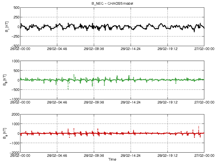
Figure 3-18: S/C A day 26/02: time series of B_{NEC} - B_{Chaos} residuals.
