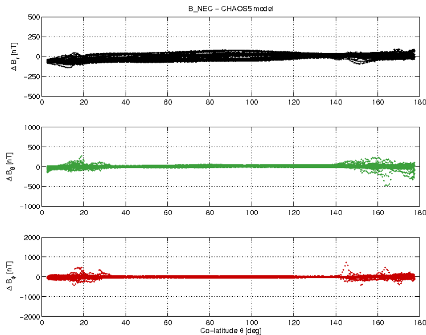
Figure 3-17: S/C A day 26/02 B NEC - B Chaos vs colatitude.
