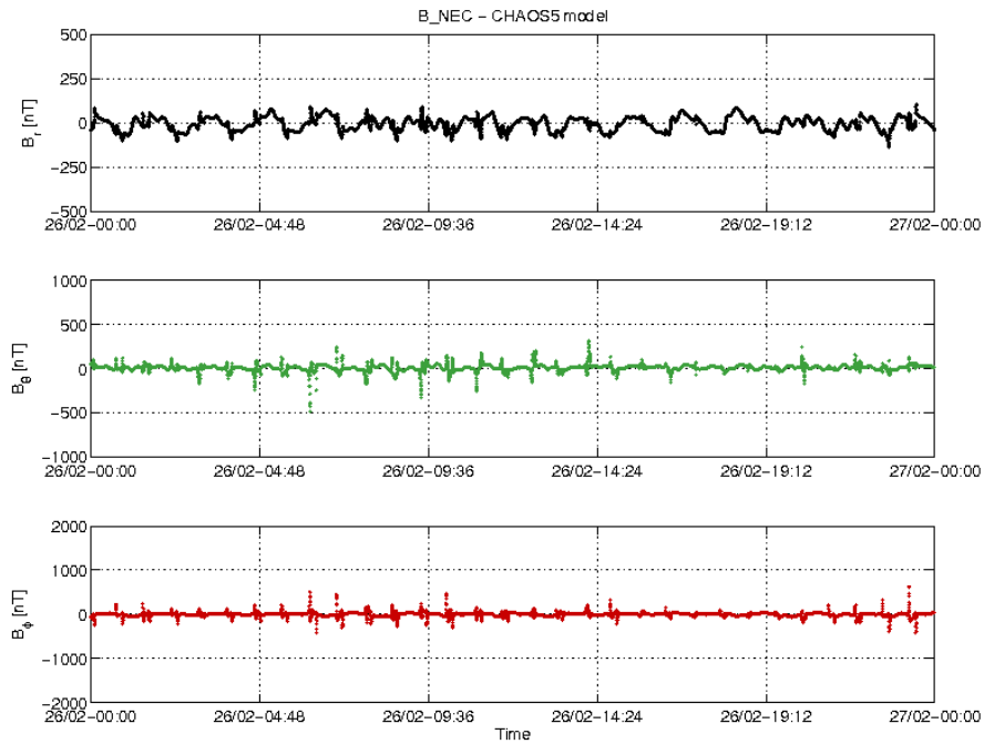
Figure 3-22: S/C C day 26/02 time series of B_{NEC} - B_{Chaos} residuals.
