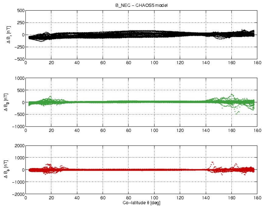
Figure 3-21: S/C C day 26/02 B_{NEC} - B_{Chaos} difference vs colatitude.
