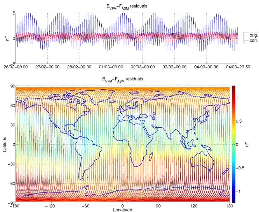
Figure 3-9: ASM-VFM residuals for S/C B, during monitoring period 26/02-04/03. In top figure are plotted: difference between |B_{VFM}| and F_{ASM} (without dB_{Sun} correction) (blue colour), and the residuals with dB_{Sun} corrections (red colour). In bottom figure residuals are presented on the world map.
