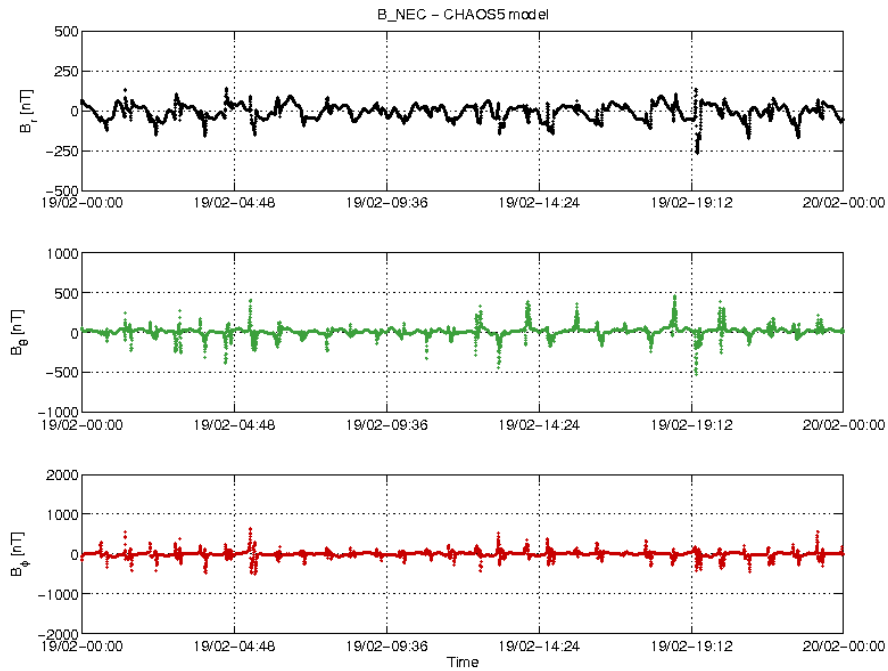
Figure 3-22: S/C C day 19/02 time series of B_{NEC} - B_{Chaos} residuals.
