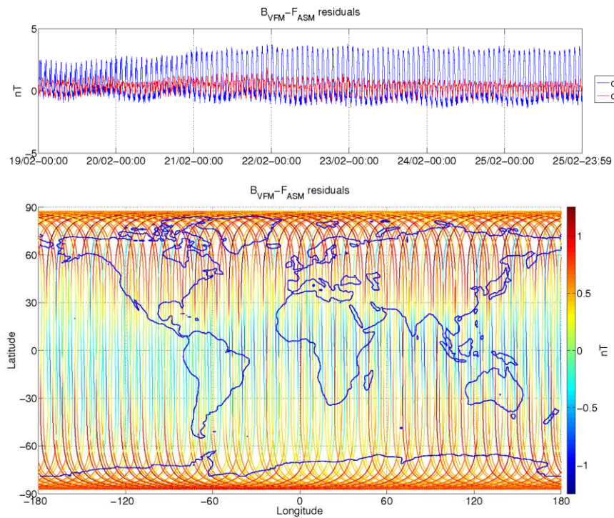
Figure 3-8: ASM-VFM residuals for S/C A, during monitoring period 19/02-25/02. In top figure are plotted: difference between |B VFM | and F ASM (without dB Sun correction) (blue colour), and the residuals with dB Sun corrections (red colour). In bottom figure residuals are presented on the world map.
