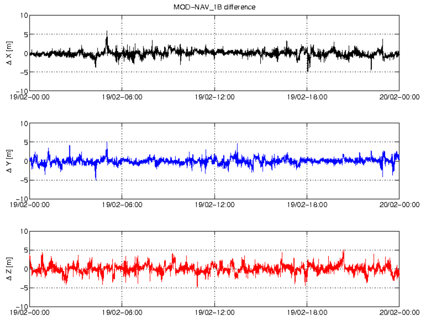
Figure 3-3: Difference MOD-GPSNAV, S/C A, 19/02. From top to bottom: X, Y and Z-axis
