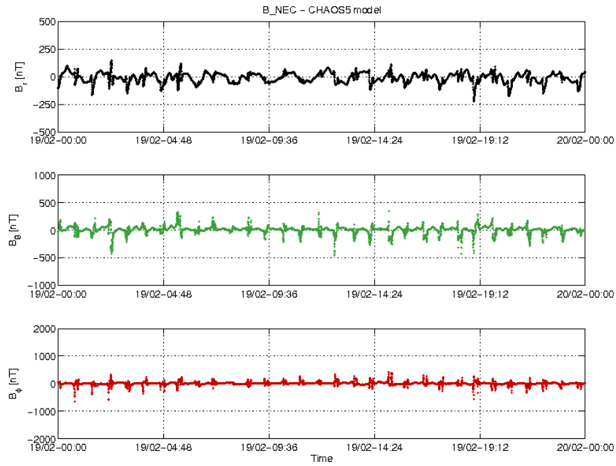
Figure 3-20: S/C B day 19/02 time series of B_{NEC} - B_{Chaos} residuals.
