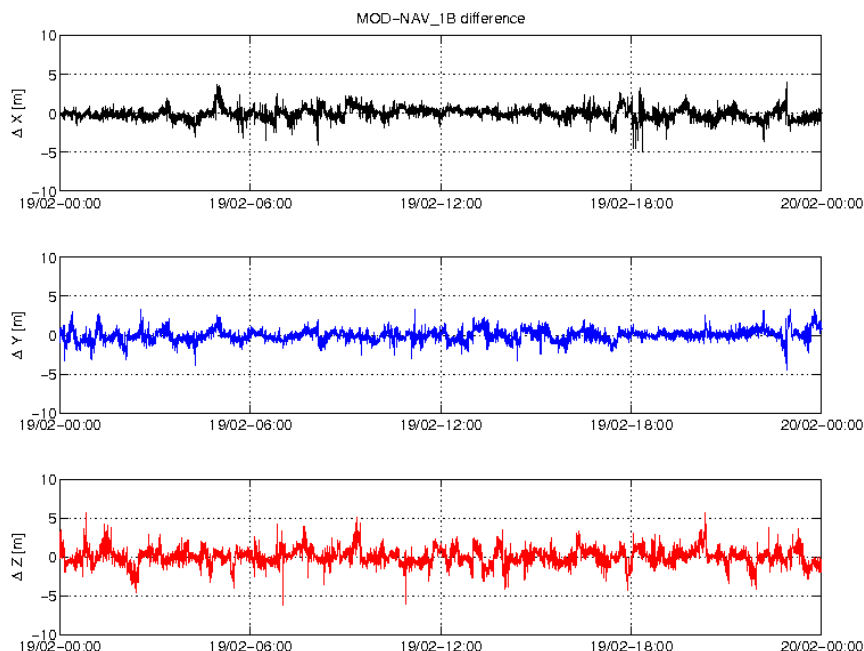
Figure 3-5: Difference MOD-GPSNAV, S/C C, 19/02. From top to bottom: X, Y and Z-axis
