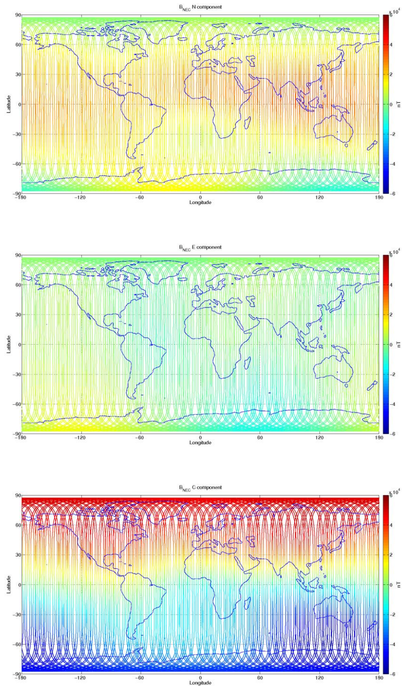
Figure 3-12: S/C C, world map plots of the geomagnetic field and components measured during monitoring period 19/02-25/02. From top to bottom: B_{NEC} components (North, East, and Centre) of magnetic field from VFM measurement.
