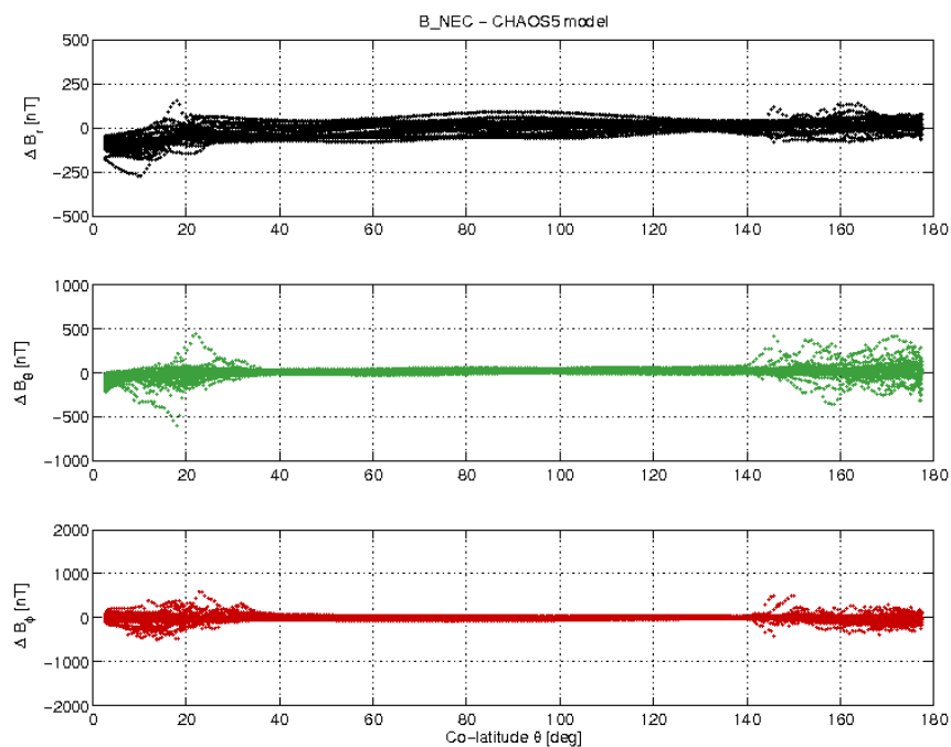
Figure 3-17: S/C A day 19/02 B_{NEC} - B_{Chaos} vs colatitude.
