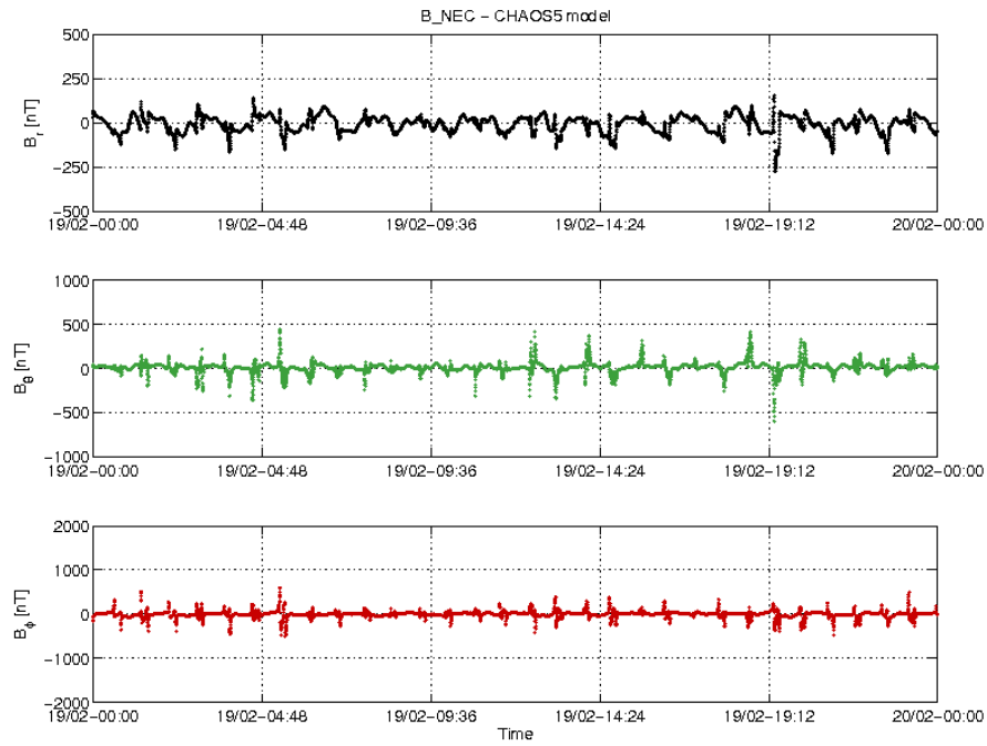
Figure 3-18: S/C A day 19/02: time series of B_{NEC} - B_{Chaos} residuals.
