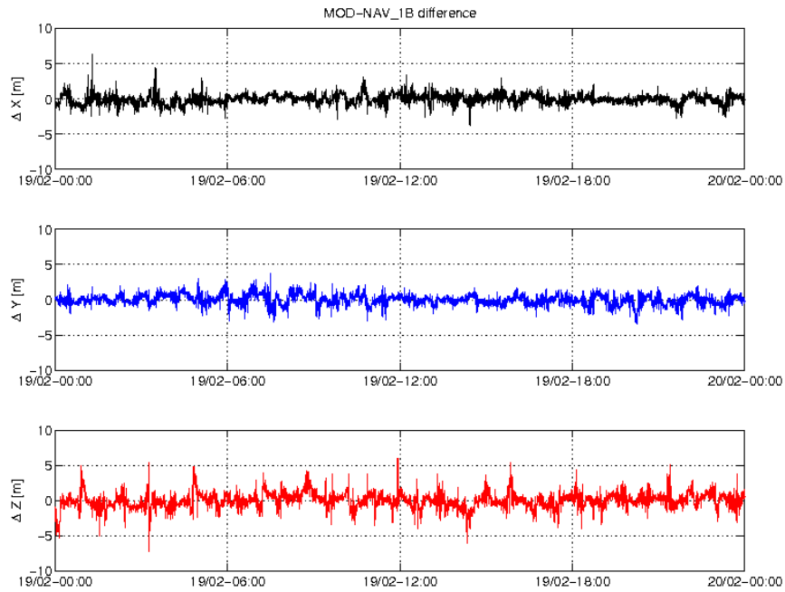
Figure 3-4: Difference MOD-GPSNAV, S/C B, 19/02. From top to bottom: X, Y and Z-axis
