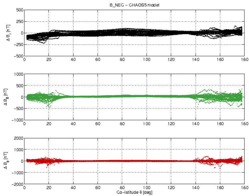
Figure 3-19: S/C B day 19/02 B_{NEC} - B_{Chaos} difference vs colatitude.
