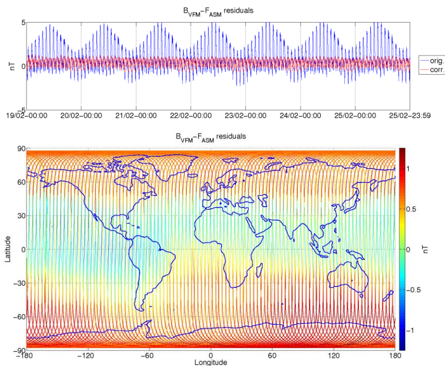
Figure 3-9: ASM-VFM residuals for S/C B, during monitoring period 19/02-25/02. In top figure are plotted: difference between |B_{VFM}| and F_{ASM} (without dB_{Sun} correction) (blue colour), and the residuals with dB_{Sun} corrections (red colour). In bottom figure residuals are presented on the world map.
