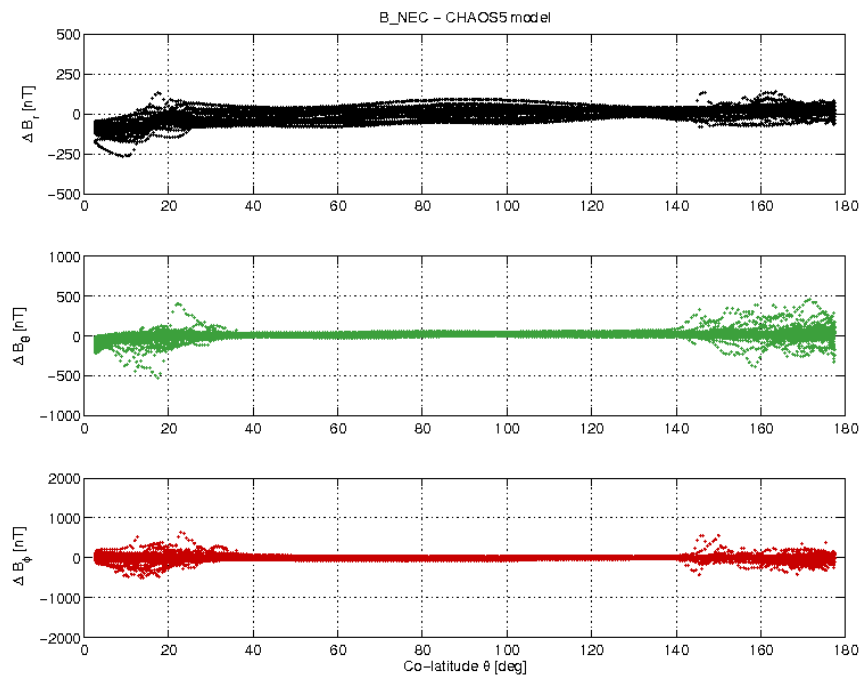
Figure 3-21: S/C C day 19/02 B_{NEC} - B_{Chaos} difference vs colatitude.
