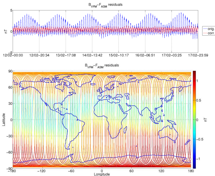
Figure 3-9: ASM-VFM residuals for S/C B, during monitoring period 12/02-18/02. In top figure are plotted: difference between |B\_VFM| and F\_ASM (without dB\_Sun correction) (blue colour), and the residuals with dB\_Sun corrections (red colour). In bottom figure residuals are presented on the world map.
