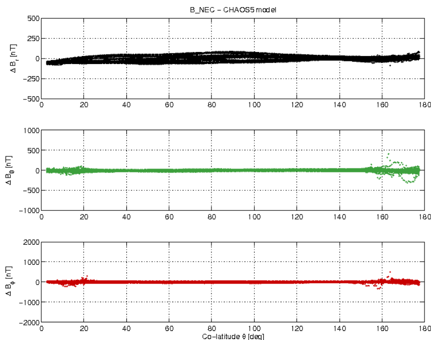
Figure 3-17: S/C A day 12/02 B NEC - B Chaos vs colatitude.
