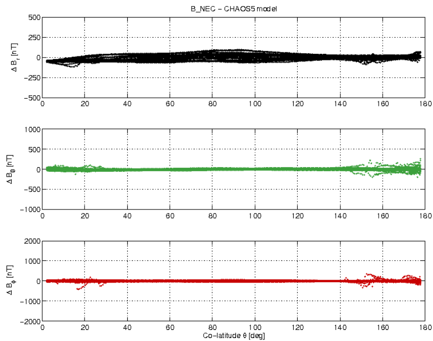
Figure 3-19: S/C B day 12/02 B_{NEC} - B_{Chaos} difference vs colatitude.
