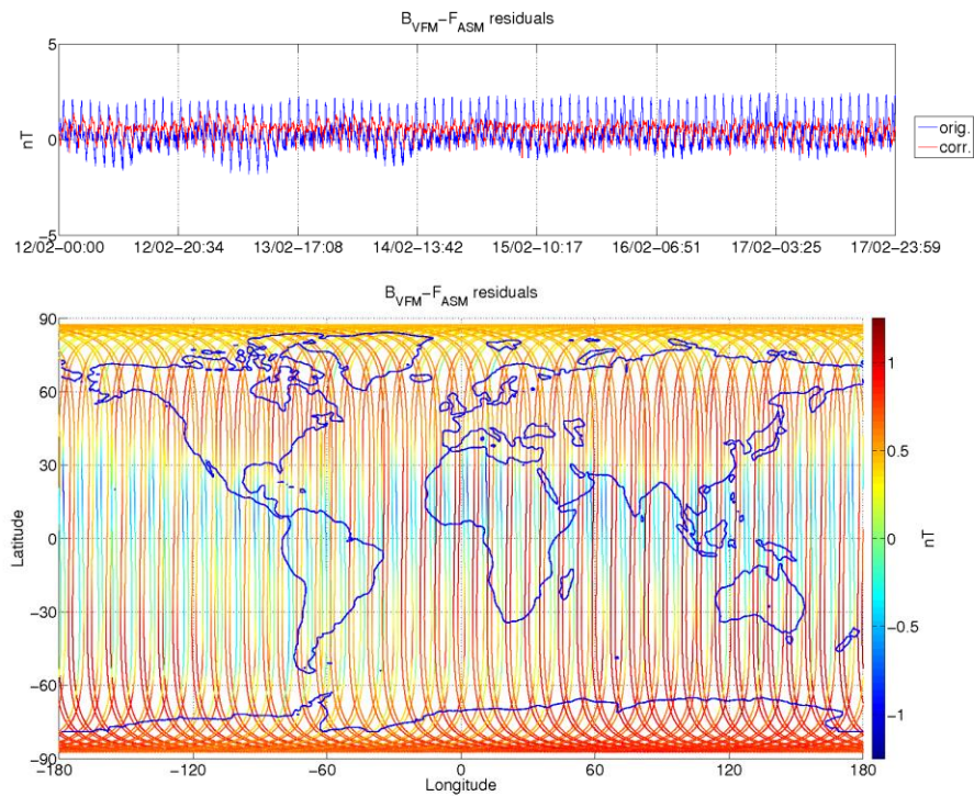
Figure 3-8: ASM-VFM residuals for S/C A, during monitoring period 12/02-18/02. In top figure are plotted: difference between |B_VFM| and F_ASM (without dB_Sun correction) (blue colour), and the residuals with dB_Sun corrections (red colour). In bottom figure residuals are presented on the world map.
