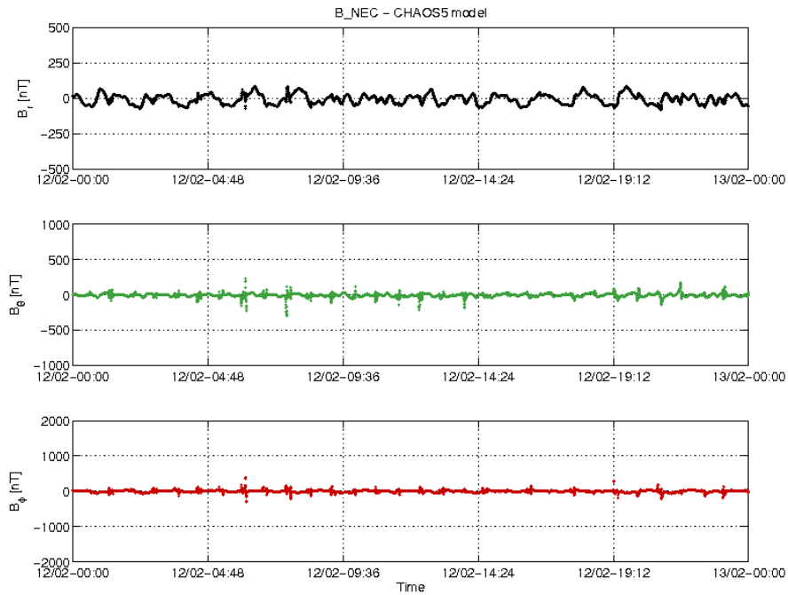
Figure 3-22: S/C C day 12/02 time series of B_{NEC} - B_{Chaos} residuals.
