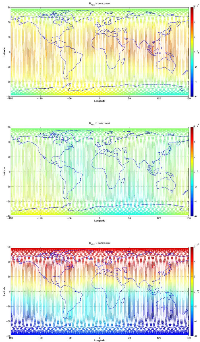
Figure 3-12: S/C C, world map plots of the geomagnetic field and components measured during monitoring period 12/02-18/02. From top to bottom: B_{NEC} components (North, East, and Centre) of magnetic field from VFM measurement.
