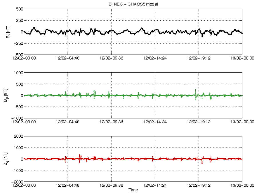
Figure 3-20: S/C B day 12/02 time series of B_{NEC} - B_{Chaos} residuals.
