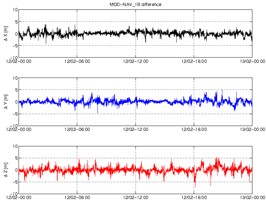
Figure 3-4: Difference MOD-GPSNAV, S/C B, 12/02. From top to bottom: X, Y and Z-axis
