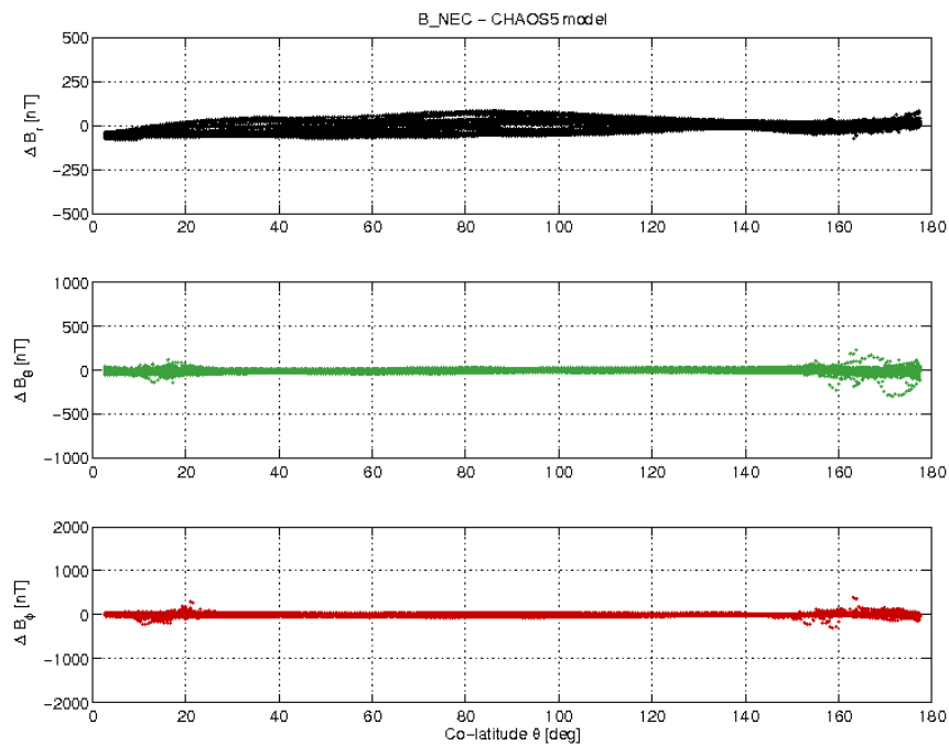
Figure 3-21: S/C C day 12/02 B_{NEC} - B_{Chaos} difference vs colatitude.
