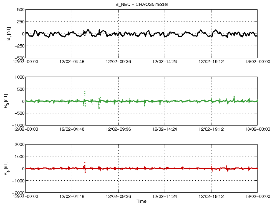
Figure 3-18: S/C A day 12/02: time series of B_{NEC} - B_{Chaos} residuals.
