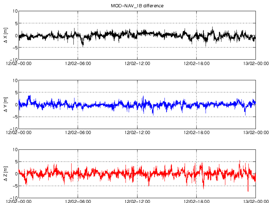
Figure 3-5: Difference MOD-GPSNAV, S/C C, 12/02. From top to bottom: X, Y and Z-axis
