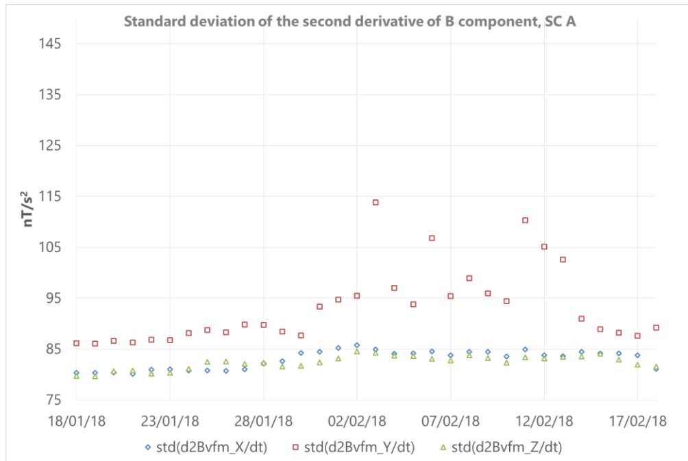
Figure 3-23: Standard deviation of the second derivative of B component
