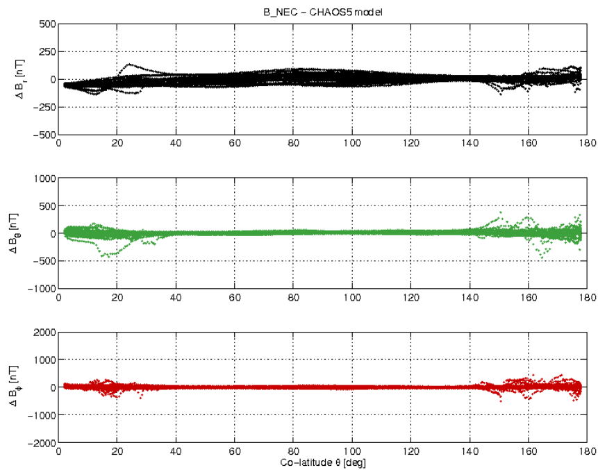
Figure 3-19: S/C B day 05/02 B_{NEC} - B_{Chaos} difference vs colatitude.
