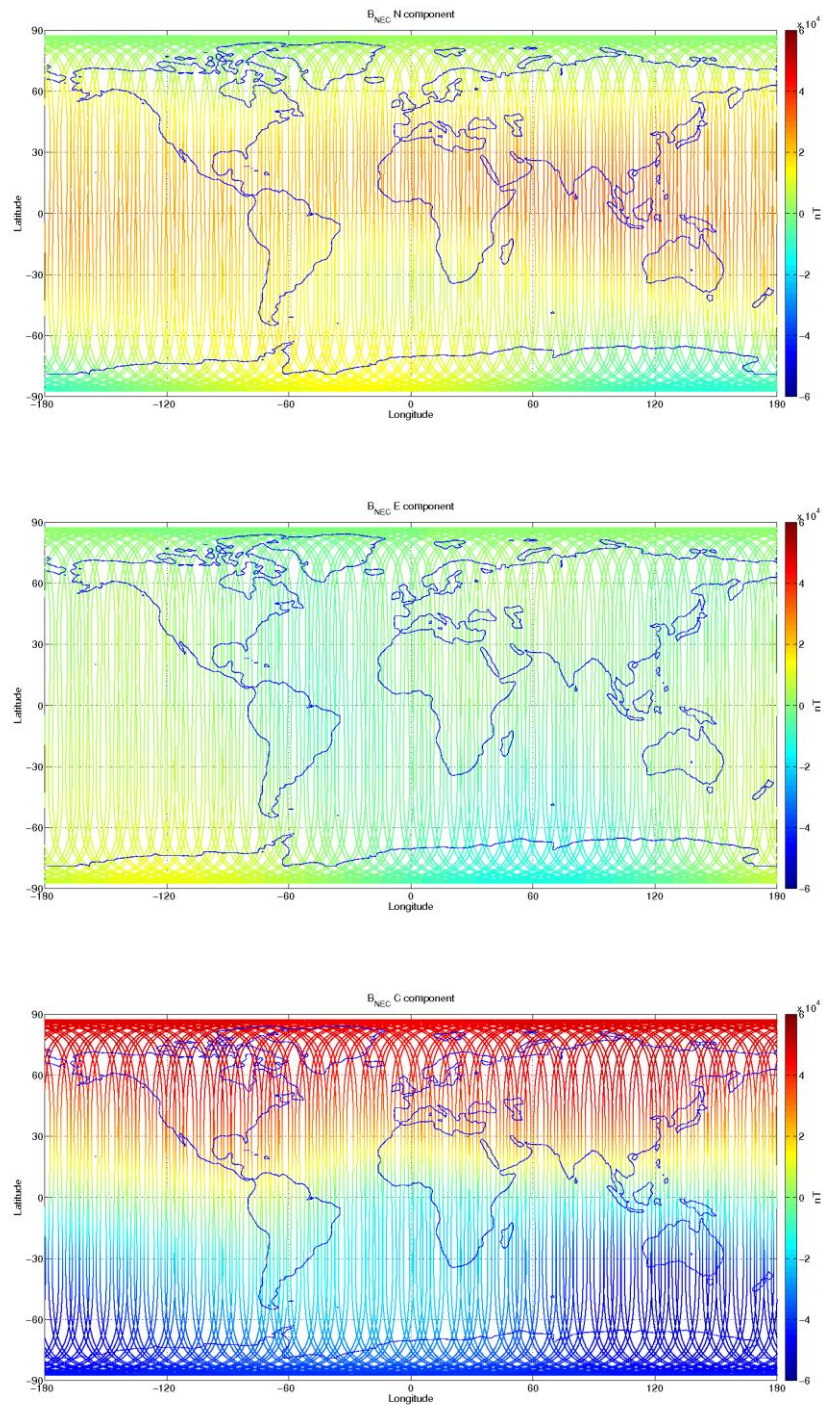
Figure 3-12: S/C C, world map plots of the geomagnetic field and components measured during monitoring period 05/02-11/02. From top to bottom: B_{NEC} components (North, East, and Centre) of magnetic field from VFM measurement.
