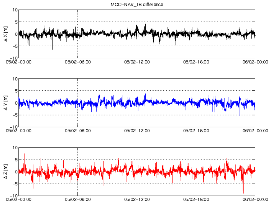
Figure 3-4: Difference MOD-GPSNAV, S/C B, 05/02. From top to bottom: X, Y and Z-axis
