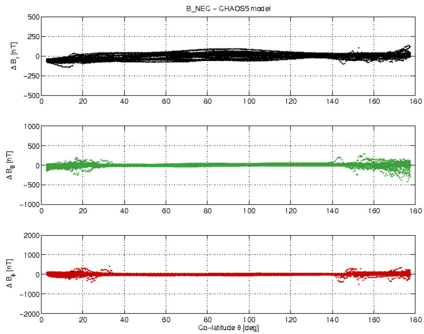
Figure 3-21: S/C C day 05/02 B_{NEC} - B_{Chaos} difference vs colatitude.
