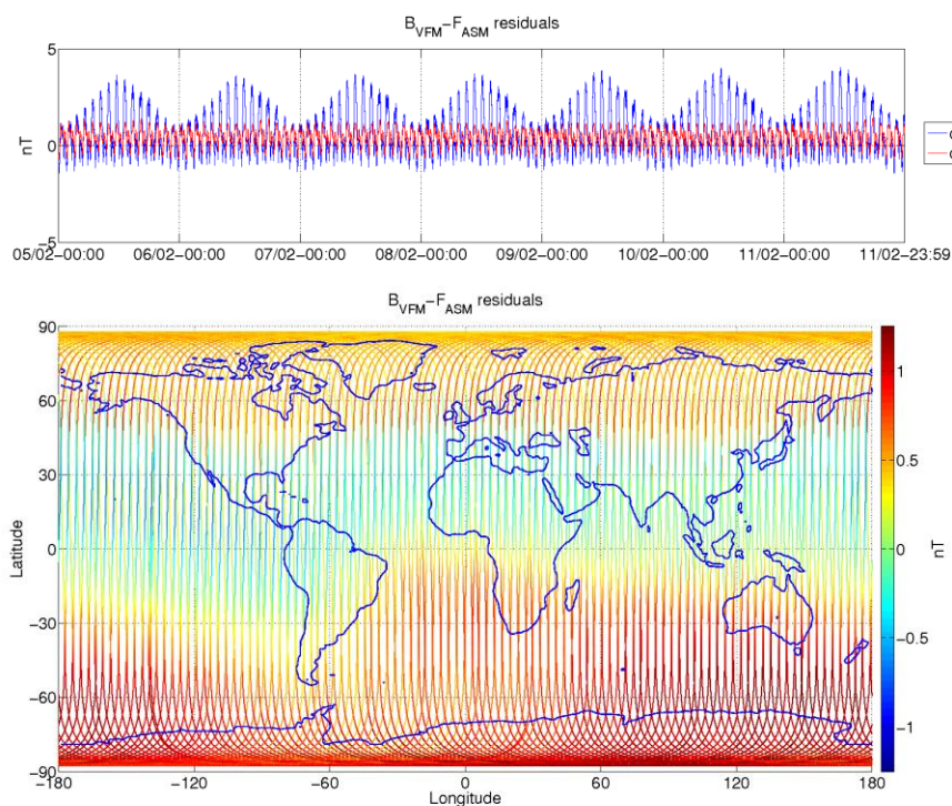
Figure 3-9: ASM-VFM residuals for S/C B, during monitoring period 05/02-11/02. In top figure are plotted: difference between |B\_VFM| and F\_ASM (without dB\_Sun correction) (blue colour), and the residuals with dB\_Sun corrections (red colour). In bottom figure residuals are presented on the world map.
