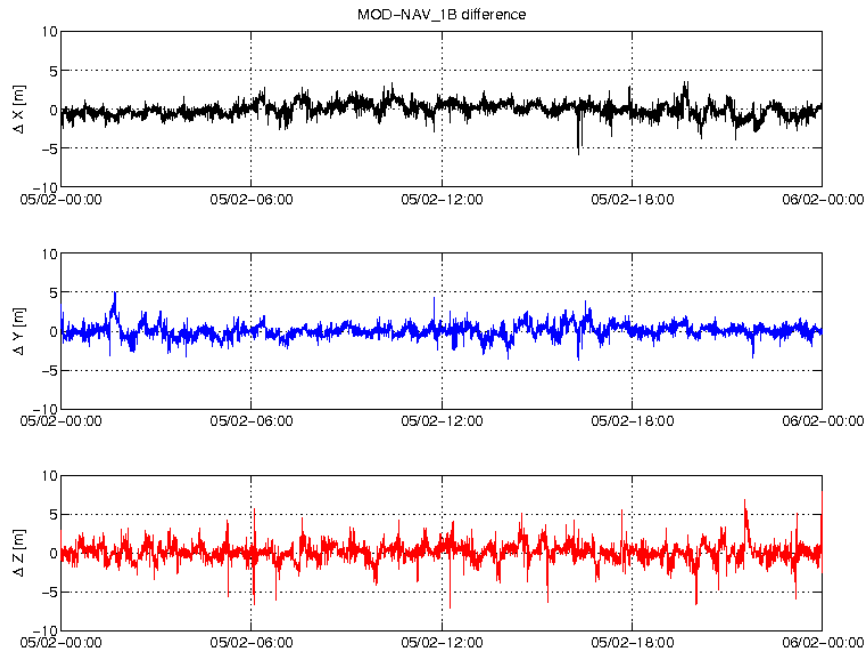
Figure 3-3: Difference MOD-GPSNAV, S/C A, 05/02. From top to bottom: X, Y and Z-axis
