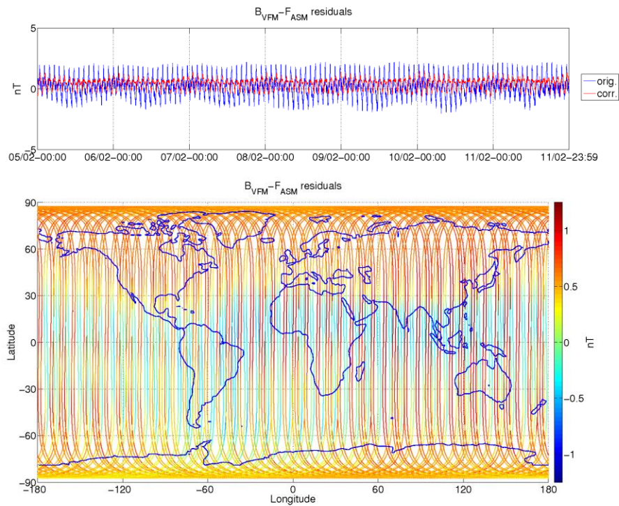
Figure 3-8: ASM-VFM residuals for S/C A, during monitoring period 05/02-11/02. In top figure are plotted: difference between |B VFM | and F ASM (without dB Sun correction) (blue colour), and the residuals with dB Sun corrections (red colour). In bottom figure residuals are presented on the world map.
