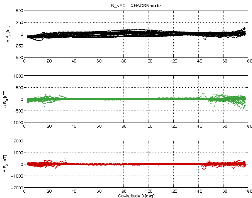
Figure 3-17: S/C A day 05/02 B_{NEC} - B_{Chaos} vs colatitude.
