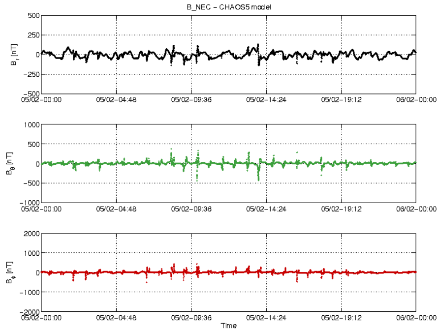
Figure 3-20: S/C B day 05/02 time series of B_{NEC} - B_{Chaos} residuals.
