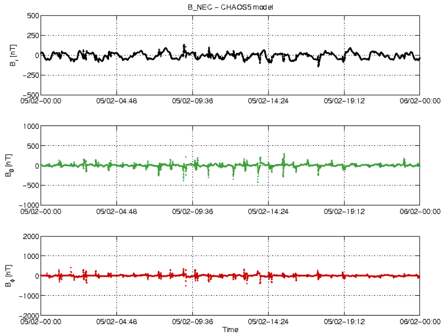
Figure 3-22: S/C C day 05/02 time series of B_{NEC} - B_{Chaos} residuals.
