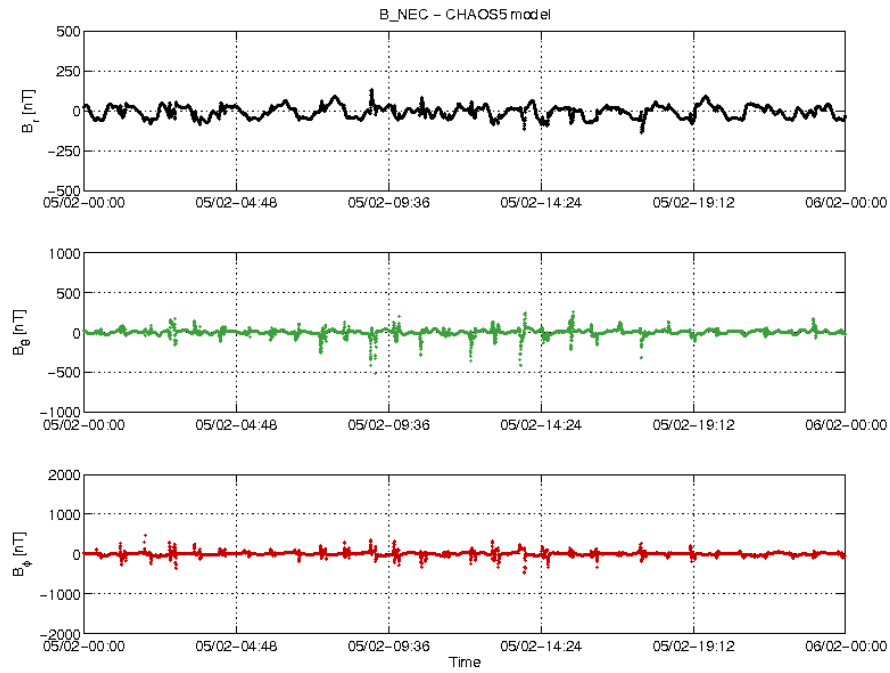
Figure 3-18: S/C A day 05/02: time series of B_{NEC} - B_{Chaos} residuals.
