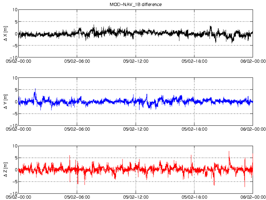
Figure 3-5: Difference MOD-GPSNAV, S/C C, 05/02. From top to bottom: X, Y and Z-axis
