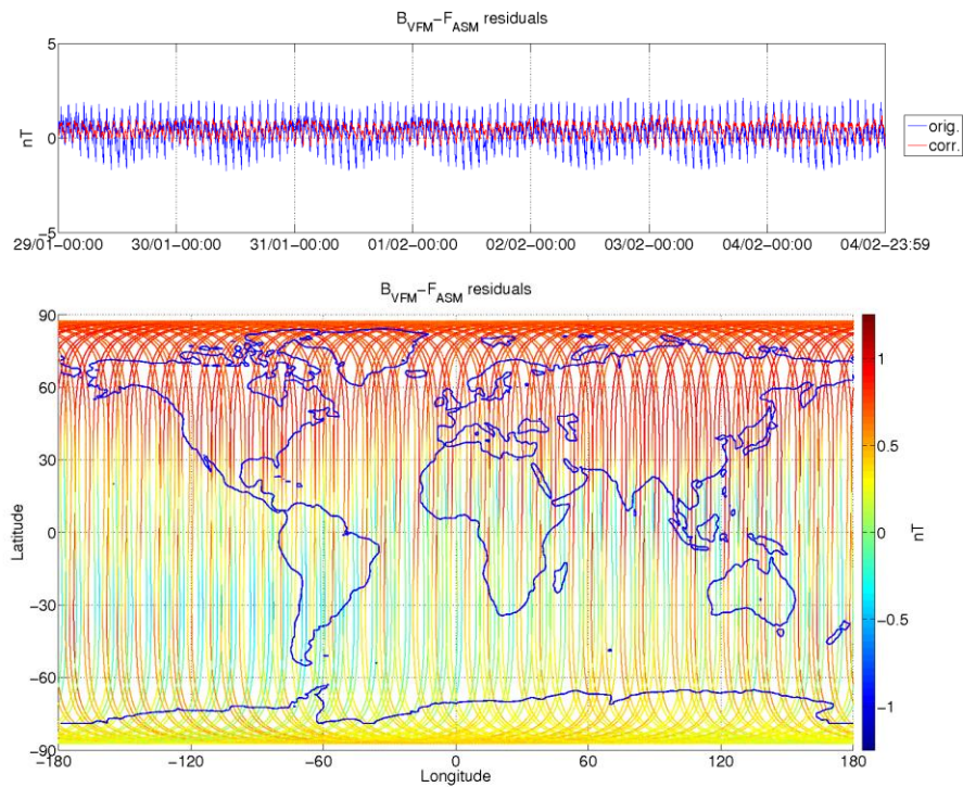
Figure 3-8: ASM-VFM residuals for S/C A, during monitoring period 29/01-04/02. In top figure are plotted: difference between |B VFM | and F ASM (without dB Sun correction) (blue colour), and the residuals with dB Sun corrections (red colour). In bottom figure residuals are presented on the world map.
