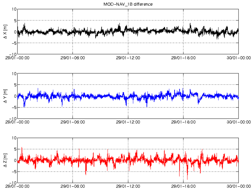
Figure 3-5: Difference MOD-GPSNAV, S/C C, 29/01. From top to bottom: X, Y and Z-axis
