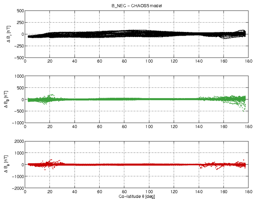
Figure 3-17: S/C A day 29/01 B_{NEC} - B_{Chaos} vs colatitude.
