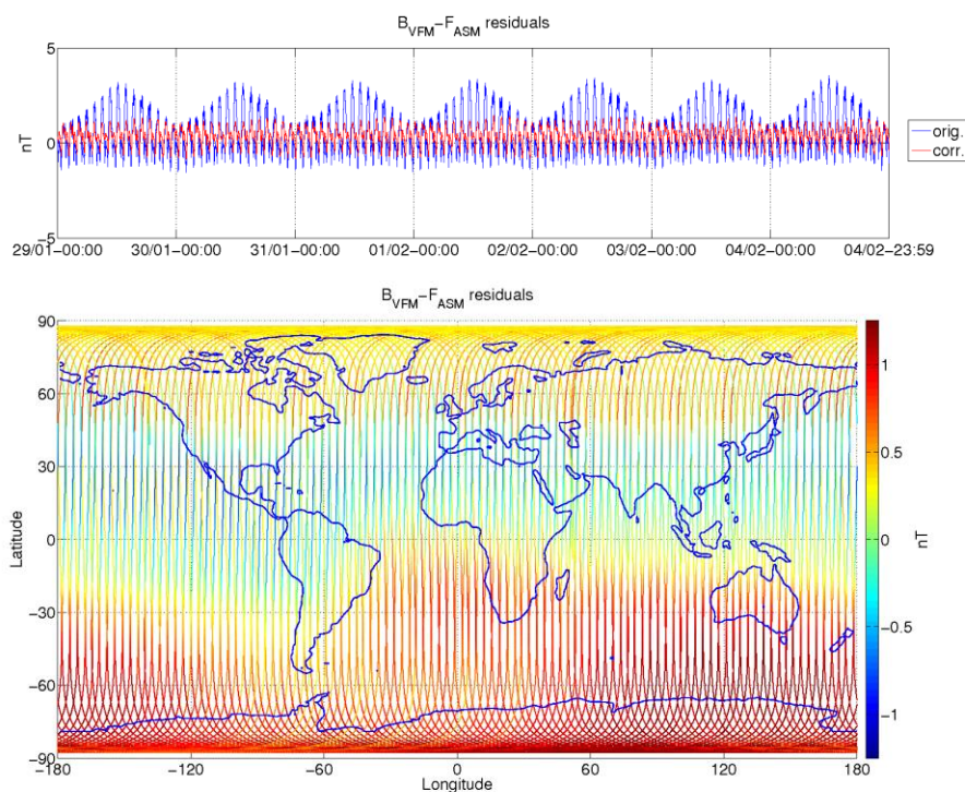
Figure 3-9: ASM-VFM residuals for S/C B, during monitoring period 29/01-04/02. In top figure are plotted: difference between |B_{VFM}| and F_{ASM} (without dB_{Sun} correction) (blue colour), and the residuals with dB_{Sun} corrections (red colour). In bottom figure residuals are presented on the world map.
