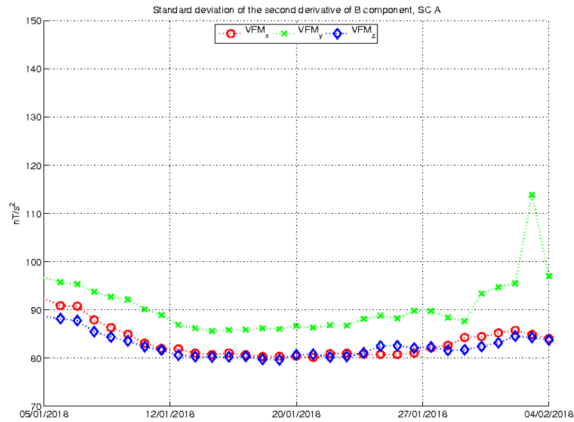
Figure 3-23: Standard deviation of the second derivative of B component
