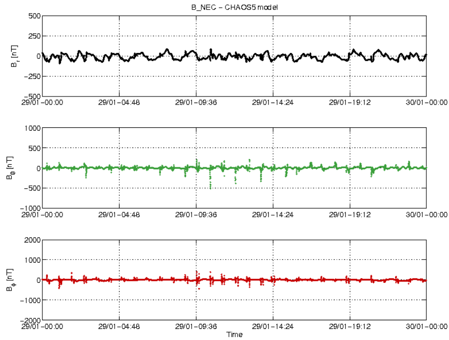
Figure 3-18: S/C A day 29/01: time series of B_{NEC} - B_{Chaos} residuals.
