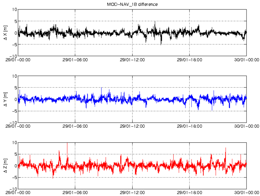
Figure 3-4: Difference MOD-GPSNAV, S/C B, 29/01. From top to bottom: X, Y and Z-axis
