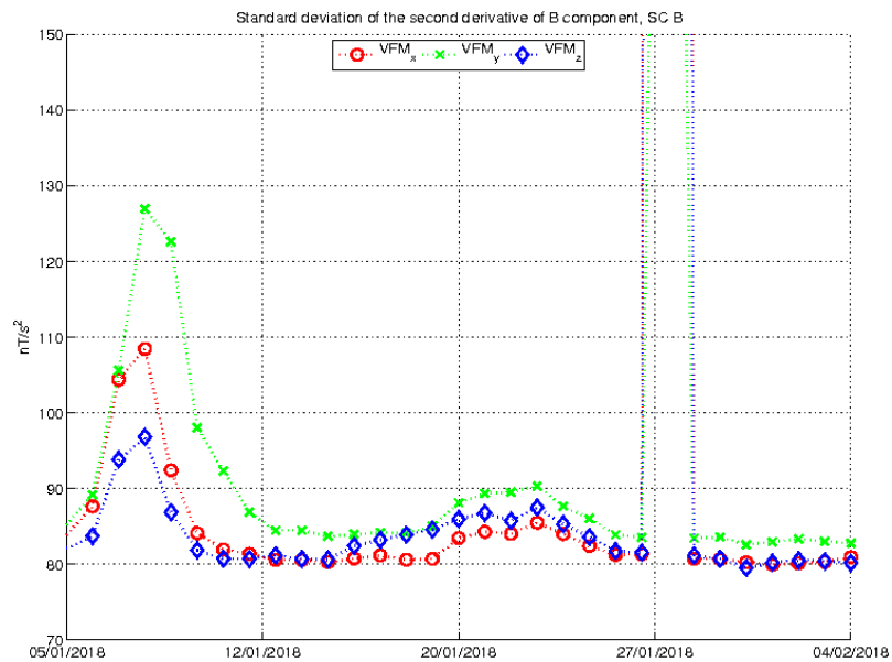
Figure 3-24: Standard deviation of the second derivative of B component
