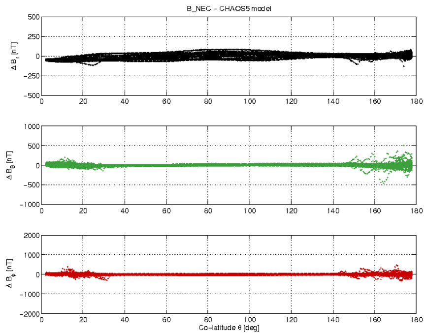
Figure 3-19: S/C B day 29/01 B_{NEC} - B_{Chaos} difference vs colatitude.
