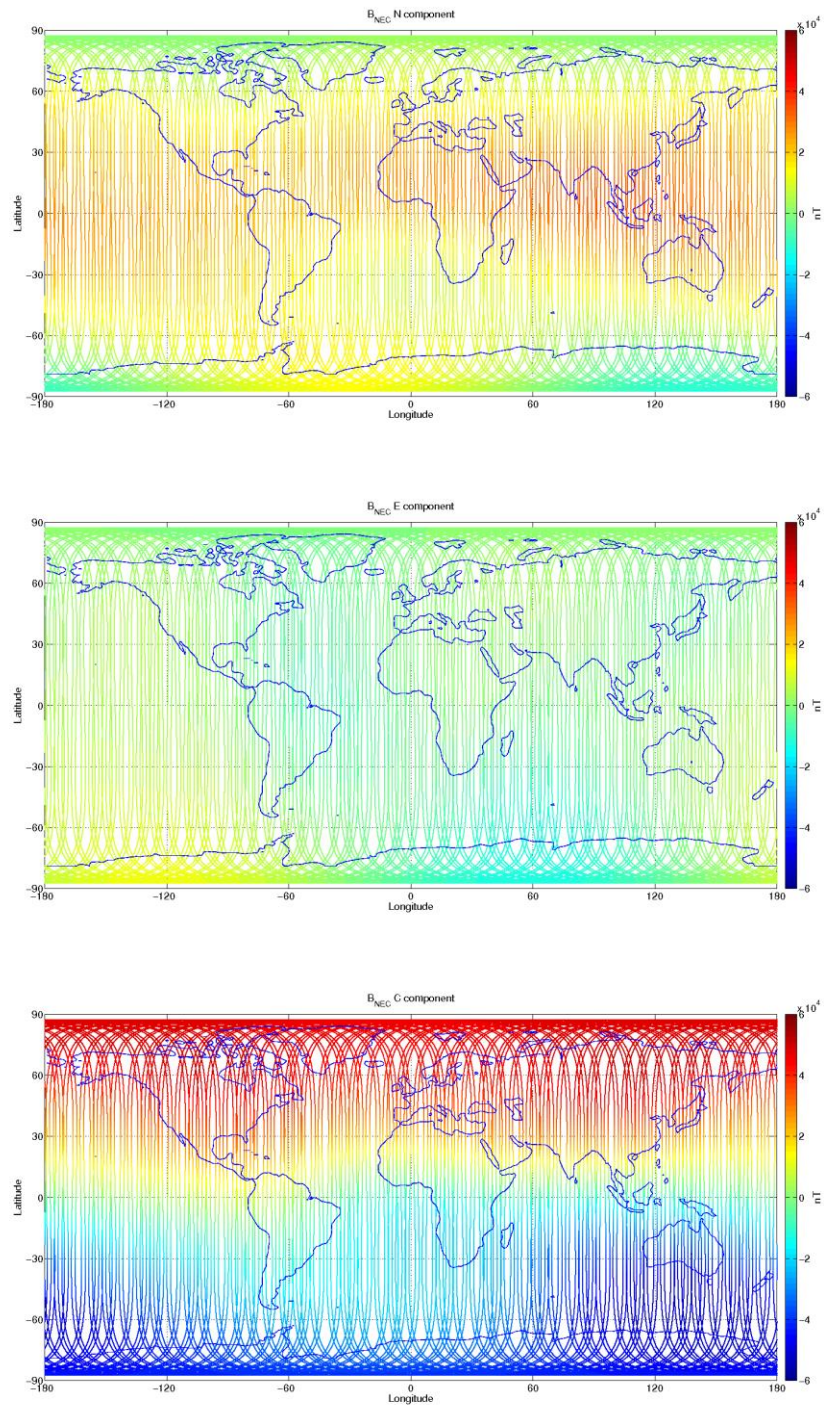
Figure 3-12: S/C C, world map plots of the geomagnetic field and components measured during monitoring period 29/01-04/02. From top to bottom: B NEC components (North, East, and Centre) of magnetic field from VFM measurement.
