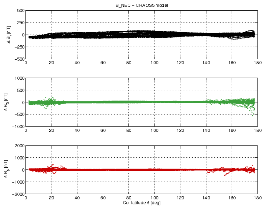
Figure 3-21: S/C C day 29/01 B_{NEC} - B_{Chaos} difference vs colatitude.
