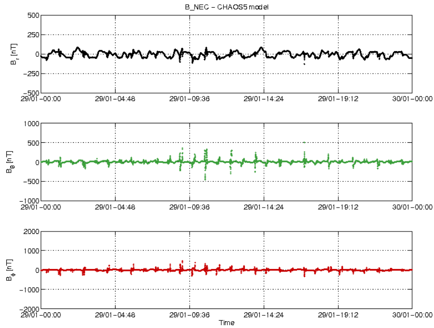
Figure 3-20: S/C B day 29/01 time series of B_{NEC} - B_{Chaos} residuals.
