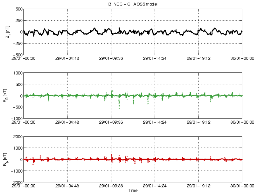
Figure 3-22: S/C C day 29/01 time series of B_{NEC} - B_{Chaos} residuals.
