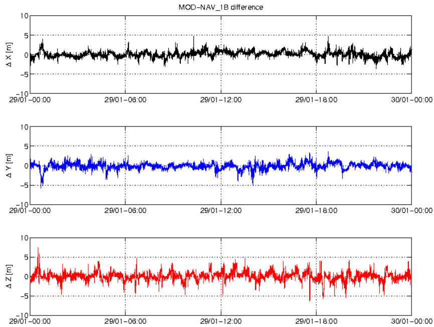
Figure 3-3: Difference MOD-GPSNAV, S/C A, 29/01. From top to bottom: X, Y and Z-axis
