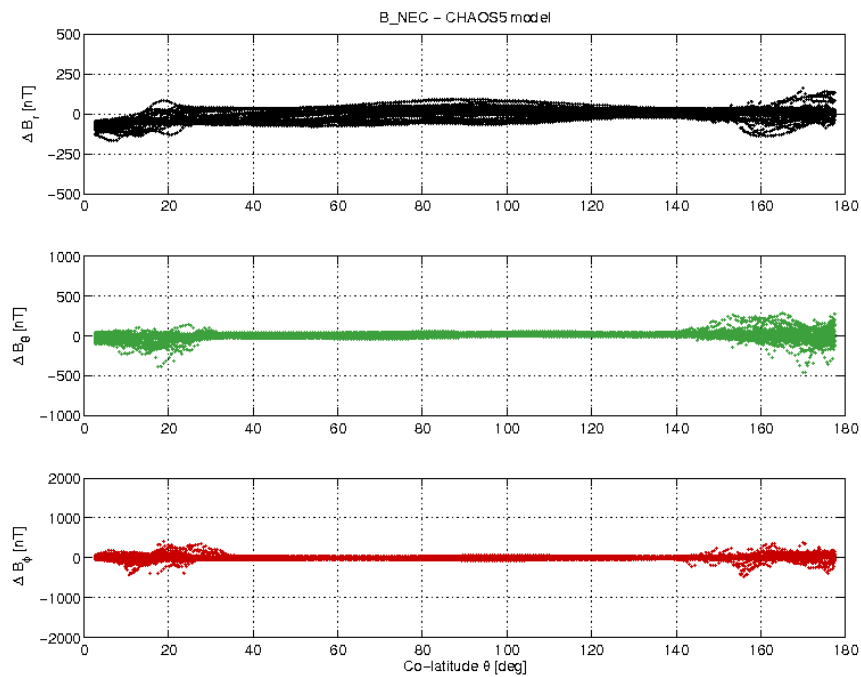
Figure 3-21: S/C C day 22/01 B_{NEC} - B_{Chaos} difference vs colatitude.
