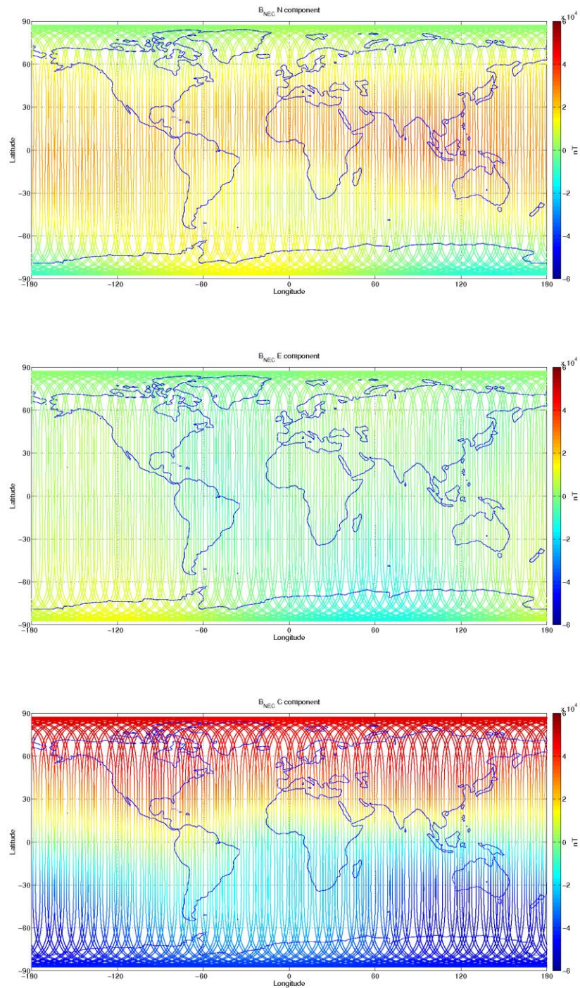
Figure 3-12: S/C C, world map plots of the geomagnetic field and components measured during monitoring period 22/01-28/01. From top to bottom: B NEC components (North, East, and Centre) of magnetic field from VFM measurement.
