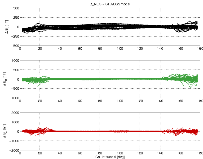
Figure 3-17: S/C A day 22/01 B_{NEC} - B_{Chaos} vs colatitude.
