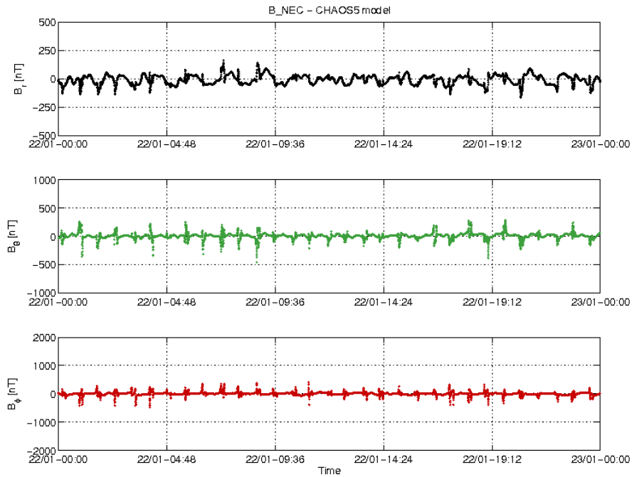
Figure 3-22: S/C C day 22/01 time series of B_{NEC} - B_{Chaos} residuals.
