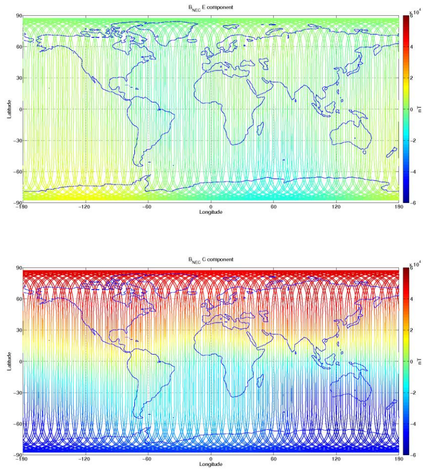
Figure 3-10: S/C A, world map plots of the geomagnetic field and components measured during monitoring period 22/01-28/01. From top to bottom: F-magnetic field from ASM measurement, B_{NEC} components (North, East, and Centre) of magnetic field from VFM measurement.
