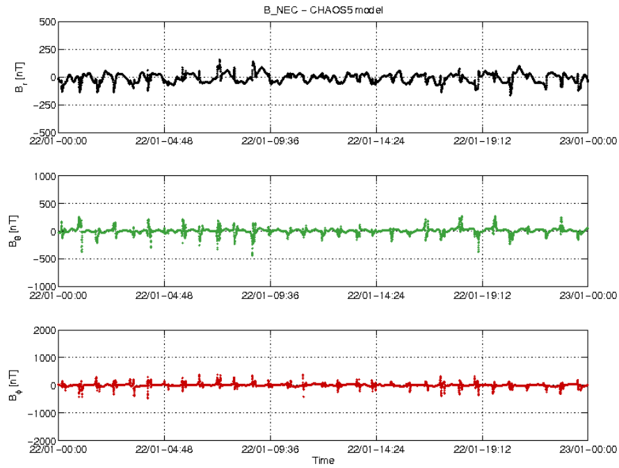
Figure 3-18: S/C A day 22/01: time series of B_{NEC} - B_{Chaos} residuals.
