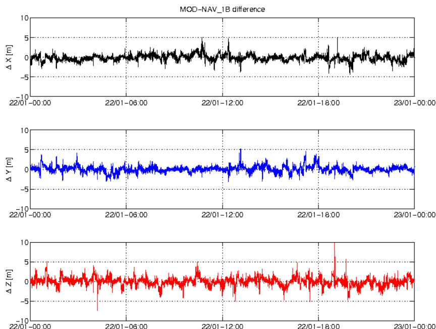
Figure 3-5: Difference MOD-GPSNAV, S/C C, 22/01. From top to bottom: X, Y and Z-axis
