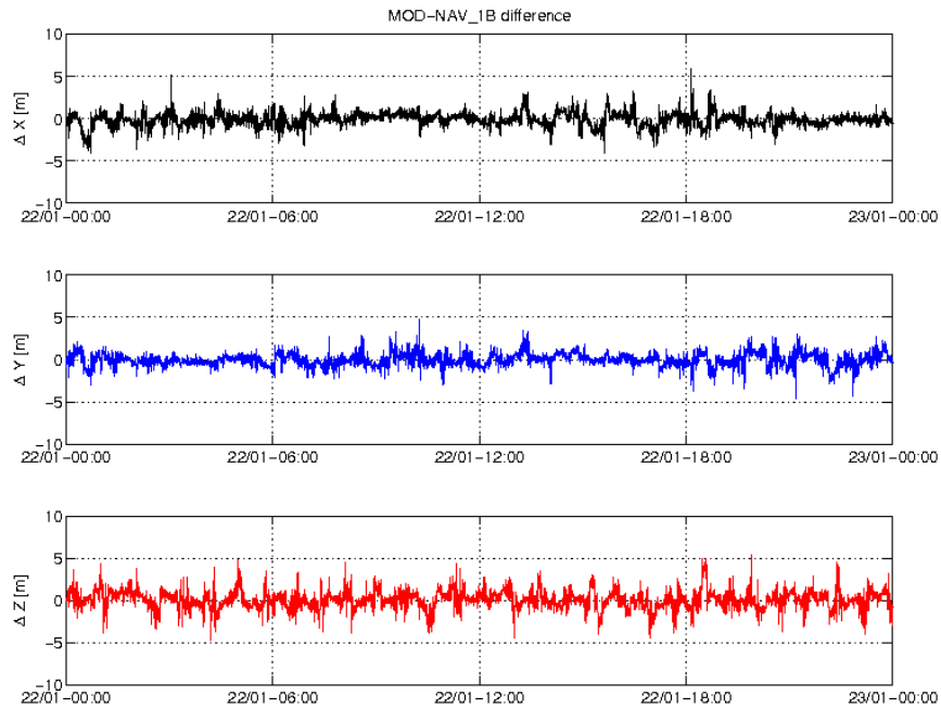
Figure 3-4: Difference MOD-GPSNAV, S/C B, 22/01. From top to bottom: X, Y and Z-axis
