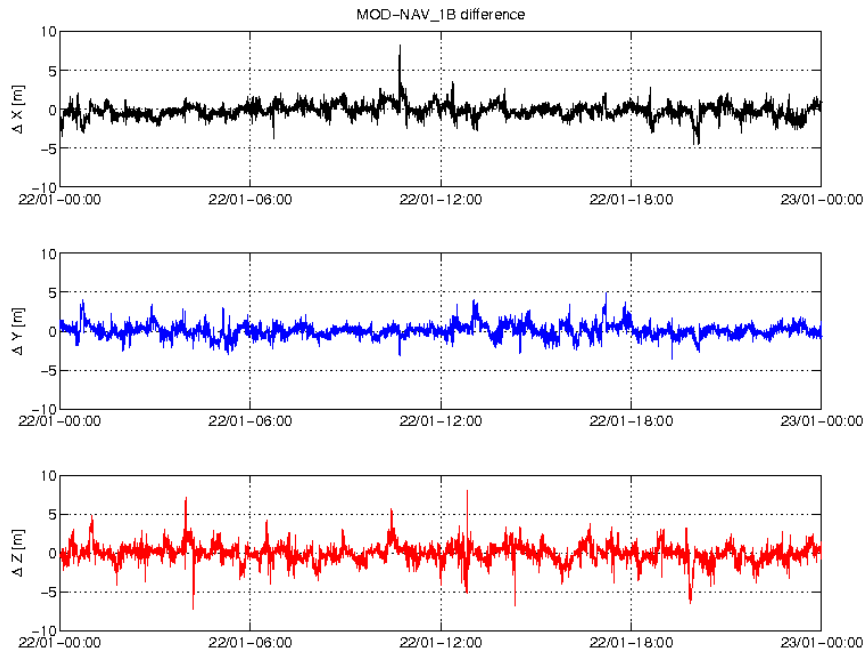
Figure 3-3: Difference MOD-GPSNAV, S/C A, 22/01. From top to bottom: X, Y and Z-axis
