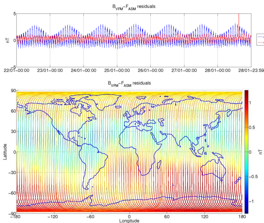
Figure 3-9: ASM-VFM residuals for S/C B, during monitoring period 22/01-28/01. In top figure are plotted: difference between |B_{VFM}| and F_{ASM} (without dB_{Sun} correction) (blue colour), and the residuals with dB_{Sun} corrections (red colour). In bottom figure residuals are presented on the world map.
