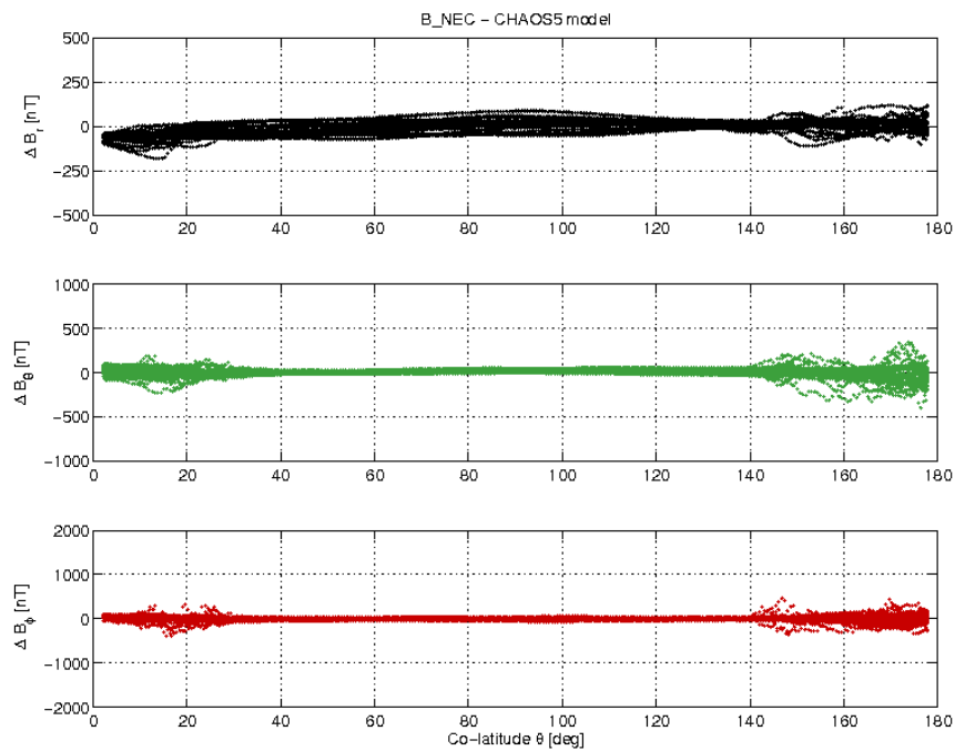
Figure 3-19: S/C B day 22/01 B_{NEC} - B_{Chaos} difference vs colatitude.
