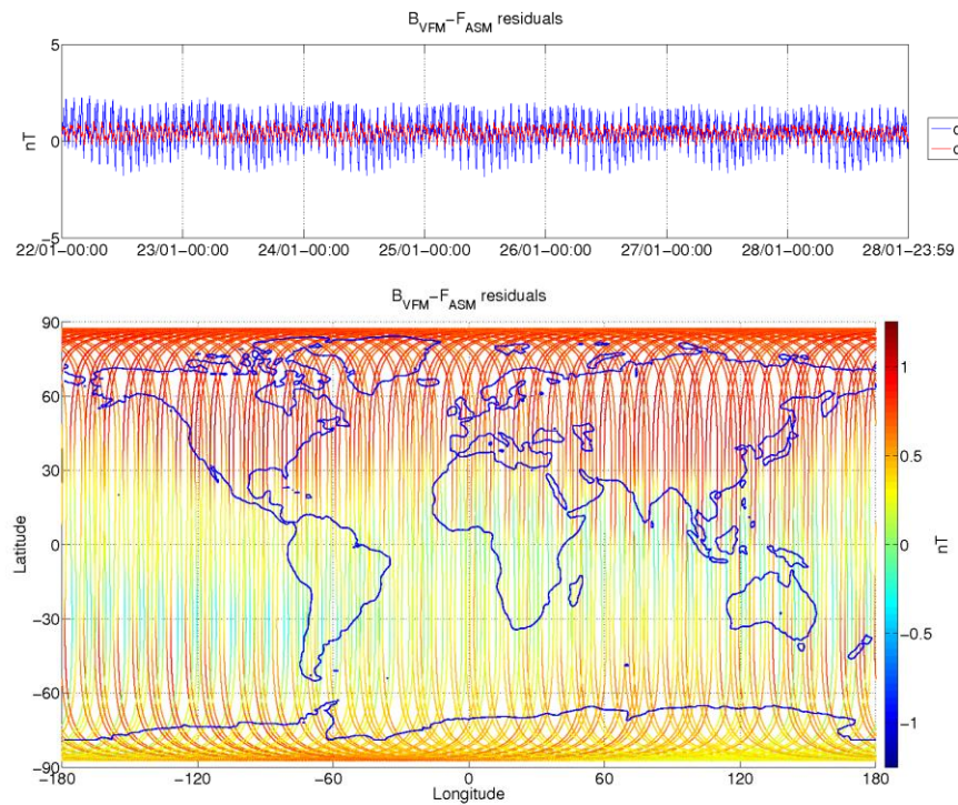
Figure 3-8: ASM-VFM residuals for S/C A, during monitoring period 22/01-28/01. In top figure are plotted: difference between |B_{VFM}| and F_{ASM} (without dB_{Sun} correction) (blue colour), and the residuals with dB_{Sun} corrections (red colour). In bottom figure residuals are presented on the world map.
