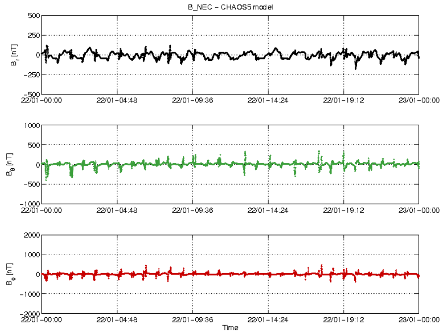
Figure 3-20: S/C B day 22/01 time series of B_{NEC} - B_{Chaos} residuals.
