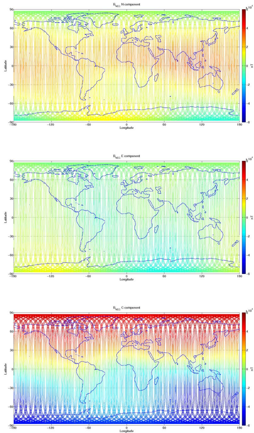
Figure 3-12: S/C C, world map plots of the geomagnetic field and components measured during monitoring period 08/01-14/01. From top to bottom: B_{NEC} components (North, East, and Centre) of magnetic field from VFM measurement.
