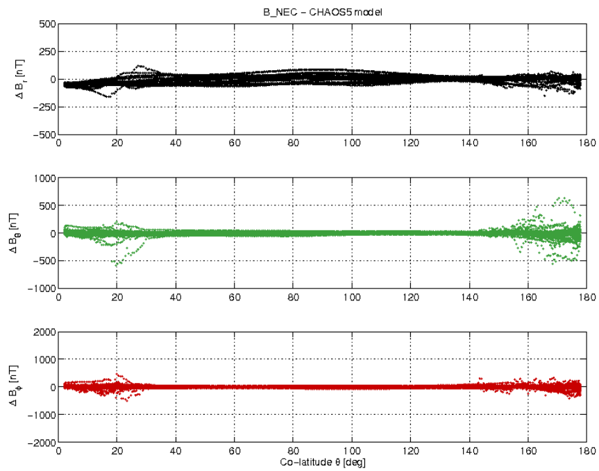
Figure 3-19: S/C B day 08/01 B_{NEC} - B_{Chaos} difference vs colatitude.
