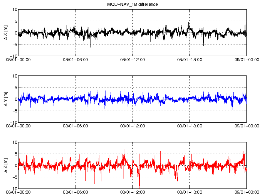
Figure 3-4: Difference MOD-GPSNAV, S/C B, 08/01. From top to bottom: X, Y and Z-axis
