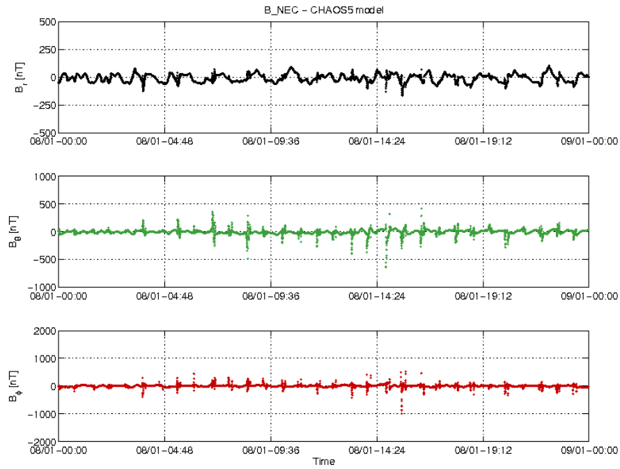
Figure 3-18: S/C A day 08/01: time series of B_{NEC} - B_{Chaos} residuals.
