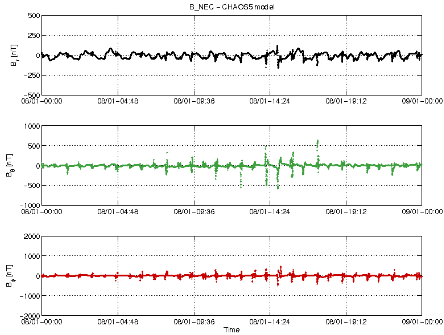
Figure 3-20: S/C B day 08/01 time series of B_{NEC} - B_{Chaos} residuals.
