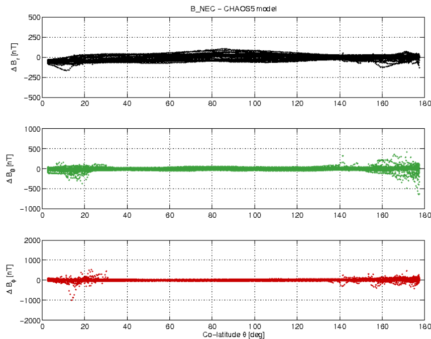
Figure 3-17: S/C A day 08/01 B_{NEC} - B_{Chaos} vs colatitude.
