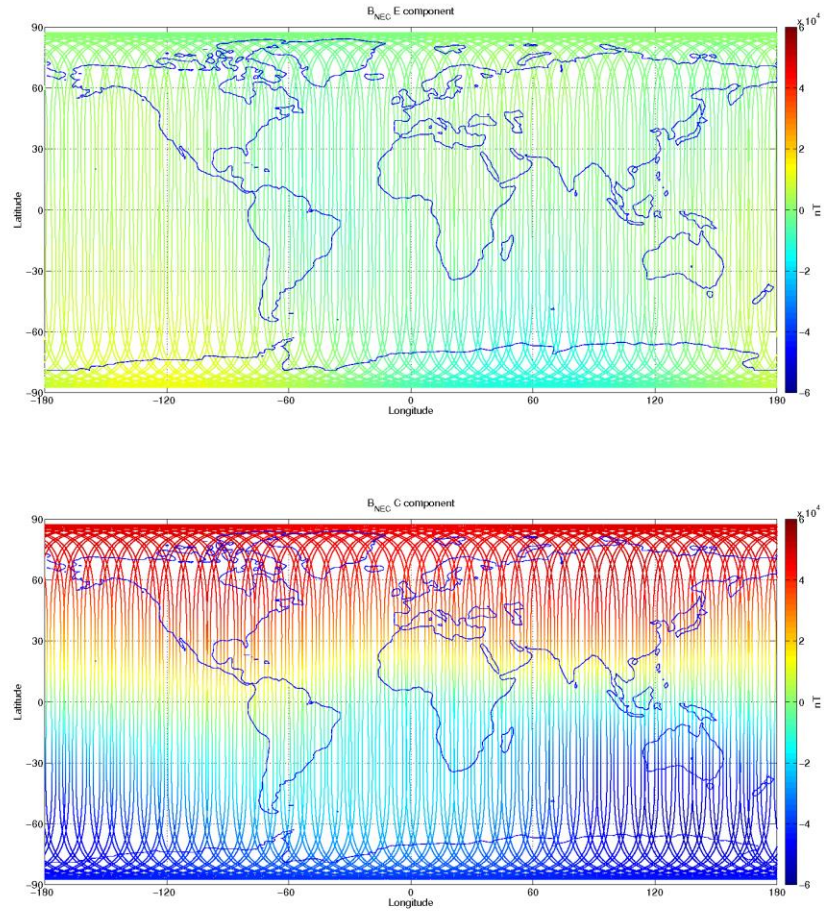
Figure 3-10: S/C A, world map plots of the geomagnetic field and components measured during monitoring period 08/01-14/01. From top to bottom: F-magnetic field from ASM measurement, B_{NEC} components (North, East, and Centre) of magnetic field from VFM measurement.
