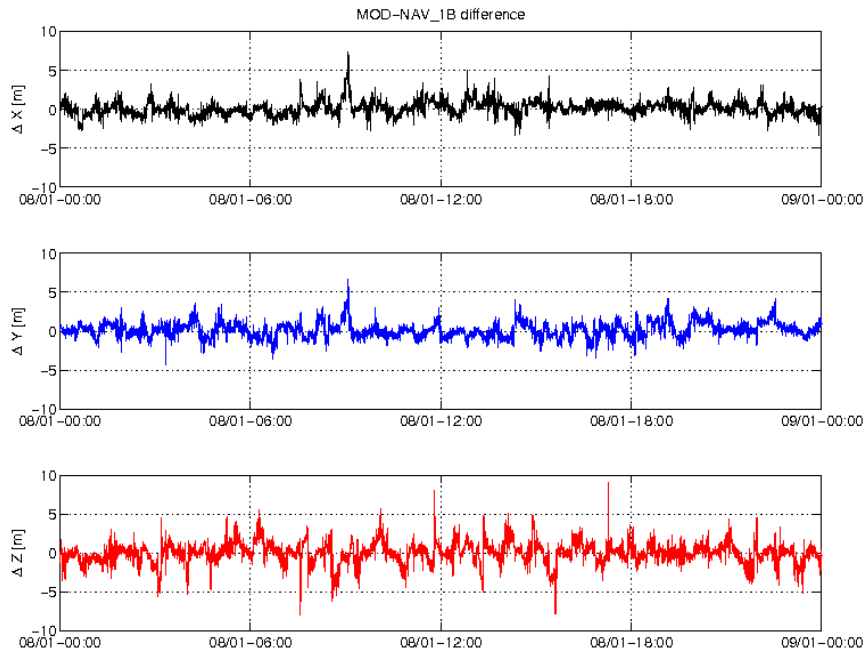
Figure 3-5: Difference MOD-GPSNAV, S/C C, 08/01. From top to bottom: X, Y and Z-axis
