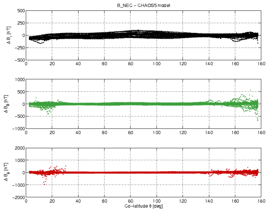
Figure 3-21: S/C C day 08/01 B_{NEC} - B_{Chaos} difference vs colatitude.
