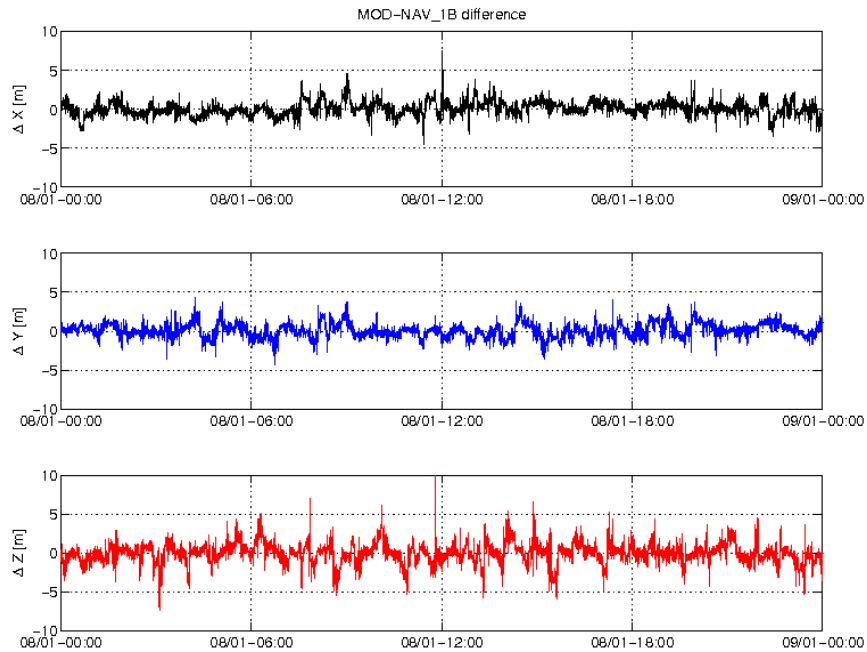
Figure 3-3: Difference MOD-GPSNAV, S/C A, 08/01. From top to bottom: X, Y and Z-axis
