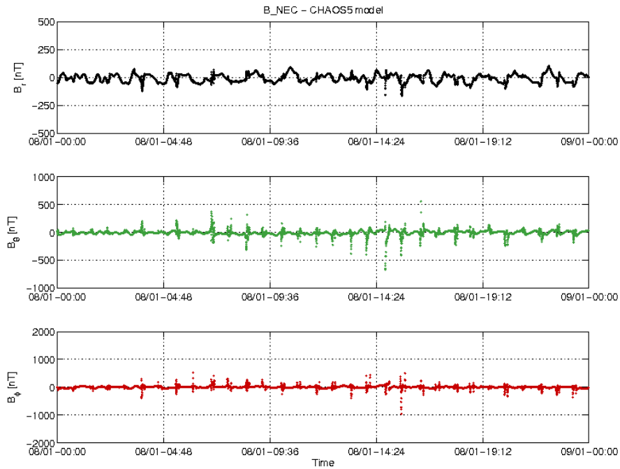
Figure 3-22: S/C C day 08/01 time series of B_{NEC} - B_{Chaos} residuals.
