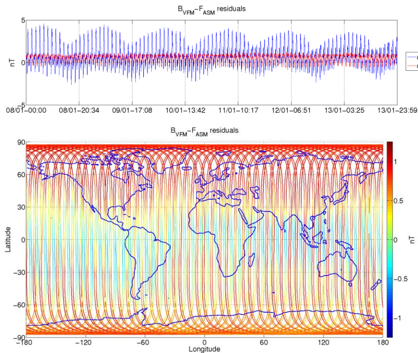
Figure 3-8: ASM-VFM residuals for S/C A, during monitoring period 08/01-14/01. In top figure are plotted: difference between |B_{VFM}| and F_{ASM} (without dB_{Sun} correction) (blue colour), and the residuals with dB_{Sun} corrections (red colour). In bottom figure residuals are presented on the world map.
