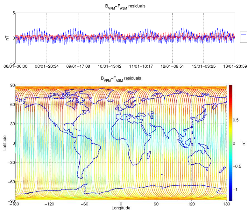
Figure 3-9: ASM-VFM residuals for S/C B, during monitoring period 08/01-14/01. In top figure are plotted: difference between |B_{VFM}| and F_{ASM} (without dB_{Sun} correction) (blue colour), and the residuals with dB_{Sun} corrections (red colour). In bottom figure residuals are presented on the world map.
