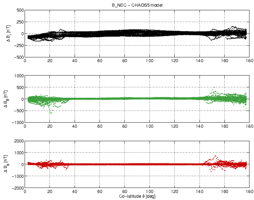
Figure 3-21: S/C C day 01/01 B_{NEC} - B_{Chaos} difference vs colatitude.
