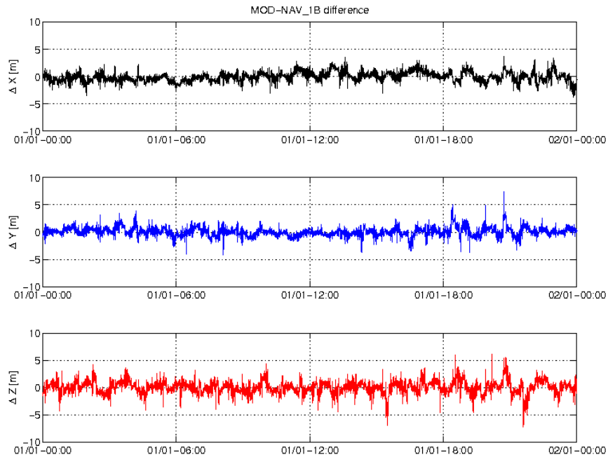
Figure 3-3: Difference MOD-GPSNAV, S/C A, 01/01. From top to bottom: X, Y and Z-axis
