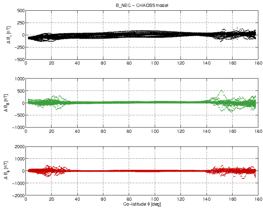
Figure 3-19: S/C B day 01/01 B_{NEC} - B_{Chaos} difference vs colatitude.
