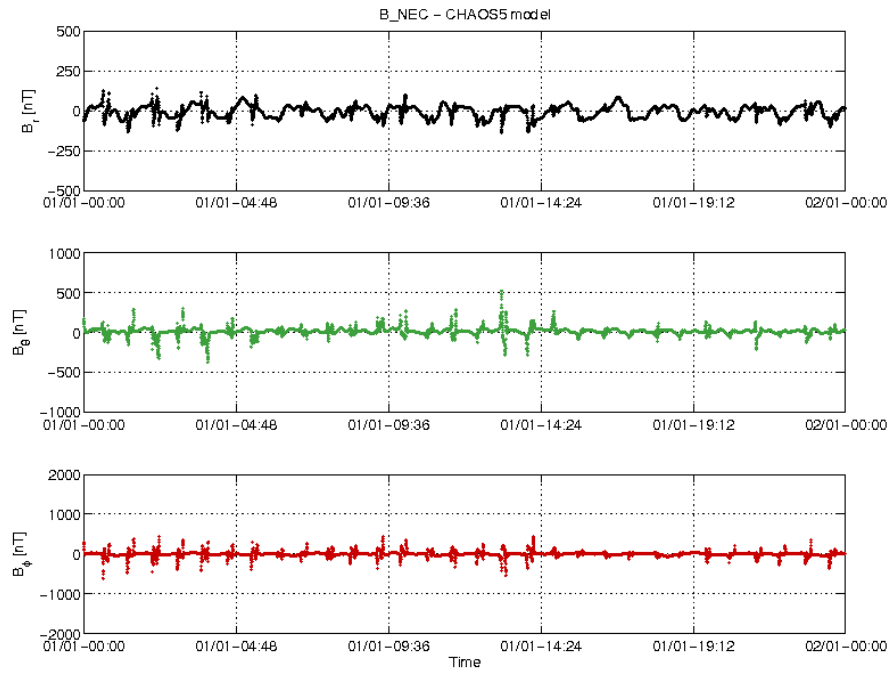
Figure 3-20: S/C B day 01/01 time series of B_{NEC} - B_{Chaos} residuals.
