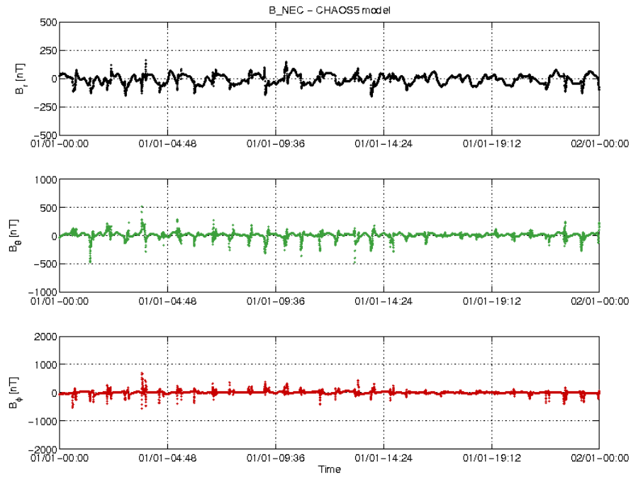
Figure 3-18: S/C A day 01/01: time series of B_{NEC} - B_{Chaos} residuals.
