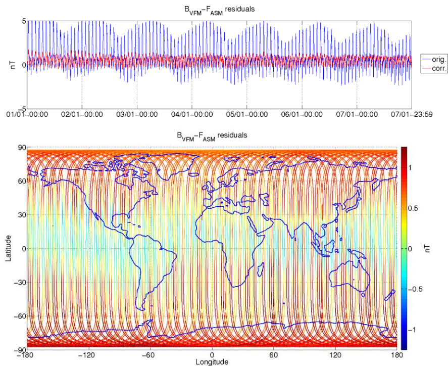
Figure 3-8: ASM-VFM residuals for S/C A, during monitoring period 01/01-07/01. In top figure are plotted: difference between |B_{VFM}| and F_{ASM} (without dB_{Sun} correction) (blue colour), and the residuals with dB_{Sun} corrections (red colour). In bottom figure residuals are presented on the world map.
