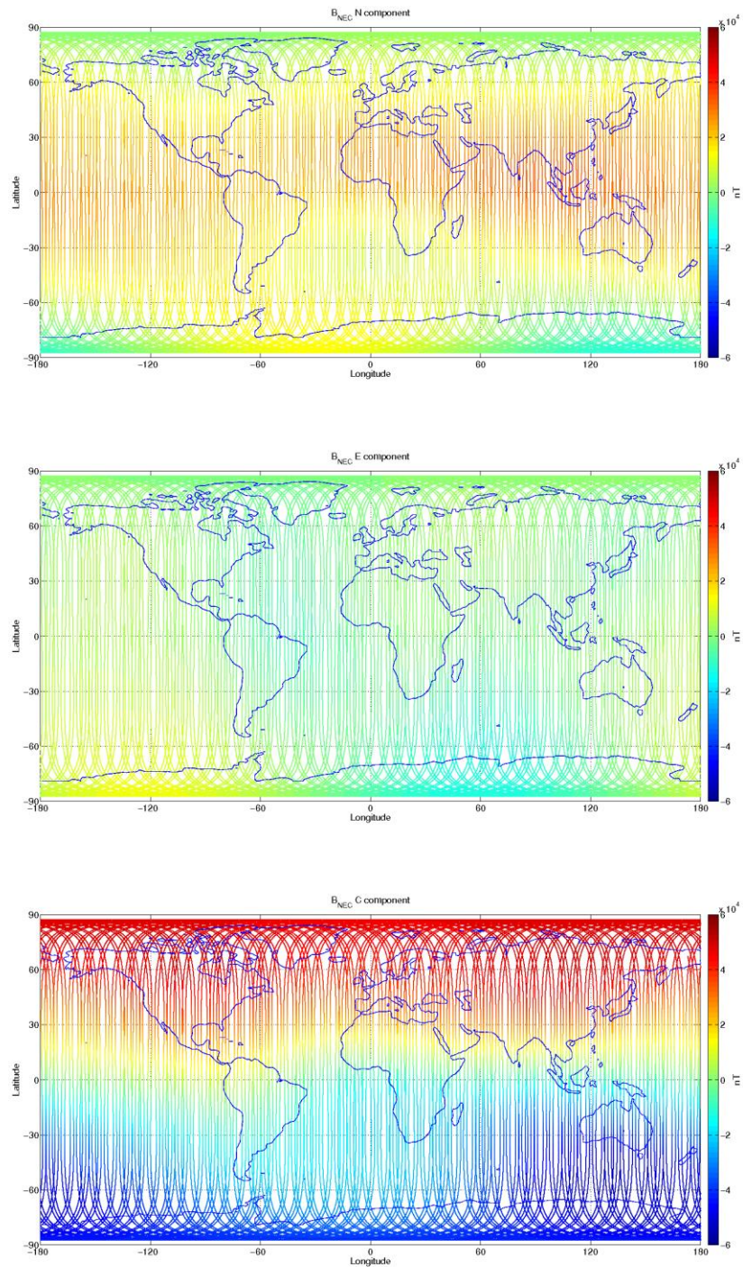
Figure 3-12: S/C C, world map plots of the geomagnetic field and components measured during monitoring period 01/01-07/01. From top to bottom: B_{NEC} components (North, East, and Centre) of magnetic field from VFM measurement.
