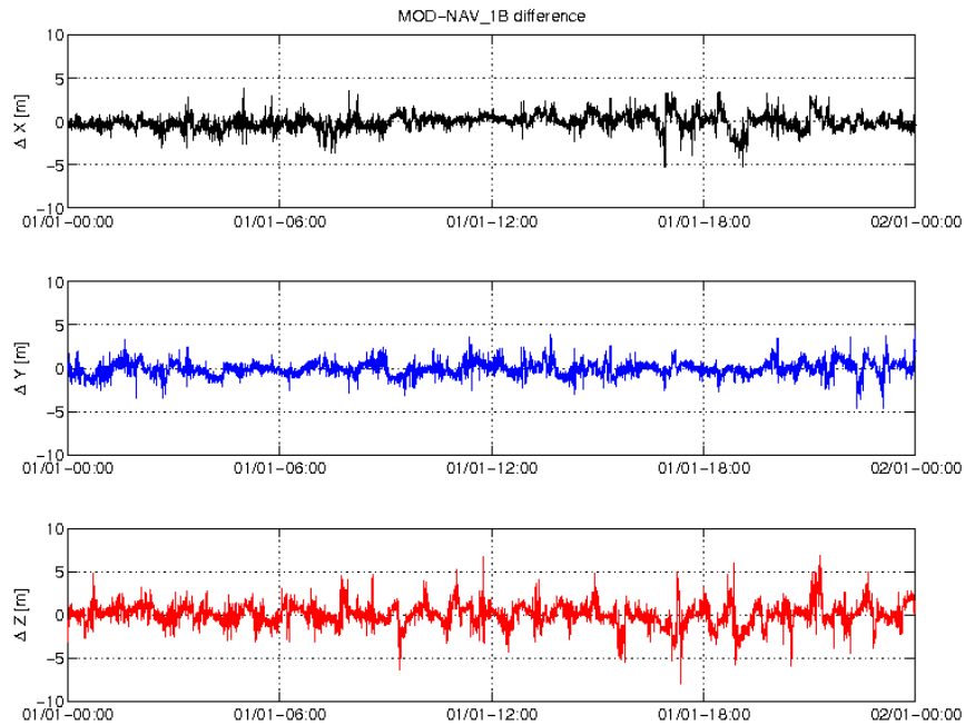
Figure 3-4: Difference MOD-GPSNAV, S/C B, 01/01. From top to bottom: X, Y and Z-axis
