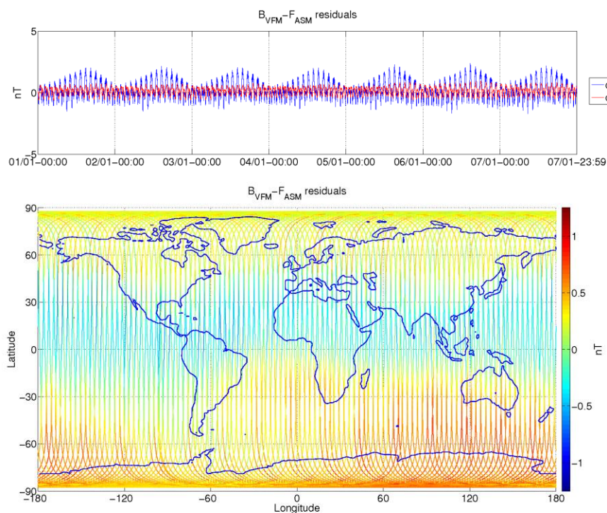
Figure 3-9: ASM-VFM residuals for S/C B, during monitoring period 01/01-07/01. In top figure are plotted: difference between |B_{VFM}| and F_{ASM} (without dB_{Sun} correction) (blue colour), and the residuals with dB_{Sun} corrections (red colour). In bottom figure residuals are presented on the world map.
