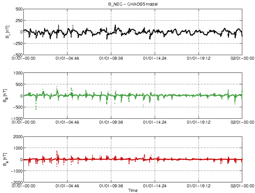
Figure 3-22: S/C C day 01/01 time series of B_{NEC} - B_{Chaos} residuals.
