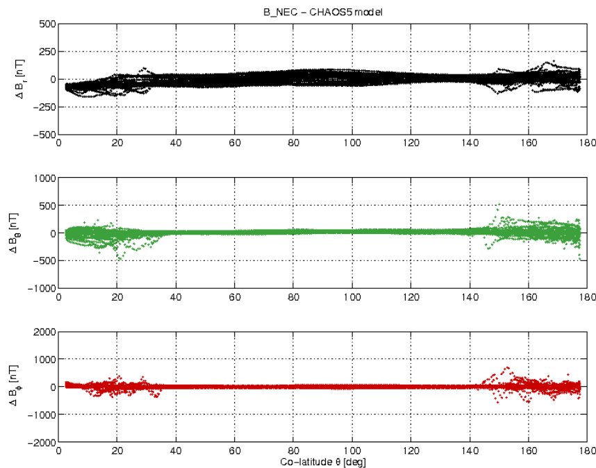
Figure 3-17: S/C A day 01/01 B_{NEC} - B_{Chaos} vs colatitude.
