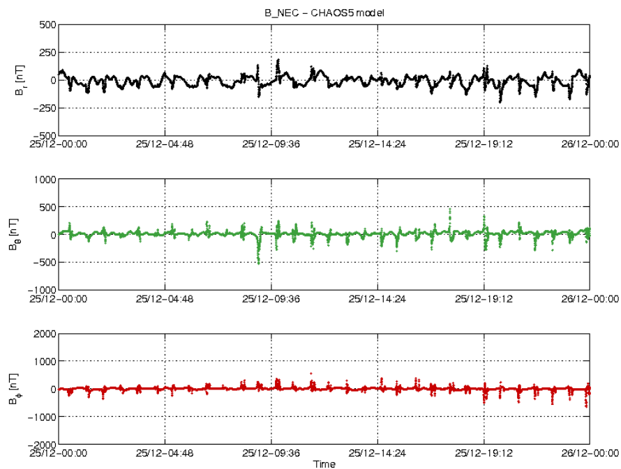
Figure 3-18: S/C A day 25/12: time series of B_{NEC} - B_{Chao5} residuals.
