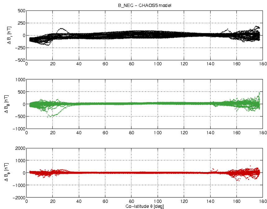
Figure 3-17: S/C A day 25/12 B_{NEC} - B_{Chaos} vs colatitude.
