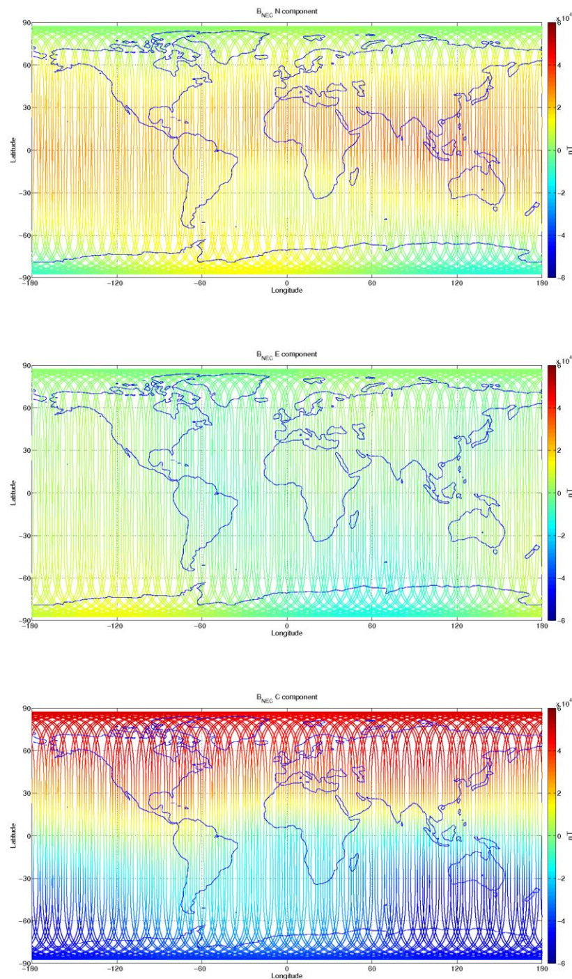
Figure 3-12: S/C C, world map plots of the geomagnetic field and components measured during monitoring period 25/12-31/12. From top to bottom: B_{NEC} components (North, East, and Centre) of magnetic field from VFM measurement.
