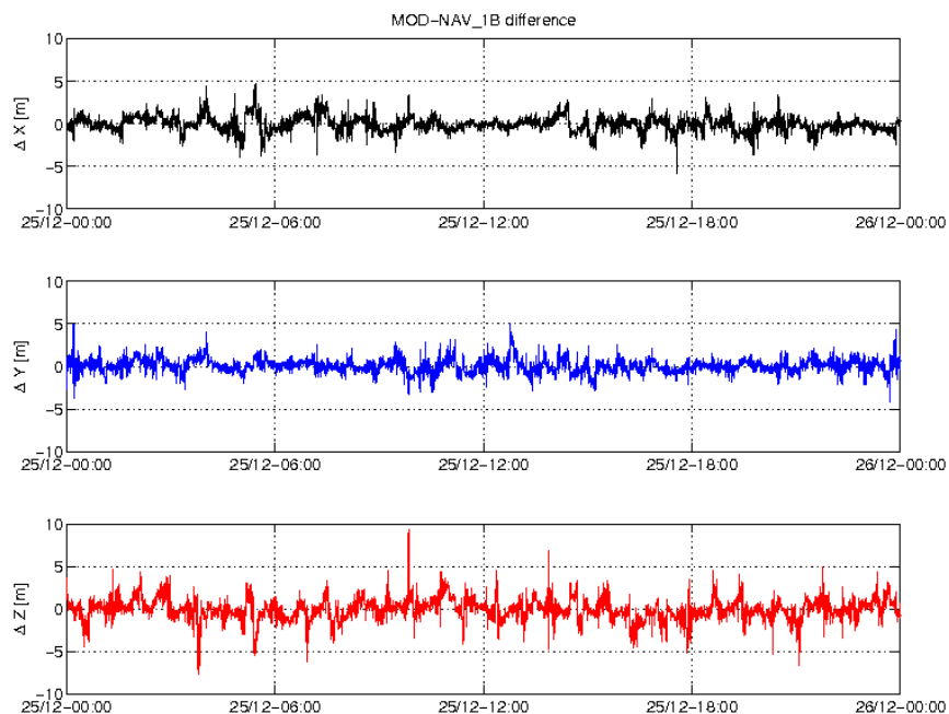
Figure 3-4: Difference MOD-GPSNAV, S/C B, 25/12. From top to bottom: X, Y and Z-axis
