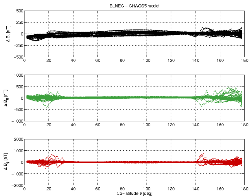
Figure 3-19: S/C B day 25/12 B_{NEC} - B_{Chao5} difference vs colatitude.
