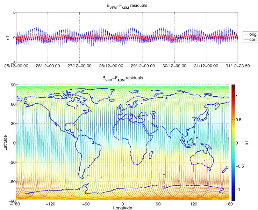
Figure 3-9: ASM-VFM residuals for S/C B, during monitoring period 25/12-31/12. In top figure are plotted: difference between |B_{VFM}| and F_{ASM} (without dB_Sun correction) (blue colour), and the residuals with dB_Sun corrections (red colour). In bottom figure residuals are presented on the world map.
