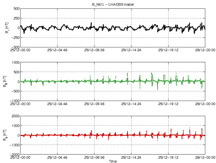
Figure 3-20: S/C B day 25/12 time series of B_{NEC} - B_{Chao5} residuals.
