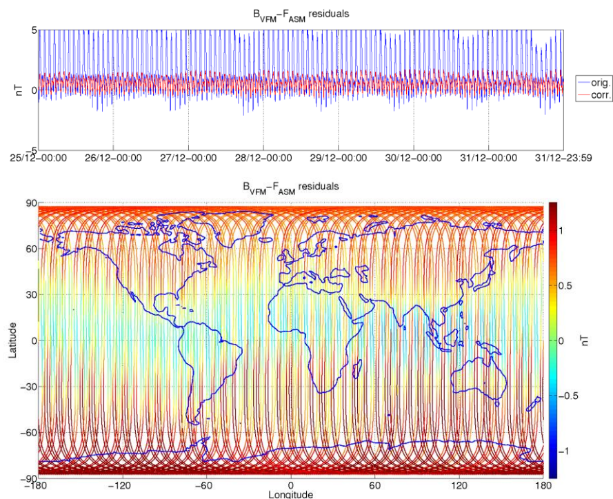
Figure 3-8: ASM-VFM residuals for S/C A, during monitoring period 25/12-31/12. In top figure are plotted: difference between |B_{VFM}| and F_{ASM} (without dB_{Sun} correction) (blue colour), and the residuals with dB_{Sun} corrections (red colour). In bottom figure residuals are presented on the world map.
