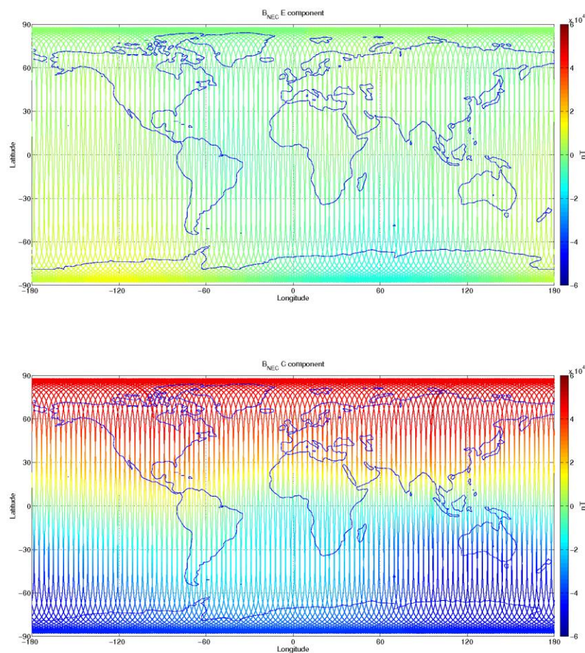
Figure 3-11: S/C B, world map plots of the geomagnetic field and components measured during monitoring period 25/12-31/12. From top to bottom: F-magnetic field from ASM measurement, B NEC components (North, East, and Centre) of magnetic field from VFM measurement.
