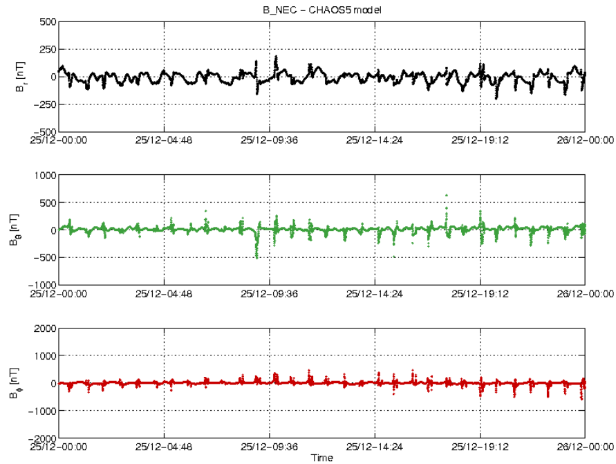
Figure 3-22: S/C C day 25/12 time series of B_{NEC} - B_{Chaos} residuals.
