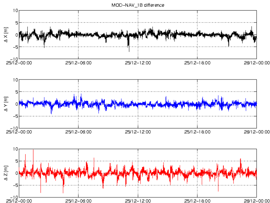
Figure 3-5: Difference MOD-GPSNAV, S/C C, 25/12. From top to bottom: X, Y and Z-axis
