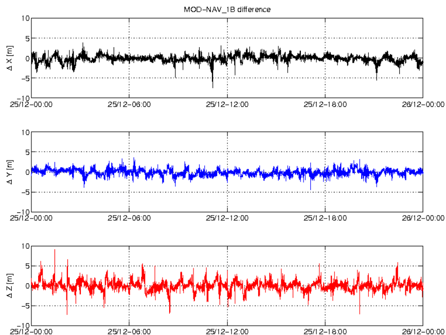
Figure 3-3: Difference MOD-GPSNAV, S/C A, 25/12. From top to bottom: X, Y and Z-axis
