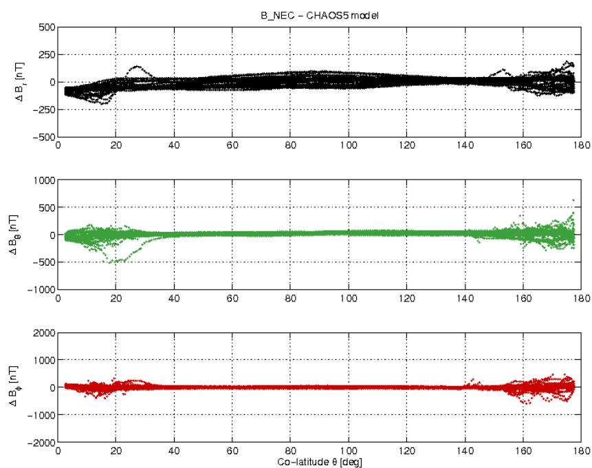
Figure 3-21: S/C C day 25/12 B_{NEC} - B_{Chao5} difference vs colatitude.
