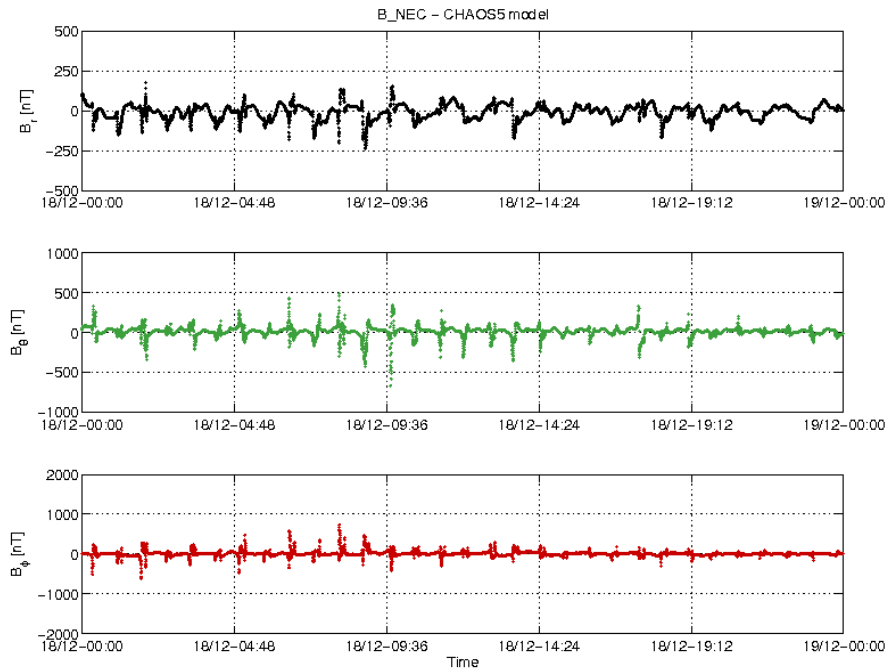
Figure 3-22: S/C C day 18/12 time series of B_{NEC} - B_{Chaos} residuals.
