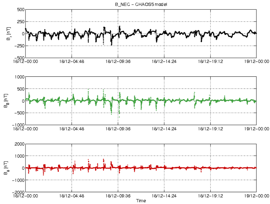
Figure 3-18: S/C A day 18/12: time series of B_{NEC} - B_{Chaos} residuals.
