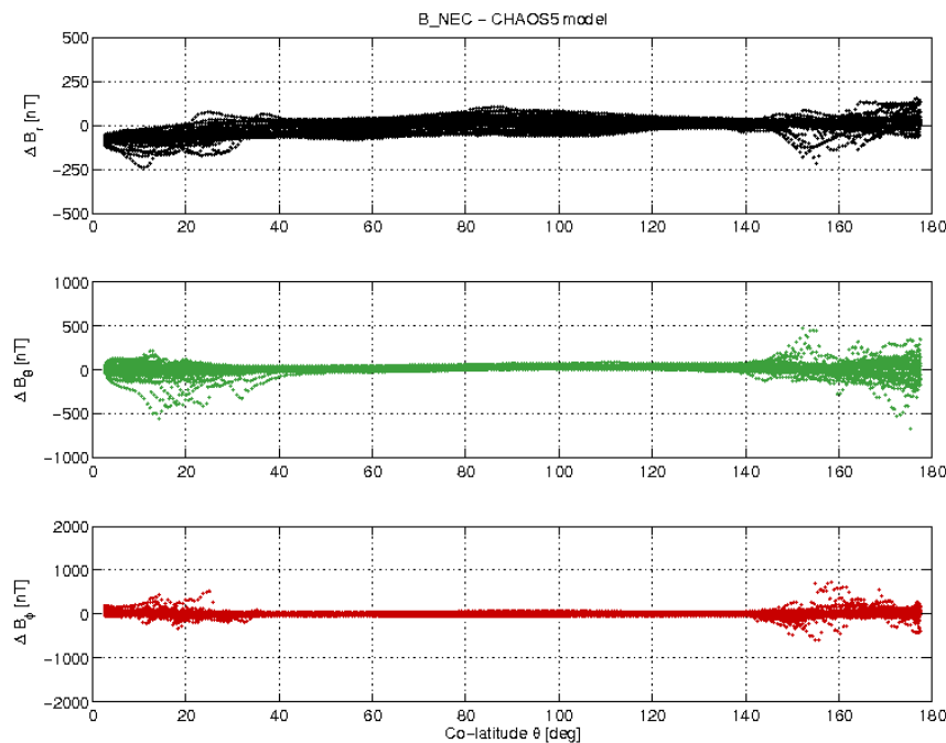
Figure 3-17: S/C A day 18/12 B_{NEC} - B_{Chaos} vs colatitude.
