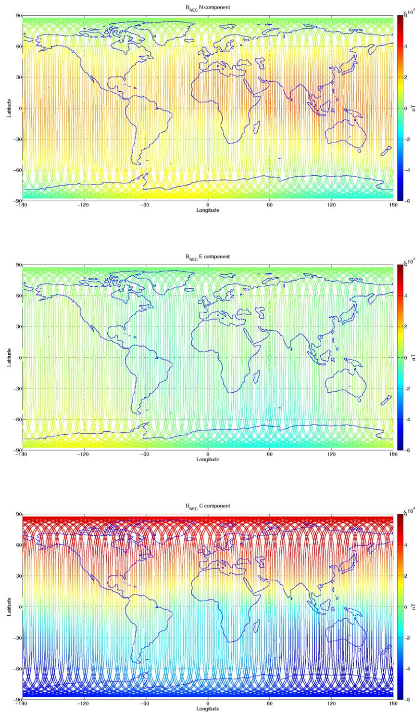
Figure 3-12: S/C C, world map plots of the geomagnetic field and components measured during monitoring period 18/12-24/12. From top to bottom: B_{NEC} components (North, East, and Centre) of magnetic field from VFM measurement.
