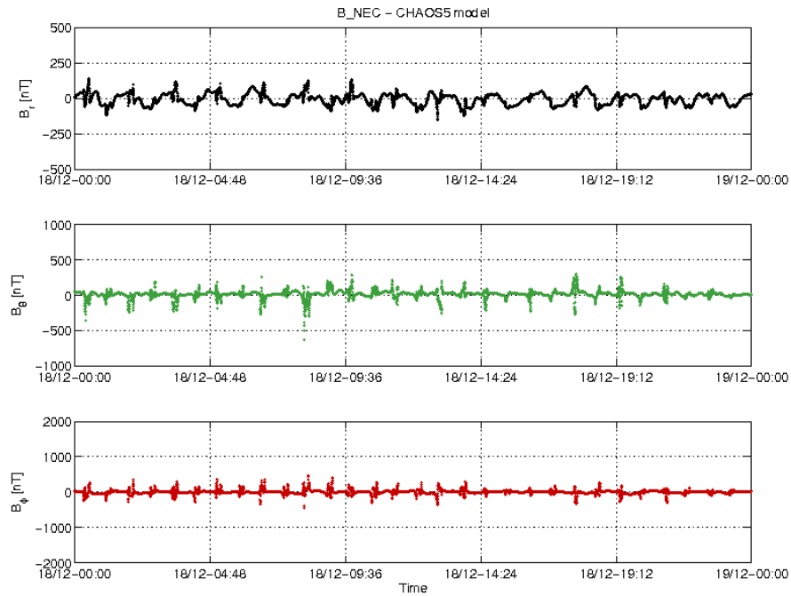
Figure 3-20: S/C B day 18/12 time series of B_{NEC} - B_{Chaos} residuals.
