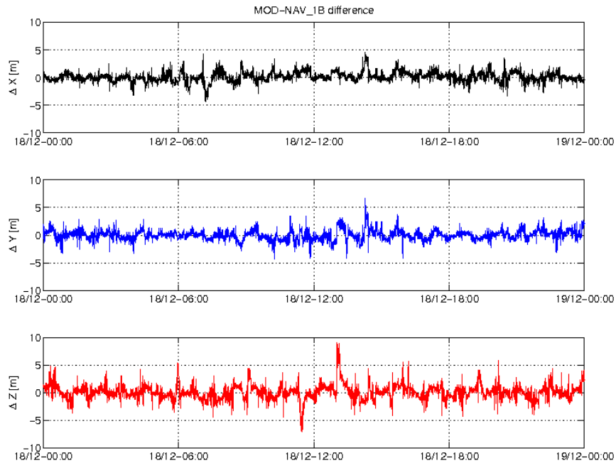
Figure 3-4: Difference MOD-GPSNAV, S/C B, 18/12. From top to bottom: X, Y and Z-axis
