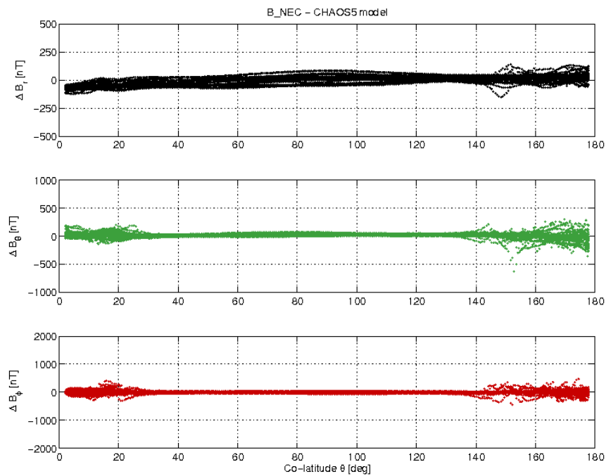
Figure 3-19: S/C B day 18/12 B_{NEC} - B_{Chaos} difference vs colatitude.
