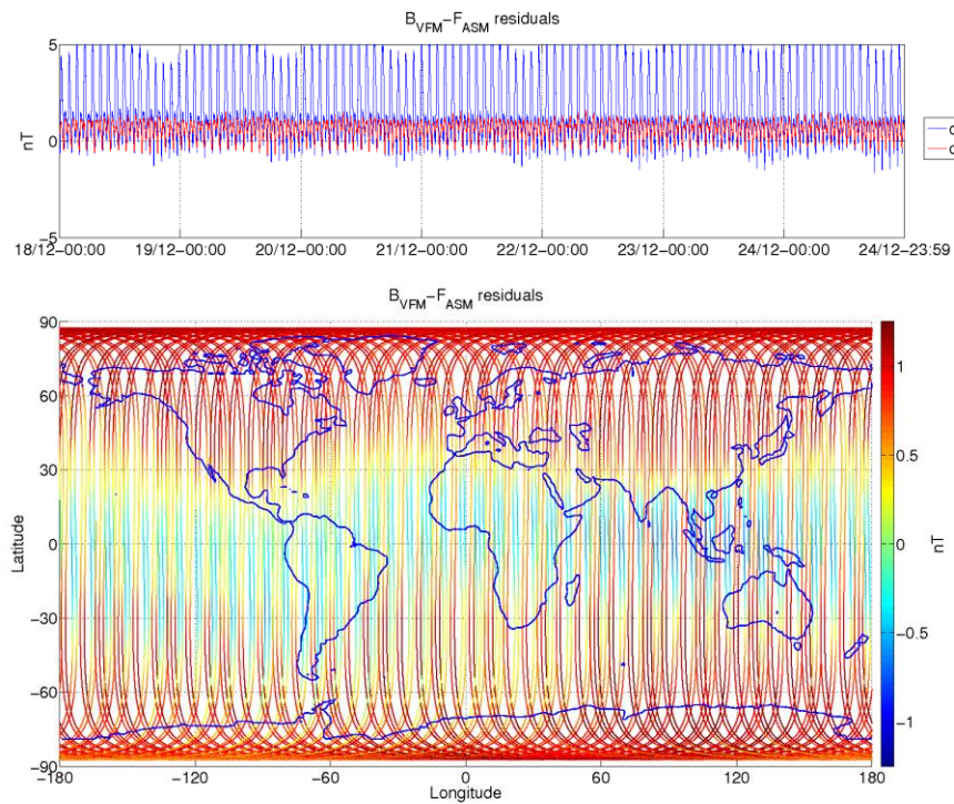
Figure 3-8: ASM-VFM residuals for S/C A, during monitoring period 18/12-24/12. In top figure are plotted: difference between |B_{VFM}| and F_{ASM} (without dB_{Sun} correction) (blue colour), and the residuals with dB_{Sun} corrections (red colour). In bottom figure residuals are presented on the world map.
