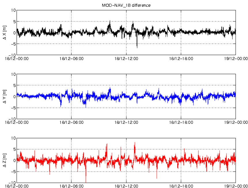
Figure 3-5: Difference MOD-GPSNAV, S/C C, 18/12. From top to bottom: X, Y and Z-axis
