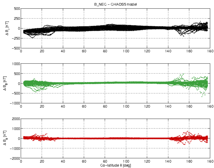
Figure 3-21: S/C C day 18/12 B_{NEC} - B_{Chaos} difference vs colatitude.
