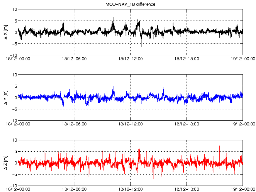
Figure 3-3: Difference MOD-GPSNAV, S/C A, 18/12. From top to bottom: X, Y and Z-axis
