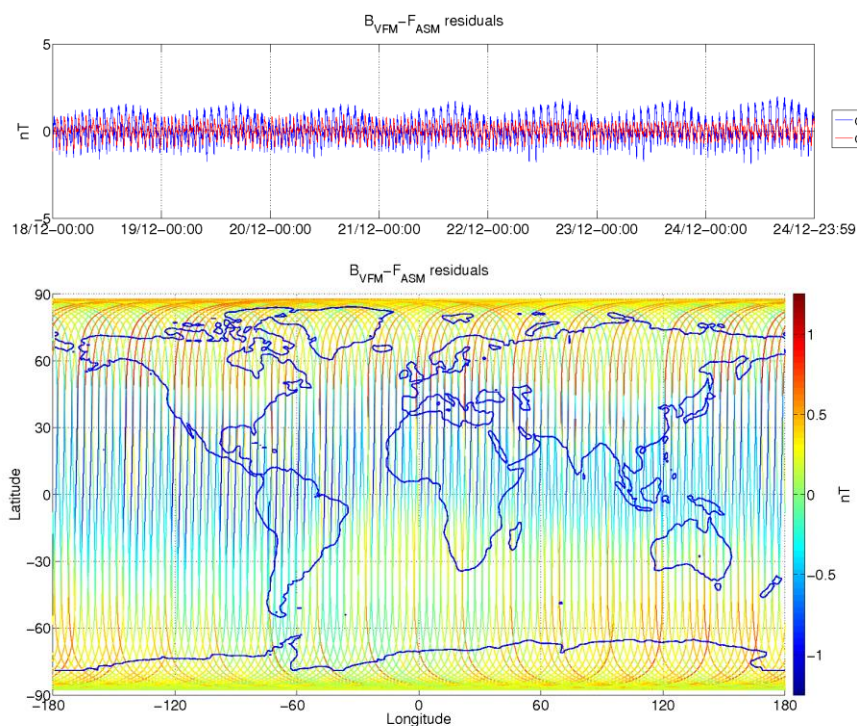
Figure 3-9: ASM-VFM residuals for S/C B, during monitoring period 18/12-24/12. In top figure are plotted: difference between |B_{VFM}| and F_{ASM} (without dB_{Sun} correction) (blue colour), and the residuals with dB_{Sun} corrections (red colour). In bottom figure residuals are presented on the world map.
