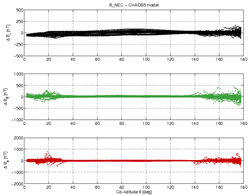
Figure 3-19: S/C B day 11/12 B_{NEC} - B_{Chaos} difference vs colatitude.
