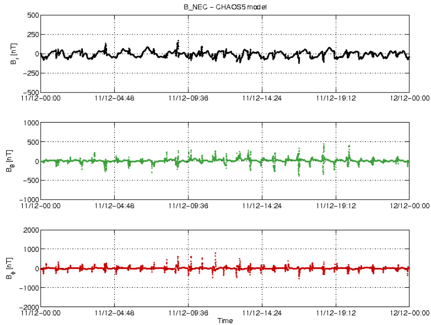
Figure 3-20: S/C B day 11/12 time series of B_{NEC} - B_{Chaos} residuals.
