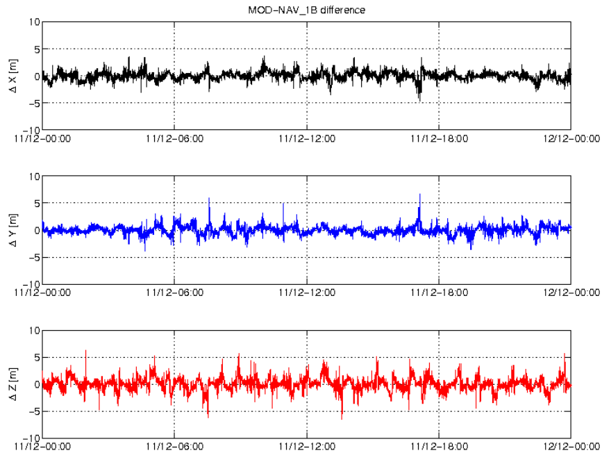
Figure 3-3: Difference MOD-GPSNAV, S/C A, 11/12. From top to bottom: X, Y and Z-axis
