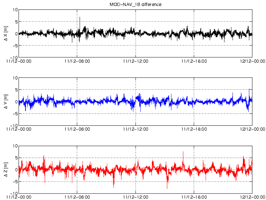
Figure 3-4: Difference MOD-GPSNAV, S/C B, 11/12. From top to bottom: X, Y and Z-axis
