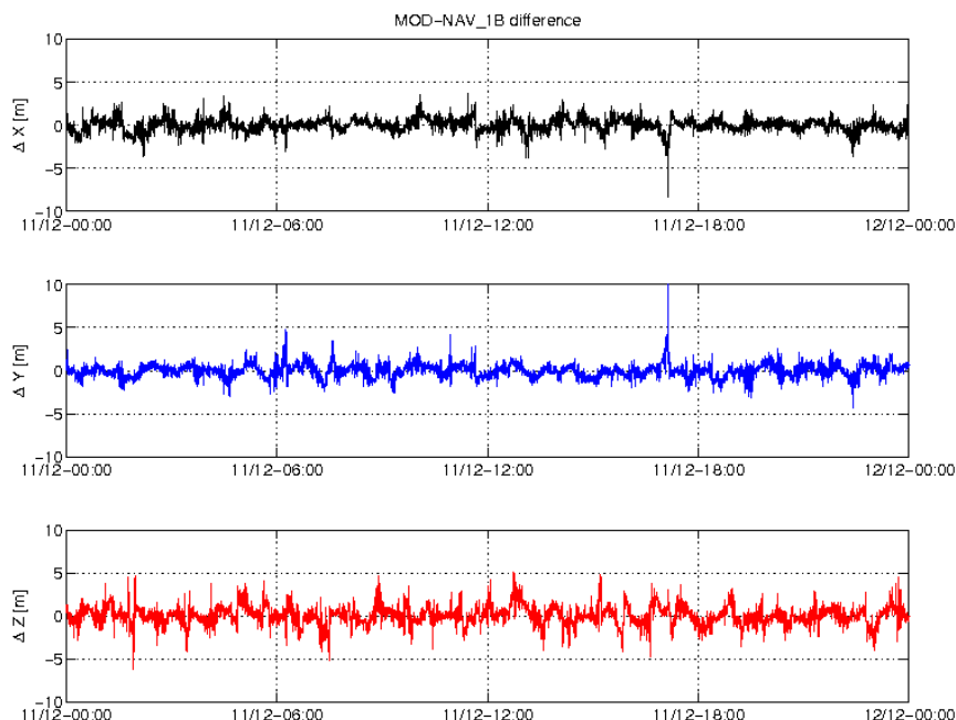
Figure 3-5: Difference MOD-GPSNAV, S/C C, 11/12. From top to bottom: X, Y and Z-axis
