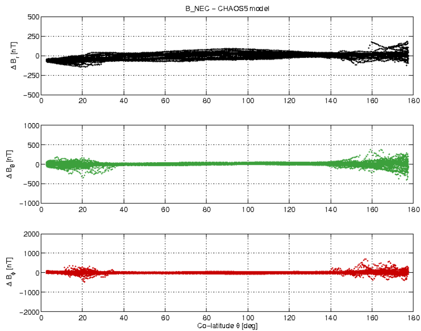
Figure 3-21: S/C C day 11/12 B_{NEC} - B_{Chaos} difference vs colatitude.
