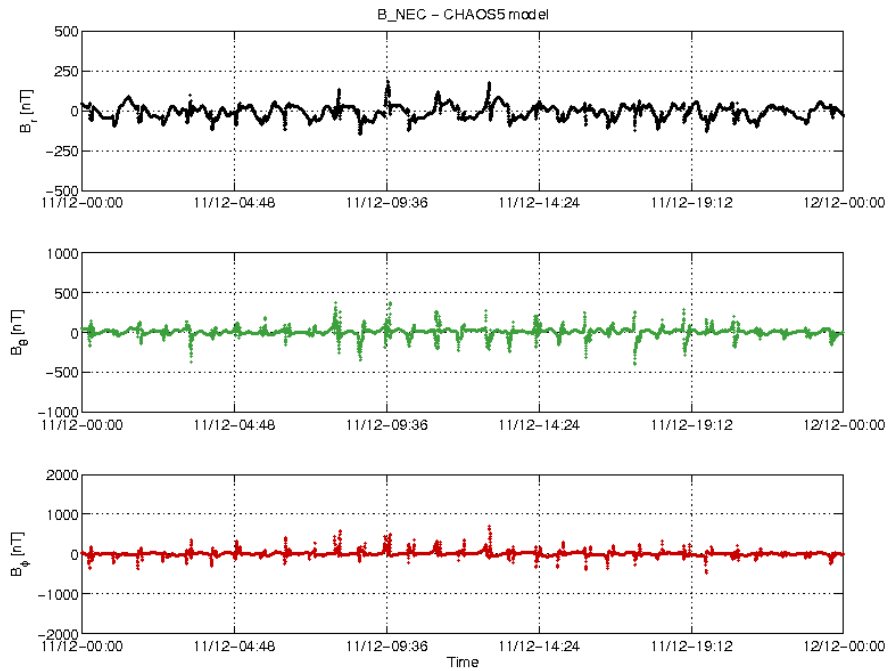
Figure 3-22: S/C C day 11/12 time series of B_{NEC} - B_{Chaos} residuals.
