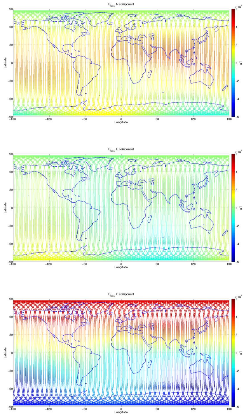
Figure 3-12: S/C C, world map plots of the geomagnetic field and components measured during monitoring period 11/12-17/12. From top to bottom: B_{NEC} components (North, East, and Centre) of magnetic field from VFM measurement.
