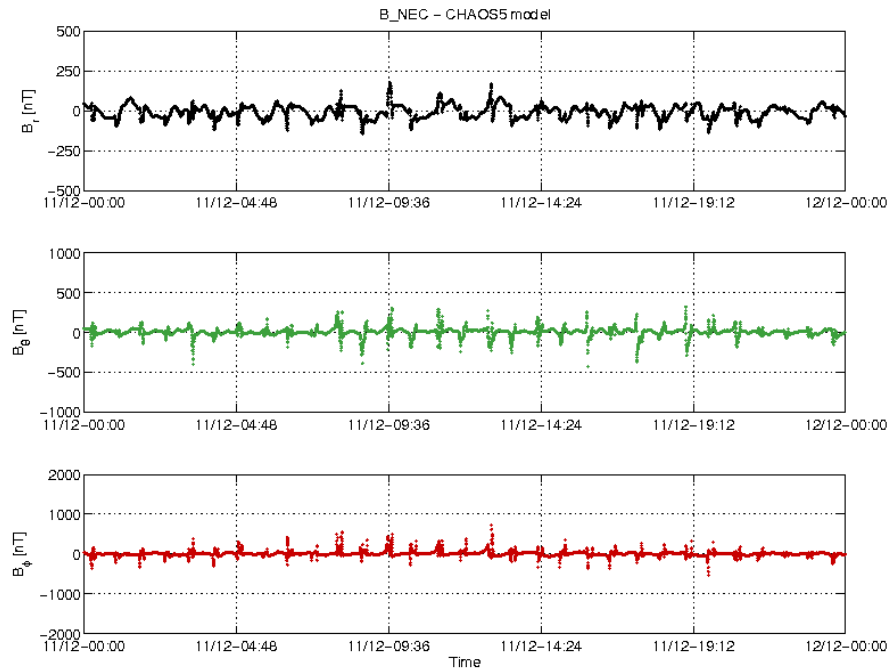
Figure 3-18: S/C A day 11/12: time series of B_{NEC} - B_{Chaos} residuals.
