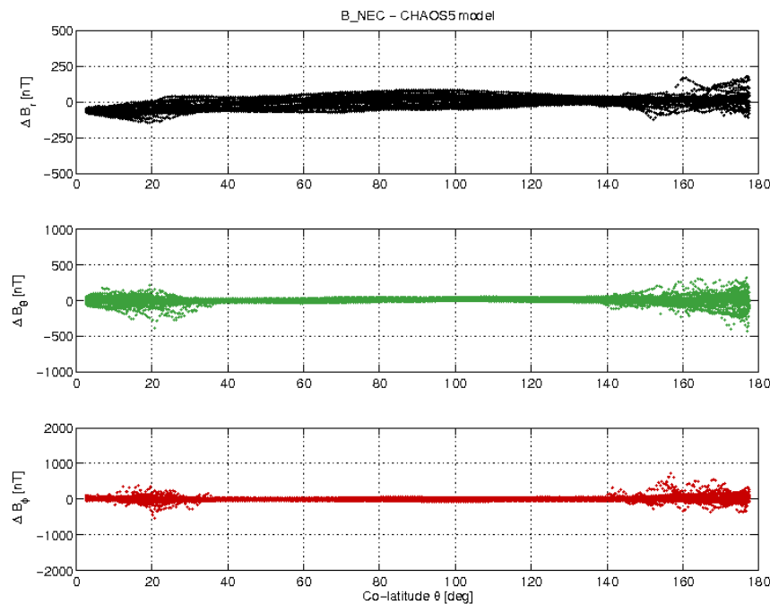
Figure 3-17: S/C A day 11/12 B_{NEC} - B_{Chaos} vs colatitude.
