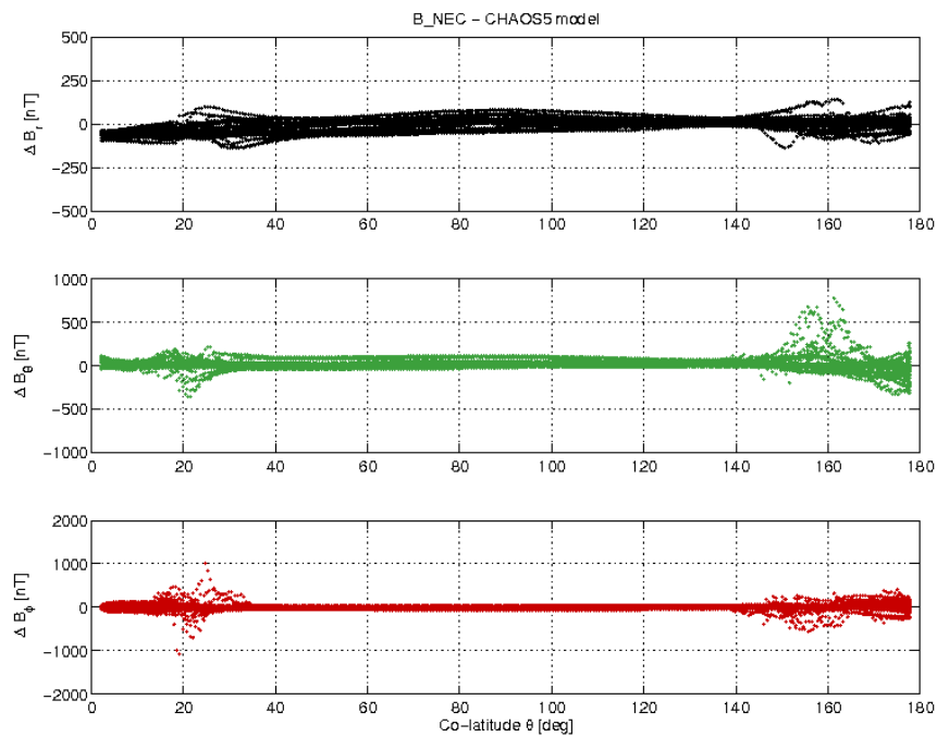
Figure 3-19: S/C B day 04/12 B_{NEC} - B_{Chaos} difference vs colatitude.
