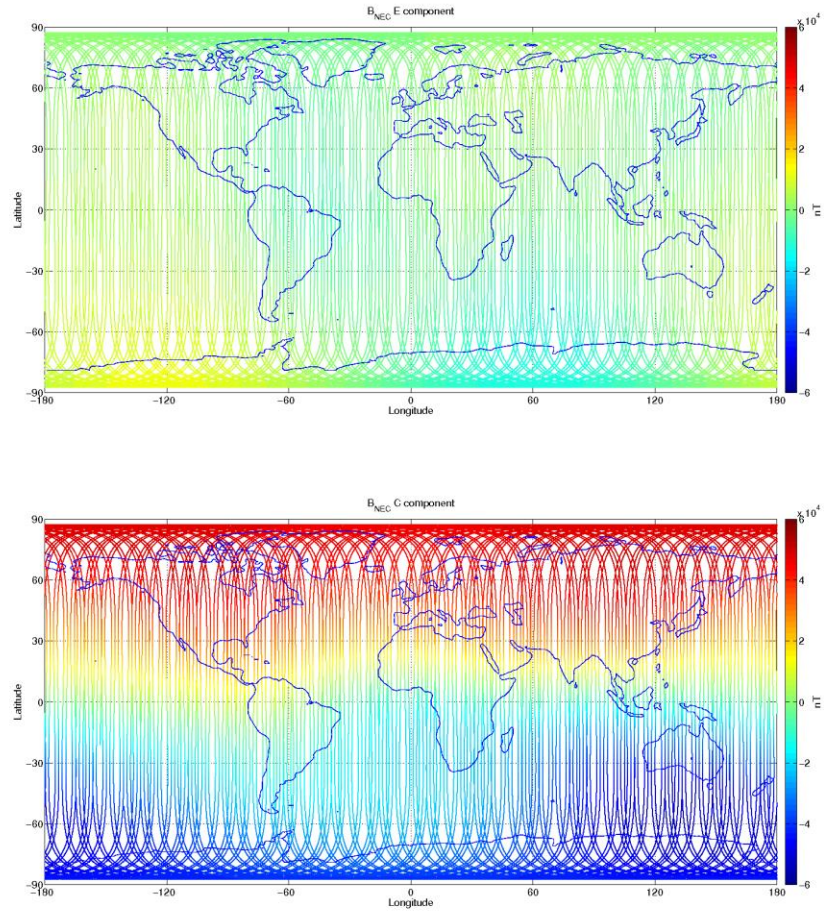
Figure 3-10: S/C A, world map plots of the geomagnetic field and components measured during monitoring period 04/12-10/12. From top to bottom: F-magnetic field from ASM measurement, B_{NEC} components (North, East, and Centre) of magnetic field from VFM measurement.
