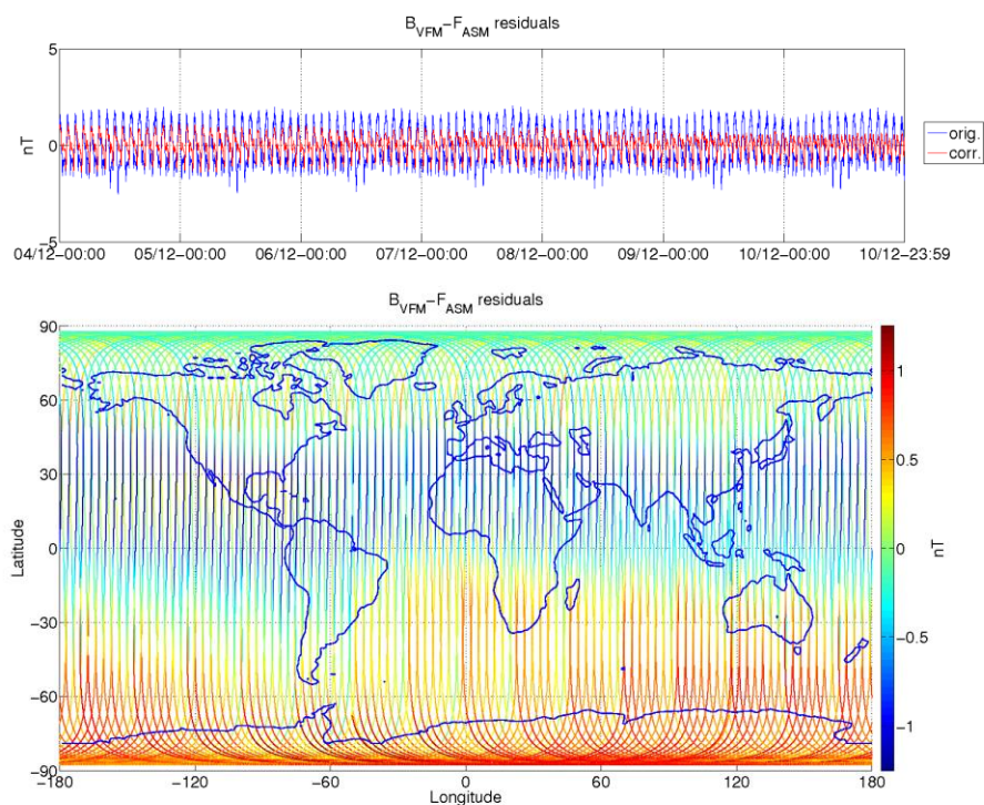
Figure 3-9: ASM-VFM residuals for S/C B, during monitoring period 04/12-10/12. In top figure are plotted: difference between |B_{VFM}| and F_{ASM} (without dB_{Sun} correction) (blue colour), and the residuals with dB_{Sun} corrections (red colour). In bottom figure residuals are presented on the world map.
