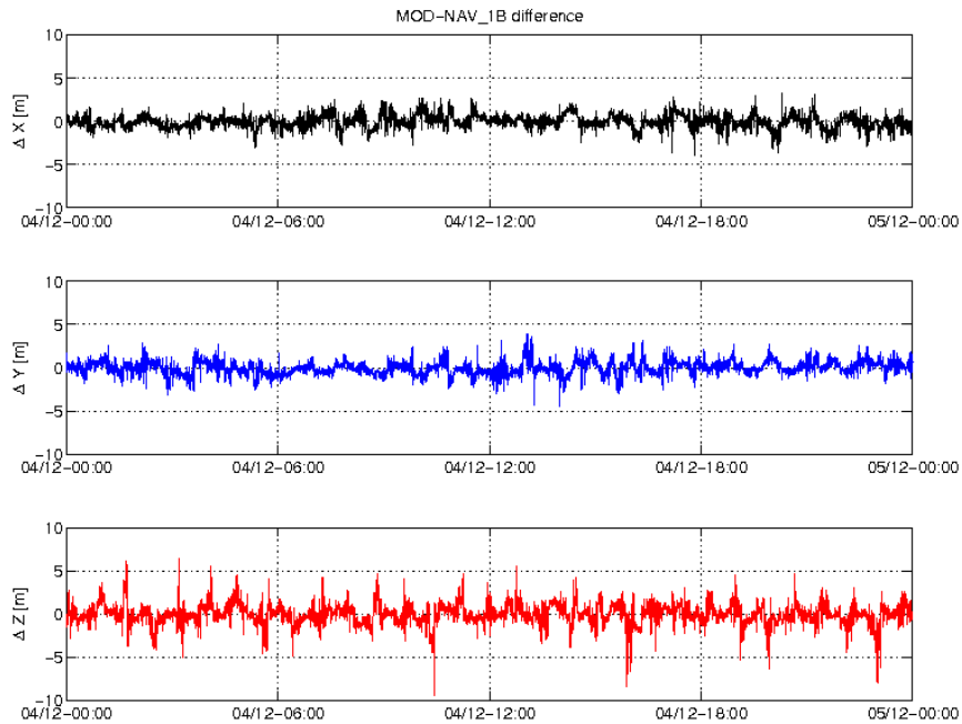
Figure 3-4: Difference MOD-GPSNAV, S/C B, 04/12. From top to bottom: X, Y and Z-axis
