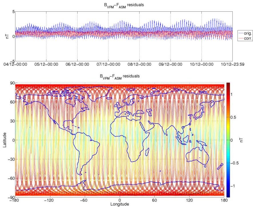
Figure 3-8: ASM-VFM residuals for S/C A, during monitoring period 04/12-10/12. In top figure are plotted: difference between |B VFM | and F ASM (without dB Sun correction) (blue colour), and the residuals with dB Sun corrections (red colour). In bottom figure residuals are presented on the world map.
