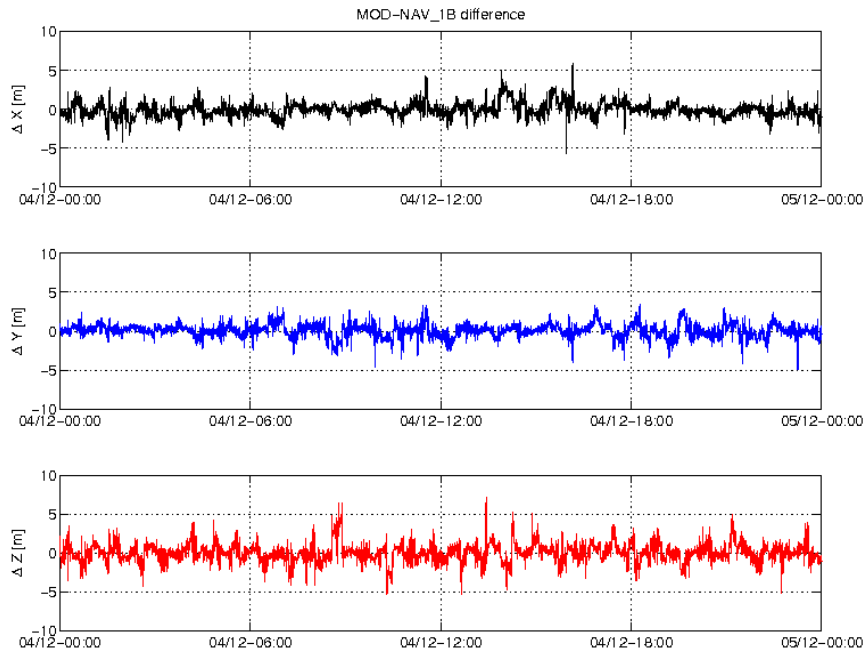
Figure 3-3: Difference MOD-GPSNAV, S/C A, 04/12. From top to bottom: X, Y and Z-axis
