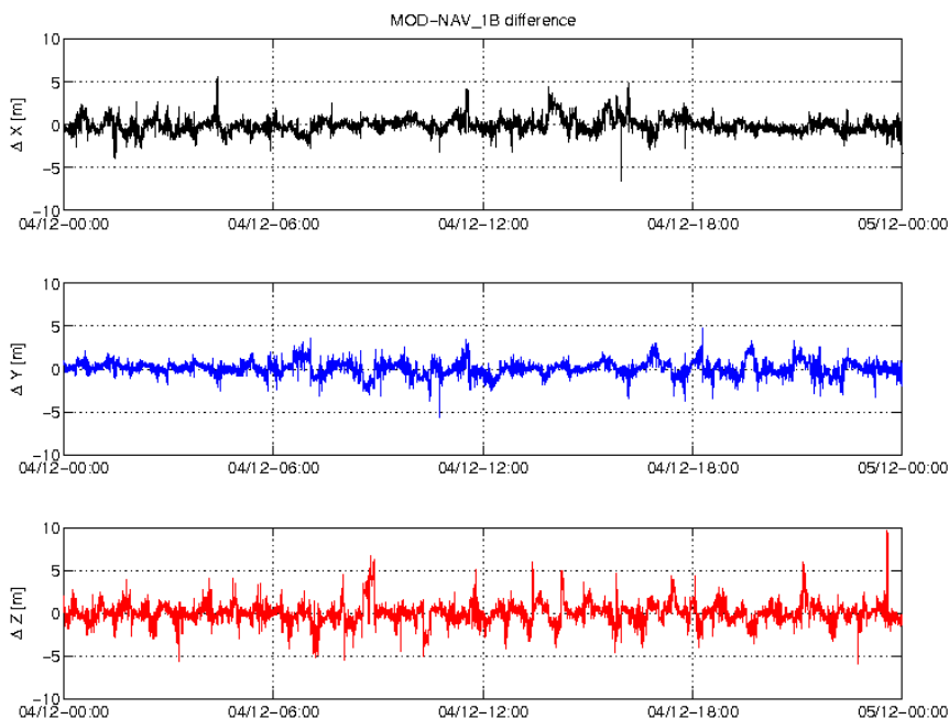
Figure 3-5: Difference MOD-GPSNAV, S/C C, 04/12. From top to bottom: X, Y and Z-axis
