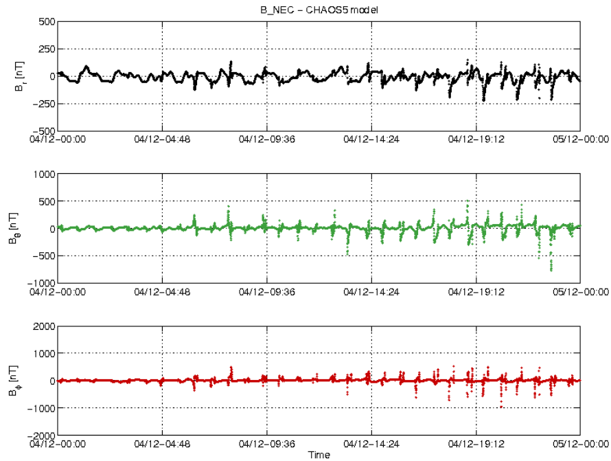
Figure 3-18: S/C A day 04/12: time series of B_{NEC} - B_{Chaos} residuals.
