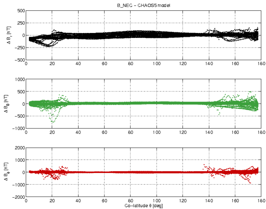
Figure 3-21: S/C C day 04/12 B_{NEC} - B_{Chaos} difference vs colatitude.
