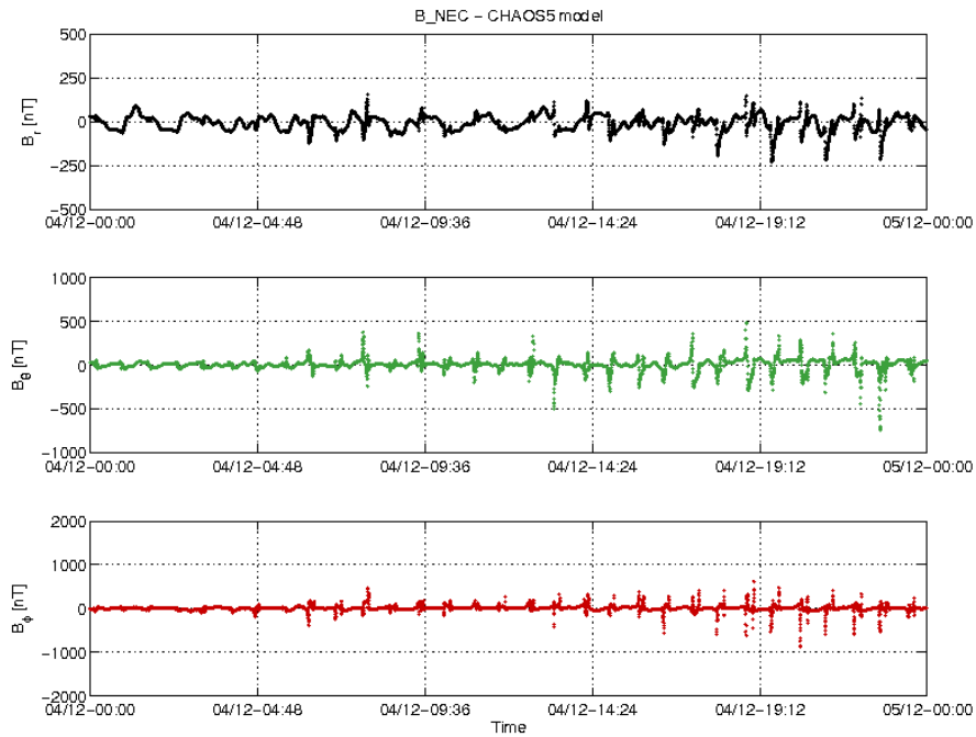
Figure 3-22: S/C C day 04/12 time series of B_{NEC} - B_{Chaos} residuals.
