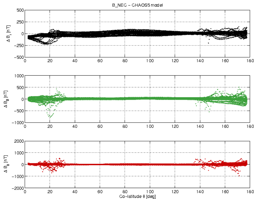
Figure 3-17: S/C A day 04/12 B_{NEC} - B_{Chaos} vs colatitude.
