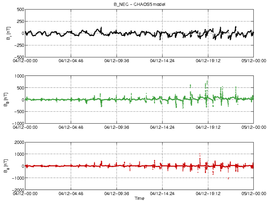
Figure 3-20: S/C B day 04/12 time series of B_{NEC} - B_{Chaos} residuals.
