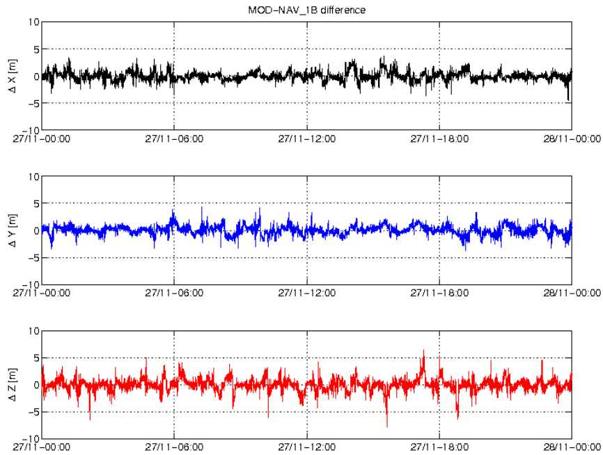
Figure 3-3: Difference MOD-GPSNAV, S/C A, 27/11. From top to bottom: X, Y and Z-axis
