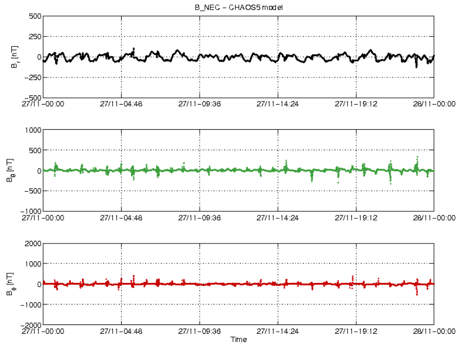
Figure 3-20: S/C B day 27/11 time series of B_{NEC} - B_{Chaos} residuals.
