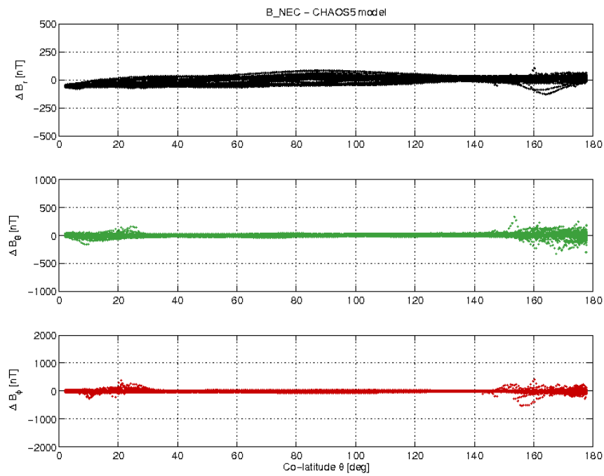
Figure 3-19: S/C B day 27/11 B_{NEC} - B_{Chaos} difference vs colatitude.
