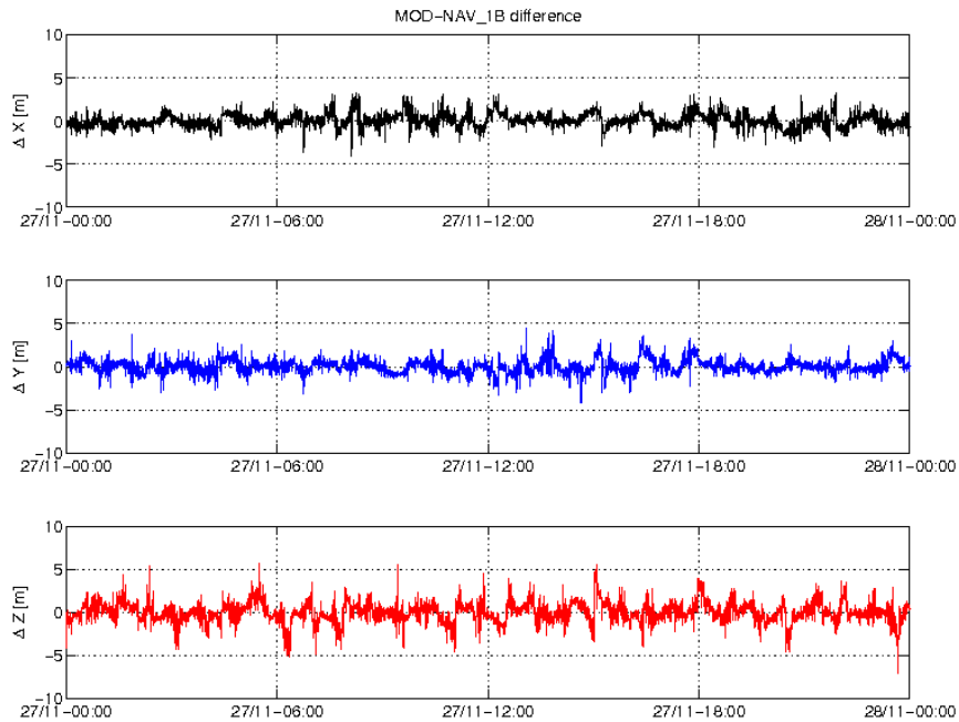
Figure 3-4: Difference MOD-GPSNAV, S/C B, 27/11. From top to bottom: X, Y and Z-axis
