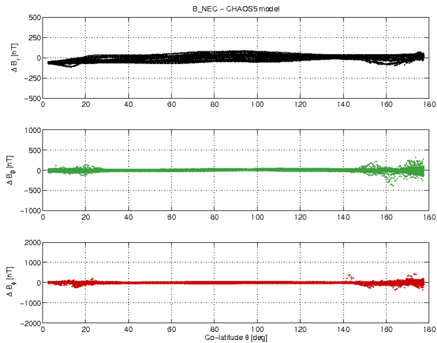
Figure 3-21: S/C C day 27/11 B_{NEC} - B_{Chaos} difference vs colatitude.
