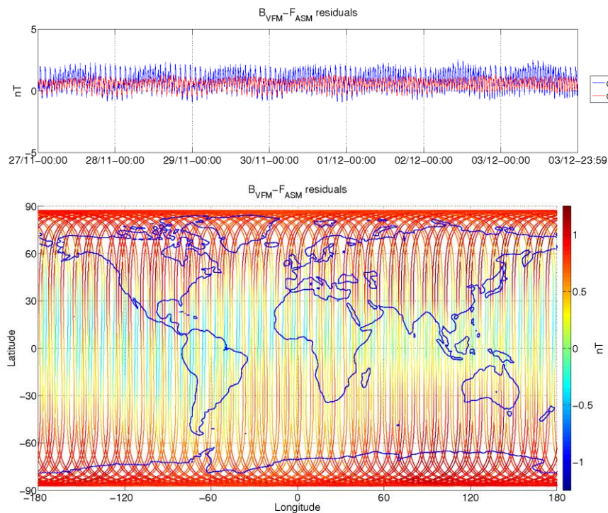
Figure 3-8: ASM-VFM residuals for S/C A, during monitoring period 27/11-03/12. In top figure are plotted: difference between |B_{VFM}| and F_{ASM} (without dB_{Sun} correction) (blue colour), and the residuals with dB_{Sun} corrections (red colour). In bottom figure residuals are presented on the world map.
