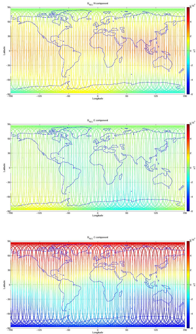
Figure 3-12: S/C C, world map plots of the geomagnetic field and components measured during monitoring period 27/11-03/12. From top to bottom: B_{NEC} components (North, East, and Centre) of magnetic field from VFM measurement.
