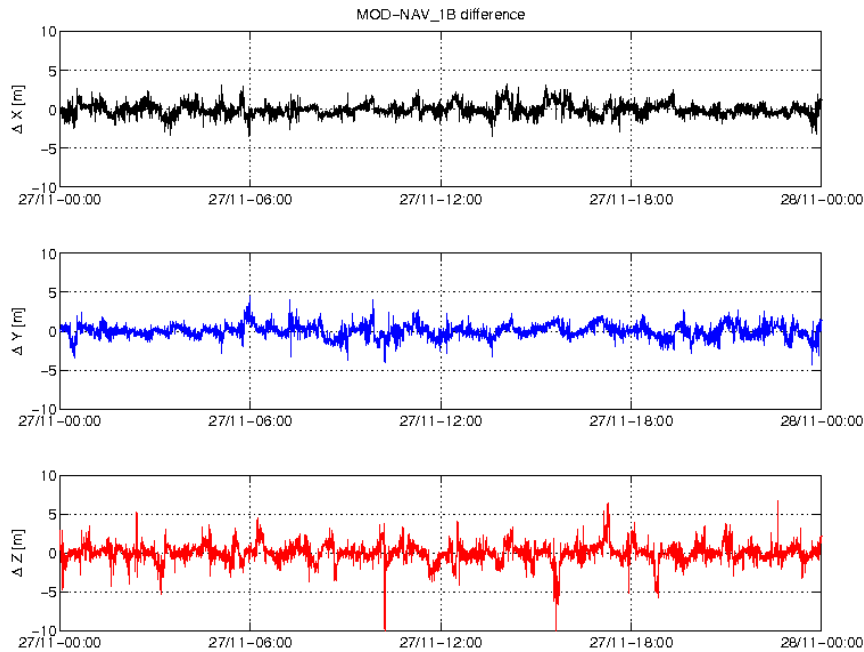
Figure 3-5: Difference MOD-GPSNAV, S/C C, 27/11. From top to bottom: X, Y and Z-axis
