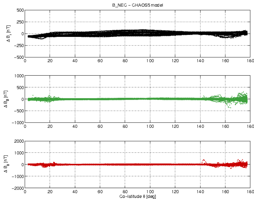
Figure 3-17: S/C A day 27/11 B_{NEC} - B_{Chaos} vs colatitude.
