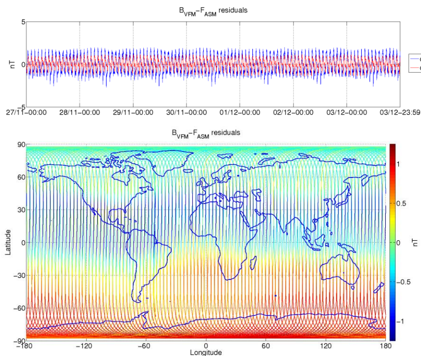
Figure 3-9: ASM-VFM residuals for S/C B, during monitoring period 27/11-03/12. In top figure are plotted: difference between |B_{VFM}| and F_{ASM} (without dB_{Sun} correction) (blue colour), and the residuals with dB_{Sun} corrections (red colour). In bottom figure residuals are presented on the world map.
