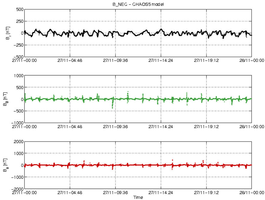
Figure 3-22: S/C C day 27/11 time series of B_{NEC} - B_{Chaos} residuals.
