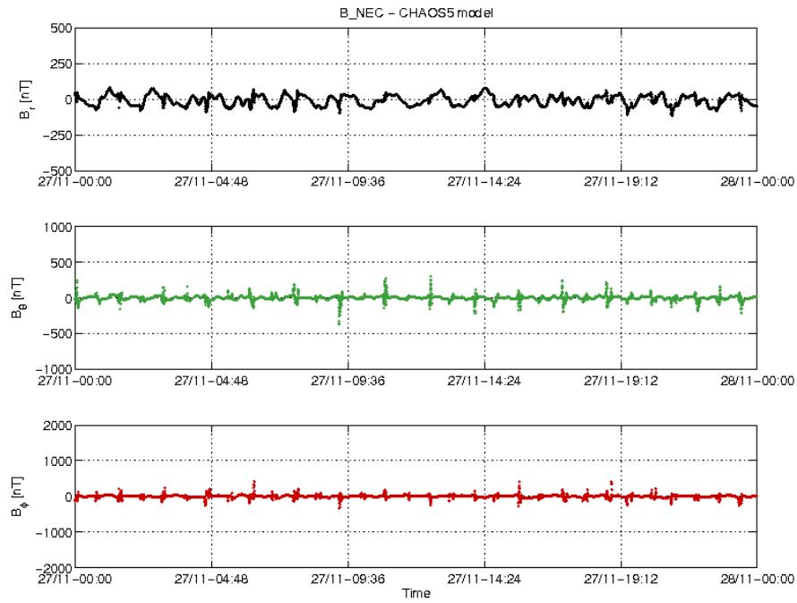
Figure 3-18: S/C A day 27/11: time series of B_{NEC} - B_{Chaos} residuals.
