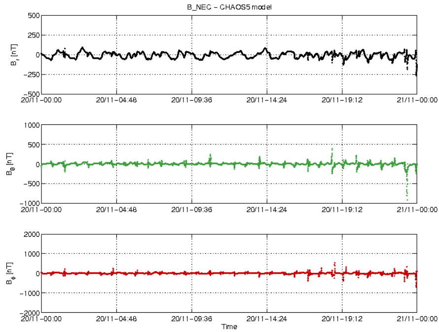
Figure 3-18: S/C A day 20/11: time series of B_{NEC} - B_{Chaos} residuals.
