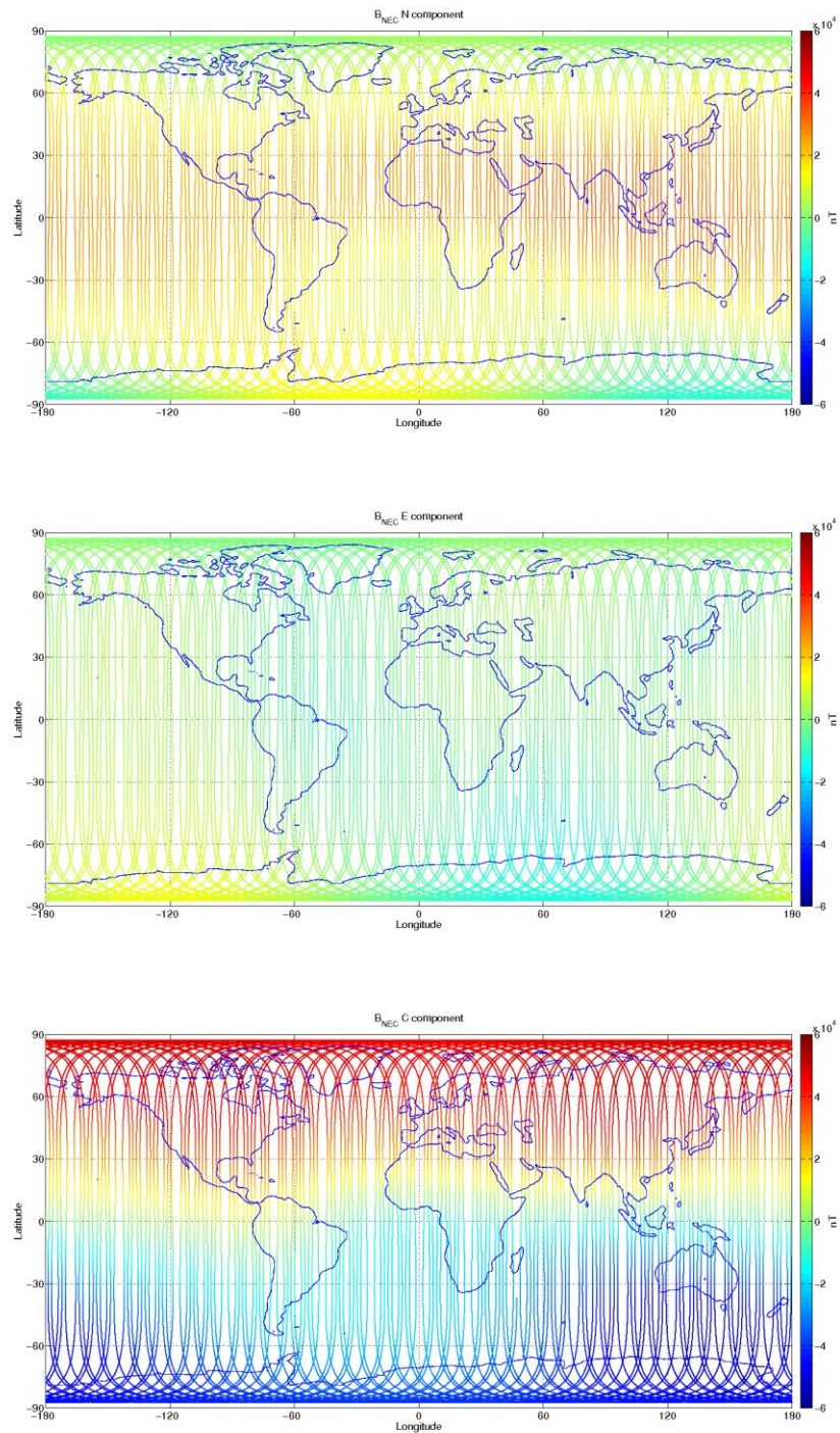
Figure 3-12: S/C C, world map plots of the geomagnetic field and components measured during monitoring period 20/11-26/11. From top to bottom: B NEC components (North, East, and Centre) of magnetic field from VFM measurement.
