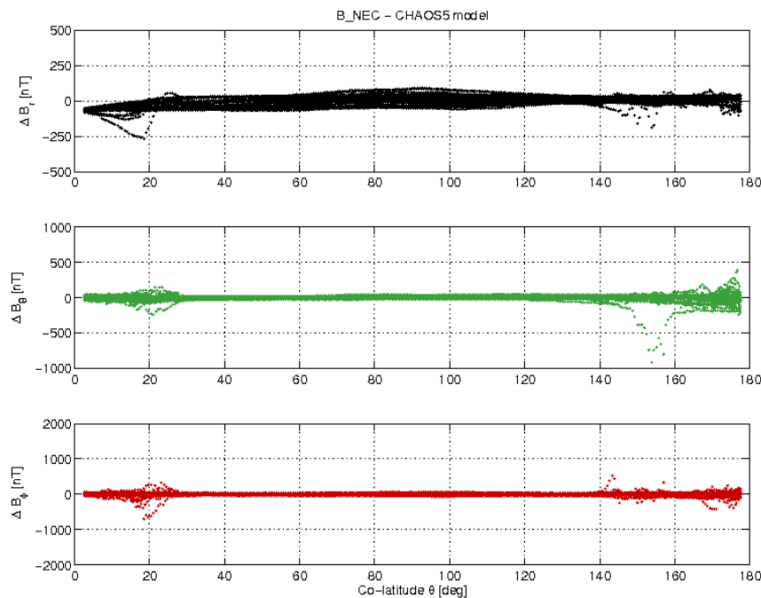
Figure 3-17: S/C A day 20/11 B_{NEC} - B_{Chaos} vs colatitude.
