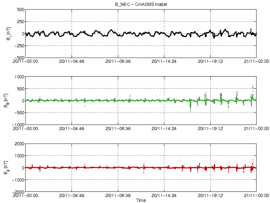
Figure 3-20: S/C B day 20/11 time series of B_{NEC} - B_{Chaos} residuals.
