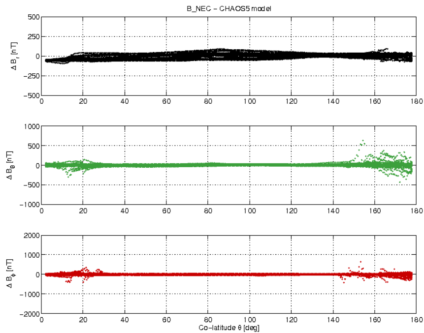
Figure 3-19: S/C B day 20/11 B_{NEC} - B_{Chaos} difference vs colatitude.
