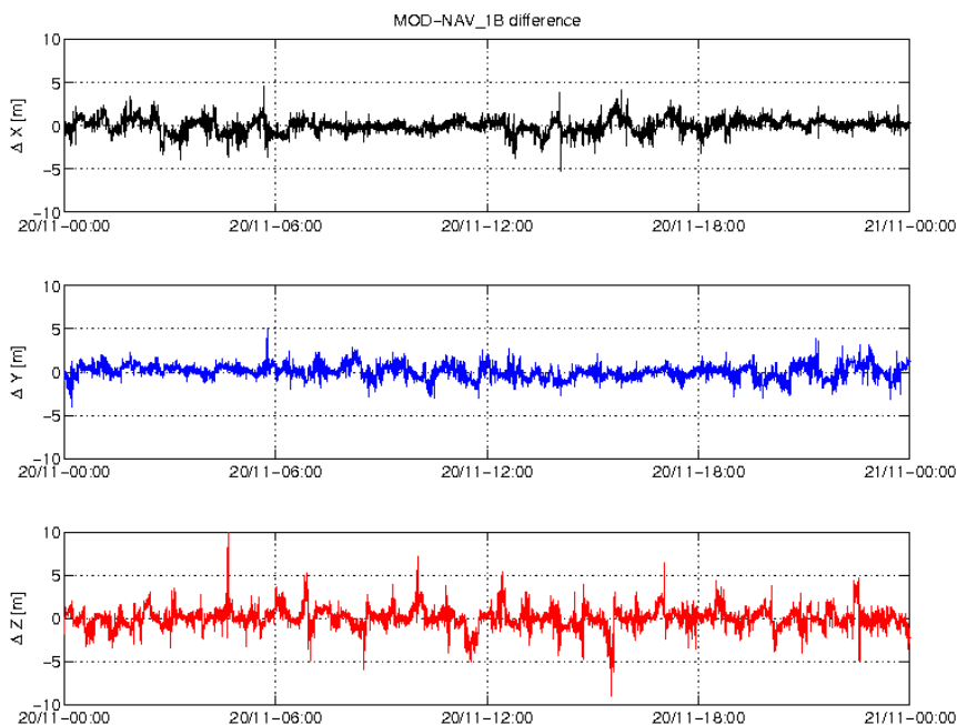
Figure 3-5: Difference MOD-GPSNAV, S/C C, 20/11. From top to bottom: X, Y and Z-axis
