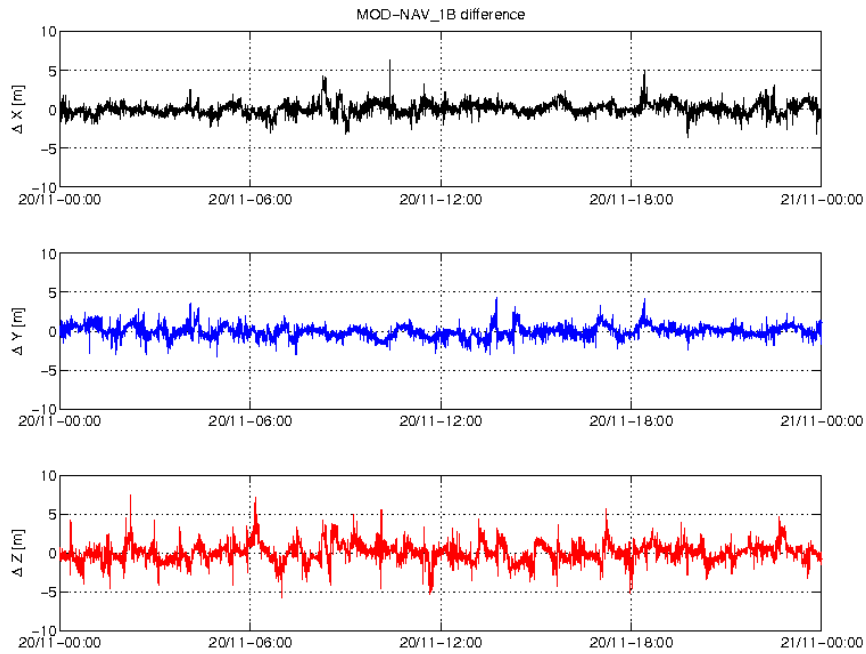
Figure 3-4: Difference MOD-GPSNAV, S/C B, 20/11. From top to bottom: X, Y and Z-axis
