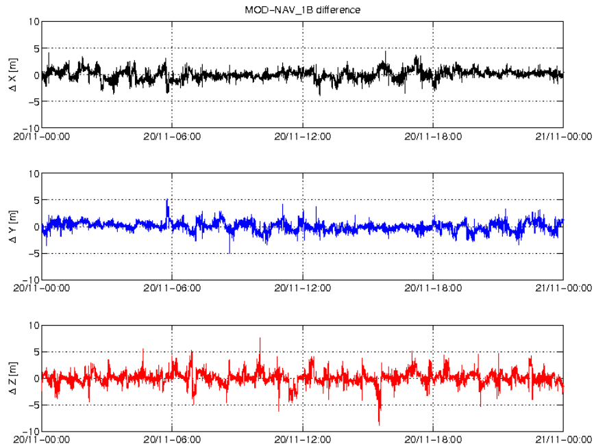
Figure 3-3: Difference MOD-GPSNAV, S/C A, 20/11. From top to bottom: X, Y and Z-axis
