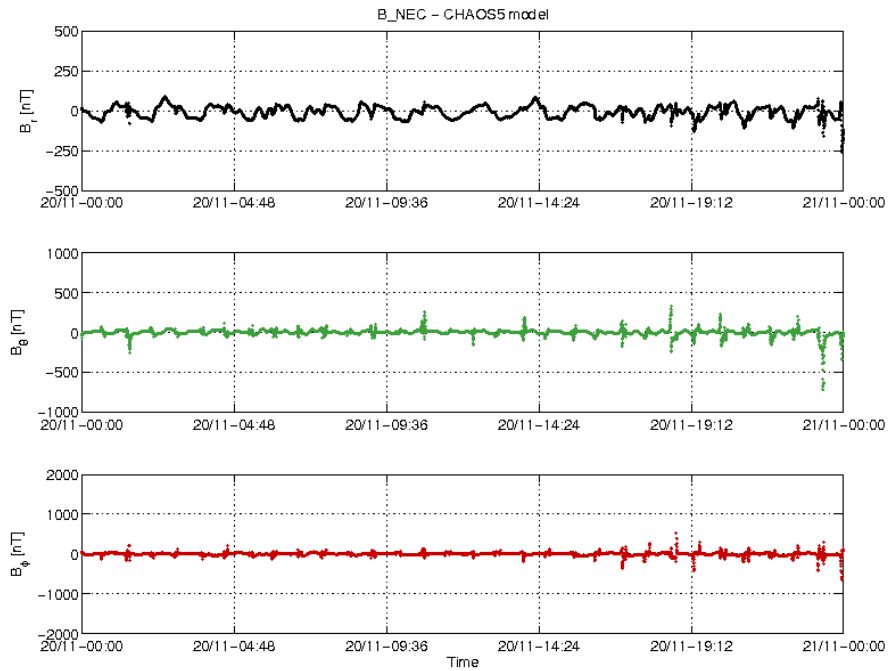
Figure 3-22: S/C C day 20/11 time series of B_{NEC} - B_{Chaos} residuals.
