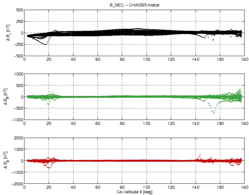
Figure 3-21: S/C C day 20/11 B_{NEC} - B_{Chaos} difference vs colatitude.
