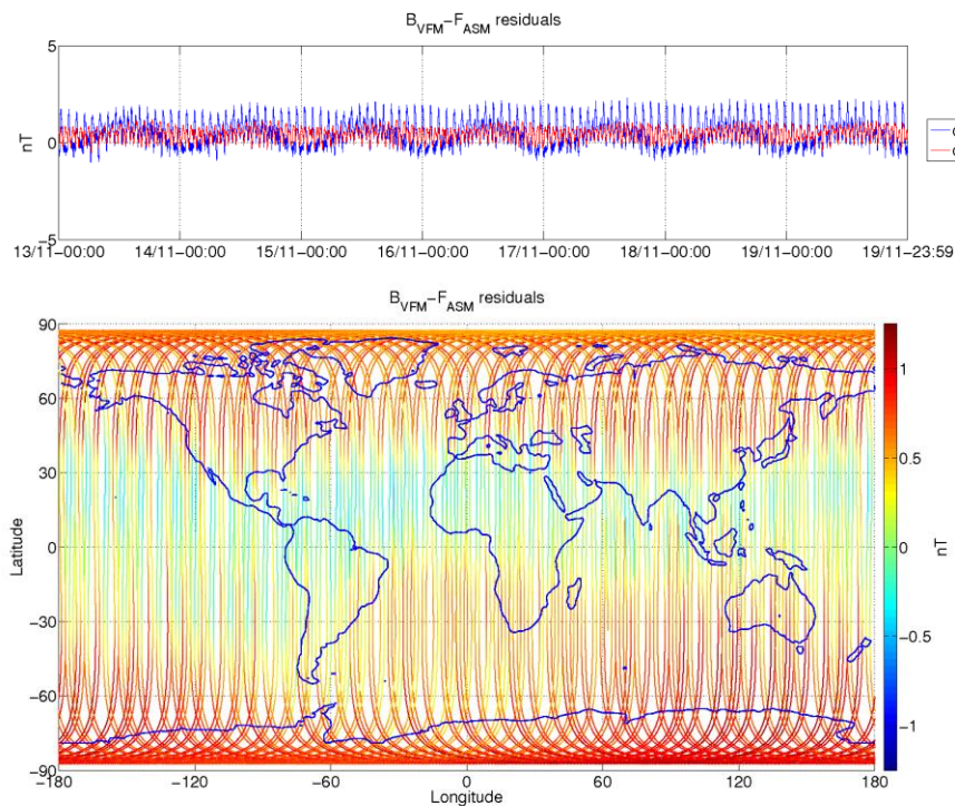
Figure 3-8: ASM-VFM residuals for S/C A, during monitoring period 13/11-19/11. In top figure are plotted: difference between |B_{VFM}| and F_{ASM} (without dB_{Sun} correction) (blue colour), and the residuals with dB_{Sun} corrections (red colour). In bottom figure residuals are presented on the world map.
