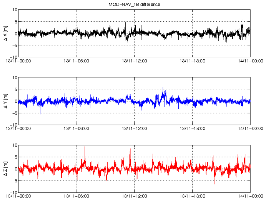
Figure 3-4: Difference MOD-GPSNAV, S/C B, 13/11. From top to bottom: X, Y and Z-axis
