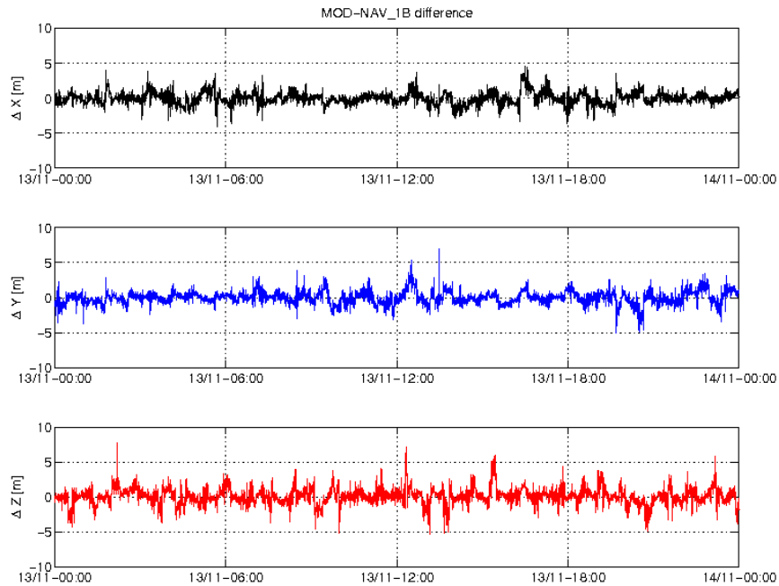
Figure 3-3: Difference MOD-GPSNAV, S/C A, 13/11. From top to bottom: X, Y and Z-axis
