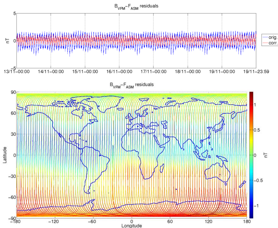
Figure 3-9: ASM-VFM residuals for S/C B, during monitoring period 13/11-19/11. In top figure are plotted: difference between |B_{VFM}| and F_{ASM} (without dB_{Sun} correction) (blue colour), and the residuals with dB_{Sun} corrections (red colour). In bottom figure residuals are presented on the world map.
