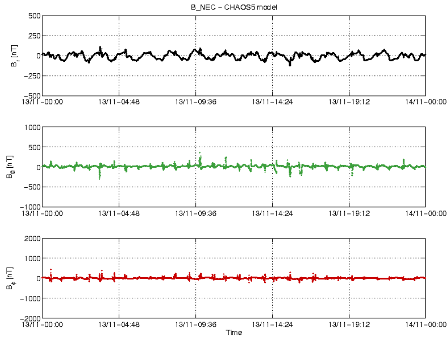
Figure 3-20: S/C B day 13/11 time series of B_{NEC} - B_{Chaos} residuals.
