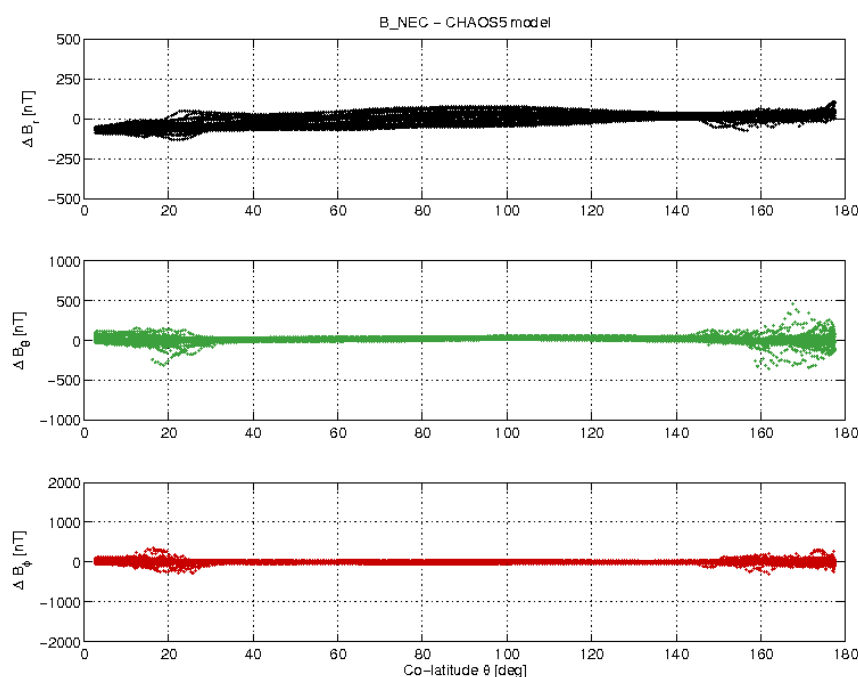
Figure 3-17: S/C A day 13/11 B_{NEC} - B_{Chaos5} vs colatitude.
