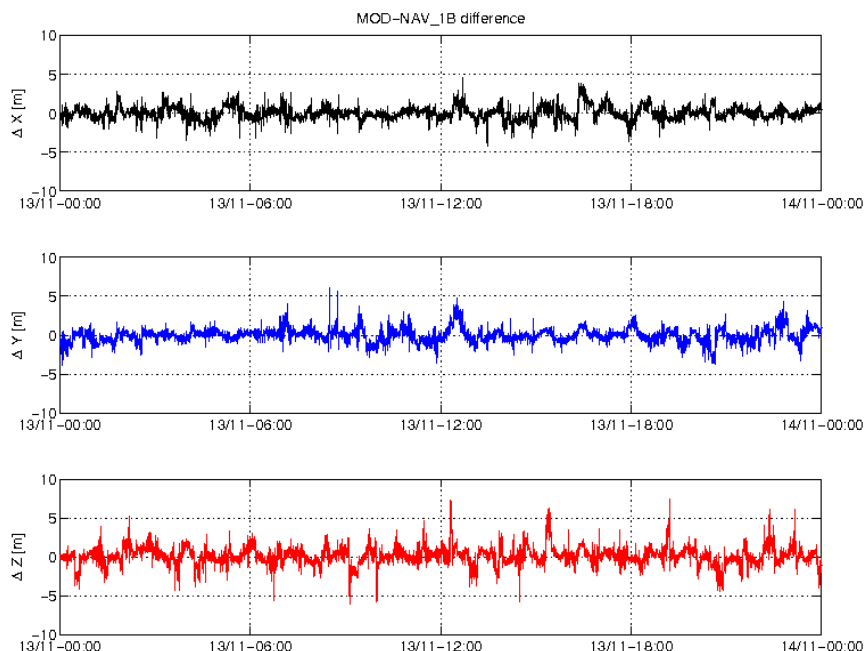
Figure 3-5: Difference MOD-GPSNAV, S/C C, 13/11. From top to bottom: X, Y and Z-axis
