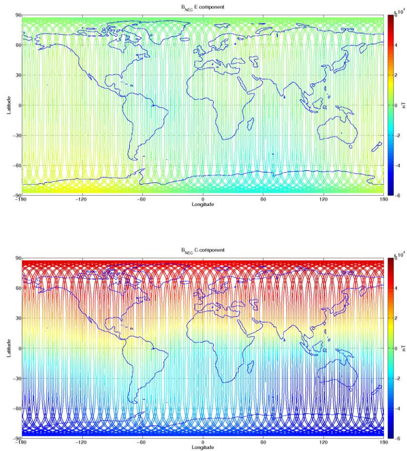
Figure 3-10: S/C A, world map plots of the geomagnetic field and components measured during monitoring period 13/11-19/11. From top to bottom: F-magnetic field from ASM measurement, B_{NEC} components (North, East, and Centre) of magnetic field from VFM measurement.
