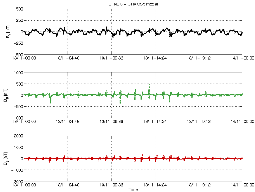
Figure 3-18: S/C A day 13/11: time series of B_{NEC} - B_{Chaos} residuals.
