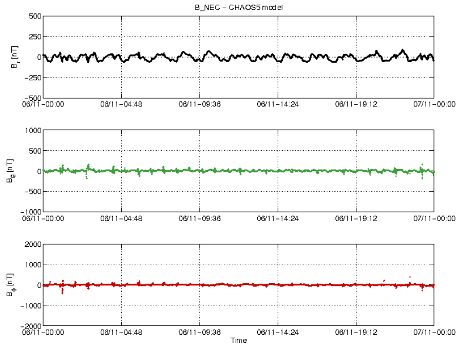
Figure 3-20: S/C B day 06/11 time series of B_{NEC} - B_{Chaos} residuals.
