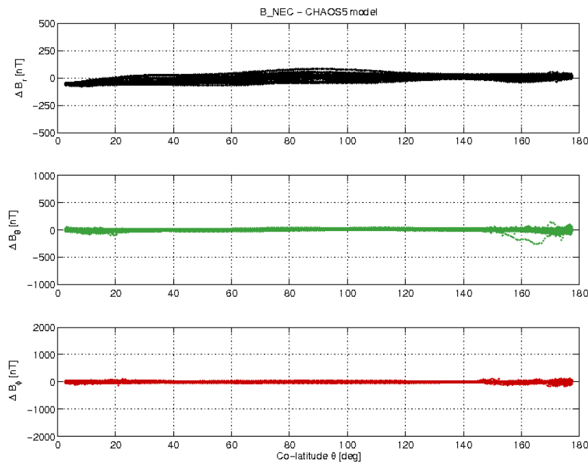
Figure 3-17: S/C A day 06/11 B_{NEC} - B_{Chaos} vs colatitude.
