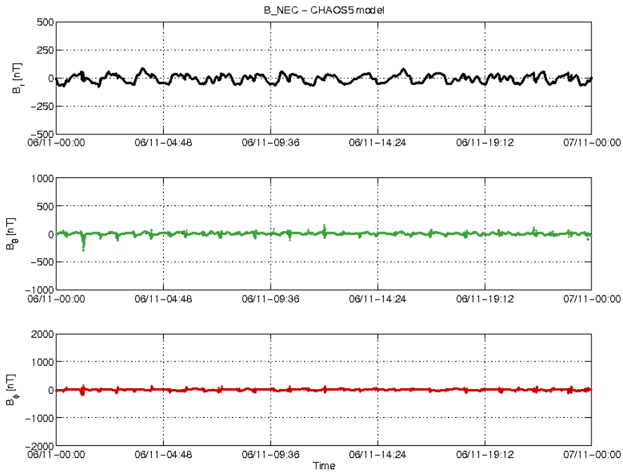
Figure 3-22: S/C C day 06/11 time series of B_{NEC} - B_{Chaos} residuals.
