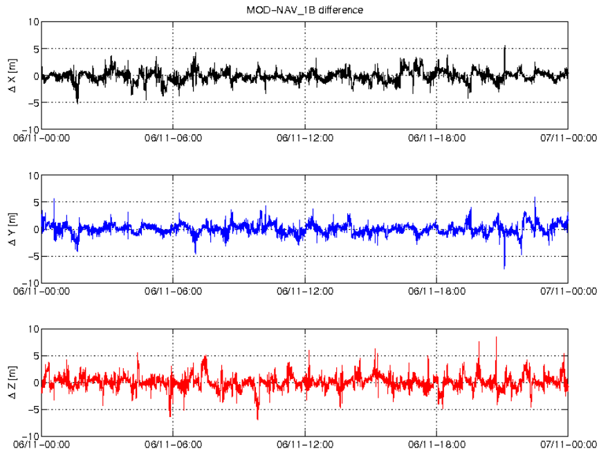
Figure 3-3: Difference MOD-GPSNAV, S/C A, 06/11. From top to bottom: X, Y and Z-axis
