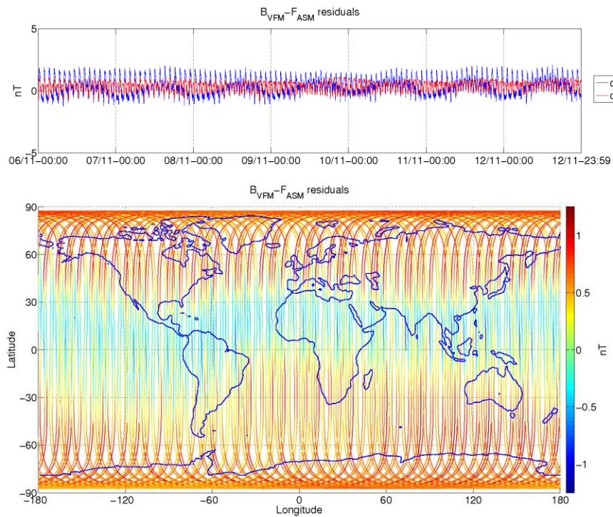
Figure 3-8: ASM-VFM residuals for S/C A, during monitoring period 06/11-12/11. In top figure are plotted: difference between |B_{VFM}| and F_{ASM} (without dB_{Sun} correction) (blue colour), and the residuals with dB_{Sun} corrections (red colour). In bottom figure residuals are presented on the world map.
