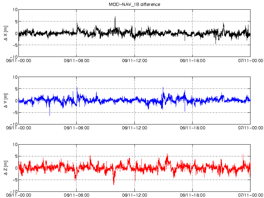
Figure 3-4: Difference MOD-GPSNAV, S/C B, 06/11. From top to bottom: X, Y and Z-axis
