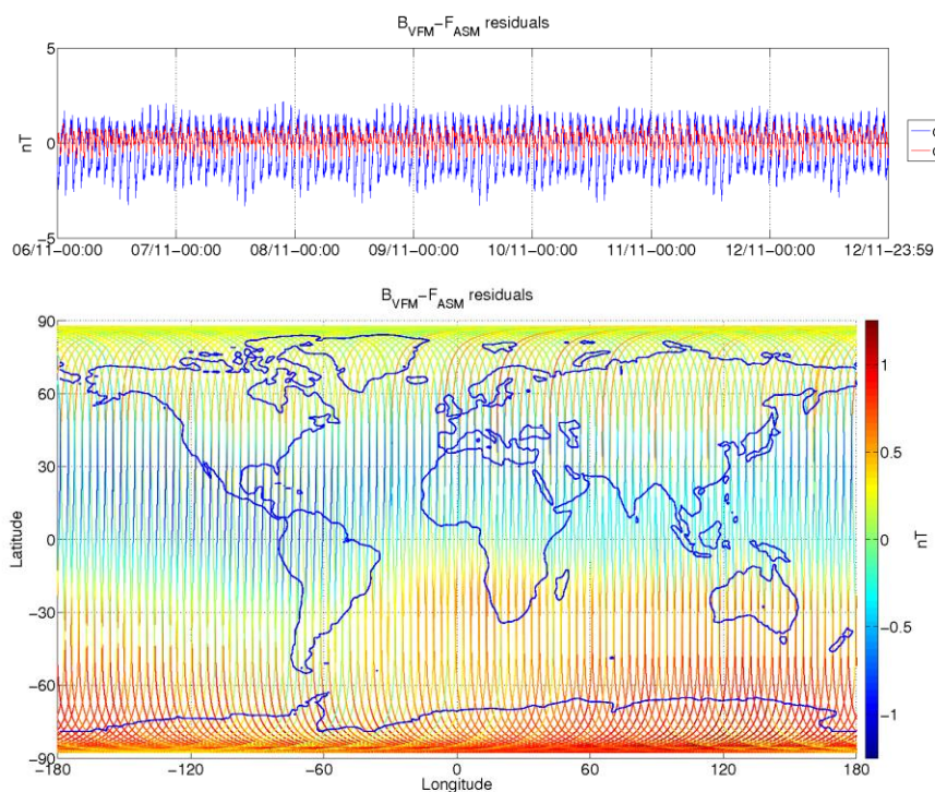
Figure 3-9: ASM-VFM residuals for S/C B, during monitoring period 06/11-12/11. In top figure are plotted: difference between |B VFM | and F ASM (without dB Sun correction) (blue colour), and the residuals with dB Sun corrections (red colour). In bottom figure residuals are presented on the world map.
