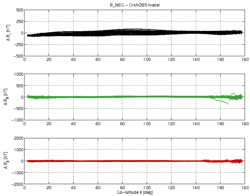
Figure 3-21: S/C C day 06/11 B_{NEC} - B_{Chaos} difference vs colatitude.
