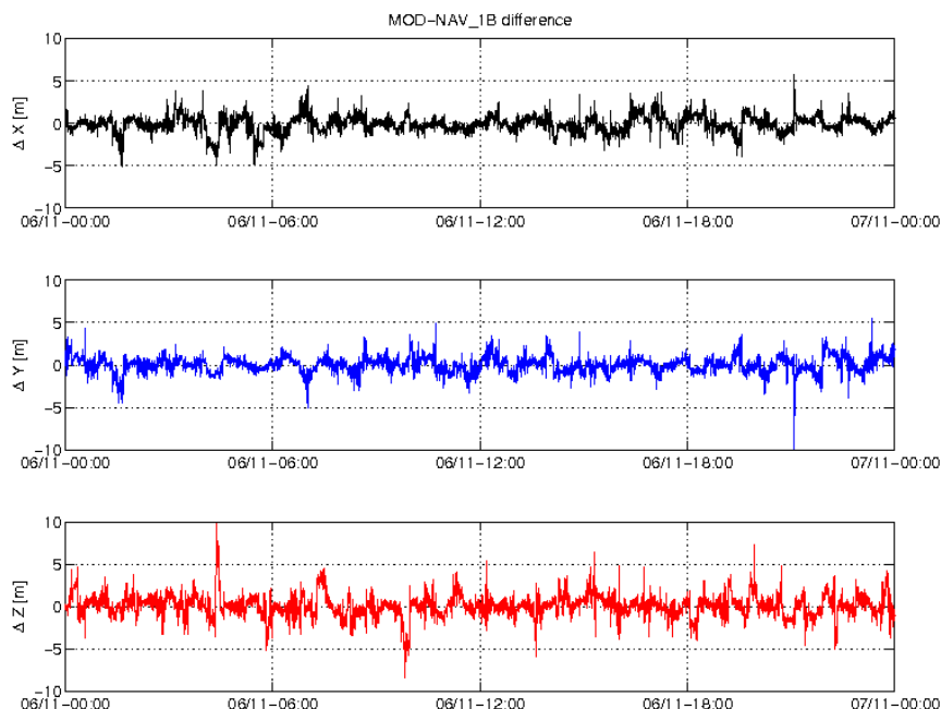
Figure 3-5: Difference MOD-GPSNAV, S/C C, 06/11. From top to bottom: X, Y and Z-axis
