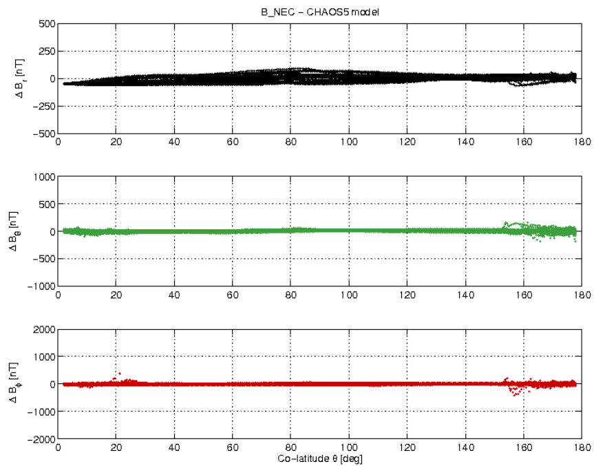
Figure 3-19: S/C B day 06/11 B_{NEC} - B_{Chaos} difference vs colatitude.
