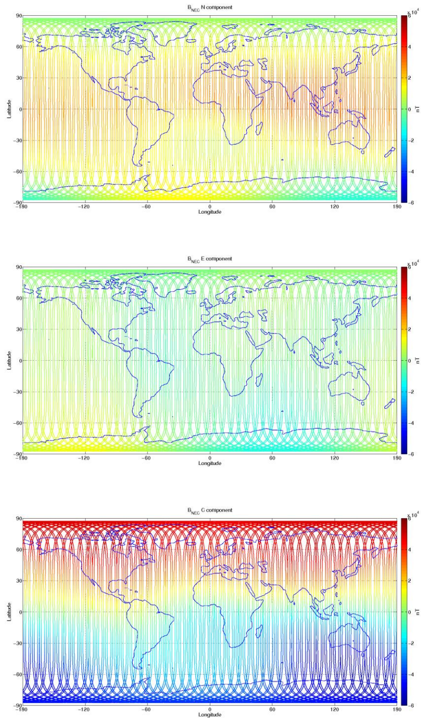
Figure 3-12: S/C C, world map plots of the geomagnetic field and components measured during monitoring period 06/11-12/11. From top to bottom: B_{NEC} components (North, East, and Centre) of magnetic field from VFM measurement.
