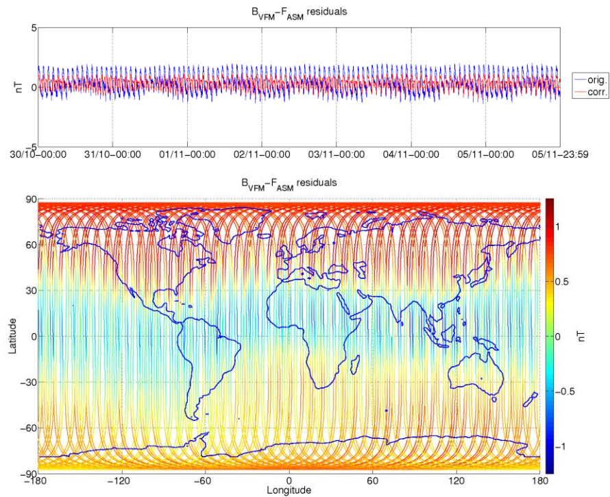
Figure 3-8: ASM-VFM residuals for S/C A, during monitoring period 30/10-05/11. In top figure are plotted: difference between |B_{VFM}| and F_{ASM} (without dB_Sun correction) (blue colour), and the residuals with dB_Sun corrections (red colour). In bottom figure residuals are presented on the world map.
