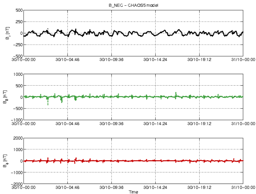
Figure 3-18: S/C A day 30/10: time series of B_{NEC} - B_{Chao5} residuals.
