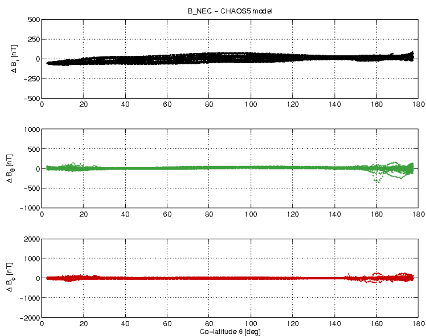
Figure 3-21: S/C C day 30/10 B_{NEC} - B_{Chao5} difference vs colatitude.
