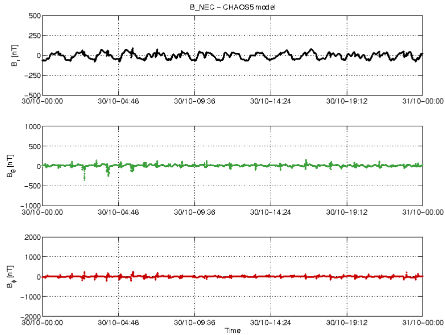
Figure 3-22: S/C C day 30/10 time series of B_{\text{NEC}} - B_{\text{Chaos}} residuals.
