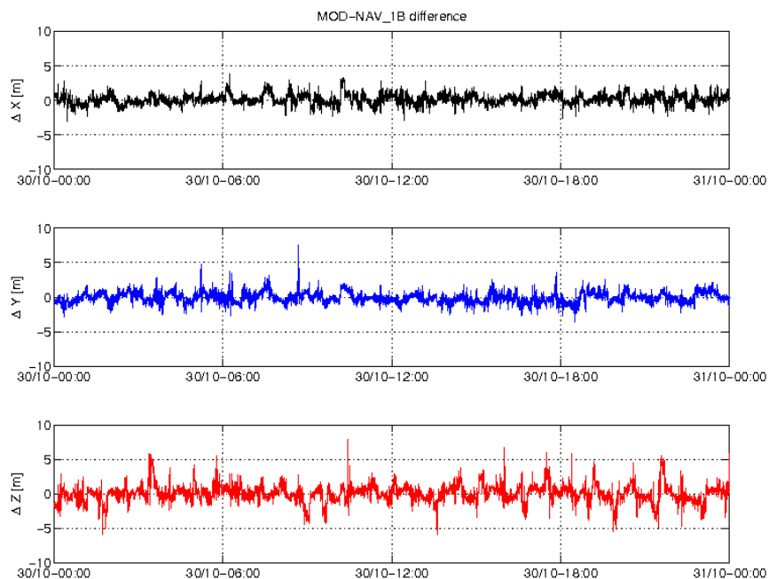
Figure 3-4: Difference MOD-GPSNAV, S/C B, 30/10. From top to bottom: X, Y and Z-axis
