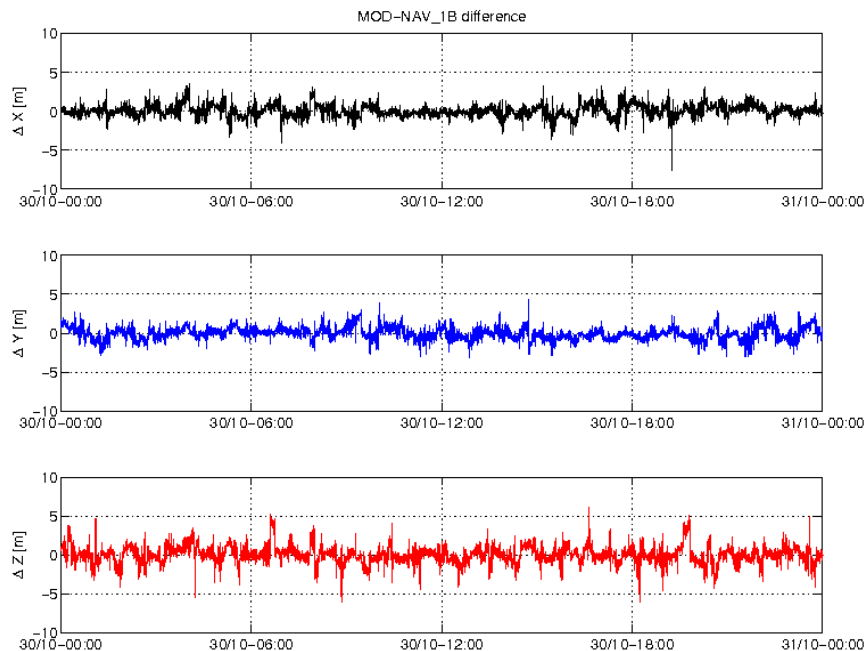
Figure 3-5: Difference MOD-GPSNAV, S/C C, 30/10. From top to bottom: X, Y and Z-axis
