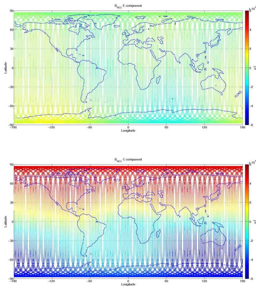
Figure 3-10: S/C A, world map plots of the geomagnetic field and components measured during monitoring period 30/10-05/11. From top to bottom: F-magnetic field from ASM measurement, B NEC components (North, East, and Centre) of magnetic field from VFM measurement.
