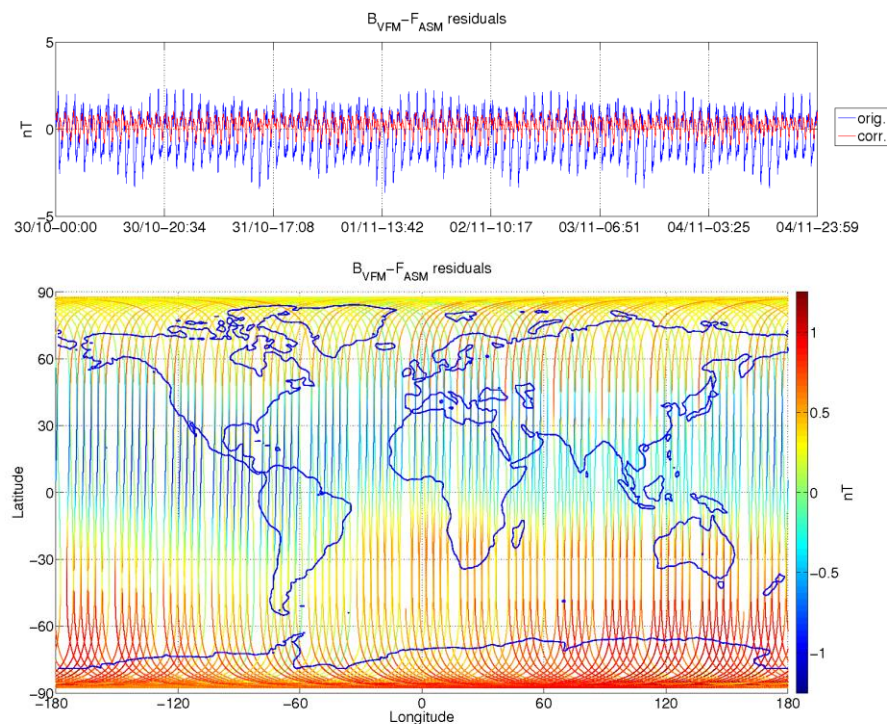
Figure 3-9: ASM-VFM residuals for S/C B, during monitoring period 30/10-05/11. In top figure are plotted: difference between |B_{VFM}| and F_{ASM} (without dB_{Sun} correction) (blue colour), and the residuals with dB_{Sun} corrections (red colour). In bottom figure residuals are presented on the world map.
