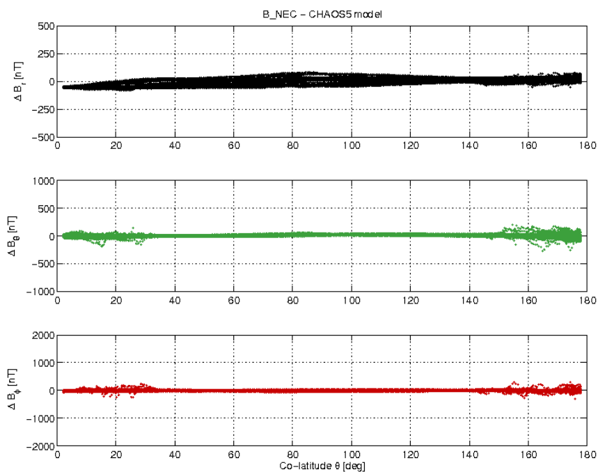
Figure 3-19: S/C B day 30/10 B_{NEC} - B_{Chao5} difference vs colatitude.
