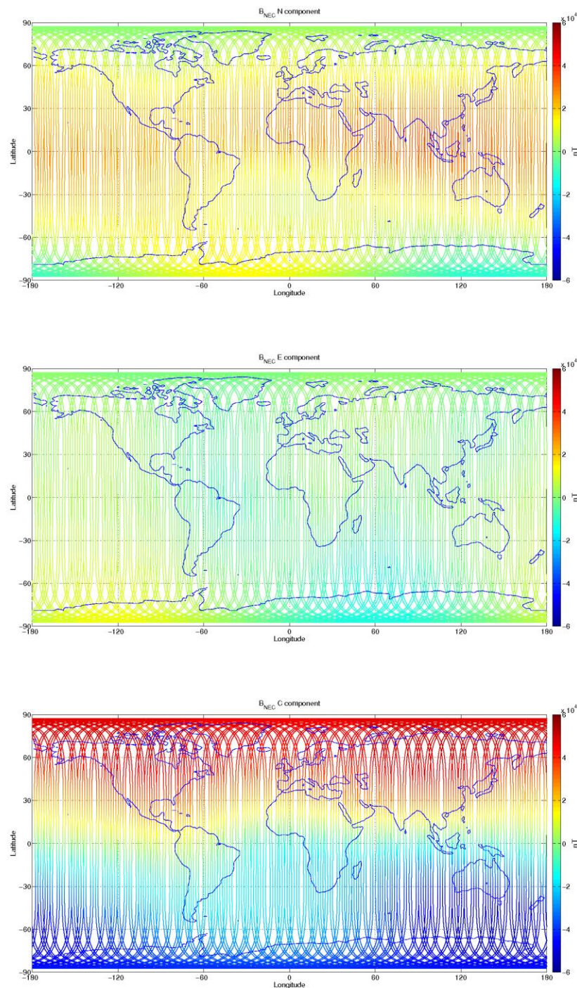
Figure 3-12: S/C C, world map plots of the geomagnetic field and components measured during monitoring period 30/10-05/11. From top to bottom: B_{NEC} components (North, East, and Centre) of magnetic field from VFM measurement.
