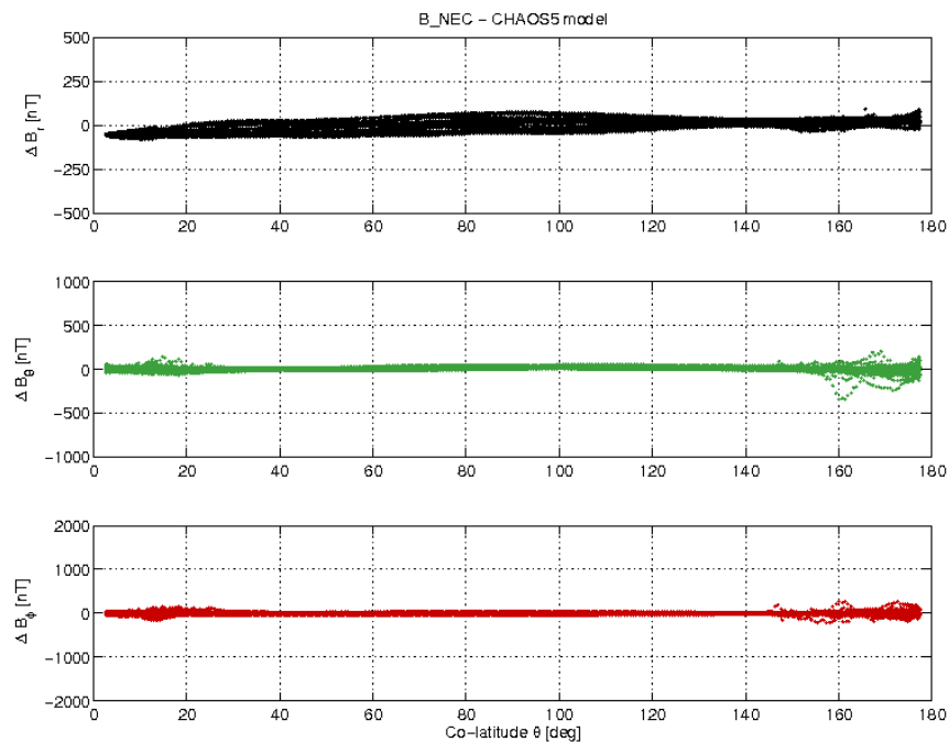
Figure 3-17: S/C A day 30/10 B_{NEC} - B_{Chaos} vs colatitude.
