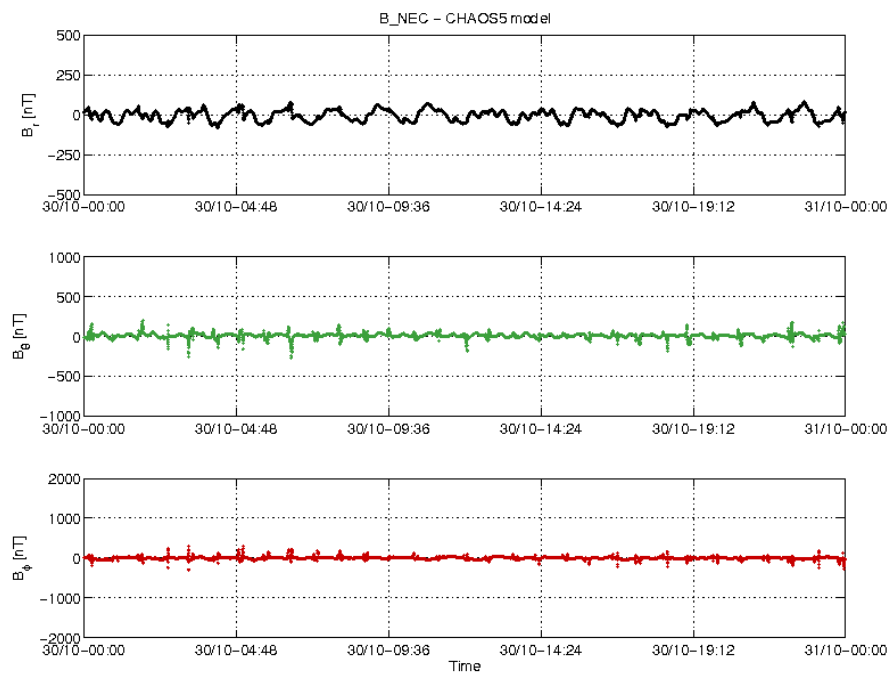
Figure 3-20: S/C B day 30/10 time series of B_{NEC} - B_{Chao5} residuals.
