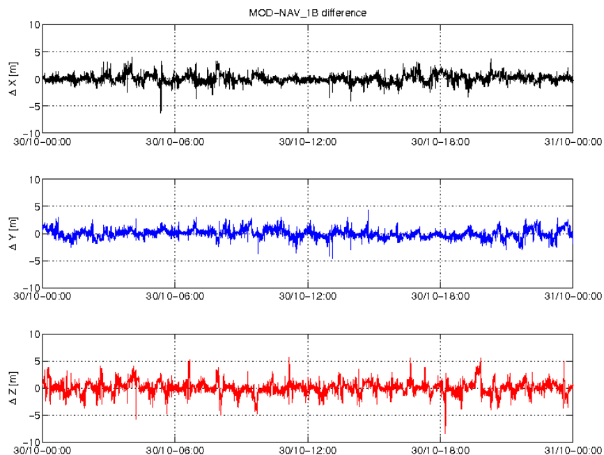
Figure 3-3: Difference MOD-GPSNAV, S/C A, 30/10. From top to bottom: X, Y and Z-axis
