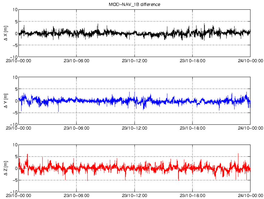
Figure 3-3: Difference MOD-GPSNAV, S/C A, 23/10. From top to bottom: X, Y and Z-axis
