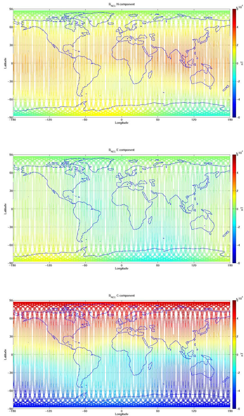
Figure 3-12: S/C C, world map plots of the geomagnetic field and components measured during monitoring period 23/10-29/10. From top to bottom: B_{NEC} components (North, East, and Centre) of magnetic field from VFM measurement.
