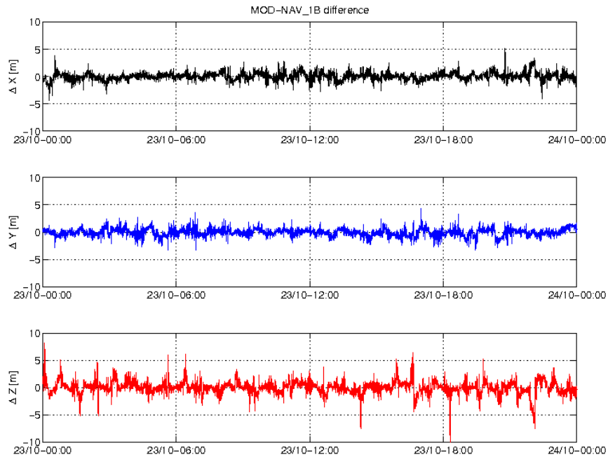
Figure 3-4: Difference MOD-GPSNAV, S/C B, 23/10. From top to bottom: X, Y and Z-axis
