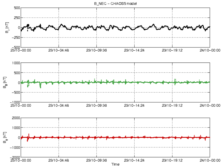
Figure 3-18: S/C A day 23/10: time series of B_{NEC} - B_{Chaos} residuals.
