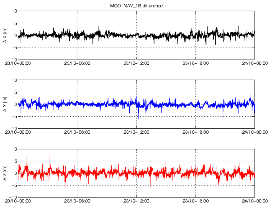
Figure 3-5: Difference MOD-GPSNAV, S/C C, 23/10. From top to bottom: X, Y and Z-axis
