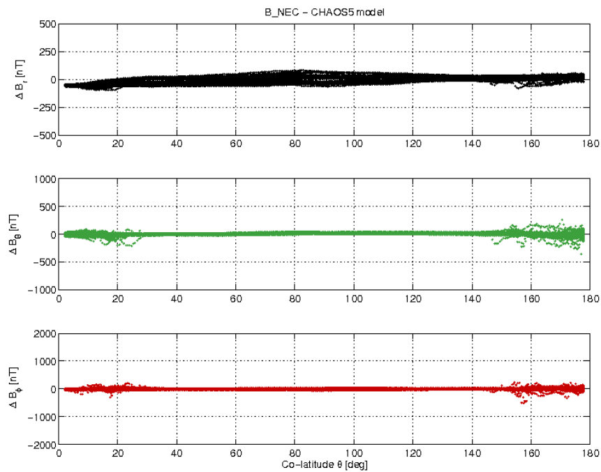
Figure 3-19: S/C B day 23/10 B_{NEC} - B_{Chaos} difference vs colatitude.
