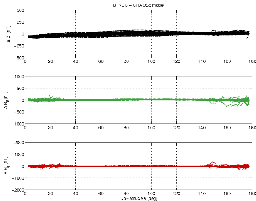
Figure 3-17: S/C A day 23/10 B_{NEC} - B_{Chaos} vs colatitude.
