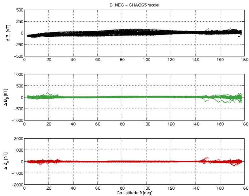
Figure 3-21: S/C C day 23/10 B_{NEC} - B_{Chaos} difference vs colatitude.
