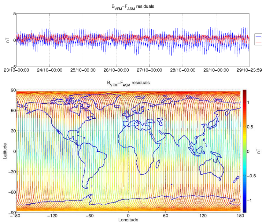
Figure 3-9: ASM-VFM residuals for S/C B, during monitoring period 23/10-29/10. In top figure are plotted: difference between |B_{VFM}| and F_{ASM} (without dB_{Sun} correction) (blue colour), and the residuals with dB_{Sun} corrections (red colour). In bottom figure residuals are presented on the world map.
