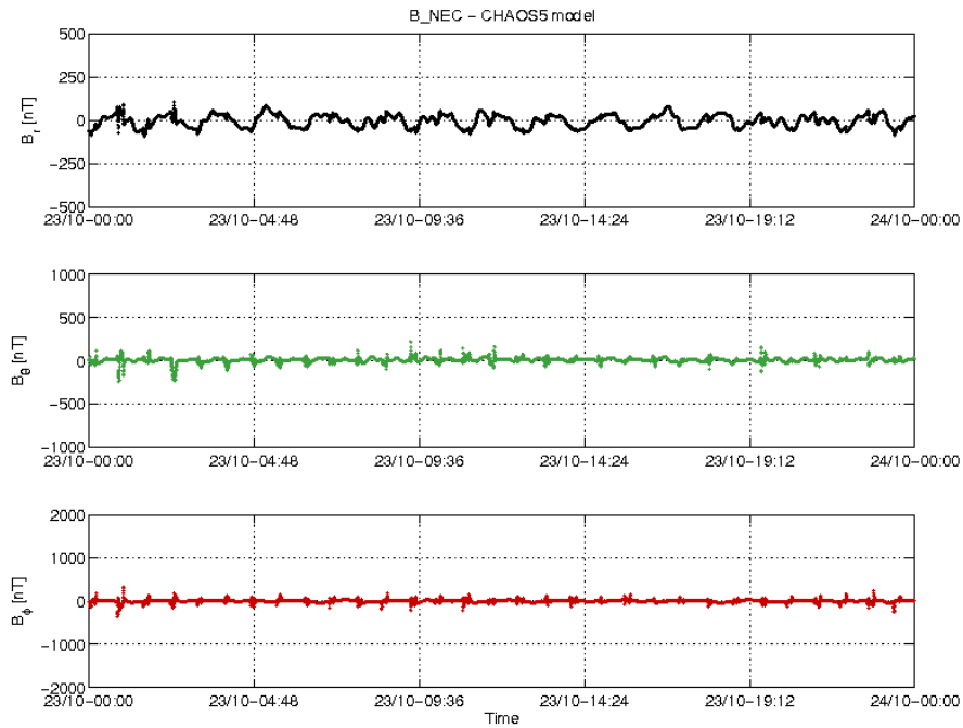
Figure 3-22: S/C C day 23/10 time series of B_{NEC} - B_{Chaos} residuals.
