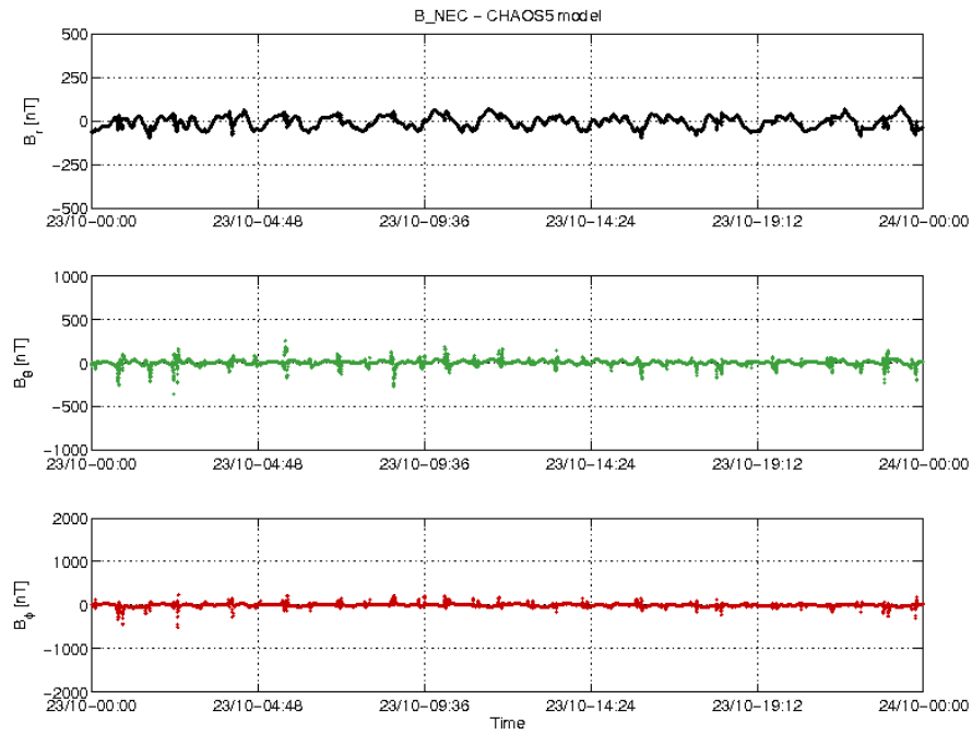
Figure 3-20: S/C B day 23/10 time series of B_{NEC} - B_{Chaos} residuals.
