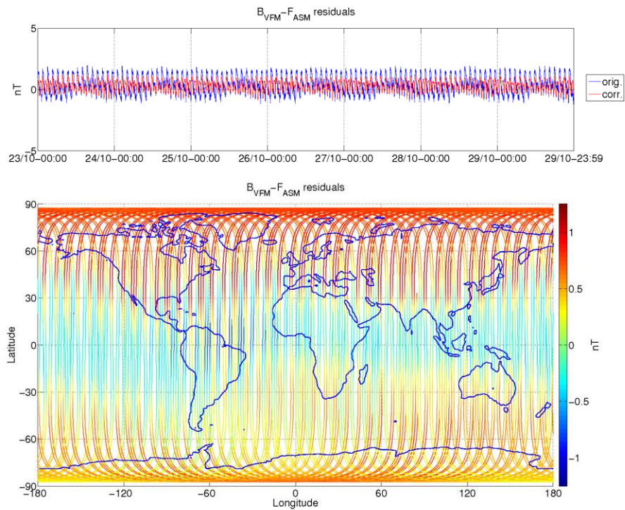
Figure 3-8: ASM-VFM residuals for S/C A, during monitoring period 23/10-29/10. In top figure are plotted: difference between |B_{VFM}| and F_{ASM} (without dB_{Sun} correction) (blue colour), and the residuals with dB_{Sun} corrections (red colour). In bottom figure residuals are presented on the world map.
