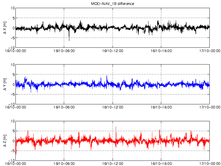
Figure 3-3: Difference MOD-GPSNAV, S/C A, 16/10. From top to bottom: X, Y and Z-axis
