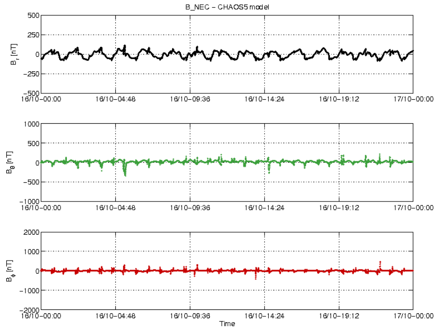
Figure 3-18: S/C A day 16/10: time series of B_{NEC} - B_{Chaos} residuals.
