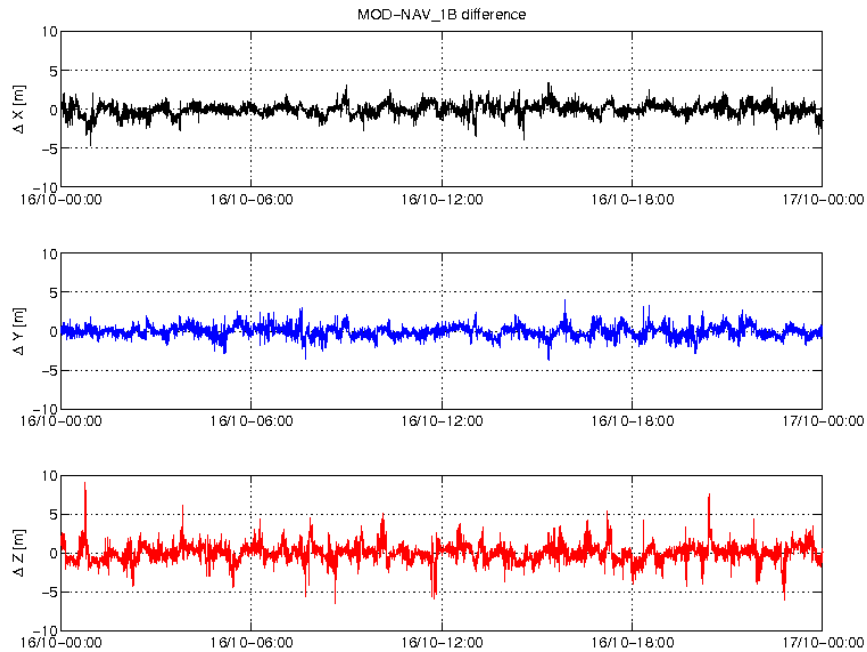
Figure 3-4: Difference MOD-GPSNAV, S/C B, 16/10. From top to bottom: X, Y and Z-axis
