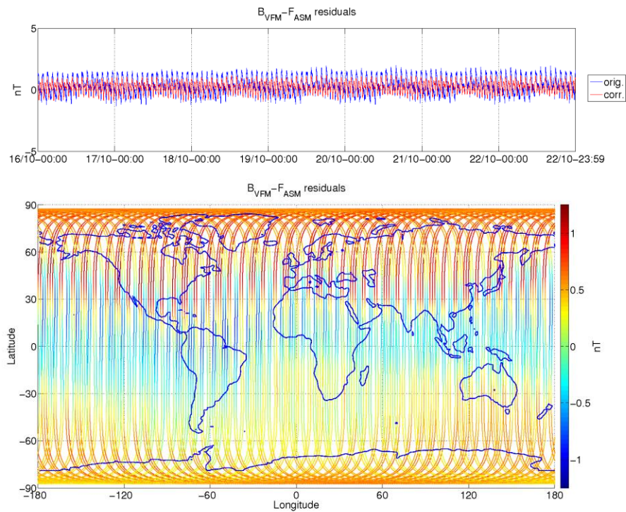
Figure 3-8: ASM-VFM residuals for S/C A, during monitoring period 16/10-22/10. In top figure are plotted: difference between |B_{VFM}| and F_{ASM} (without dB_{Sun} correction) (blue colour), and the residuals with dB_{Sun} corrections (red colour). In bottom figure residuals are presented on the world map.
