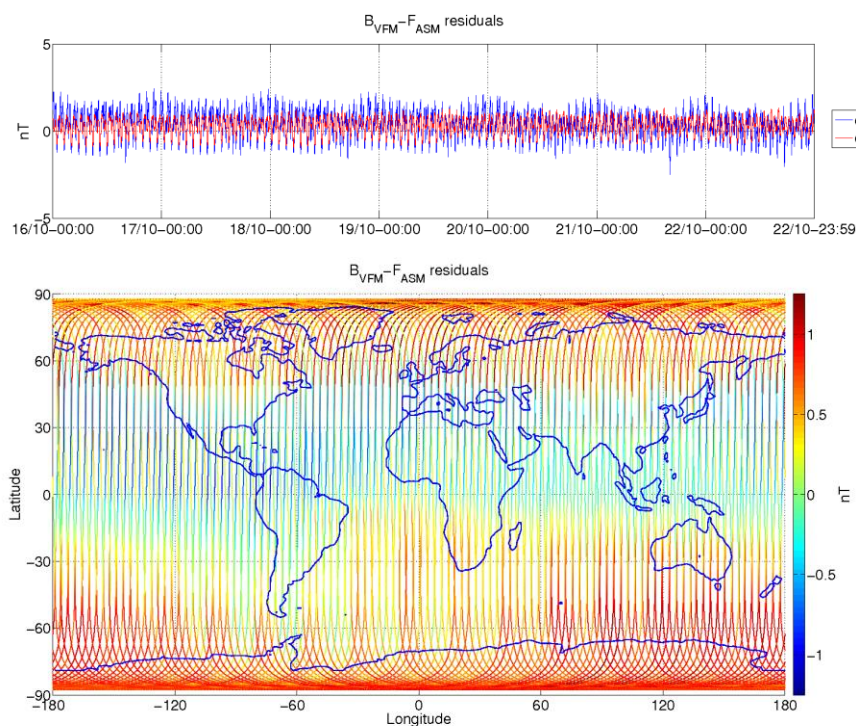
Figure 3-9: ASM-VFM residuals for S/C B, during monitoring period 16/10-22/10. In top figure are plotted: difference between |B_{VFM}| and F_{ASM} (without dB_{Sun} correction) (blue colour), and the residuals with dB_{Sun} corrections (red colour). In bottom figure residuals are presented on the world map.
