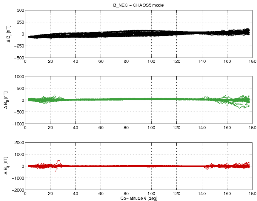
Figure 3-17: S/C A day 16/10 B_{NEC} - B_{Chaos} vs colatitude.
