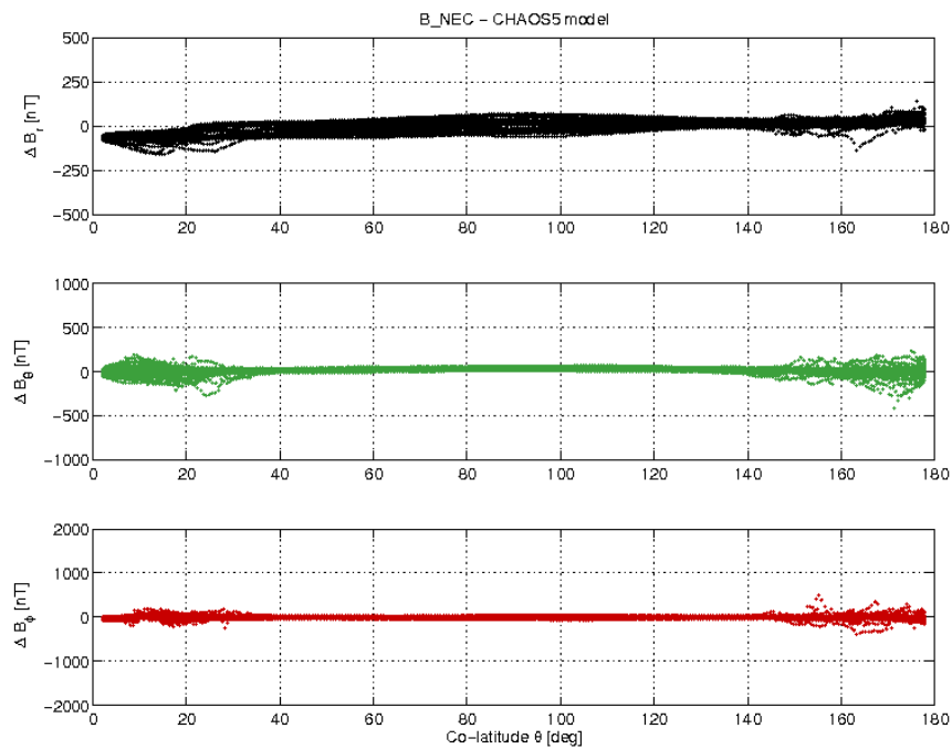
Figure 3-19: S/C B day 16/10 B_{NEC} - B_{Chaos} difference vs colatitude.
