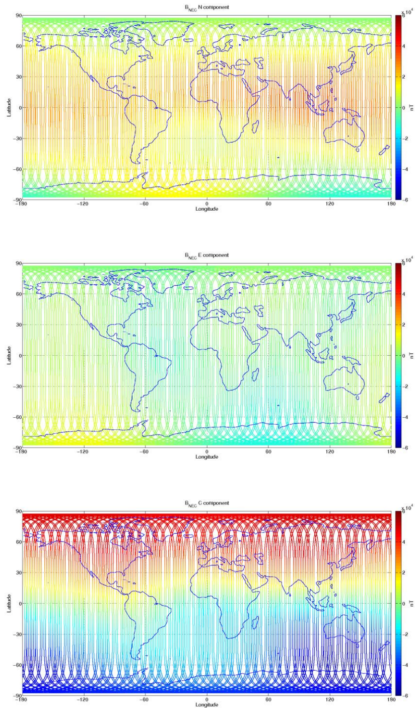
Figure 3-12: S/C C, world map plots of the geomagnetic field and components measured during monitoring period 16/10-22/10. From top to bottom: B NEC components (North, East, and Centre) of magnetic field from VFM measurement.
