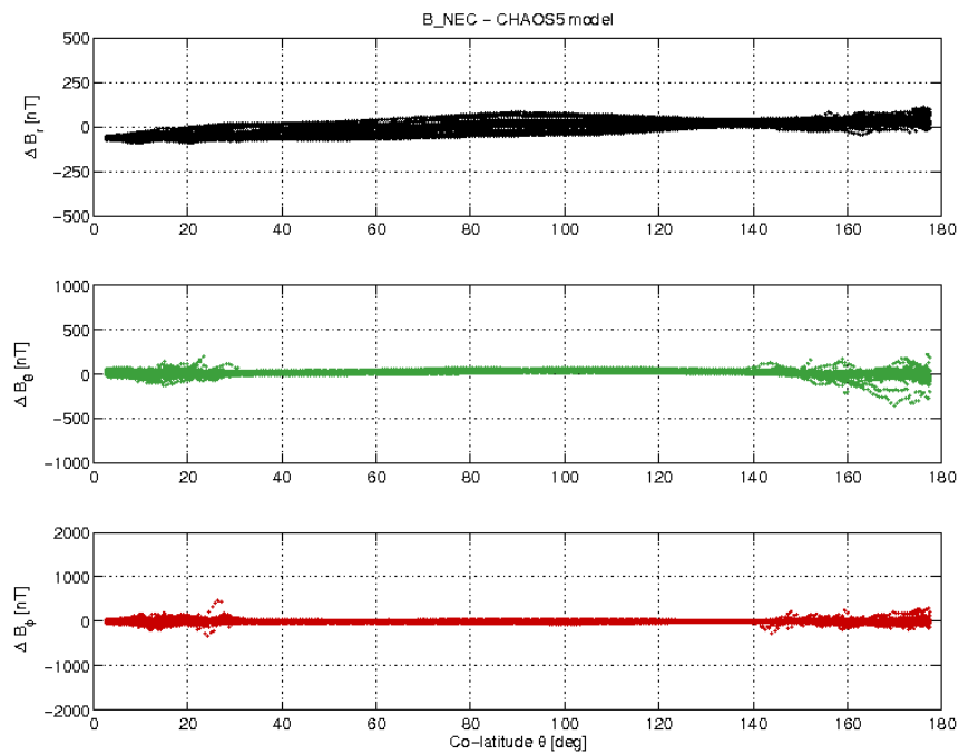
Figure 3-21: S/C C day 16/10 B_{NEC} - B_{Chaos} difference vs colatitude.
