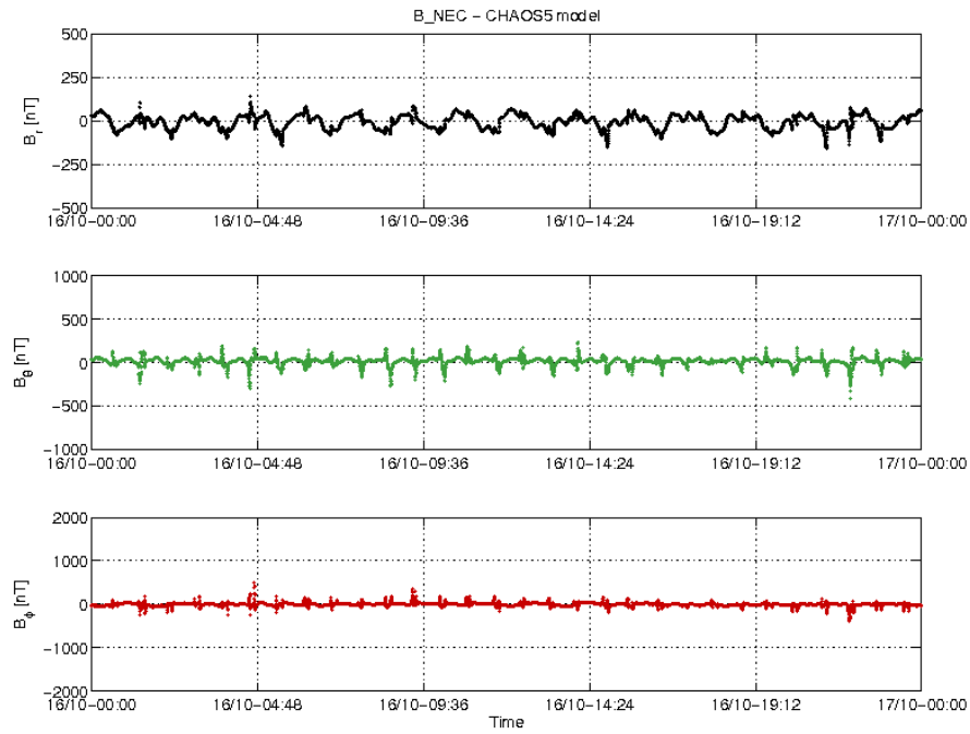
Figure 3-20: S/C B day 16/10 time series of B_{NEC} - B_{Chaos} residuals.
