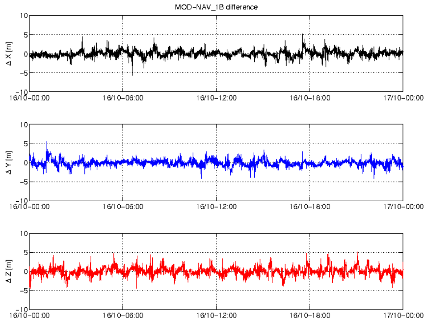
Figure 3-5: Difference MOD-GPSNAV, S/C C, 16/10. From top to bottom: X, Y and Z-axis
