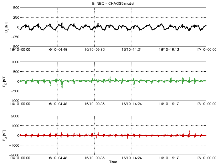
Figure 3-22: S/C C day 16/10 time series of B_{NEC} - B_{Chaos} residuals.
