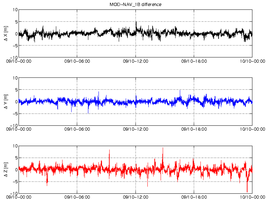
Figure 3-4: Difference MOD-GPSNAV, S/C B, 09/10. From top to bottom: X, Y and Z-axis
