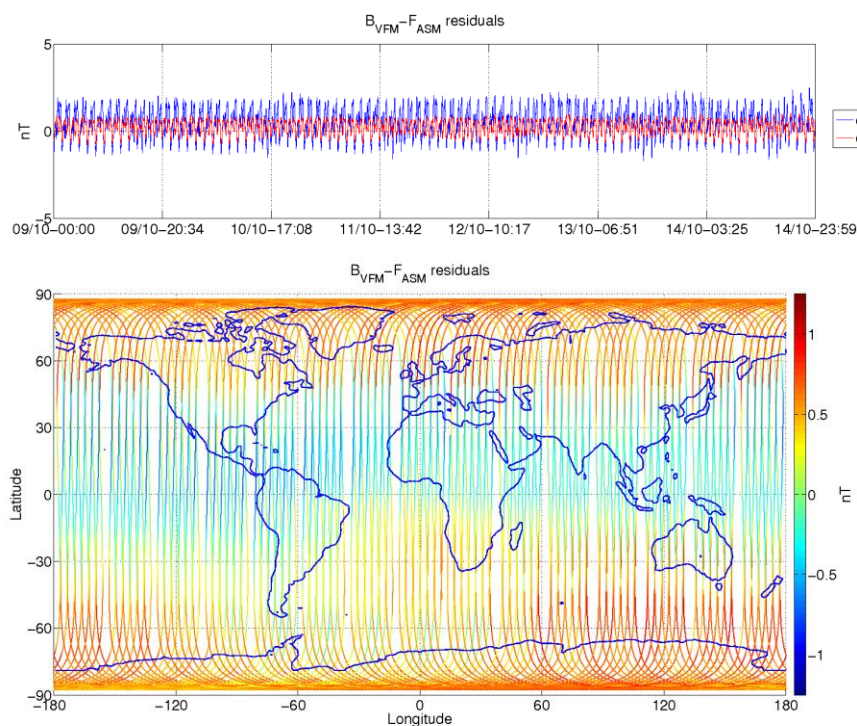
Figure 3-9: ASM-VFM residuals for S/C B, during monitoring period 09/10-15/10. In top figure are plotted: difference between |B_{VFM}| and F_{ASM} (without dB_{Sun} correction) (blue colour), and the residuals with dB_{Sun} corrections (red colour). In bottom figure residuals are presented on the world map.
