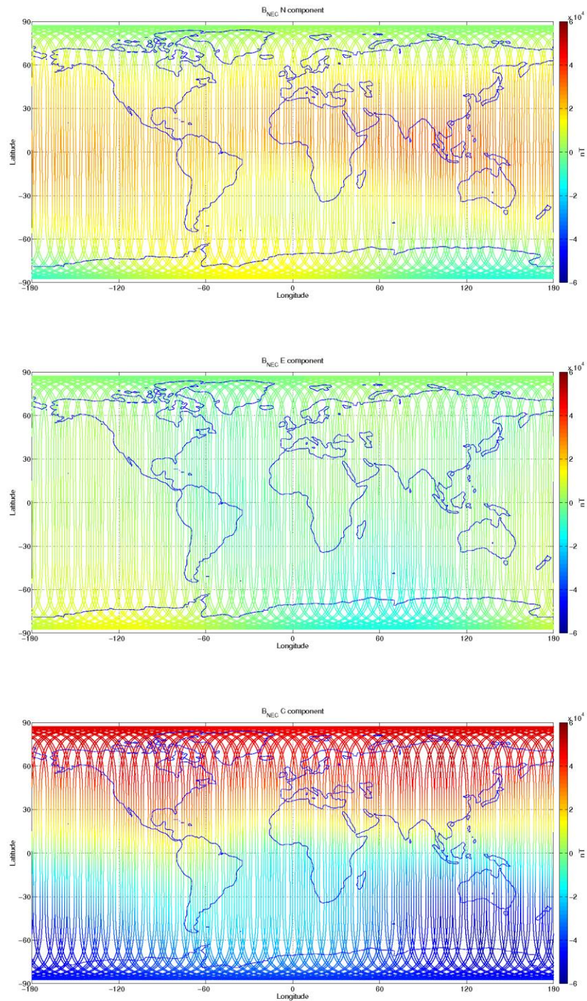
Figure 3-12: S/C C, world map plots of the geomagnetic field and components measured during monitoring period 09/10-15/10. From top to bottom: B NEC components (North, East, and Centre) of magnetic field from VFM measurement.
