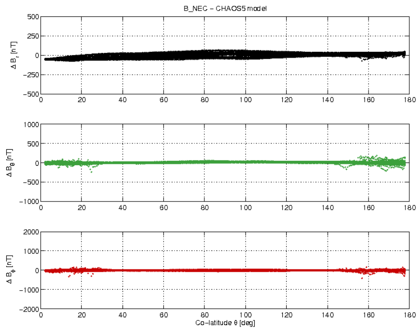
Figure 3-19: S/C B day 09/10 B_{NEC} - B_{Chaos} difference vs colatitude.
