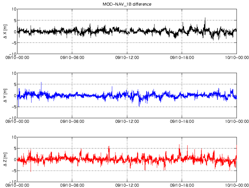
Figure 3-5: Difference MOD-GPSNAV, S/C C, 09/10. From top to bottom: X, Y and Z-axis
