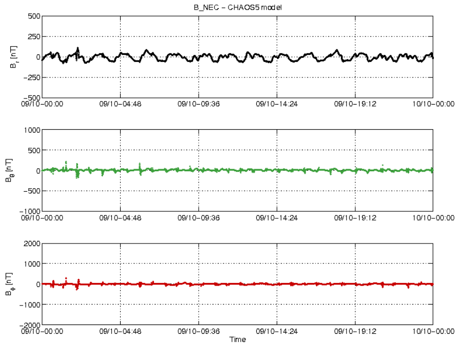
Figure 3-22: S/C C day 09/10 time series of B_{NEC} - B_{Chaos} residuals.
