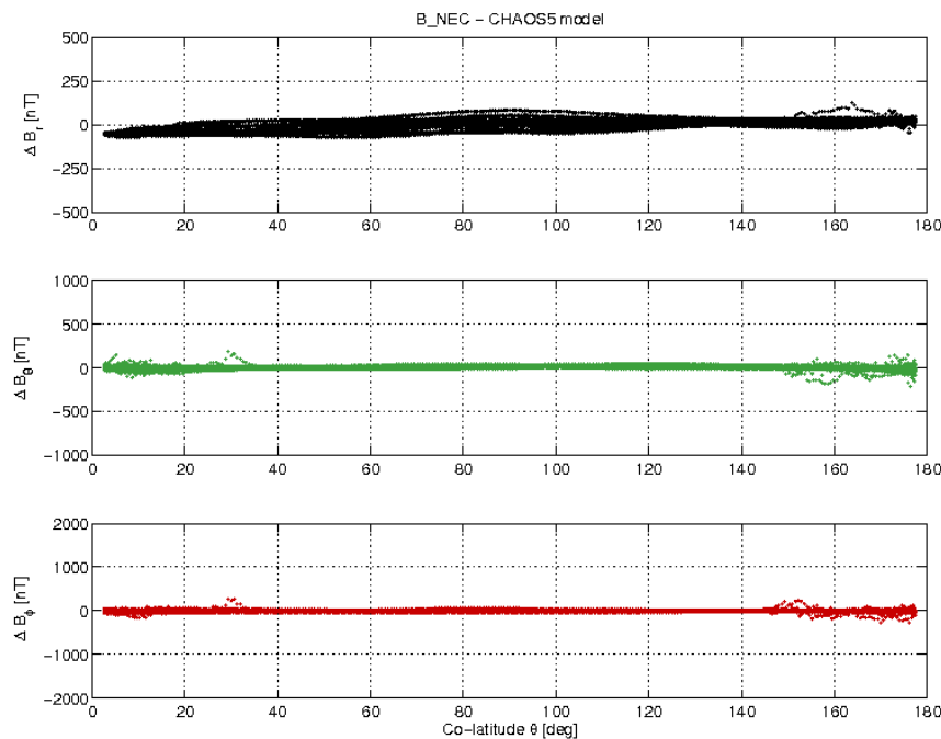
Figure 3-17: S/C A day 09/10 B_{NEC} - B_{Chaos} vs colatitude.
