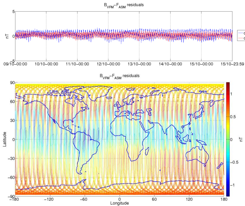
Figure 3-8: ASM-VFM residuals for S/C A, during monitoring period 09/10-15/10. In top figure are plotted: difference between |B VFM | and F ASM (without dB Sun correction) (blue colour), and the residuals with dB Sun corrections (red colour). In bottom figure residuals are presented on the world map.
