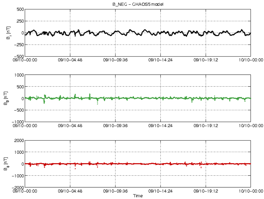
Figure 3-20: S/C B day 09/10 time series of B_{NEC} - B_{Chaos} residuals.
