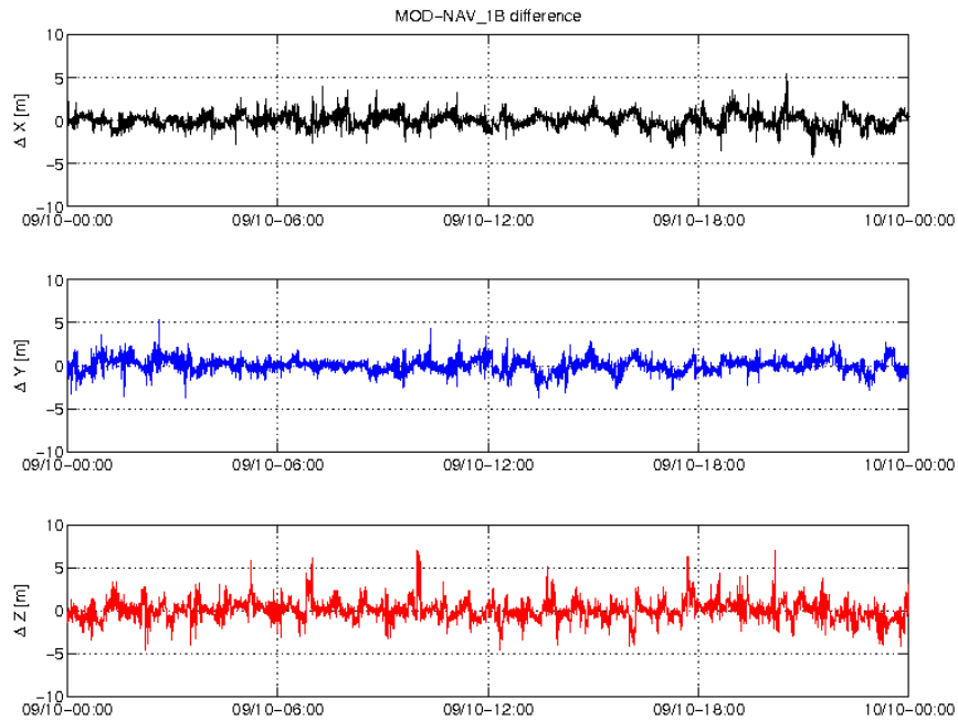
Figure 3-3: Difference MOD-GPSNAV, S/C A, 09/10. From top to bottom: X, Y and Z-axis
