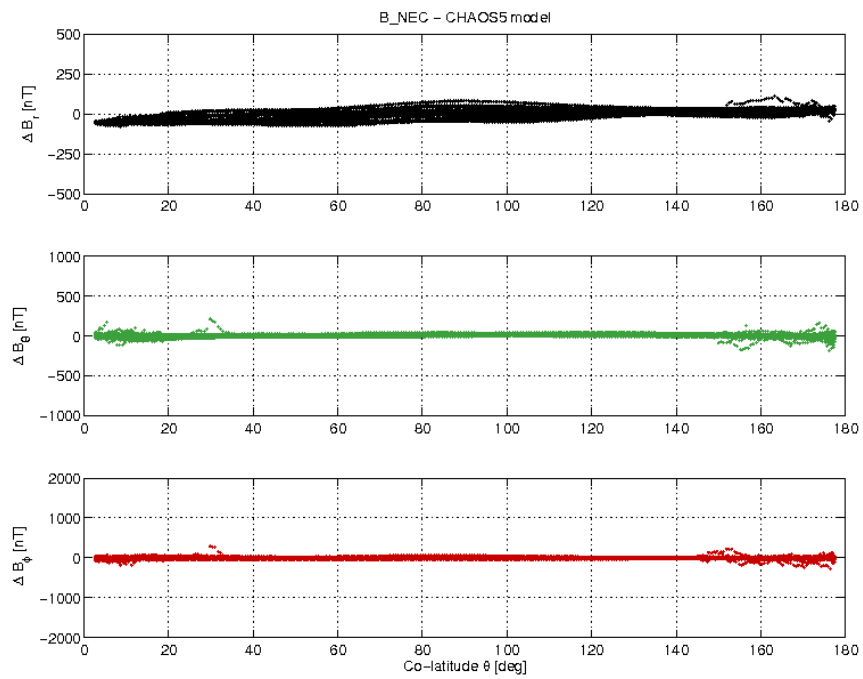
Figure 3-21: S/C C day 09/10 B_{NEC} - B_{Chaos} difference vs colatitude.
