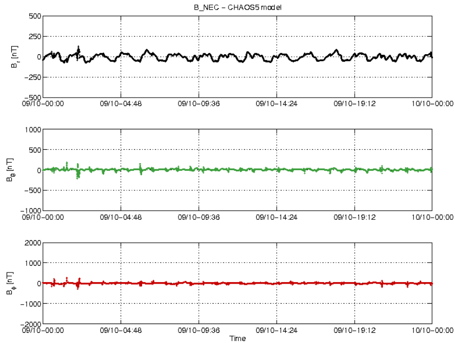
Figure 3-18: S/C A day 09/10: time series of B_{NEC} - B_{Chaos} residuals.
