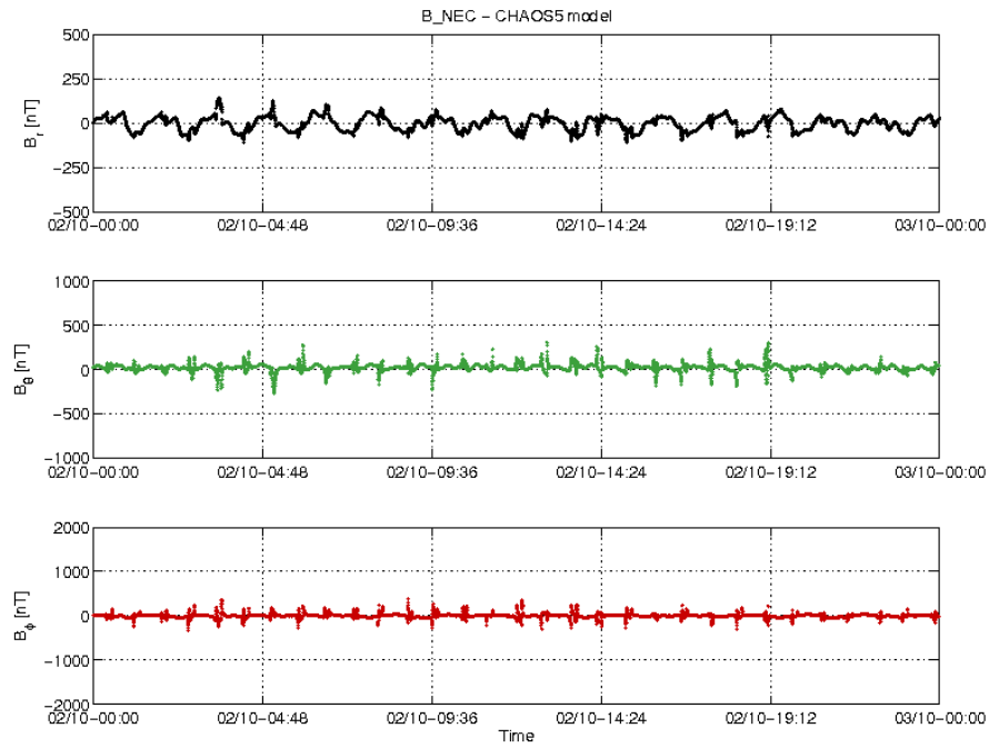
Figure 3-18: S/C A day 02/10: time series of B_{NEC} - B_{Chaos} residuals.
