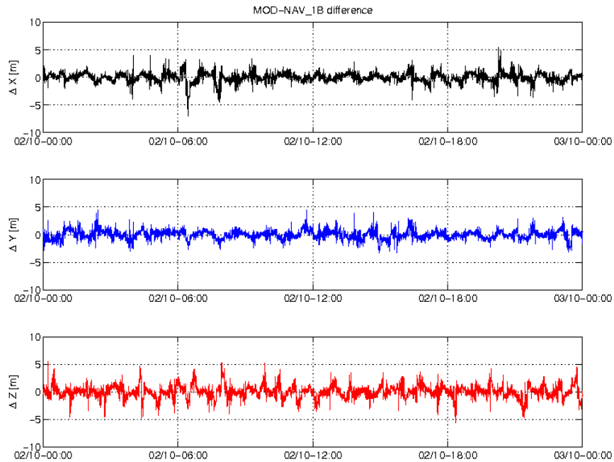
Figure 3-3: Difference MOD-GPSNAV, S/C A, 02/10. From top to bottom: X, Y and Z-axis
