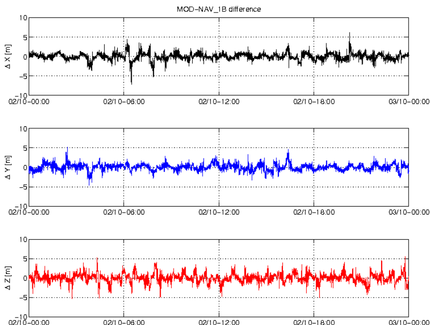
Figure 3-5: Difference MOD-GPSNAV, S/C C, 02/10. From top to bottom: X, Y and Z-axis
