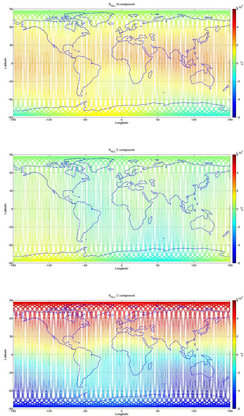
Figure 3-12: S/C C, world map plots of the geomagnetic field and components measured during monitoring period 02/10-08/10. From top to bottom: B_{NEC} components (North, East, and Centre) of magnetic field from VFM measurement.
