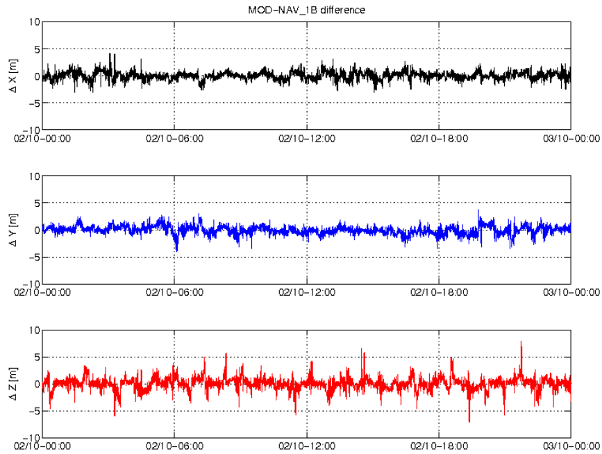
Figure 3-4: Difference MOD-GPSNAV, S/C B, 02/10. From top to bottom: X, Y and Z-axis
