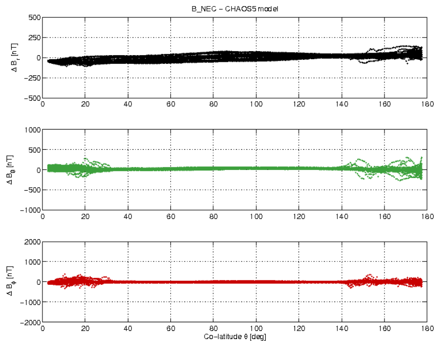
Figure 3-17: S/C A day 02/10 B_{NEC} - B_{Chaos5} vs colatitude.
