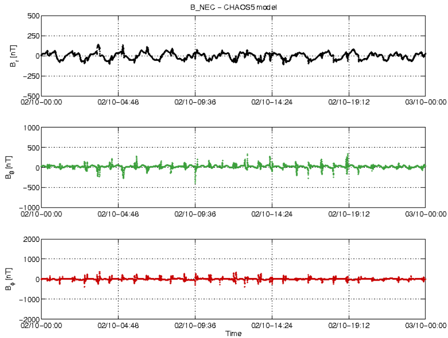
Figure 3-22: S/C C day 02/10 time series of B_{NEC} - B_{Chaos} residuals.
