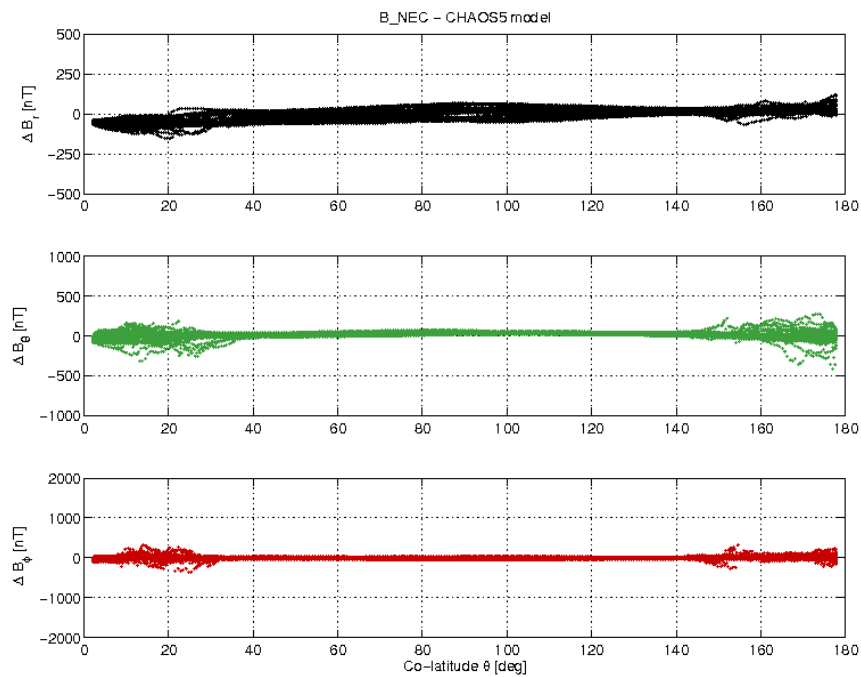
Figure 3-19: S/C B day 02/10 B_{NEC} - B_{Chaos} difference vs colatitude.
