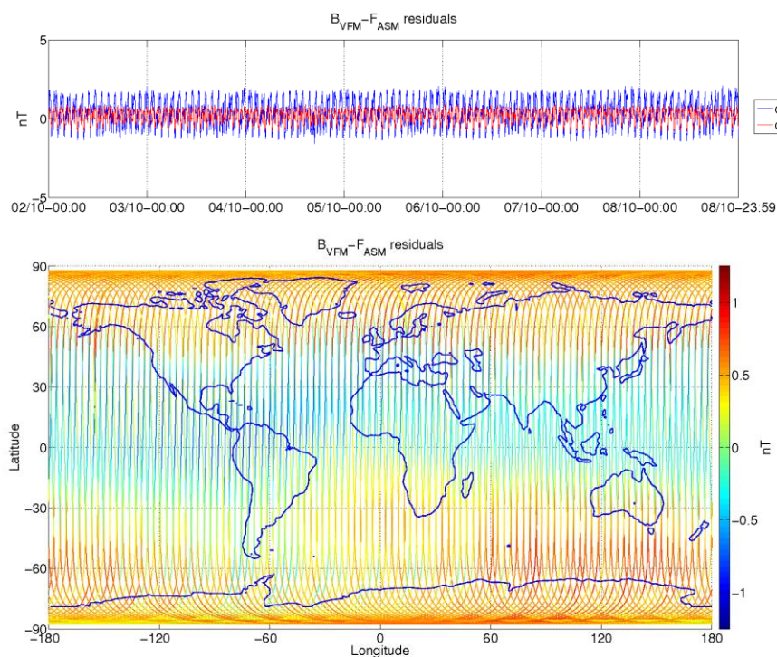
Figure 3-9: ASM-VFM residuals for S/C B, during monitoring period 02/10-08/10. In top figure are plotted: difference between |B VFM | and F ASM (without dB Sun correction) (blue colour), and the residuals with dB Sun corrections (red colour). In bottom figure residuals are presented on the world map.
