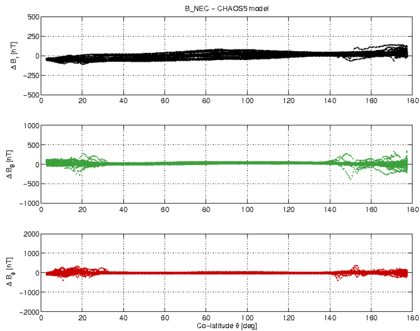
Figure 3-21: S/C C day 02/10 B_{NEC} - B_{Chaos} difference vs colatitude.
