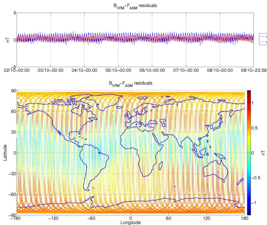
Figure 3-8: ASM-VFM residuals for S/C A, during monitoring period 02/10-08/10. In top figure are plotted: difference between |B_{VFM}| and F_{ASM} (without dB_{Sun} correction) (blue colour), and the residuals with dB_{Sun} corrections (red colour). In bottom figure residuals are presented on the world map.
