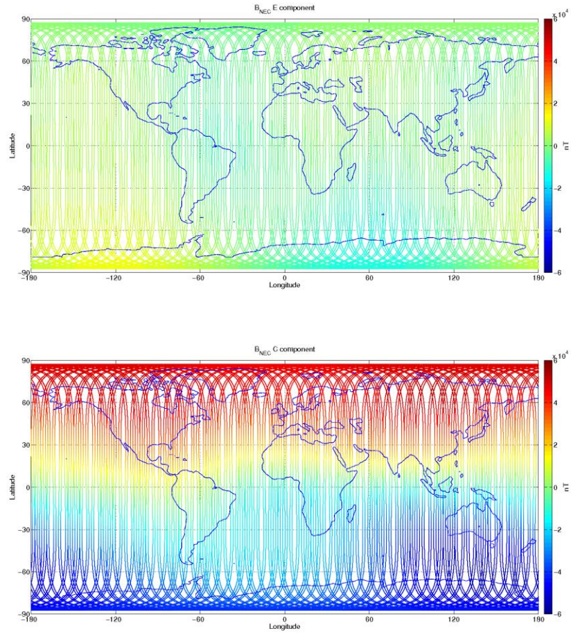
Figure 3-10: S/C A, world map plots of the geomagnetic field and components measured during monitoring period 02/10-08/10. From top to bottom: F-magnetic field from ASM measurement, B NEC components (North, East, and Centre) of magnetic field from VFM measurement.
