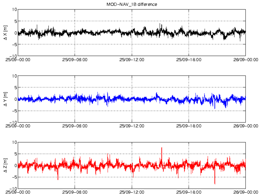
Figure 3-4: Difference MOD-GPSNAV, S/C B, 25/09. From top to bottom: X, Y and Z-axis
