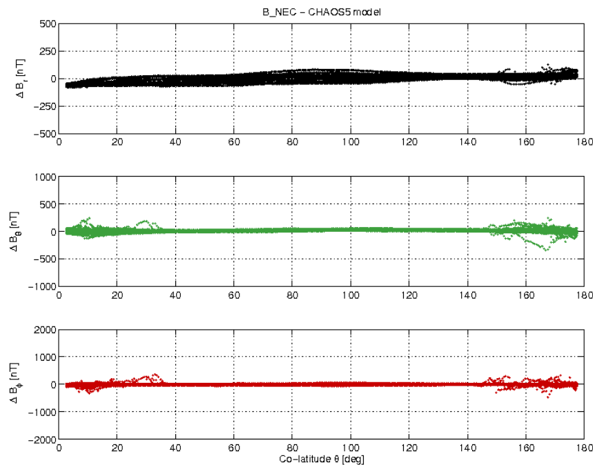
Figure 3-17: S/C A day 25/09 B_{NEC} - B_{Chaos5} vs colatitude.
