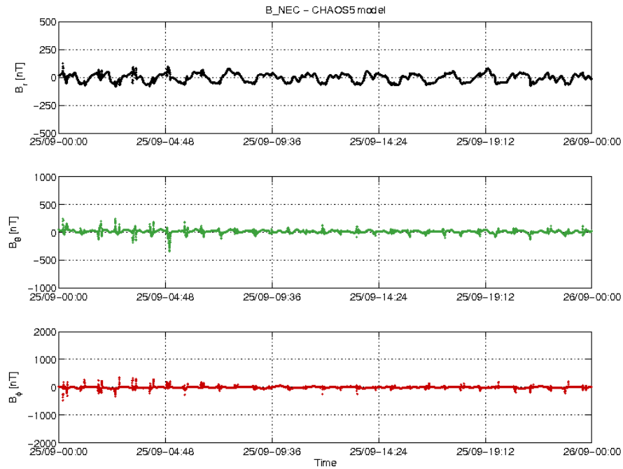
Figure 3-18: S/C A day 25/09: time series of B_{NEC} - B_{Chaos} residuals.
