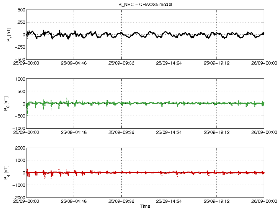
Figure 3-20: S/C B day 25/09 time series of B_{NEC} - B_{Chaos} residuals.
