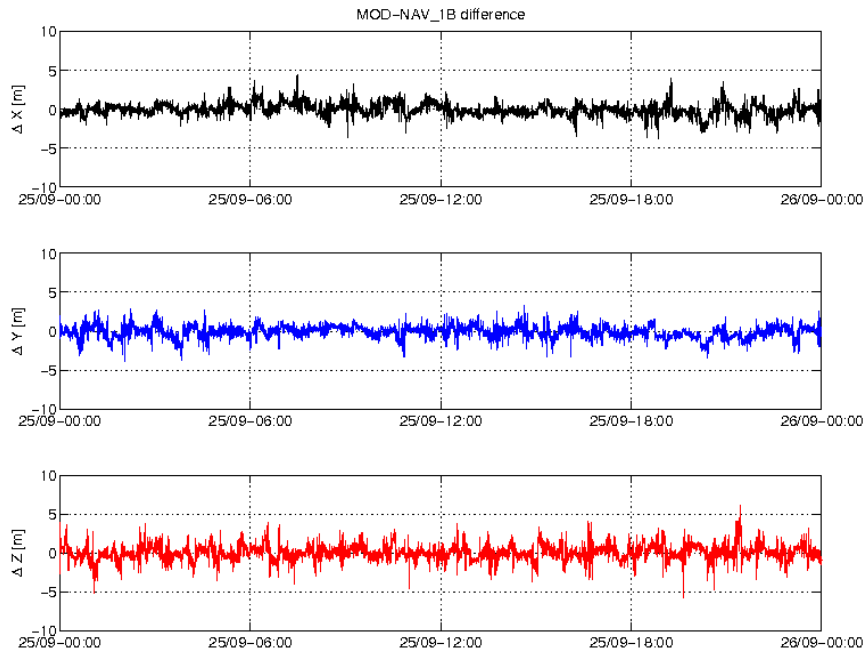
Figure 3-3: Difference MOD-GPSNAV, S/C A, 25/09. From top to bottom: X, Y and Z-axis
