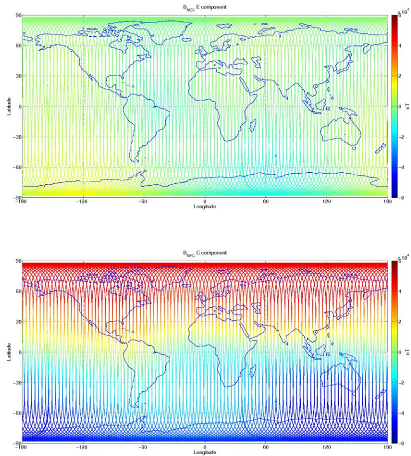
Figure 3-11: S/C B, world map plots of the geomagnetic field and components measured during monitoring period 25/09-01/10. From top to bottom: F-magnetic field from ASM measurement, B_{NEC} components (North, East, and Centre) of magnetic field from VFM measurement.
