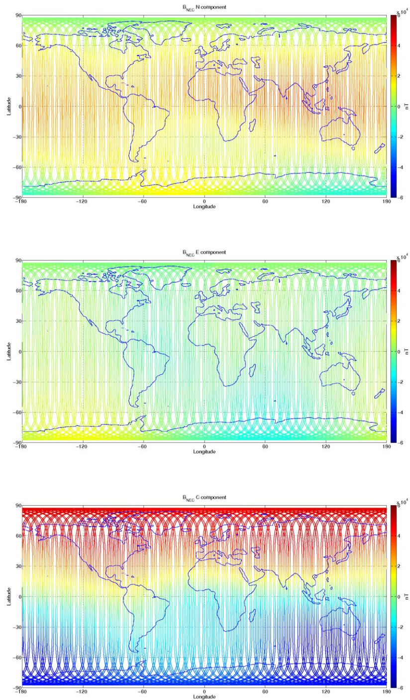
Figure 3-12: S/C C, world map plots of the geomagnetic field and components measured during monitoring period 25/09-01/10. From top to bottom: B NEC components (North, East, and Centre) of magnetic field from VFM measurement.
