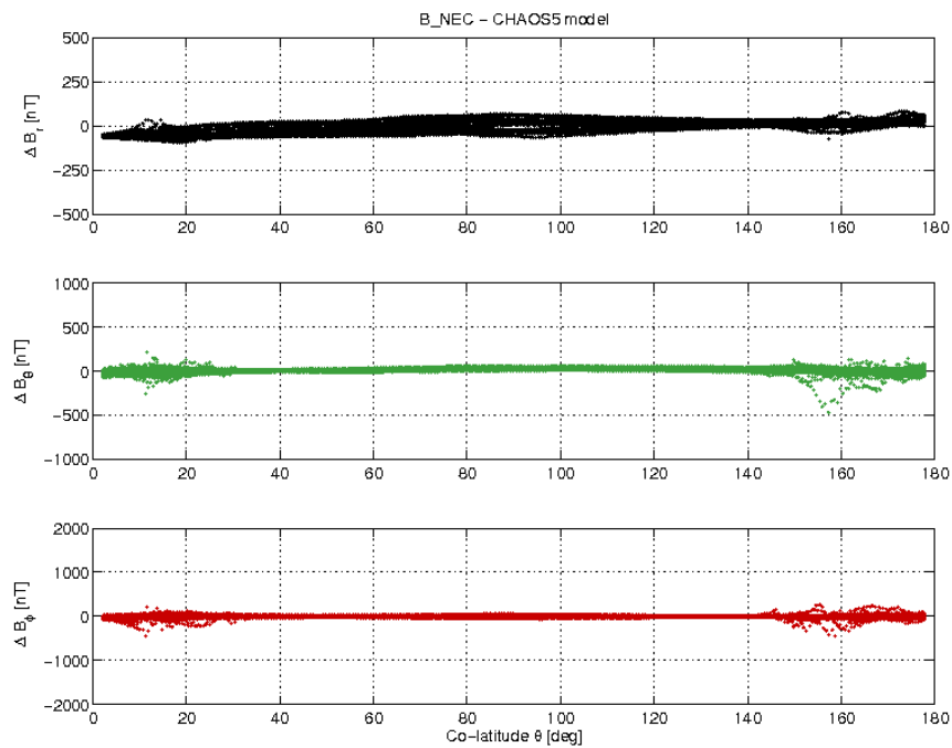
Figure 3-19: S/C B day 25/09 B_{NEC} - B_{Chaos} difference vs colatitude.
