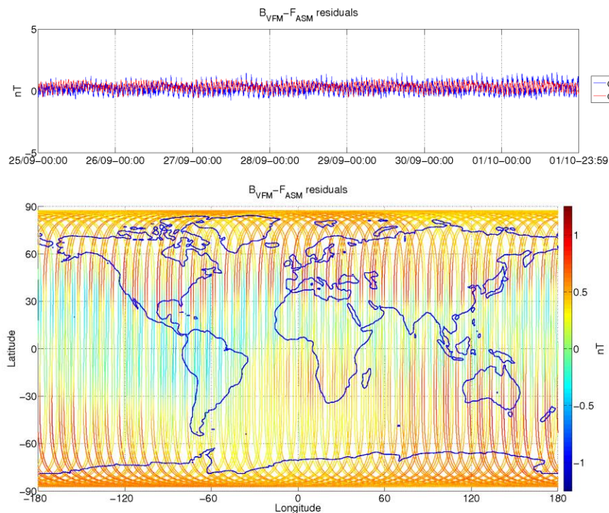
Figure 3-8: ASM-VFM residuals for S/C A, during monitoring period 25/09-01/10. In top figure are plotted: difference between |B_{VFM}| and F_{ASM} (without dB_{Sun} correction) (blue colour), and the residuals with dB_{Sun} corrections (red colour). In bottom figure residuals are presented on the world map.
