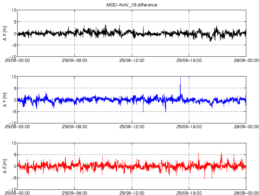
Figure 3-5: Difference MOD-GPSNAV, S/C C, 25/09. From top to bottom: X, Y and Z-axis
