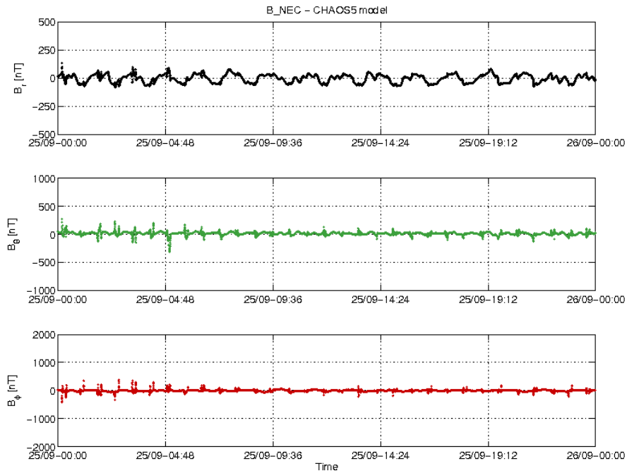
Figure 3-22: S/C C day 25/09 time series of B_{NEC} - B_{Chaos} residuals.
