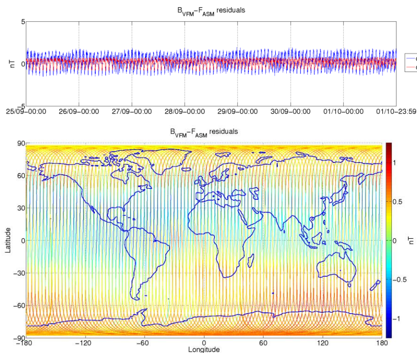
Figure 3-9: ASM-VFM residuals for S/C B, during monitoring period 25/09-01/10. In top figure are plotted: difference between |B_{VFM}| and F_{ASM} (without dB_{Sun} correction) (blue colour), and the residuals with dB_{Sun} corrections (red colour). In bottom figure residuals are presented on the world map.
