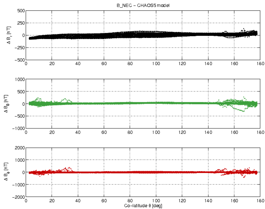
Figure 3-21: S/C C day 25/09 B_{NEC} - B_{Chaos} difference vs colatitude.
