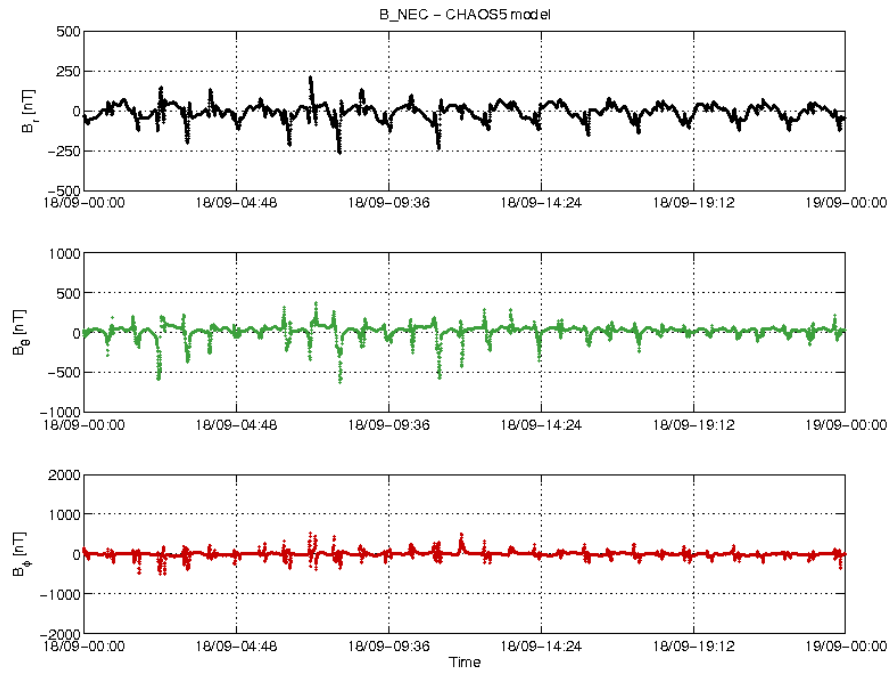
Figure 3-20: S/C B day 18/09 time series of B_{NEC} - B_{Chaos} residuals.
