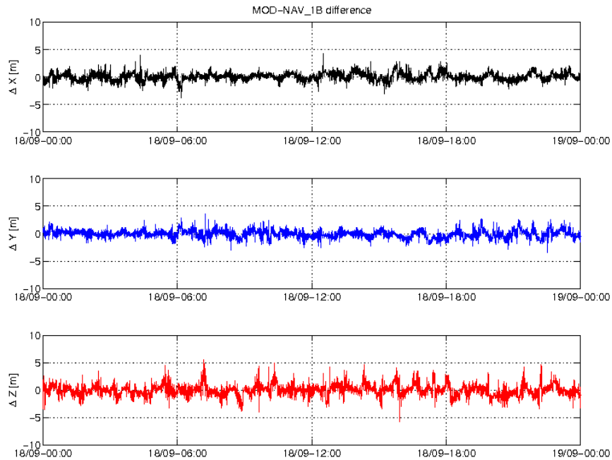
Figure 3-4: Difference MOD-GPSNAV, S/C B, 18/09. From top to bottom: X, Y and Z-axis
