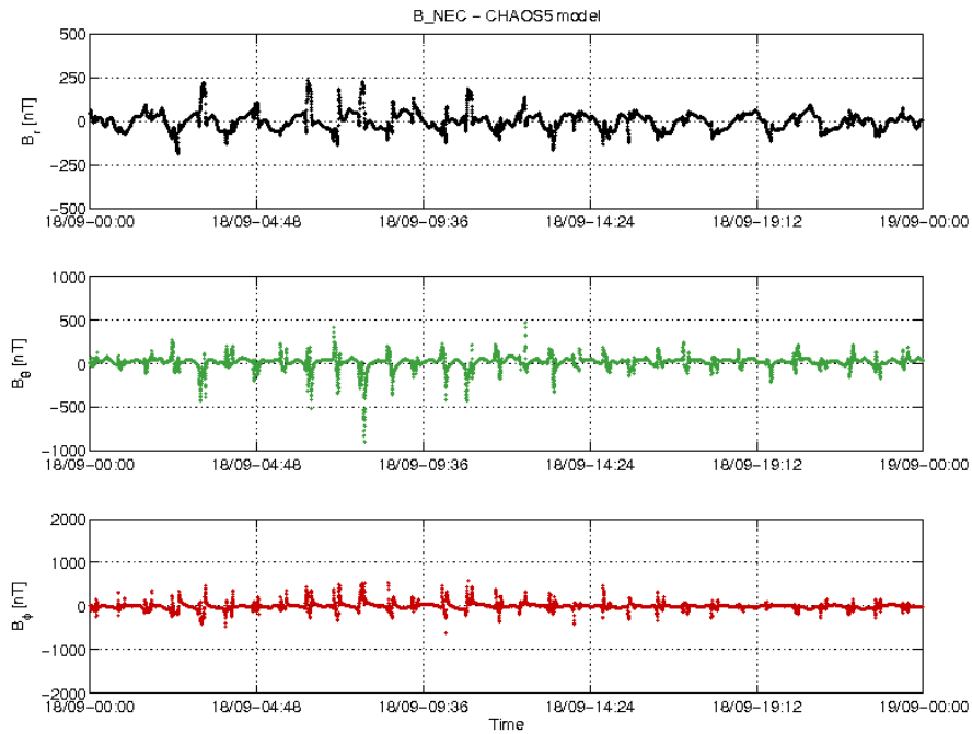
Figure 3-22: S/C C day 18/09 time series of B_{NEC} - B_{Chaos} residuals.
