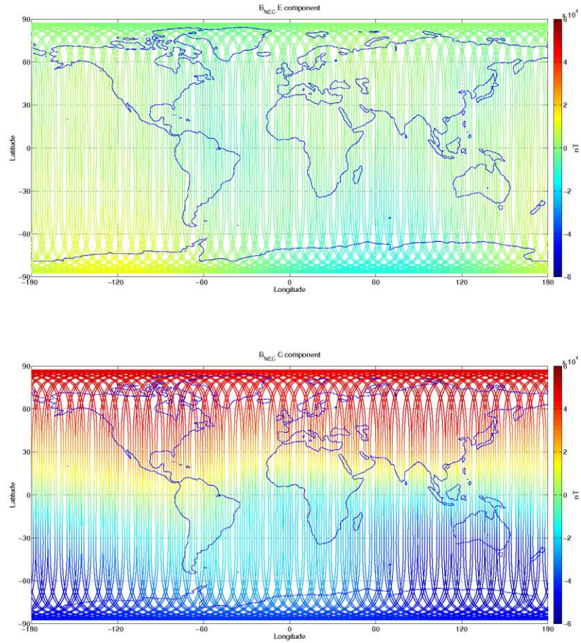
Figure 3-10: S/C A, world map plots of the geomagnetic field and components measured during monitoring period 18/09-24/09. From top to bottom: F-magnetic field from ASM measurement, B_{NEC} components (North, East, and Centre) of magnetic field from VFM measurement.
