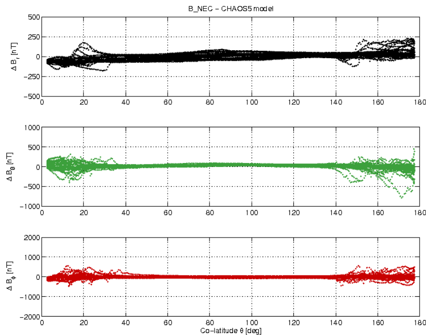
Figure 3-17: S/C A day 18/09 B_{NEC} - B_{Chaos5} vs colatitude.
