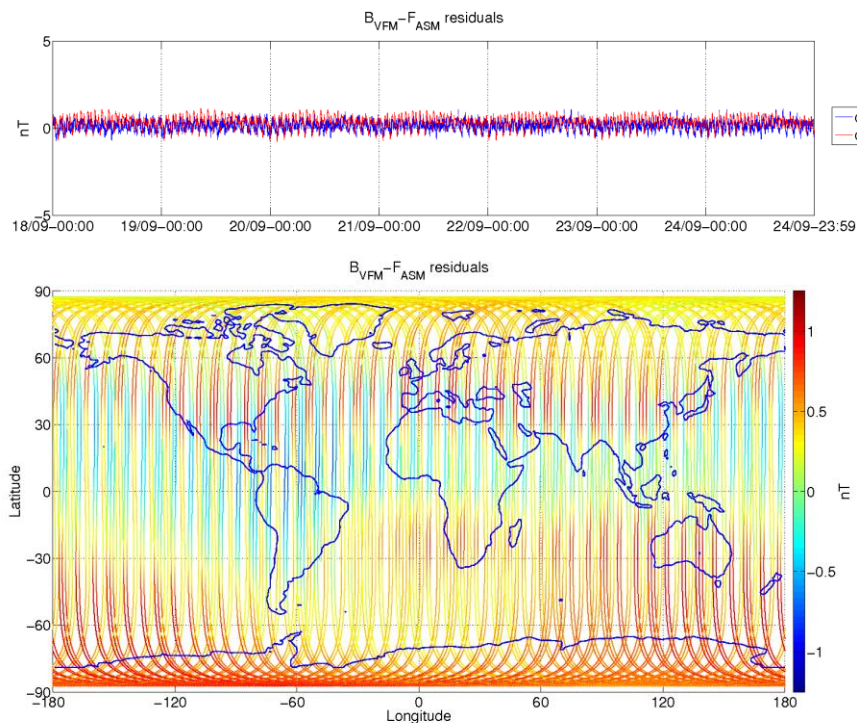
Figure 3-8: ASM-VFM residuals for S/C A, during monitoring period 18/09-24/09. In top figure are plotted: difference between |B_{VFM}| and F_{ASM} (without dB_{Sun} correction) (blue colour), and the residuals with dB_{Sun} corrections (red colour). In bottom figure residuals are presented on the world map.
