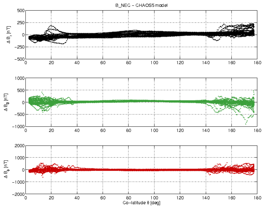
Figure 3-21: S/C C day 18/09 B_{NEC} - B_{Chaos} difference vs colatitude.
