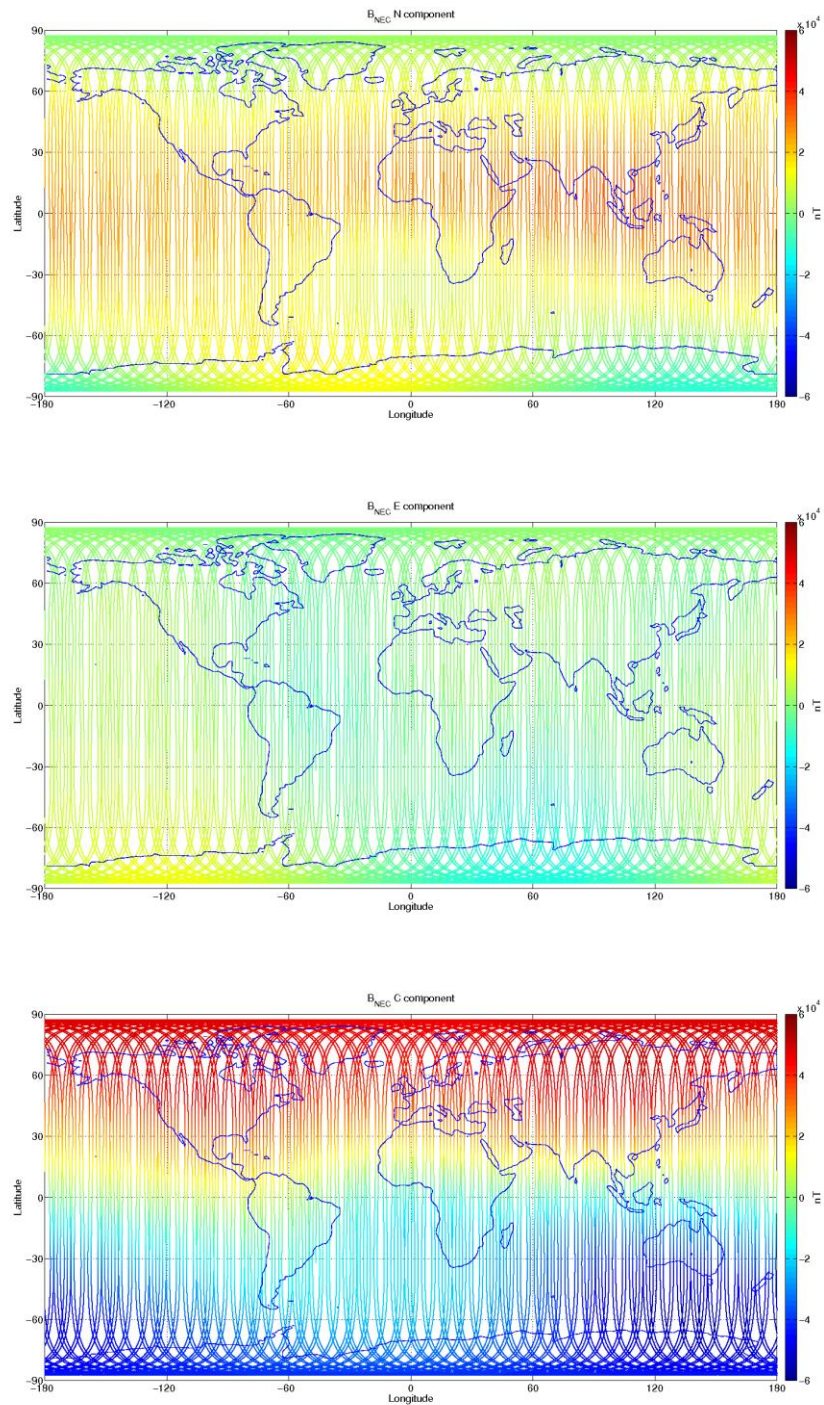
Figure 3-12: S/C C, world map plots of the geomagnetic field and components measured during monitoring period 18/09-24/09. From top to bottom: B NEC components (North, East, and Centre) of magnetic field from VFM measurement.
