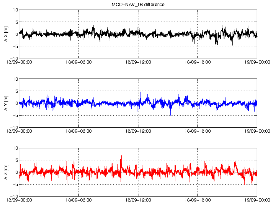
Figure 3-3: Difference MOD-GPSNAV, S/C A, 18/09. From top to bottom: X, Y and Z-axis
