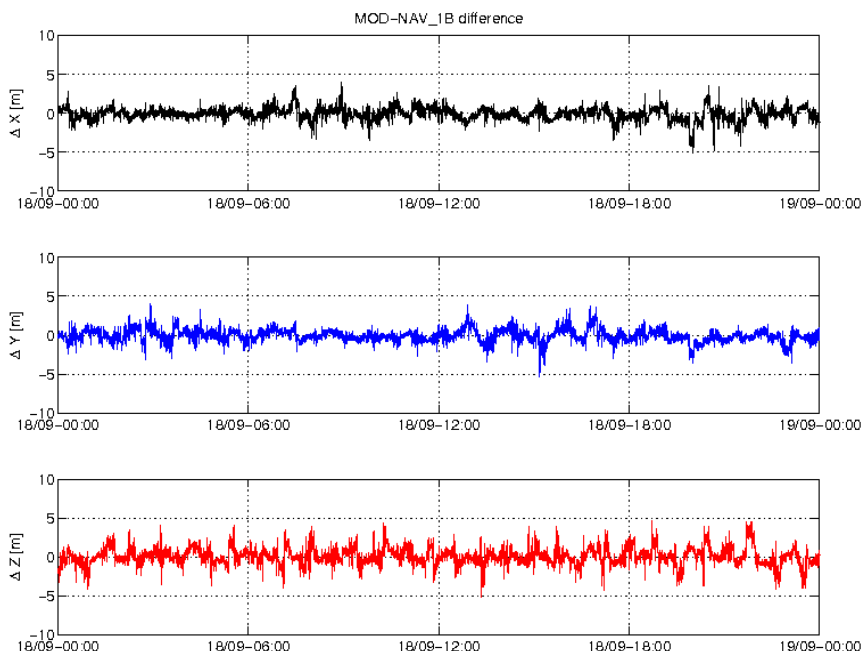
Figure 3-5: Difference MOD-GPSNAV, S/C C, 18/09. From top to bottom: X, Y and Z-axis
