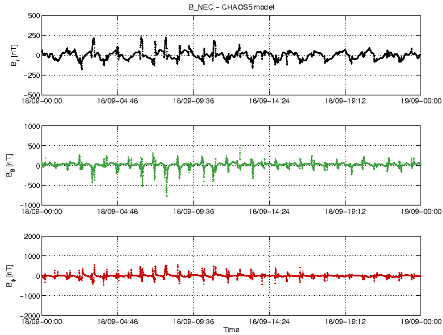
Figure 3-18: S/C A day 18/09: time series of B_{NEC} - B_{Chaos} residuals.
