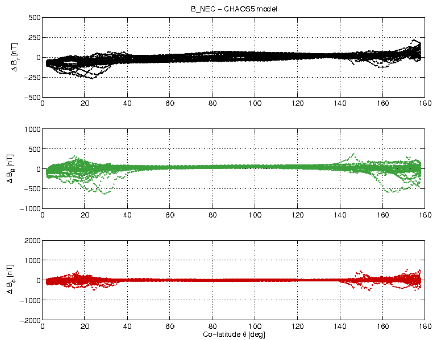
Figure 3-19: S/C B day 18/09 B_{NEC} - B_{Chaos} difference vs colatitude.
