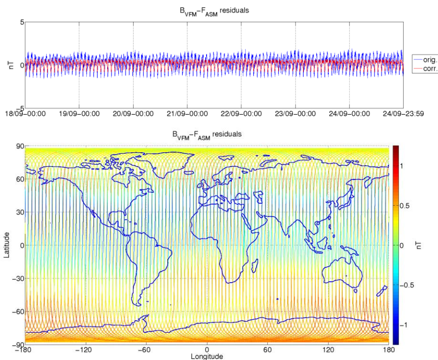
Figure 3-9: ASM-VFM residuals for S/C B, during monitoring period 18/09-24/09. In top figure are plotted: difference between |B\_VFM| and F\_ASM (without dB\_Sun correction) (blue colour), and the residuals with dB\_Sun corrections (red colour). In bottom figure residuals are presented on the world map.
