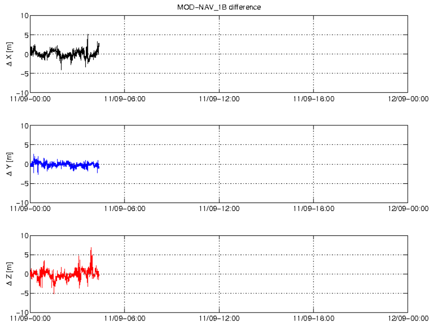
Figure 3-4: Difference MOD-GPSNAV, S/C B, 11/09. From top to bottom: X, Y and Z-axis. The gap present in this trend is caused by the anomaly in VFM-B described in section 3.1.
