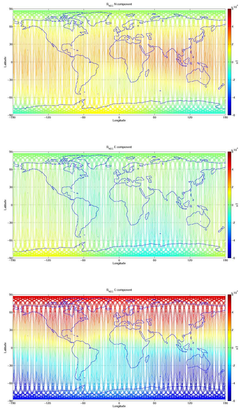
Figure 3-12: S/C C, world map plots of the geomagnetic field and components measured during monitoring period 11/09-17/09. From top to bottom: B_{NEC} components (North, East, and Centre) of magnetic field from VFM measurement.
