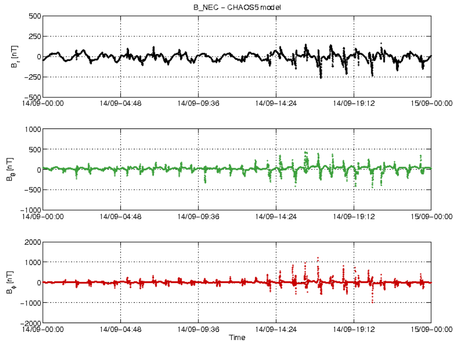
Figure 3-20: S/C B day 11/09 time series of B_{NEC} - B_{Chaos} residuals.
