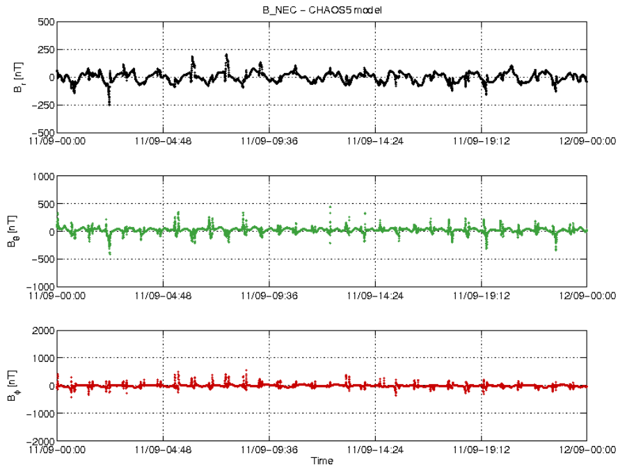
Figure 3-22: S/C C day 11/09 time series of B_{NEC} - B_{Chaos} residuals.
