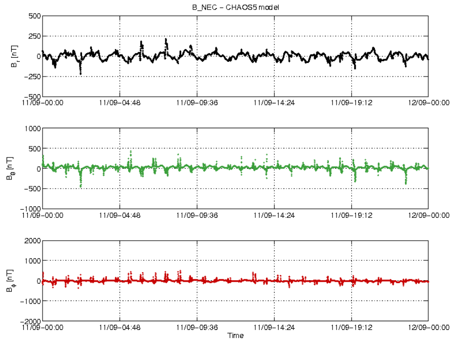
Figure 3-18: S/C A day 11/09: time series of B_{NEC} - B_{Chaos} residuals.
