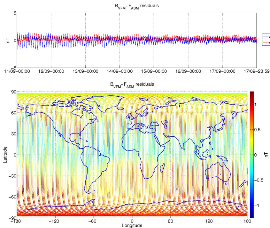
Figure 3-8: ASM-VFM residuals for S/C A, during monitoring period 11/09-17/09. In top figure are plotted: difference between |B_{VFM}| and F_{ASM} (without dB_{Sun} correction) (blue colour), and the residuals with dB_{Sun} corrections (red colour). In bottom figure residuals are presented on the world map.
