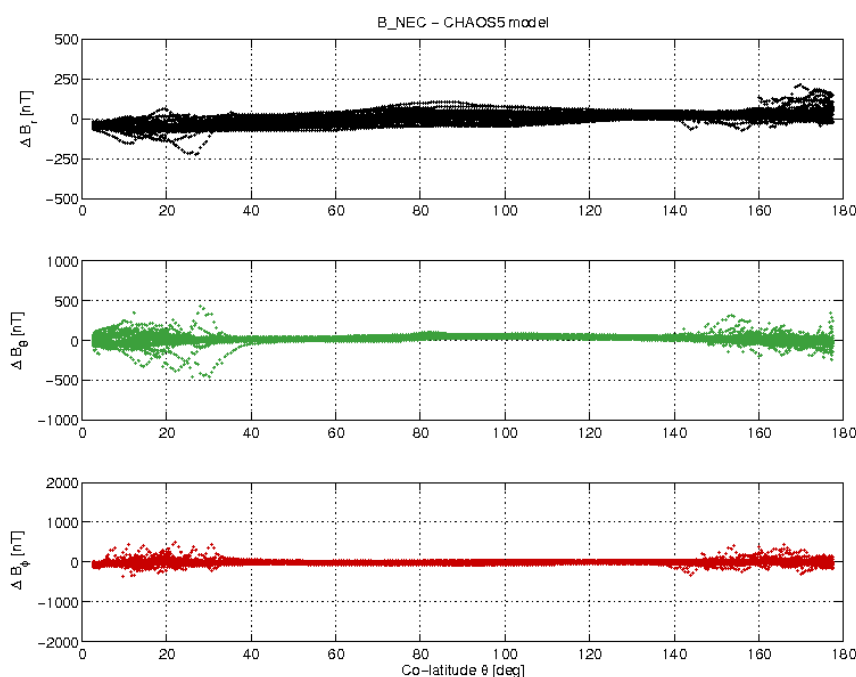
Figure 3-17: S/C A day 11/09 B_{NEC} - B_{Chaos5} vs colatitude.
