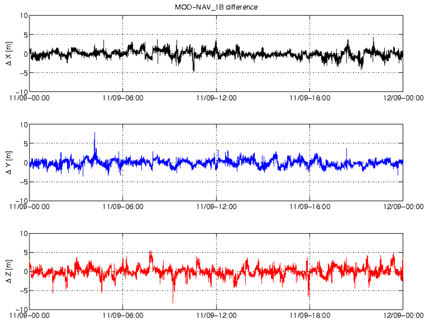
Figure 3-5: Difference MOD-GPSNAV, S/C C, 11/09. From top to bottom: X, Y and Z-axis
