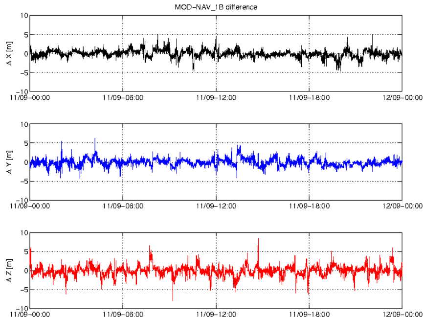
Figure 3-3: Difference MOD-GPSNAV, S/C A, 11/09. From top to bottom: X, Y and Z-axis
