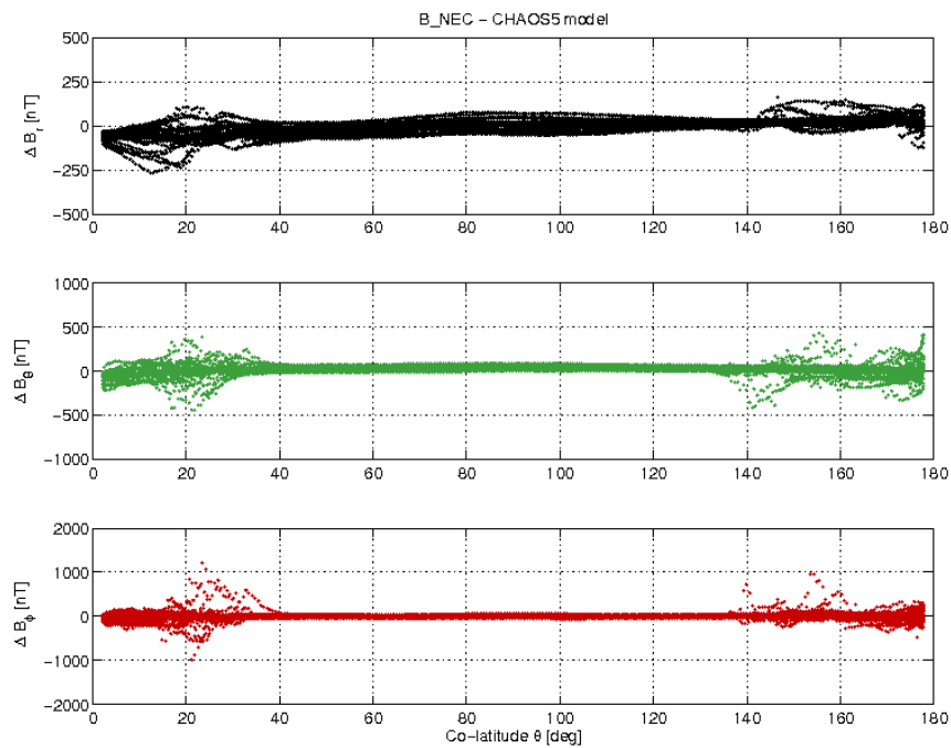
Figure 3-19: S/C B day 11/09 B_{NEC} - B_{Chaos} difference vs colatitude.
