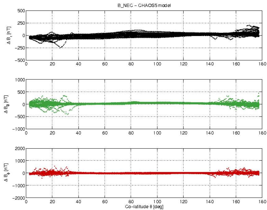
Figure 3-21: S/C C day 11/09 B_{NEC} - B_{Chaos} difference vs colatitude.
