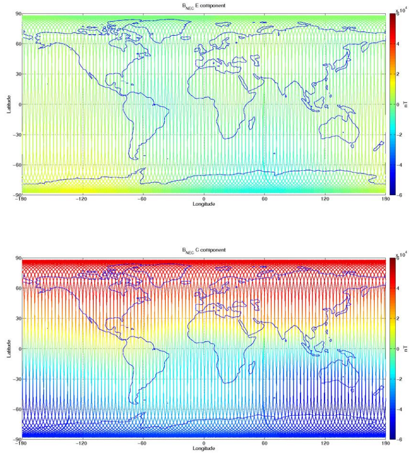
Figure 3-11: S/C B, world map plots of the geomagnetic field and components measured during monitoring period 04/09-10/09. From top to bottom: F-magnetic field from ASM measurement, B_{NEC} components (North, East, and Centre) of magnetic field from VFM measurement.
