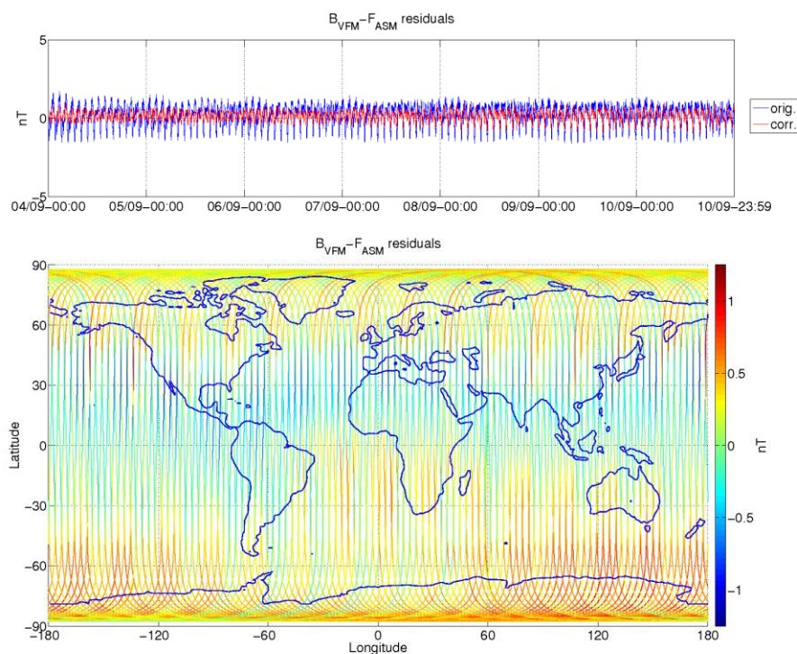
Figure 3-9: ASM-VFM residuals for S/C B, during monitoring period 04/09-10/09. In top figure are plotted: difference between |B_{VFM}| and F_{ASM} (without dB_{Sun} correction) (blue colour), and the residuals with dB_{Sun} corrections (red colour). In bottom figure residuals are presented on the world map.
