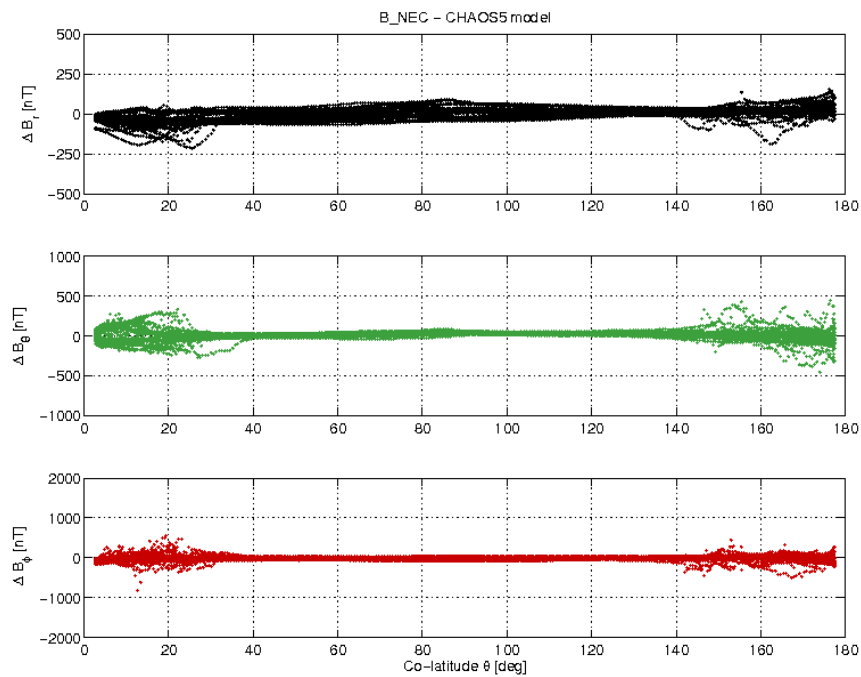
Figure 3-21: S/C C day 04/09 B_{NEC} - B_{Chaos} difference vs colatitude.
