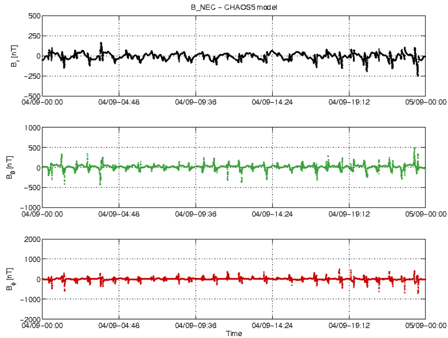
Figure 3-20: S/C B day 04/09 time series of B_{NEC} - B_{Chaos} residuals.
