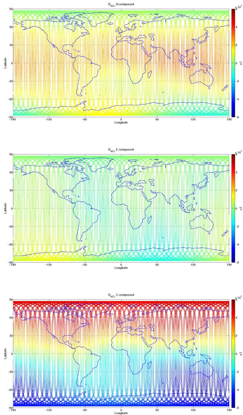
Figure 3-12: S/C C, world map plots of the geomagnetic field and components measured during monitoring period 04/09-10/09. From top to bottom: B_{NEC} components (North, East, and Centre) of magnetic field from VFM measurement.
