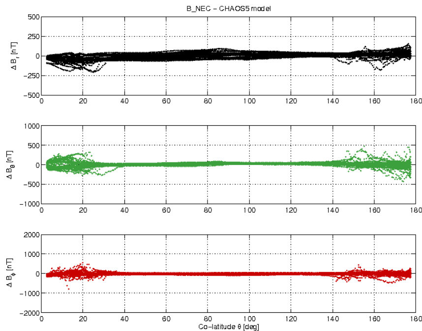
Figure 3-17: S/C A day 04/09 B_{NEC} - B_{Chaos} vs colatitude.
