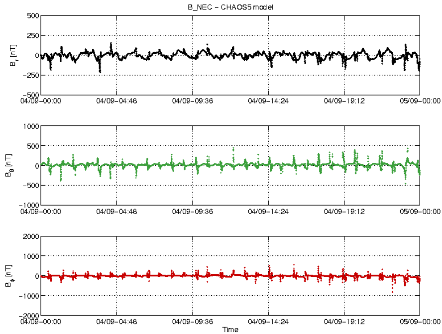
Figure 3-22: S/C C day 04/09 time series of B_{NEC} - B_{Chaos} residuals.
