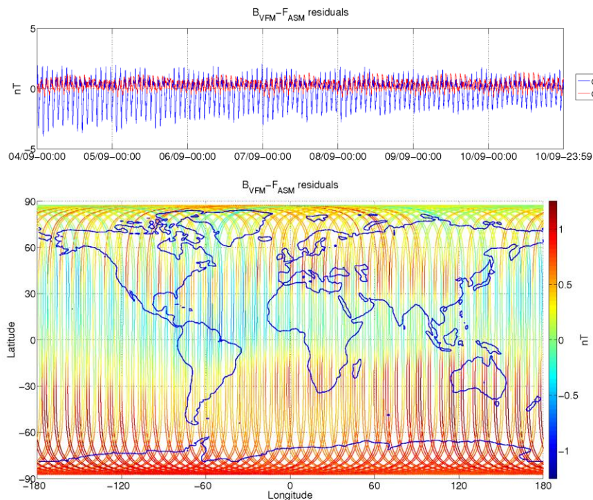
Figure 3-8: ASM-VFM residuals for S/C A, during monitoring period 04/09-10/09. In top figure are plotted: difference between |B_{VFM}| and F_{ASM} (without dB_{Sun} correction) (blue colour), and the residuals with dB_{Sun} corrections (red colour). In bottom figure residuals are presented on the world map.
