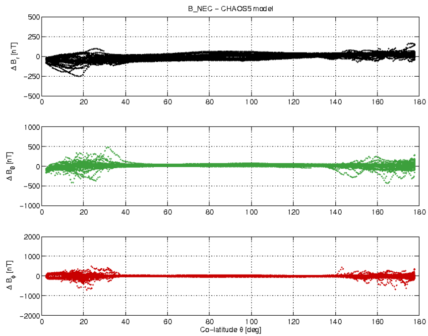
Figure 3-19: S/C B day 04/09 B_{NEC} - B_{Chaos} difference vs colatitude.
