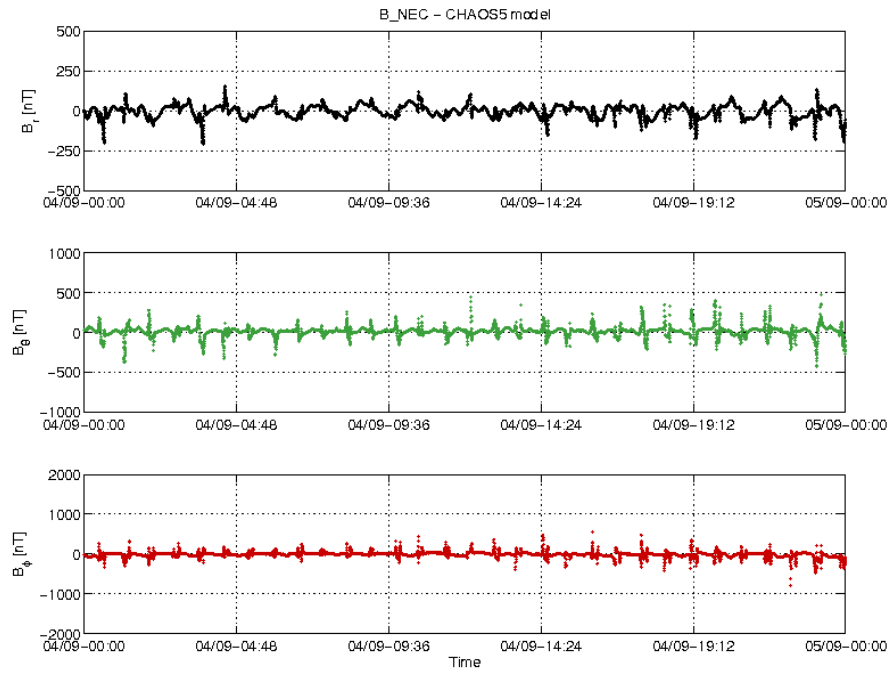
Figure 3-18: S/C A day 04/09: time series of B_{NEC} - B_{Chaos} residuals.
