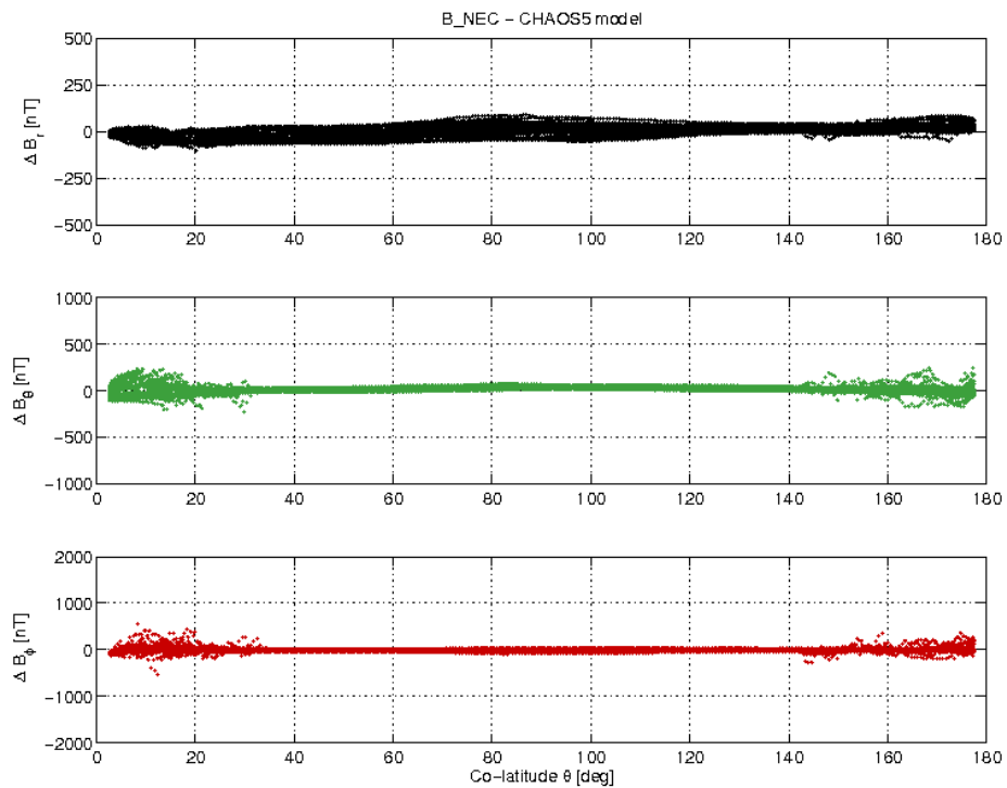
Figure 3-21: S/C C day 28/08 B_{NEC} - B_{Chaos} difference vs colatitude.
