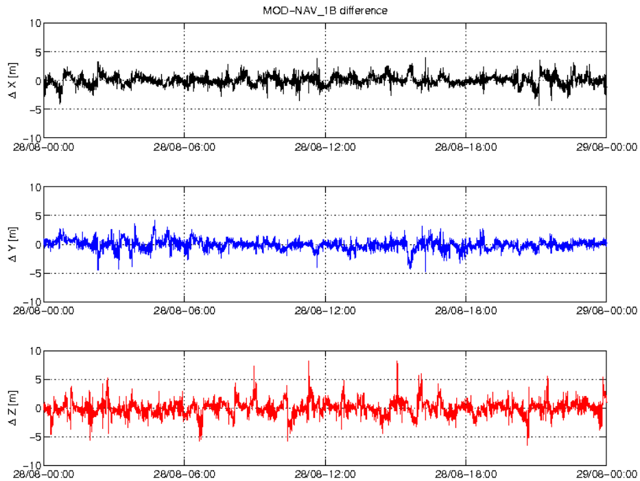
Figure 3-3: Difference MOD-GPSNAV, S/C A, 28/08. From top to bottom: X, Y and Z-axis
