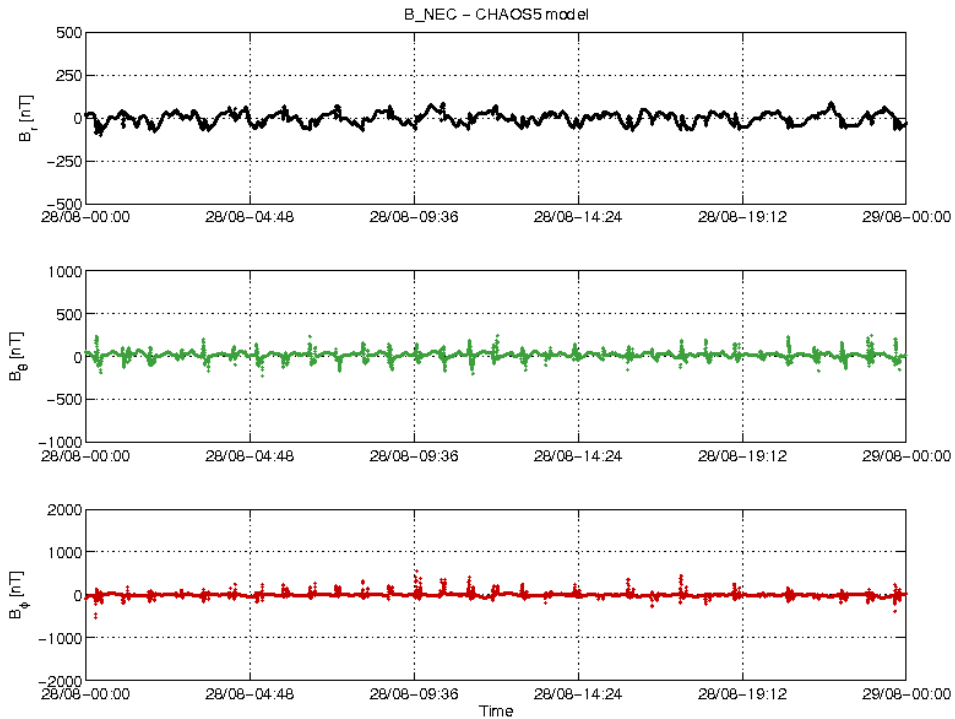
Figure 3-22: S/C C day 28/08 time series of B_{NEC} - B_{Chaos} residuals.
