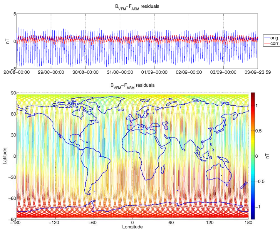
Figure 3-8: ASM-VFM residuals for S/C A, during monitoring period 28/08-03/09. In top figure are plotted: difference between |B_{VFM}| and F_{ASM} (without dB_{Sun} correction) (blue colour), and the residuals with dB_{Sun} corrections (red colour). In bottom figure residuals are presented on the world map.
