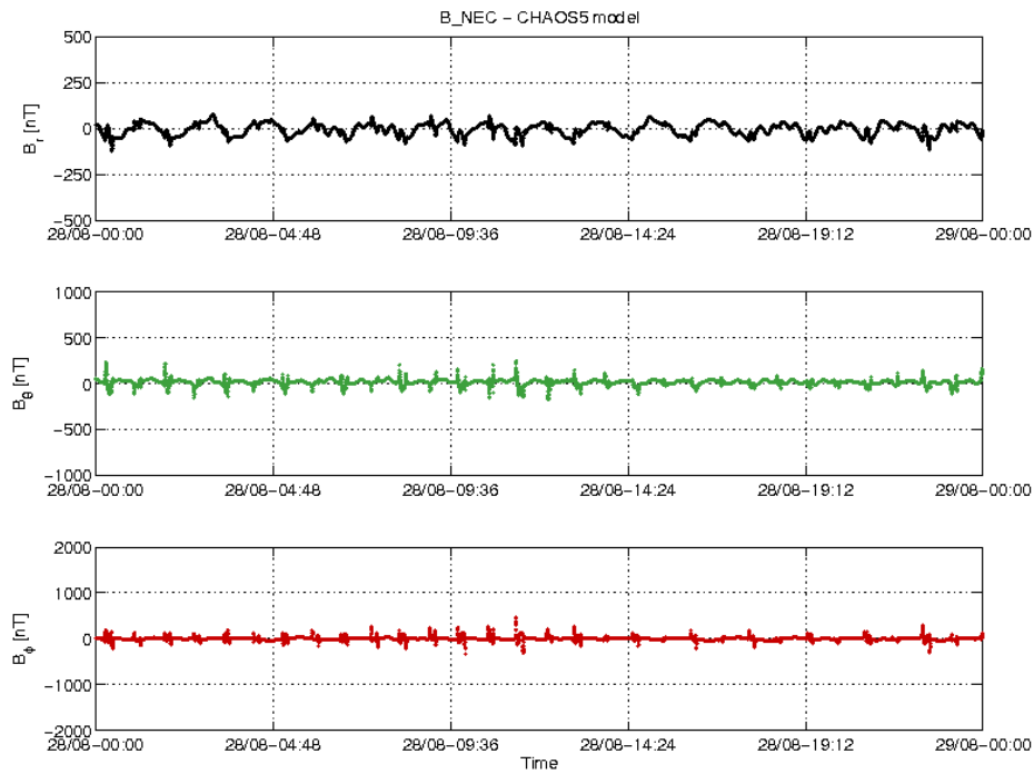
Figure 3-20: S/C B day 28/08 time series of B_{NEC} - B_{Chaos} residuals.
