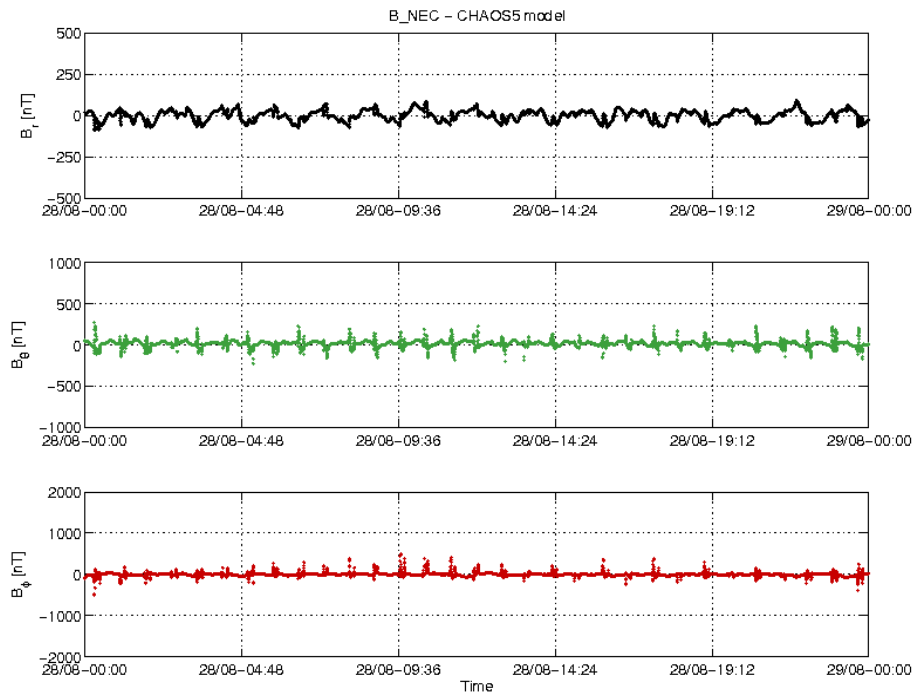
Figure 3-18: S/C A day 28/08: time series of B_{NEC} - B_{Chaos} residuals.
