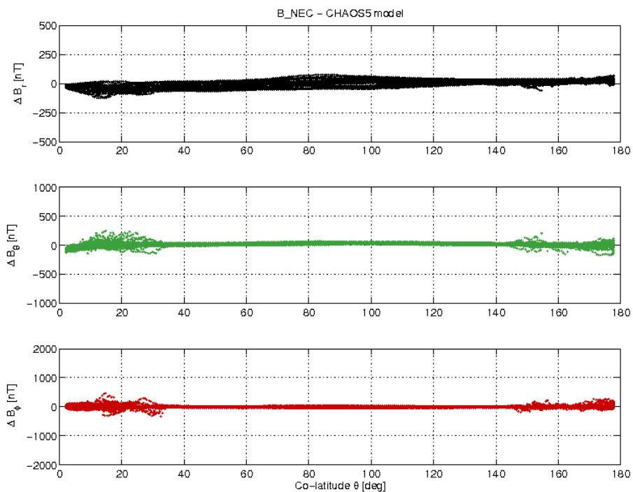
Figure 3-19: S/C B day 28/08 B_{NEC} - B_{Chaos} difference vs colatitude.
