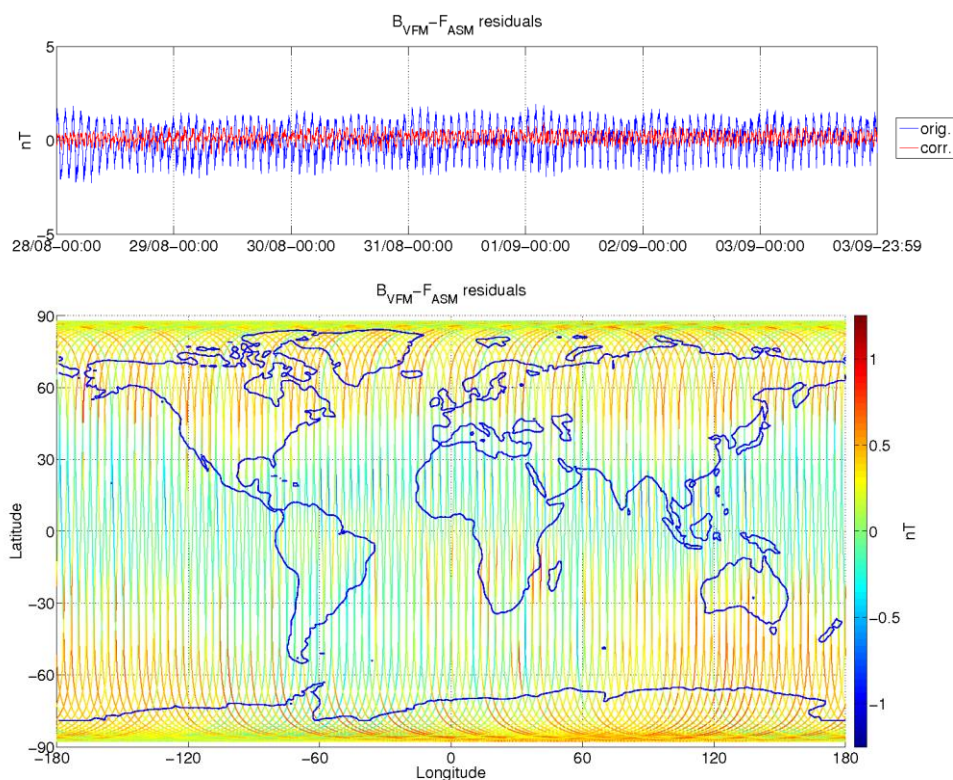
Figure 3-9: ASM-VFM residuals for S/C B, during monitoring period 28/08-03/09. In top figure are plotted: difference between |B_{VFM}| and F_{ASM} (without dB_{Sun} correction) (blue colour), and the residuals with dB_{Sun} corrections (red colour). In bottom figure residuals are presented on the world map.
