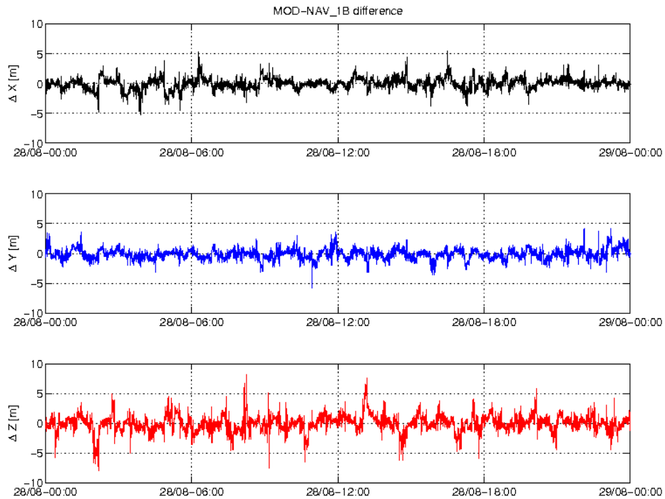
Figure 3-4: Difference MOD-GPSNAV, S/C B, 28/08. From top to bottom: X, Y and Z-axis
