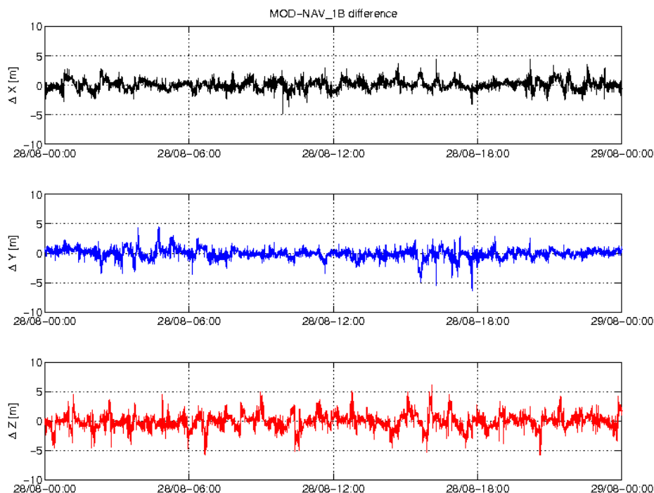
Figure 3-5: Difference MOD-GPSNAV, S/C C, 28/08. From top to bottom: X, Y and Z-axis
