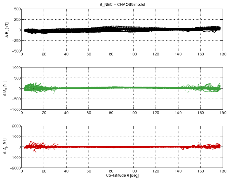
Figure 3-17: S/C A day 28/08 B_{NEC} - B_{Chaos} vs colatitude.
