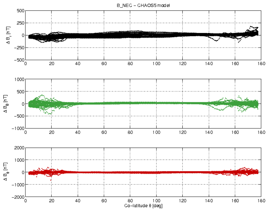
Figure 3-21: S/C C day 21/08 B_{NEC} - B_{Chaos} difference vs colatitude.
