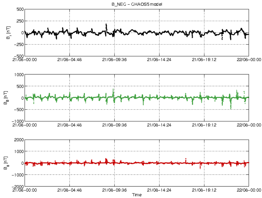
Figure 3-18: S/C A day 21/08: time series of B_{NEC} - B_{Chaos} residuals.
