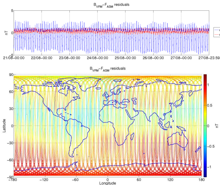
Figure 3-8: ASM-VFM residuals for S/C A, during monitoring period 21/08-27/08. In top figure are plotted: difference between |B_{VFM}| and F_{ASM} (without dB_{Sun} correction) (blue colour), and the residuals with dB_{Sun} corrections (red colour). In bottom figure residuals are presented on the world map.
