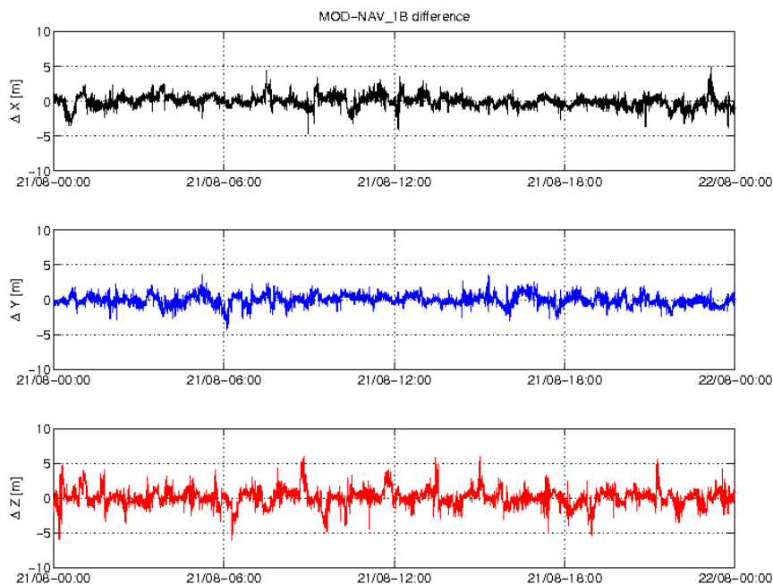
Figure 3-5: Difference MOD-GPSNAV, S/C C, 21/08. From top to bottom: X, Y and Z-axis
