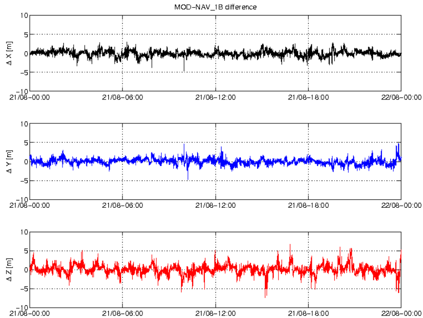
Figure 3-4: Difference MOD-GPSNAV, S/C B, 21/08. From top to bottom: X, Y and Z-axis
