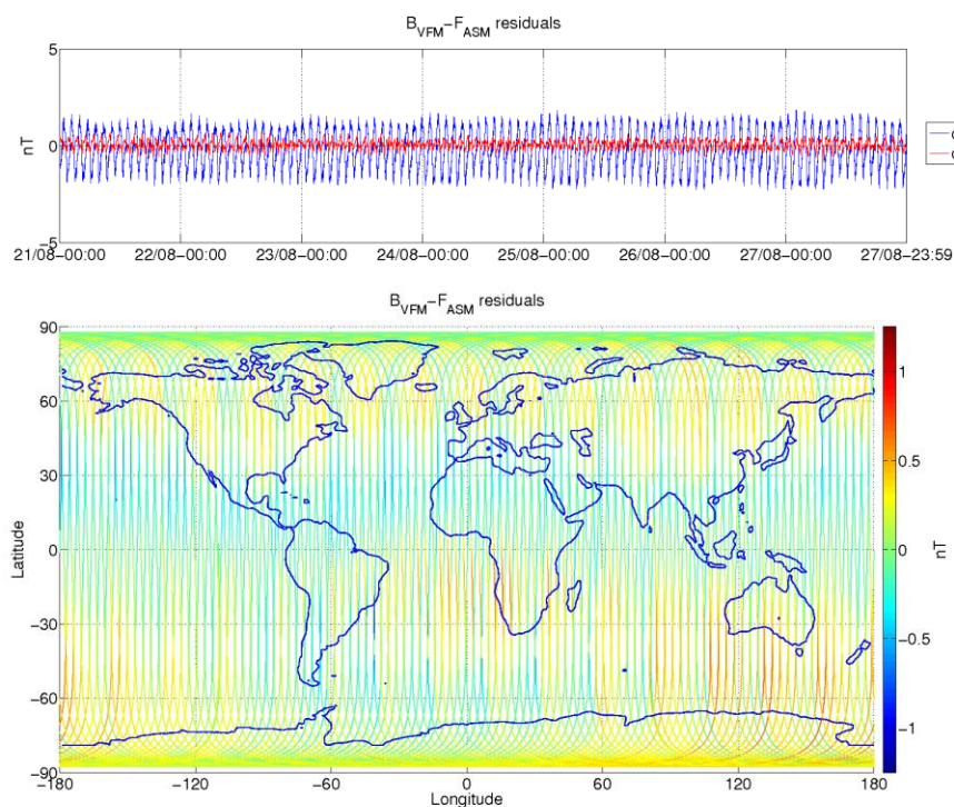
Figure 3-9: ASM-VFM residuals for S/C B, during monitoring period 21/08-27/08. In top figure are plotted: difference between |B_{VFM}| and F_{ASM} (without dB_{Sun} correction) (blue colour), and the residuals with dB_{Sun} corrections (red colour). In bottom figure residuals are presented on the world map.
