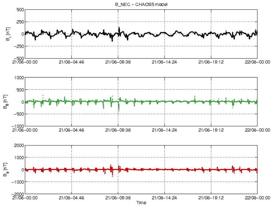
Figure 3-20: S/C B day 21/08 time series of B_{NEC} - B_{Chaos} residuals.
