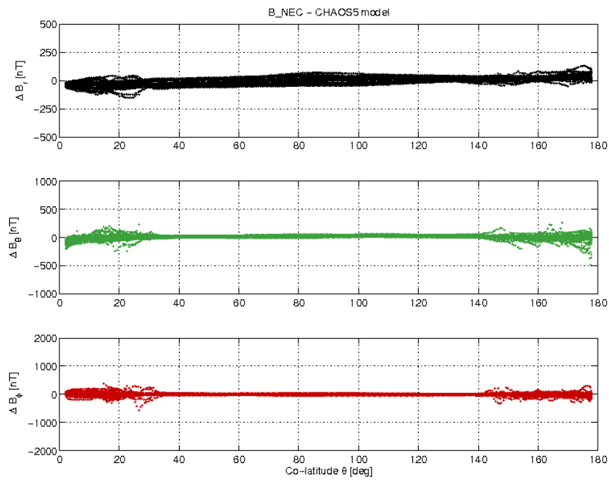
Figure 3-19: S/C B day 21/08 B_{NEC} - B_{Chaos} difference vs colatitude.
