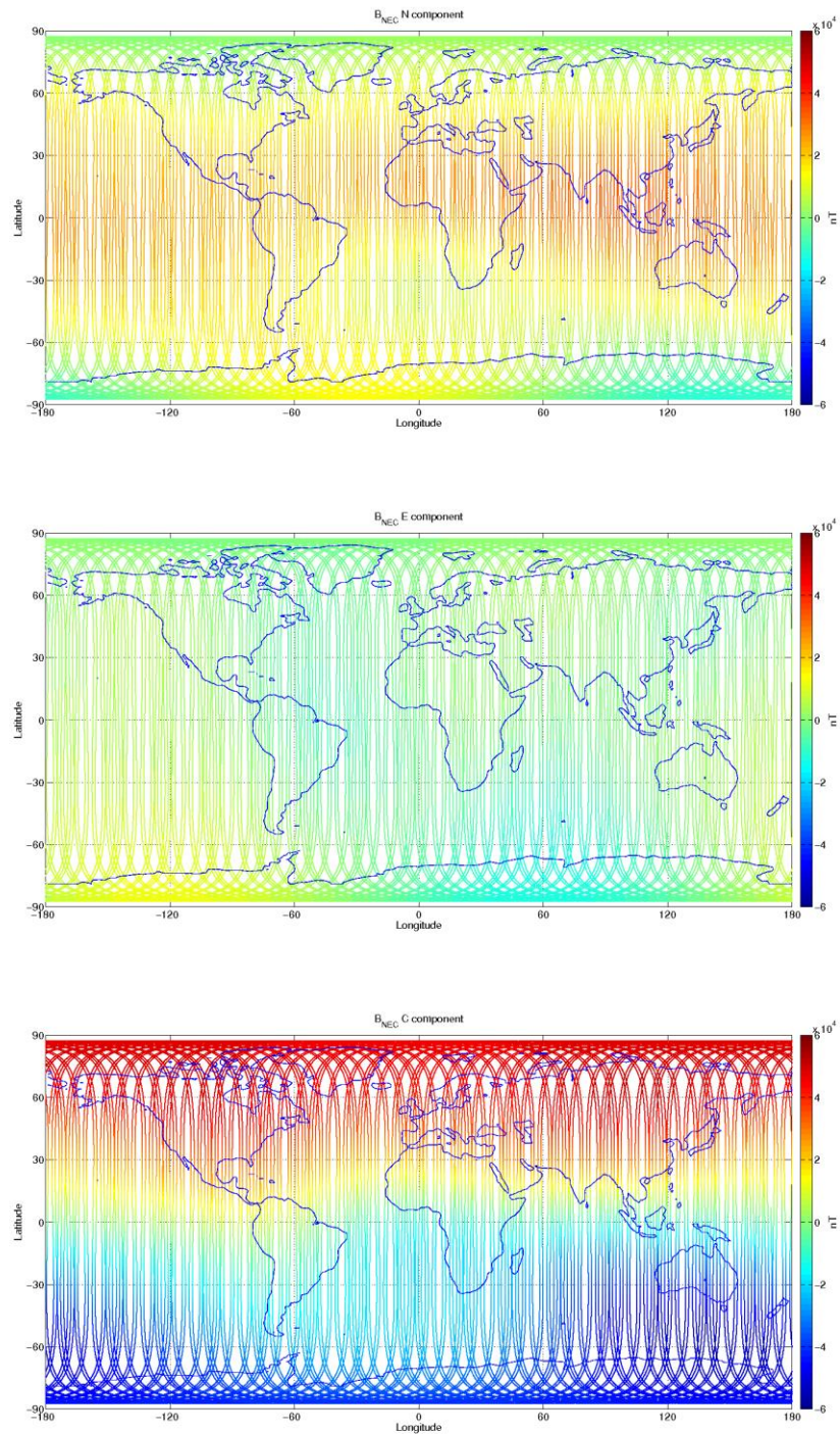
Figure 3-12: S/C C, world map plots of the geomagnetic field and components measured during monitoring period 21/08-27/08. From top to bottom: B_{NEC} components (North, East, and Centre) of magnetic field from VFM measurement.
