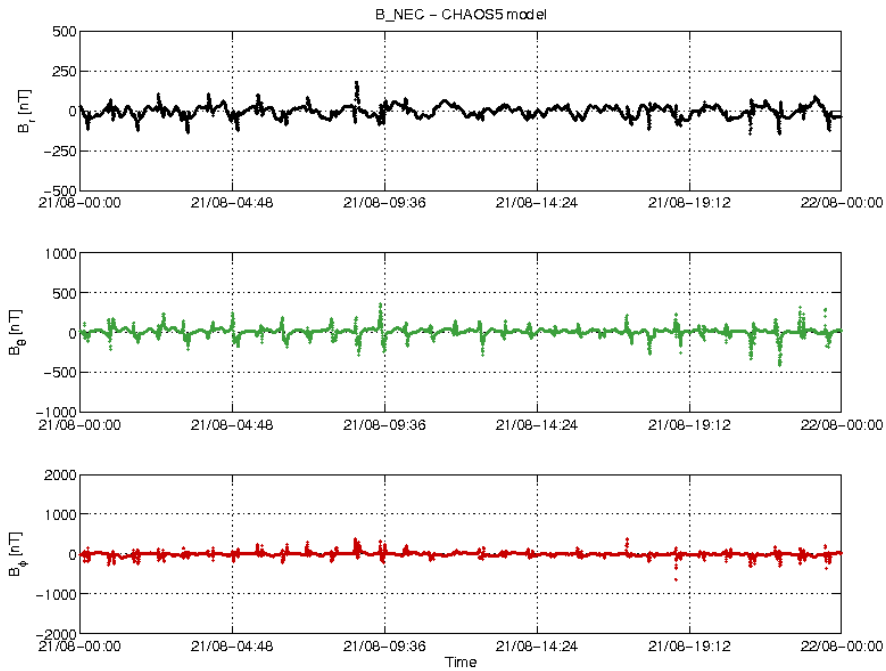
Figure 3-22: S/C C day 21/08 time series of B_{NEC} - B_{Chaos} residuals.
