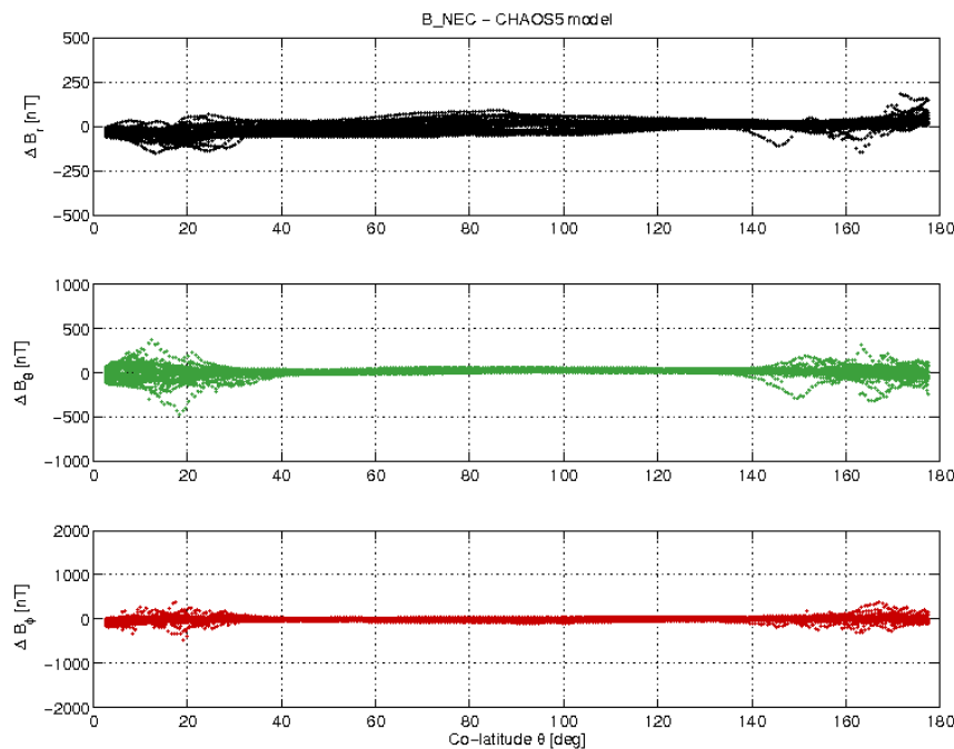
Figure 3-17: S/C A day 21/08 B_{NEC} - B_{Chaos} vs colatitude.
