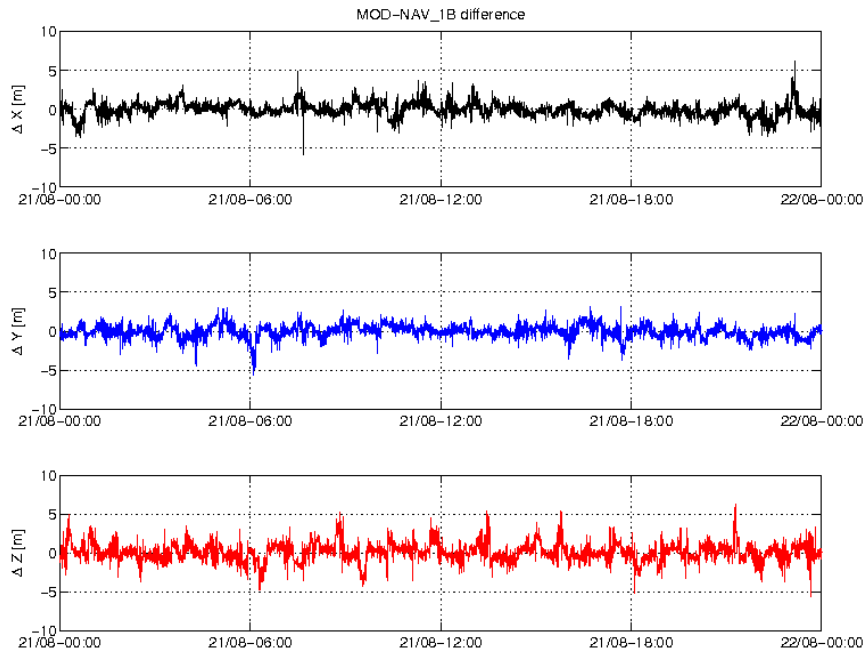
Figure 3-3: Difference MOD-GPSNAV, S/C A, 21/08. From top to bottom: X, Y and Z-axis
