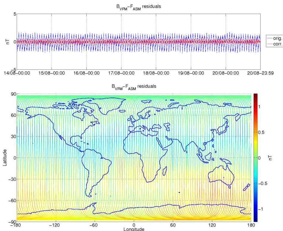
Figure 3-9: ASM-VFM residuals for S/C B, during monitoring period 14/08-20/08. In top figure are plotted: difference between |B_{VFM}| and F_{ASM} (without dB_{Sun} correction) (blue colour), and the residuals with dB_{Sun} corrections (red colour). In bottom figure residuals are presented on the world map.
