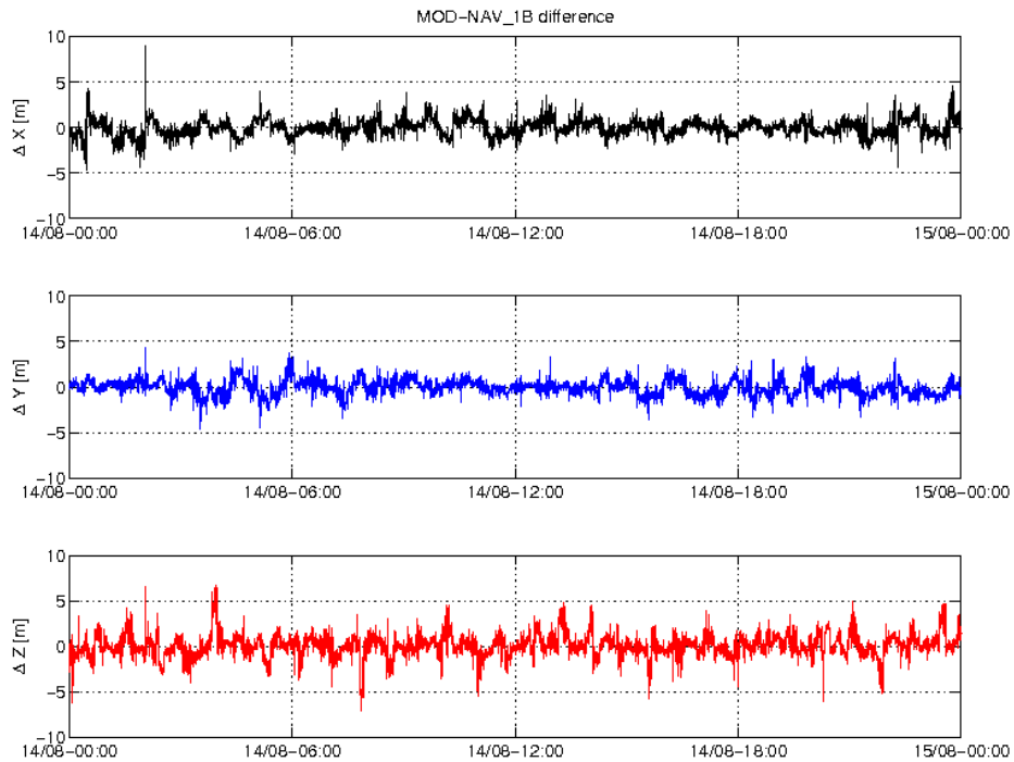
Figure 3-3: Difference MOD-GPSNAV, S/C A, 14/08. From top to bottom: X, Y and Z-axis
