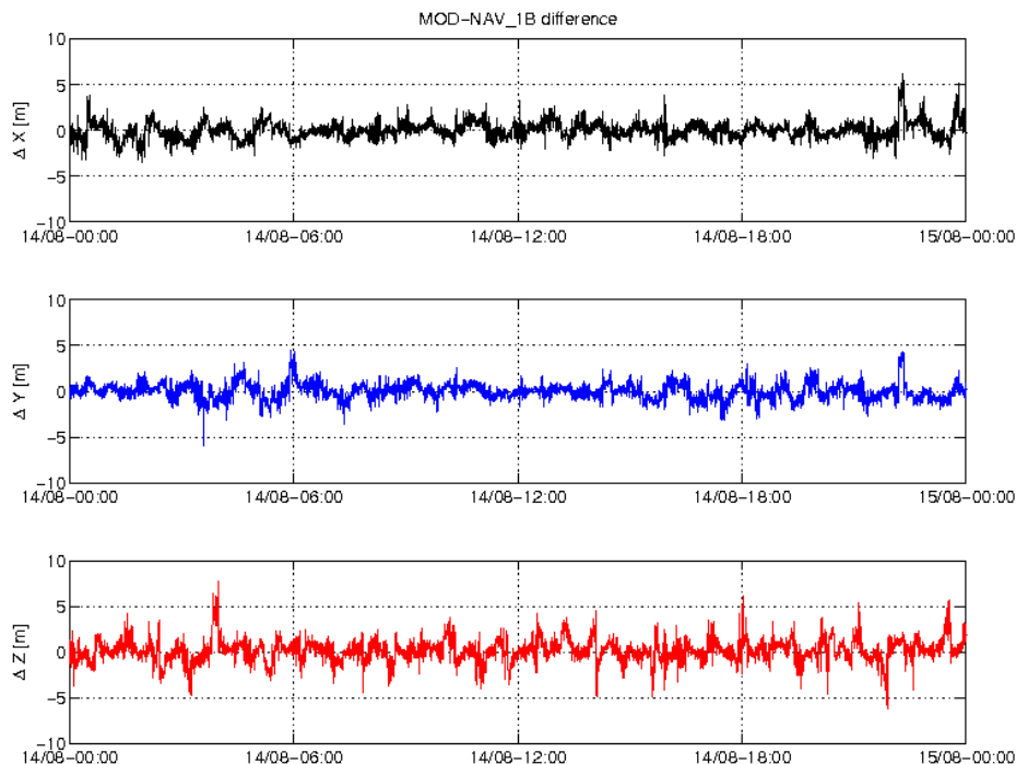
Figure 3-5: Difference MOD-GPSNAV, S/C C, 14/08. From top to bottom: X, Y and Z-axis
