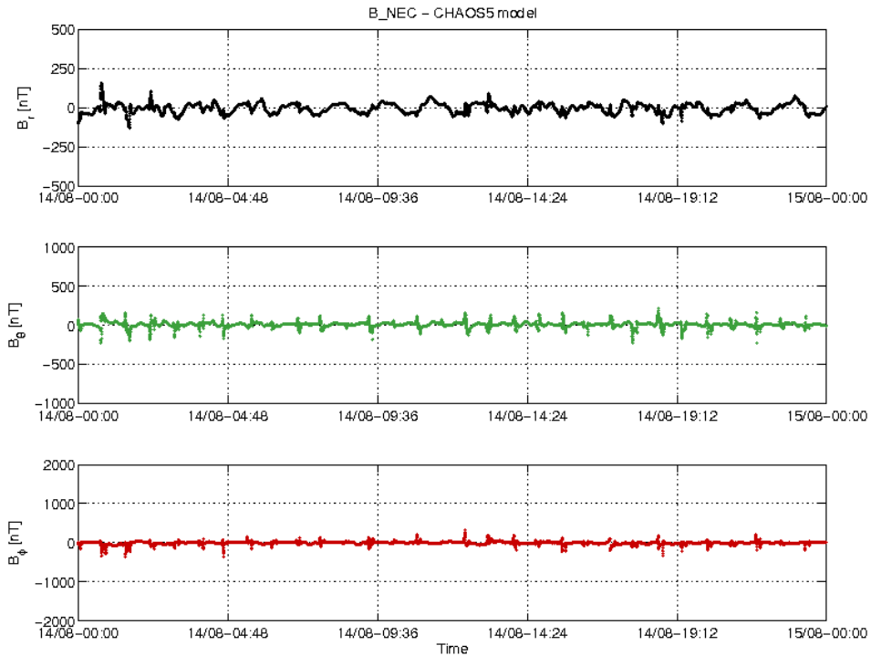
Figure 3-22: S/C C day 14/08 time series of B_{NEC} - B_{Chaos} residuals.
