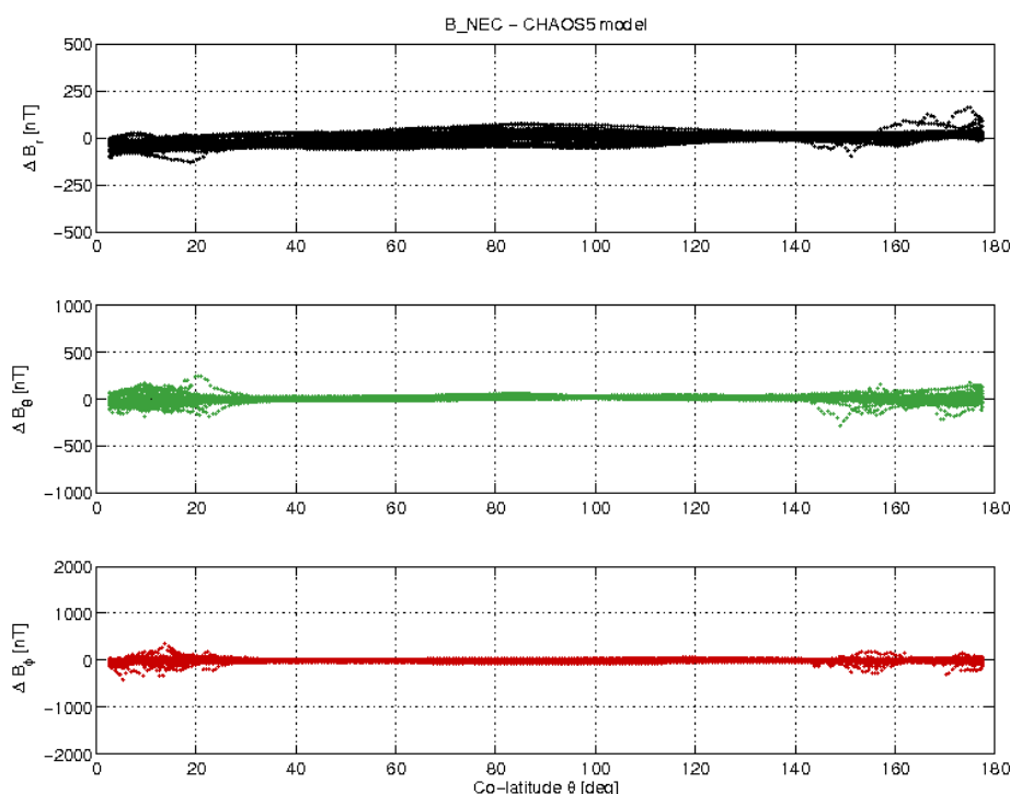
Figure 3-17: S/C A day 14/08 B_{NEC} - B_{Chaos} vs colatitude.
