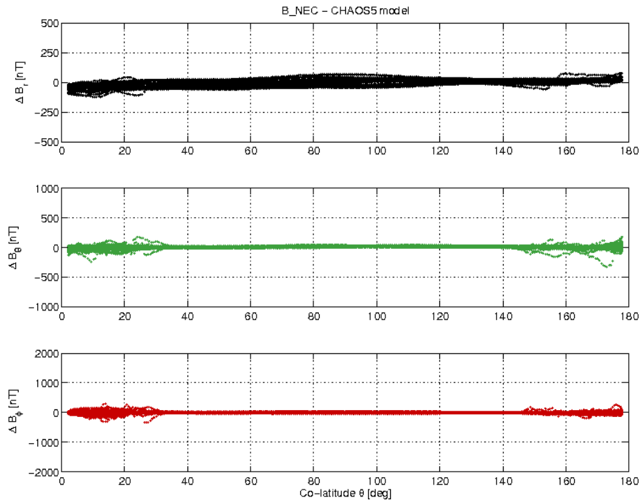
Figure 3-19: S/C B day 14/08 B NEC - B Chaos difference vs colatitude.
