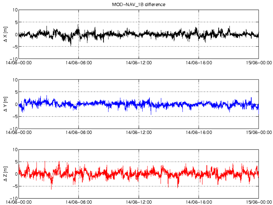
Figure 3-4: Difference MOD-GPSNAV, S/C B, 14/08. From top to bottom: X, Y and Z-axis
