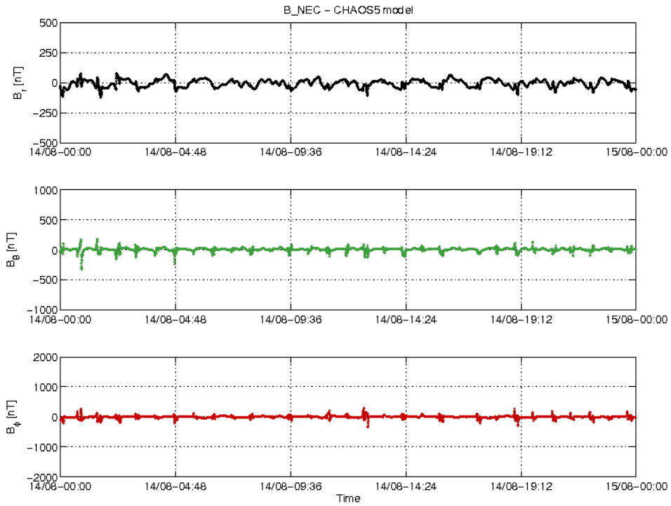
Figure 3-20: S/C B day 14/08 time series of B_{NEC} - B_{Chaos} residuals.
