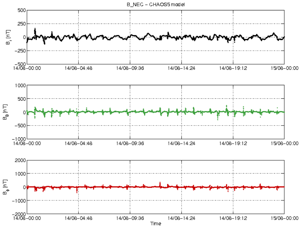
Figure 3-18: S/C A day 14/08: time series of B_{NEC} - B_{Chaos} residuals.
