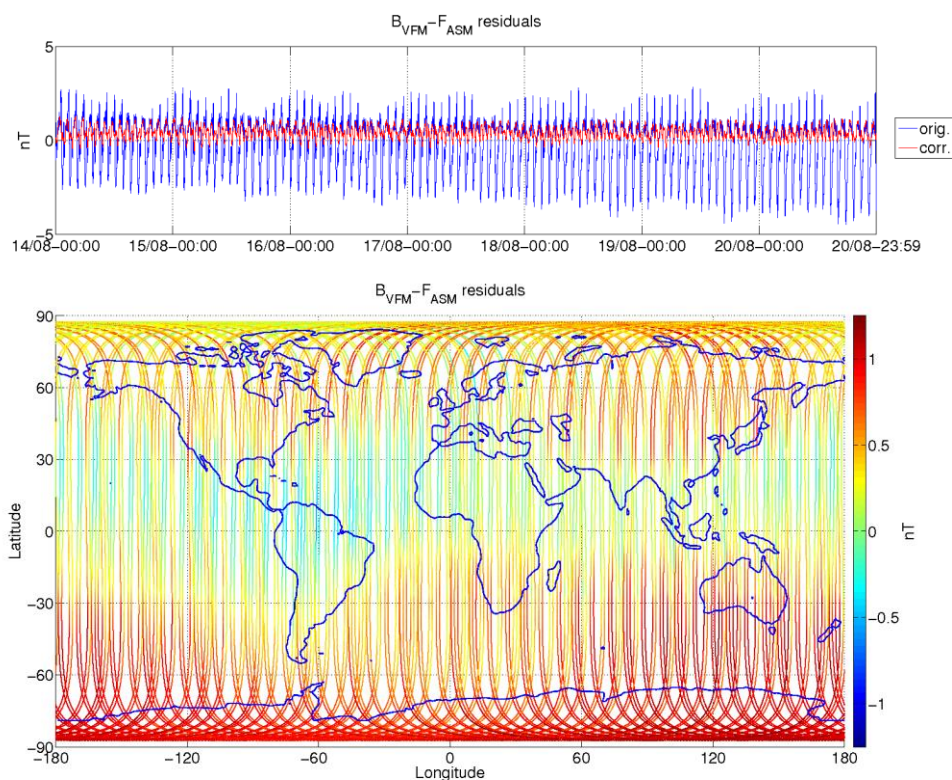
Figure 3-8: ASM-VFM residuals for S/C A, during monitoring period 14/08-20/08. In top figure are plotted: difference between |B_{VFM}| and F_{ASM} (without dB_Sun correction) (blue colour), and the residuals with dB_Sun corrections (red colour). In bottom figure residuals are presented on the world map.
