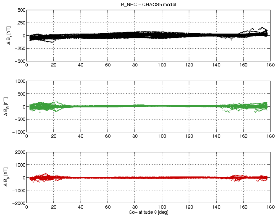
Figure 3-21: S/C C day 14/08 B_{NEC} - B_{Chaos} difference vs colatitude.
